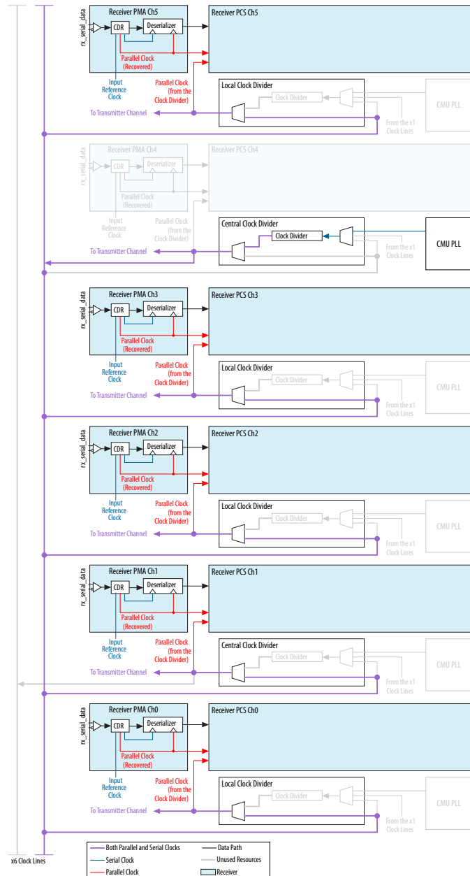
Figure 2-30: Five Bonded Receiver Channels with Rate Match FIFO Enabled
