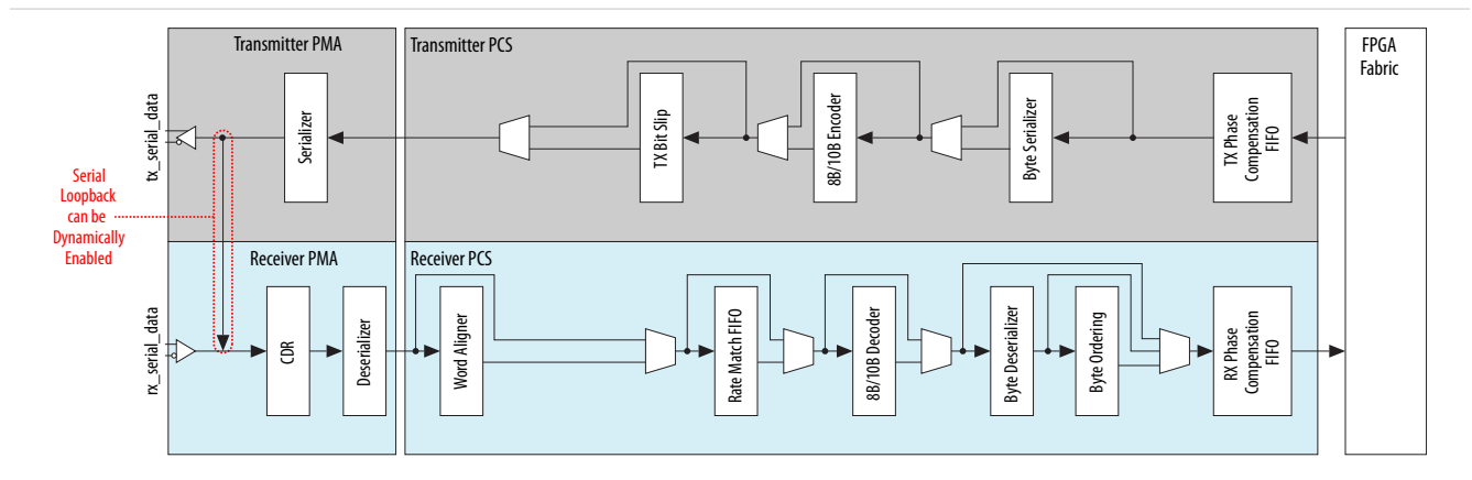
Figure 7-1: Serial Loopback Datapath
