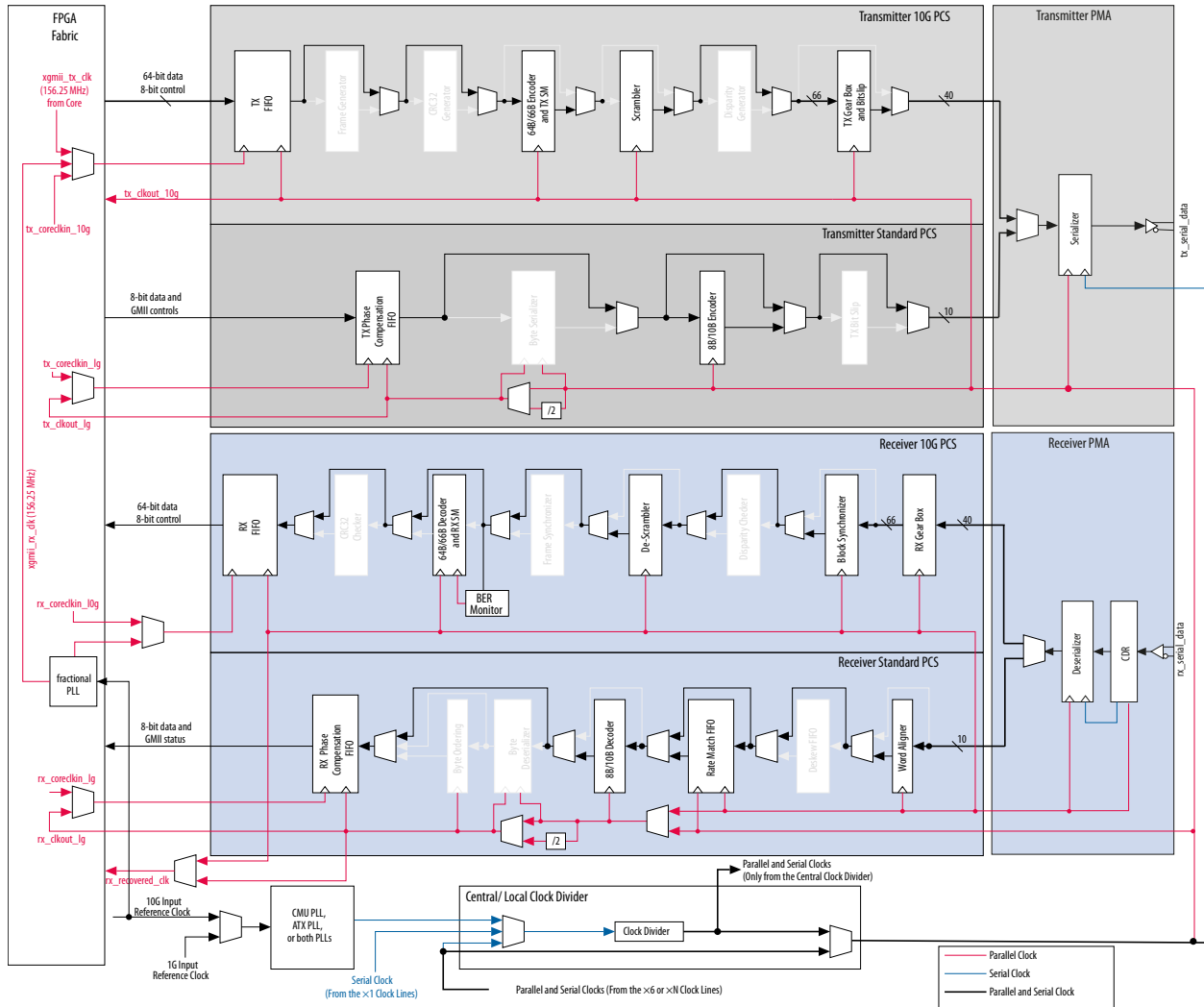
Figure 6-6: Transceiver Channel Datapath for 10GBASE-R/KR and 1000BASE-X/KX Configuration
