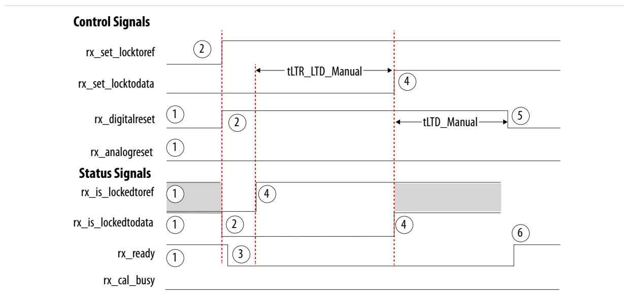
Figure 3-9: Reset Sequence Timing Diagram for Receiver when CDR is in Manual Lock Mode
