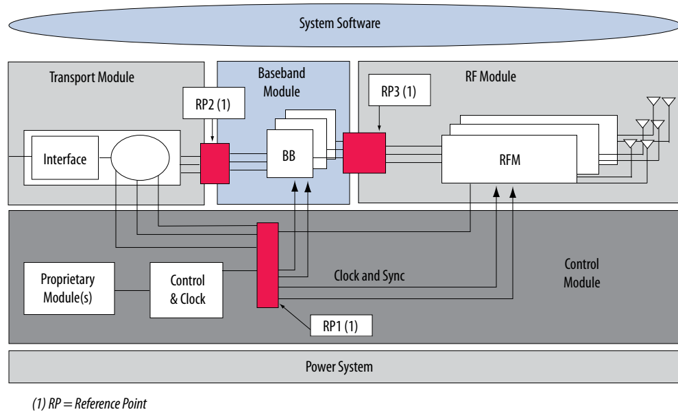
Figure 4-39: Example of the OBSAI BTS Architecture
