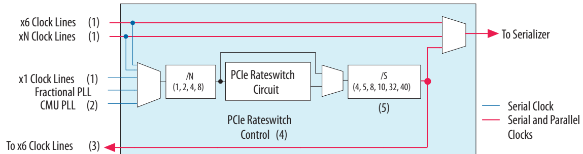
Figure 1-21: Clock Divider for a Transceiver Channel in Arria V Devices
