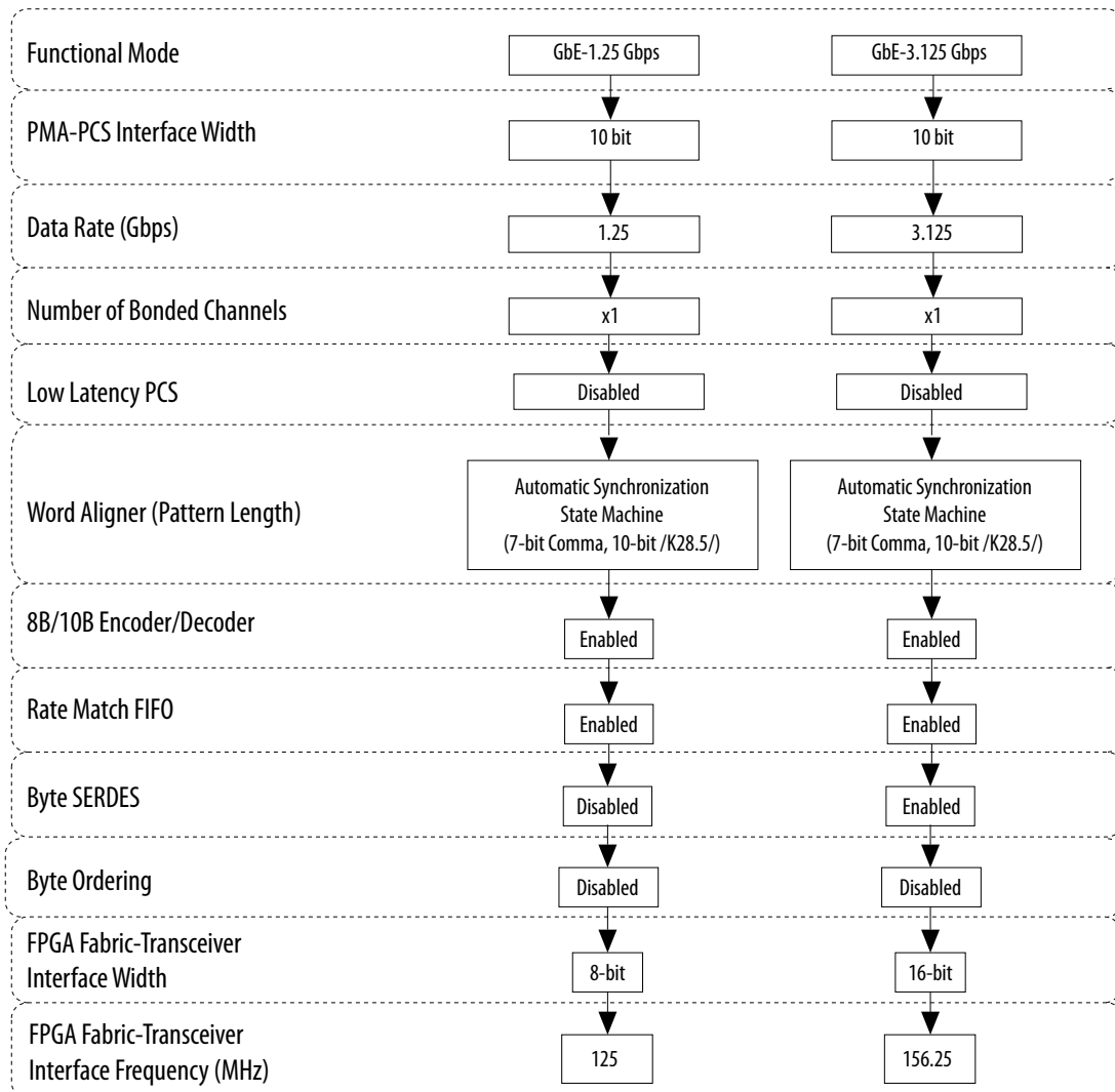
Figure 4-17: Transceiver Blocks in a GbE Configuration
