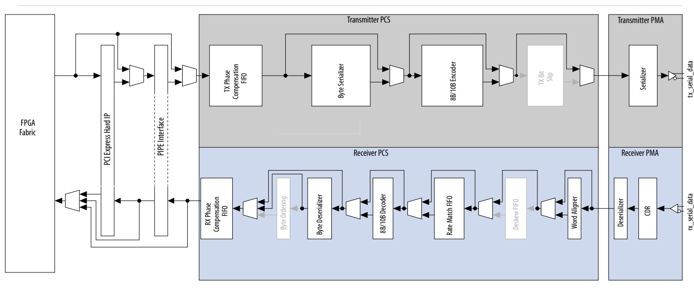
Figure 4-4: Transceiver Channel Datapath in a PIPE Configuration
