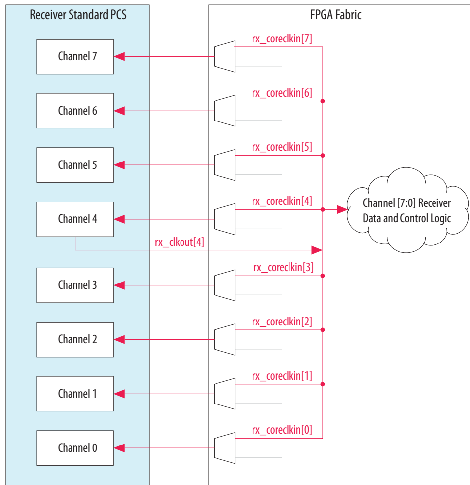
Figure 2-44: Eight Identical Channels with a Single User-Selected Receiver Interface Clock
