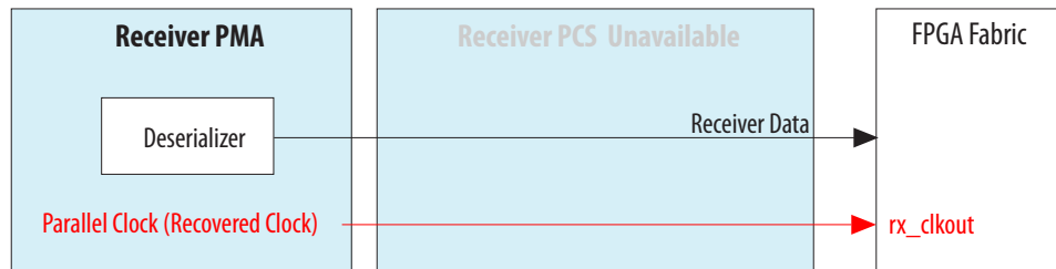
Figure 2-40: Arria V GT/ST 10-Gbps Receiver Datapath Interface Clocking
