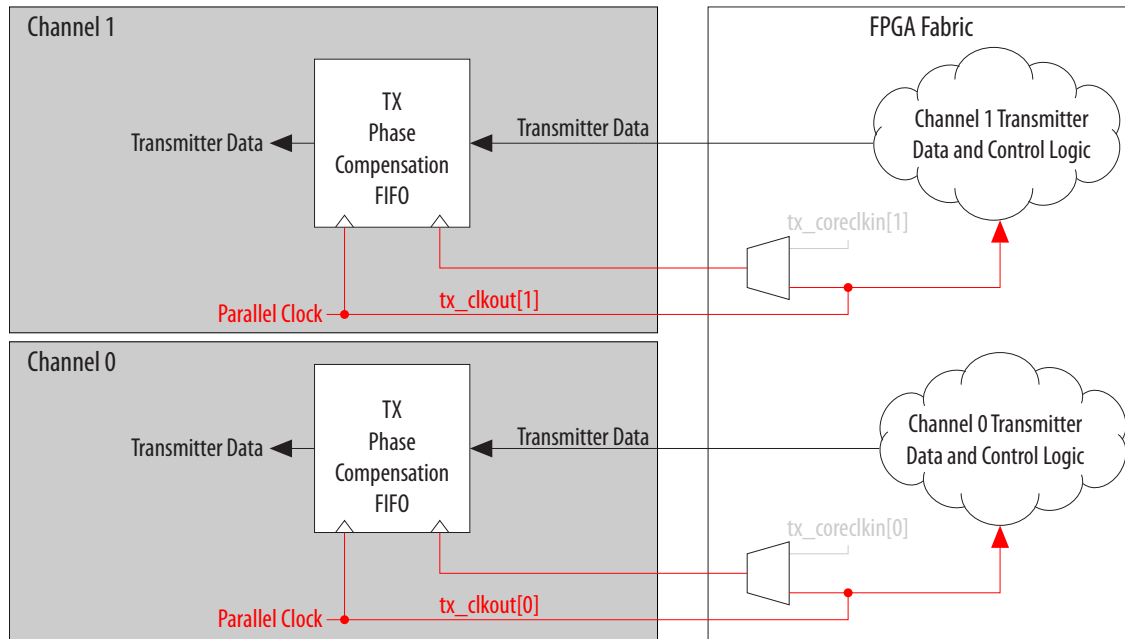
Figure 2-36: Arria V GT/ST 10-Gbps Transmitter Datapath Interface Clocking for Non-Bonded Channels
