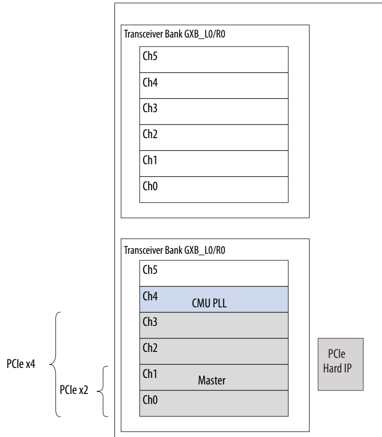
Figure 4-11: PCIe HIP Supported x2 and x4 Guidelines
