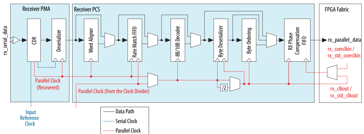
Figure 2-25: Clocking Architecture for Receiver PCS and PMA Configuration
