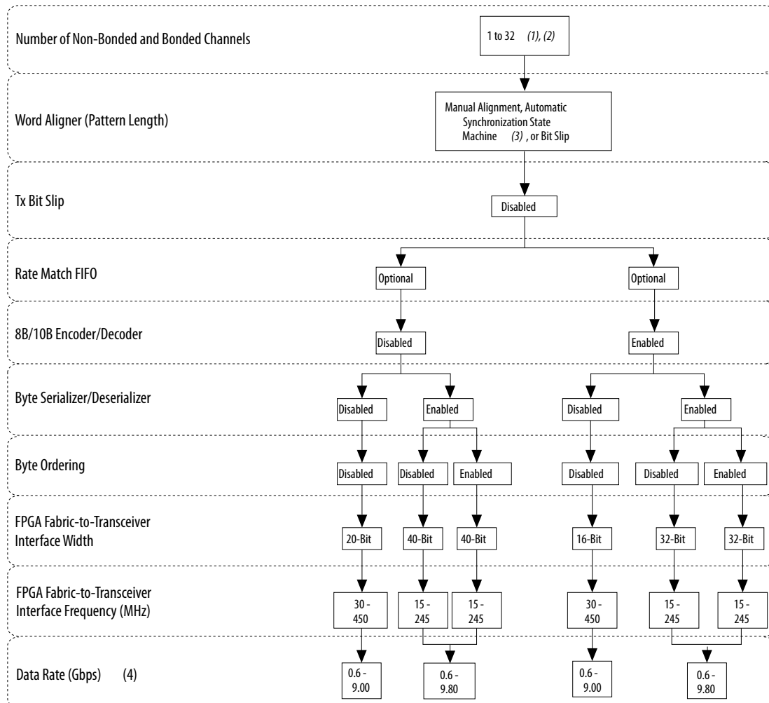
Figure 6-56: Standard PCS Custom 20-Bit PMA-PCS Interface Width
