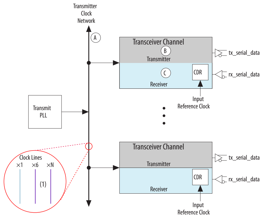
Figure 2-9: Internal Clocking
