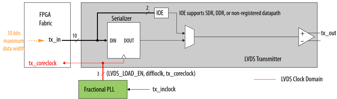
Figure 6-21: LVDS Transmitter
