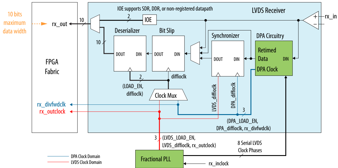
Figure 6-26: Receiver Block Diagram
