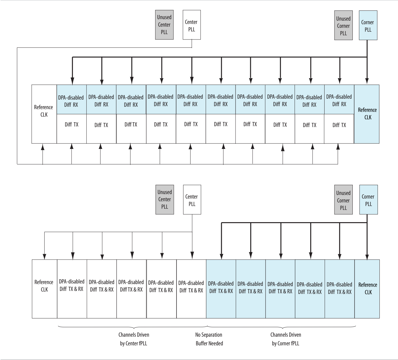
Figure 6-17: Corner and Center PLLs Driving DPA-Disabled Differential I/Os in the Same Bank
