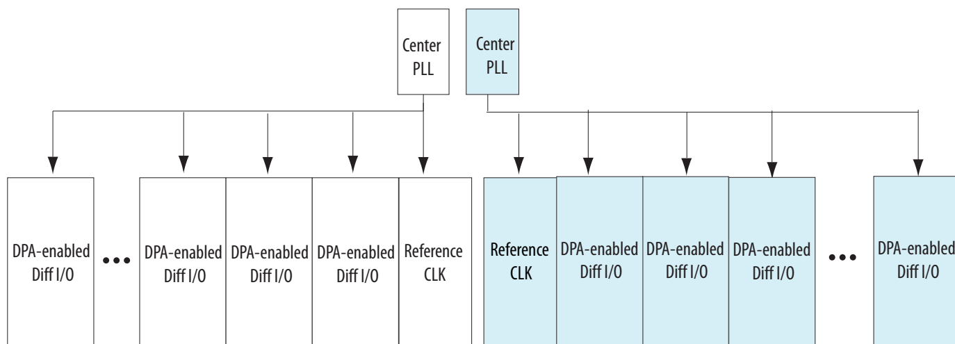
Figure 6-15: Invalid Placement of DPA-enabled Differential I/Os Driven by Both Center PLLs
