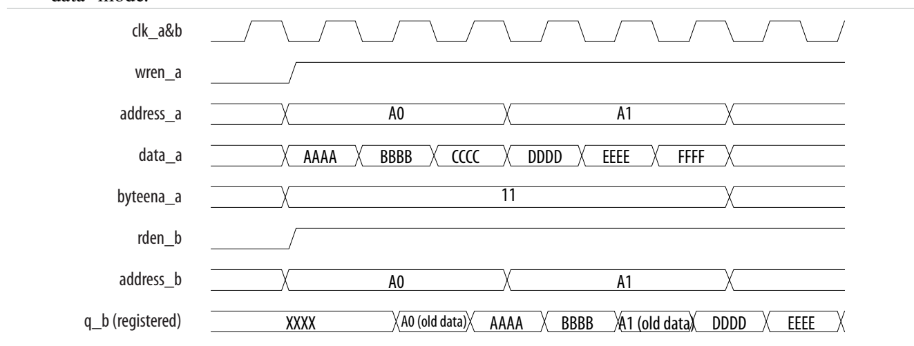
Figure 2-5: Mixed-Port Read-During-Write: Don't Care or Constrained Don't Care Mode
