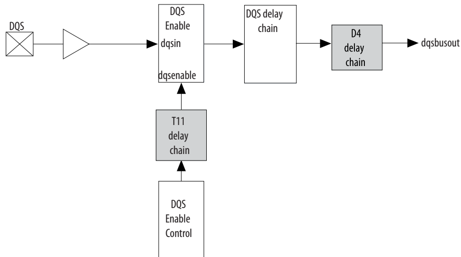
Figure 7-23: Delay Chains in the DQS Input Path
