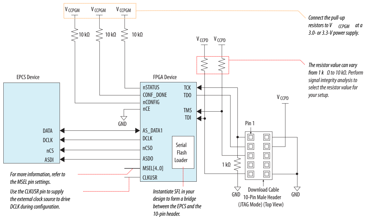
Figure 8-12: Connection Setup for Programming the EPCS Using the JTAG Interface
