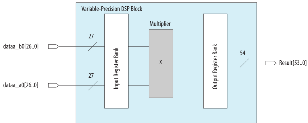
Figure 3-16: One 27 x 27 Independent Multiplier Mode per Variable Precision DSP Block for Arria V Devices
