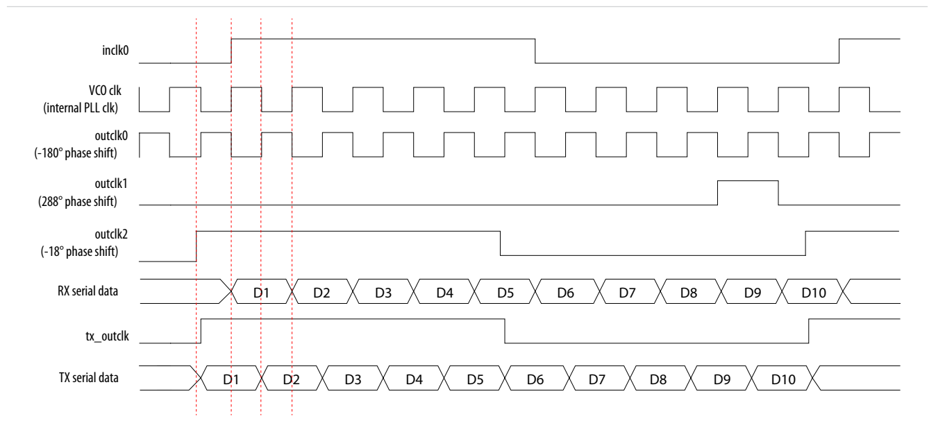
Figure 6-7: Phase Relationship for External PLL Interface Signals
