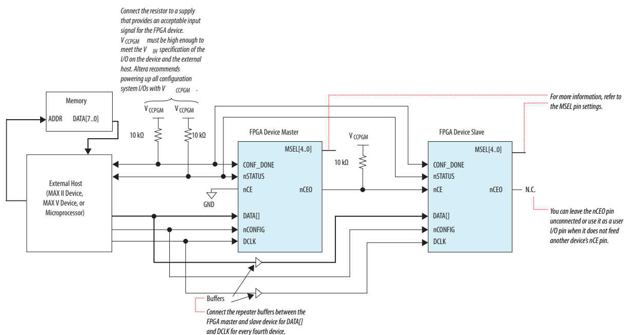
Figure 8-7: Multiple Device FPP Configuration Using an External Host When Both Devices Receive a Different Set of Configuration Data
