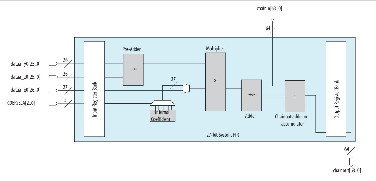
Figure 3-39: 27-Bit Systolic FIR Mode for Arria V GZ Devices
