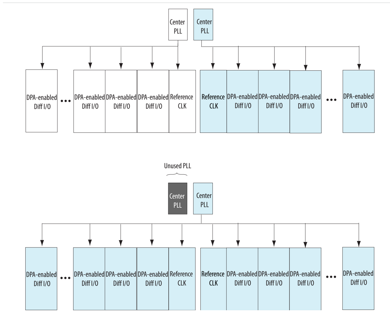
Figure 6-13: Center PLLs Driving DPA-enabled Differential I/Os in Arria V GX, GT, SX, and ST Devices
