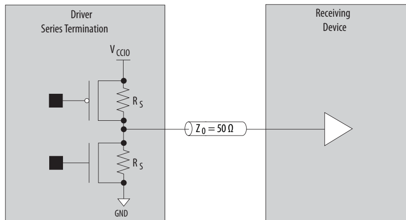
Figure 5-8: R_S OCT Without Calibration
