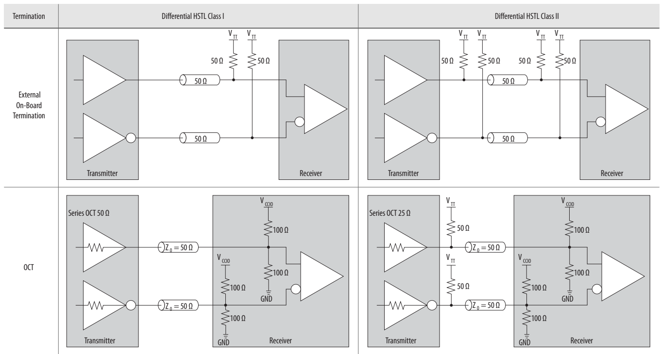
Figure 5-18: Differential HSTL I/O Standard Termination
