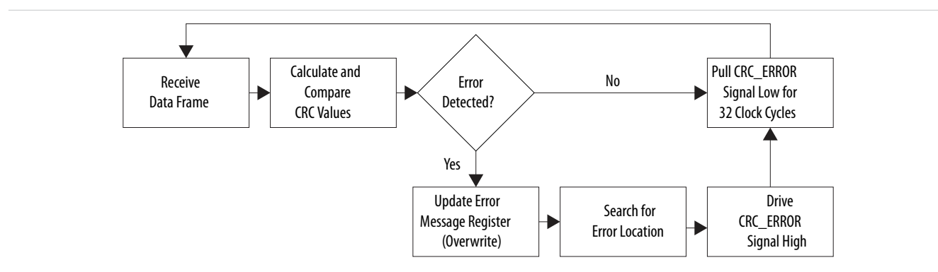
Figure 9-4: Error Detection Process Flow in User Mode
