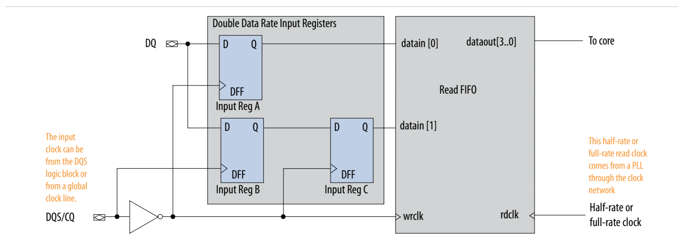
Figure 7-18: IOE Input Registers for Arria V Devices
