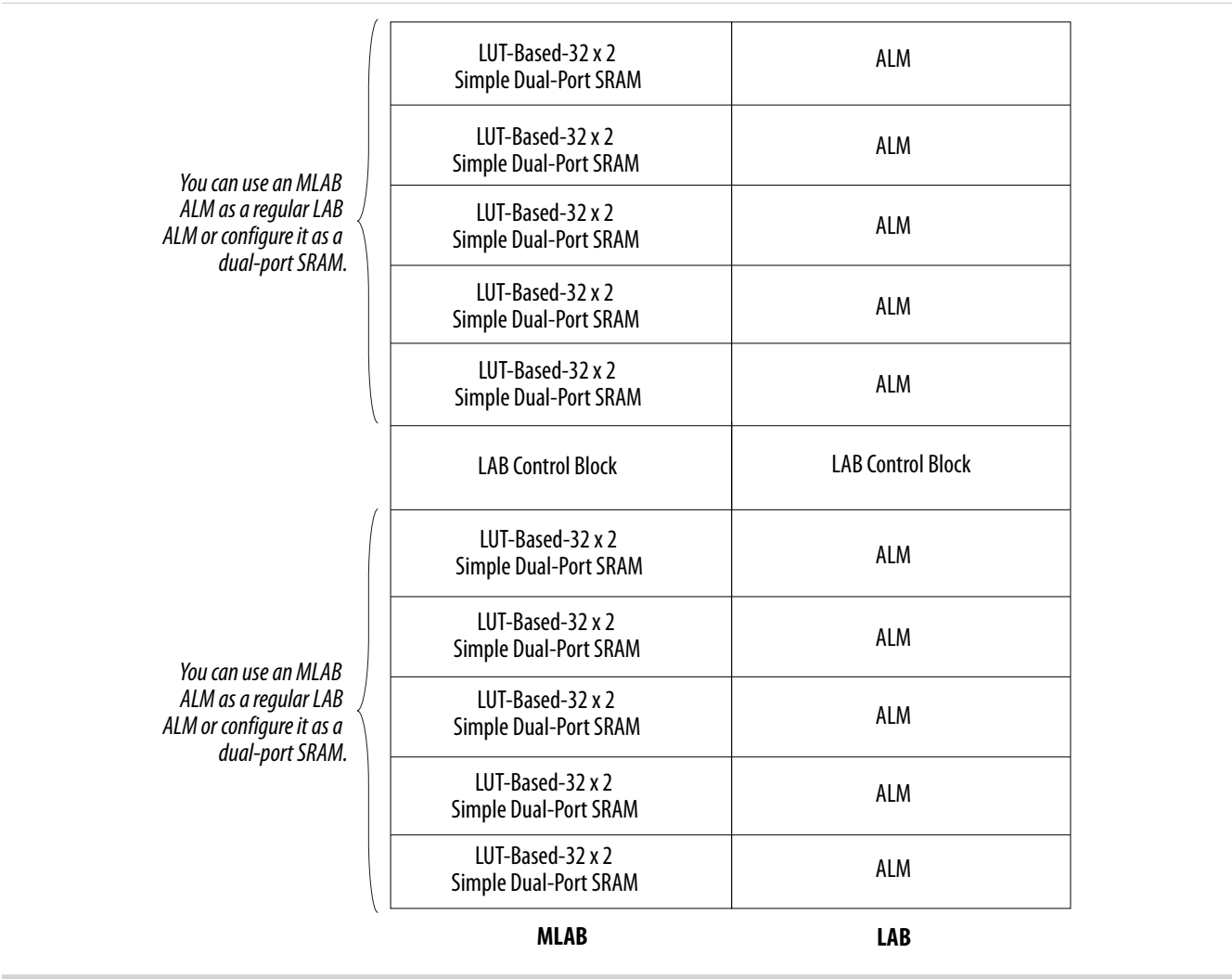
Figure 1-2: LAB and MLAB Structure for Arria V GX, GT, SX, and, ST Devices
