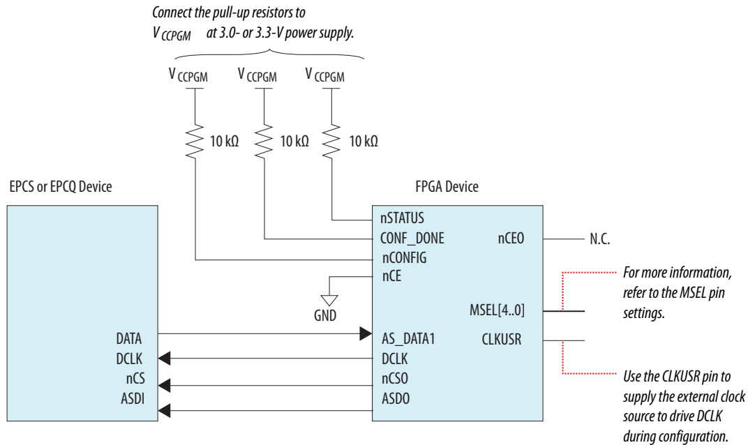
Figure 8-9: Single Device AS x1 Mode Configuration
