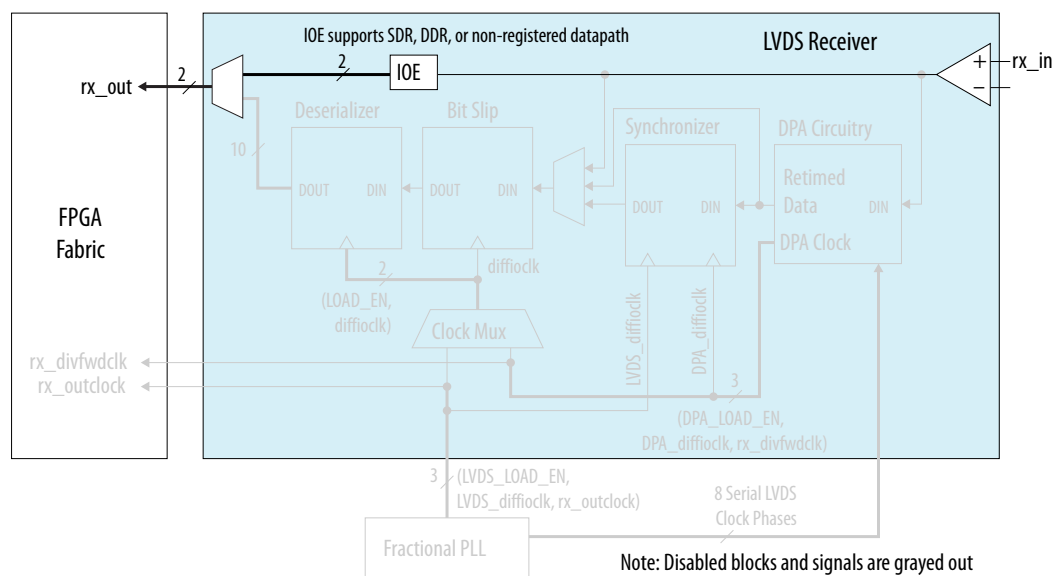
Figure 6-30: Deserializer Bypass
