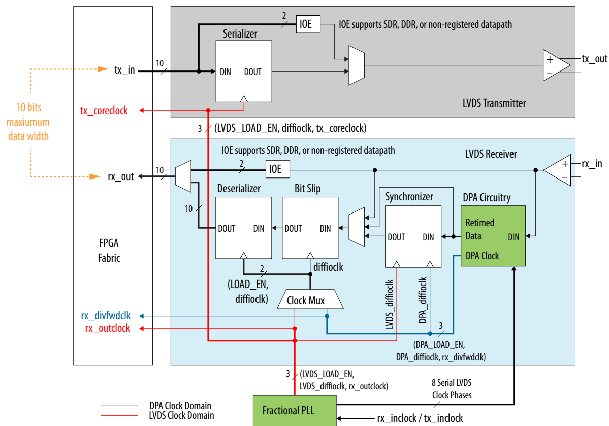
Figure 6-6: LVDS SERDES
