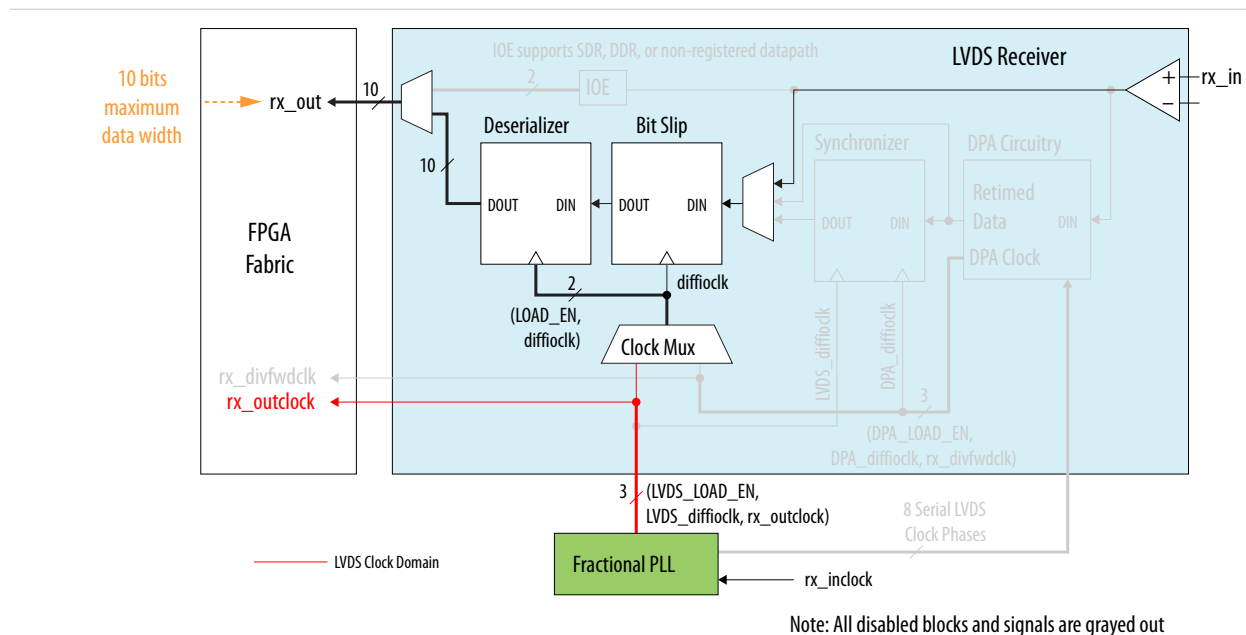
Figure 6-31: Receiver Data Path in Non-DPA Mode
