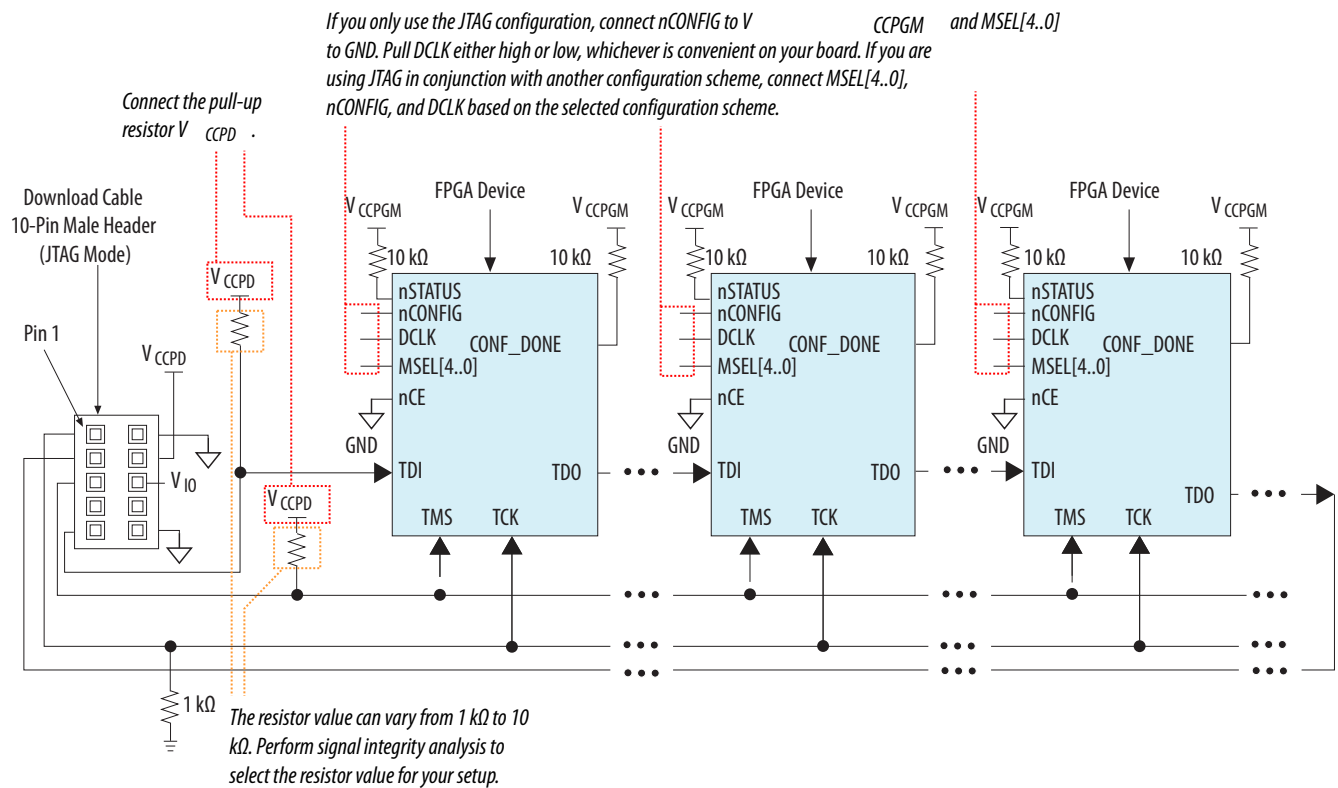
Figure 8-23: JTAG Configuration of Multiple Devices Using a Download Cable
