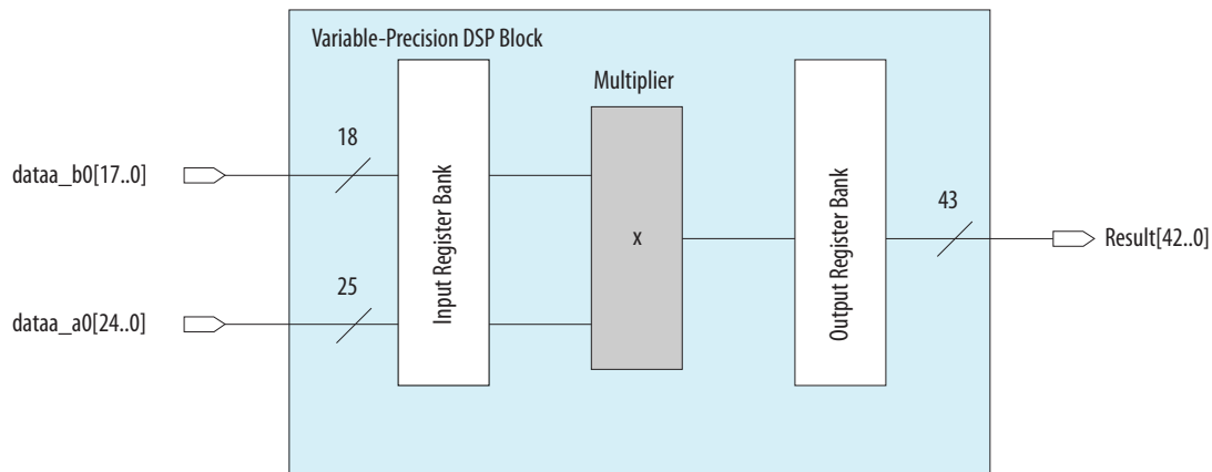
Figure 3-14: One 18 x 25 Independent Multiplier Mode per Variable Precision DSP Block for Arria V GX, GT, SX, and ST Devices
