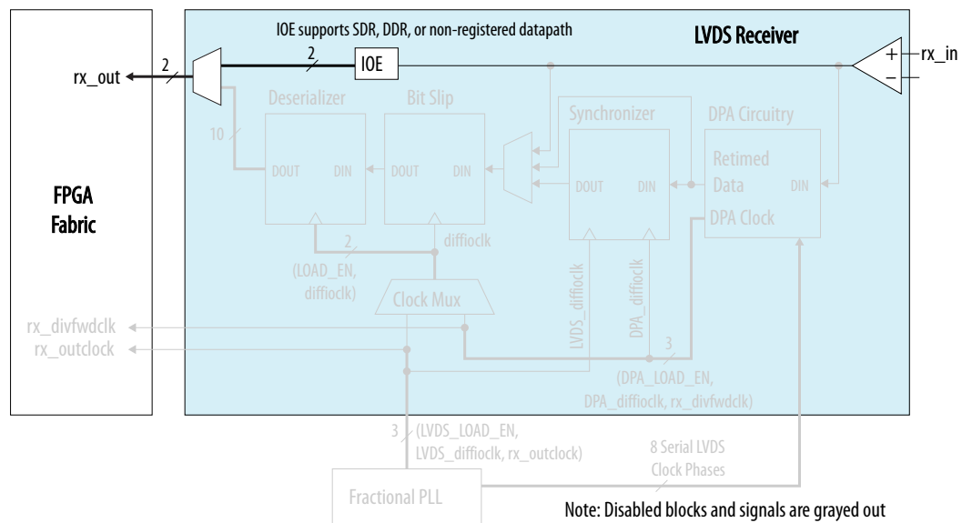
Figure 6-30: Deserializer Bypass
