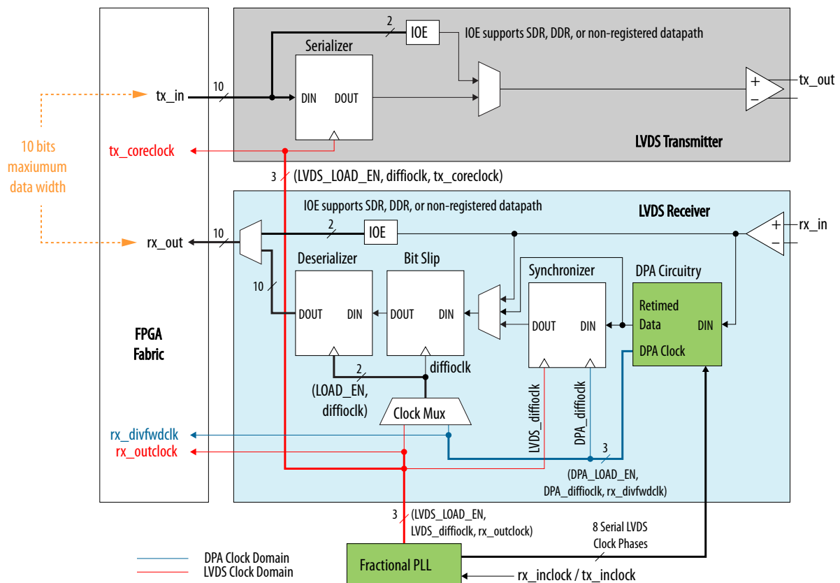
Figure 6-6: LVDS SERDES
