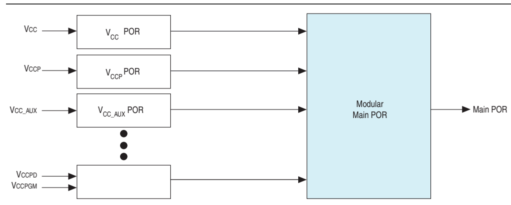
Figure 11-4. Simplified POR Diagram for Arria V Devices
