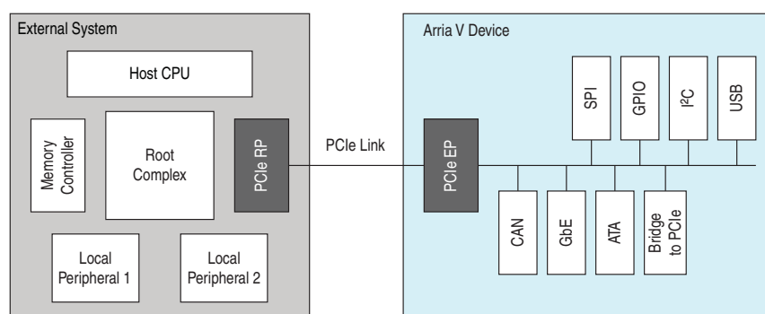
Figure 4-1. PCIe Multifunction for Arria V Devices
