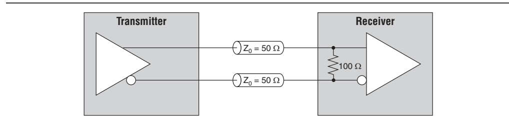
Figure 5-11. Differential Input OCT
