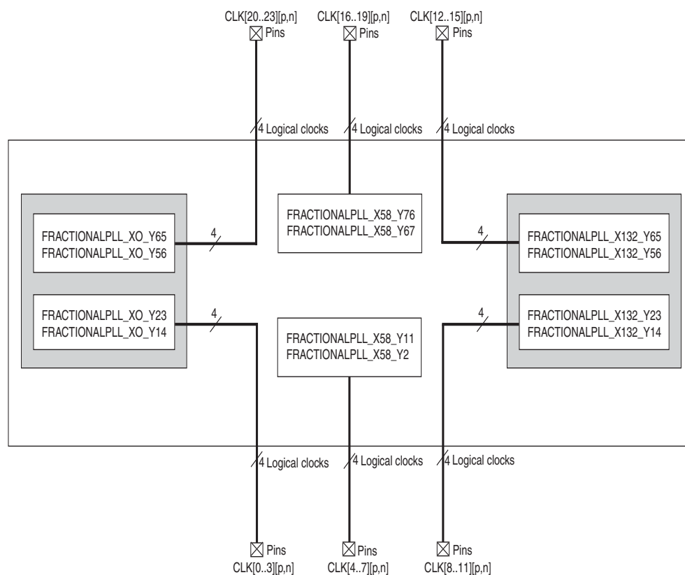
Figure 4–13. PLL Locations for Arria V GX A5 and A7 Devices, and Arria V GT C7 (1) Device
