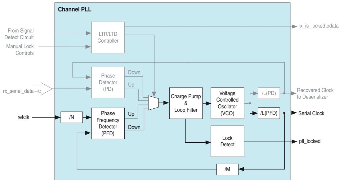
Figure 1-13. CMU PLL in Arria V Devices
