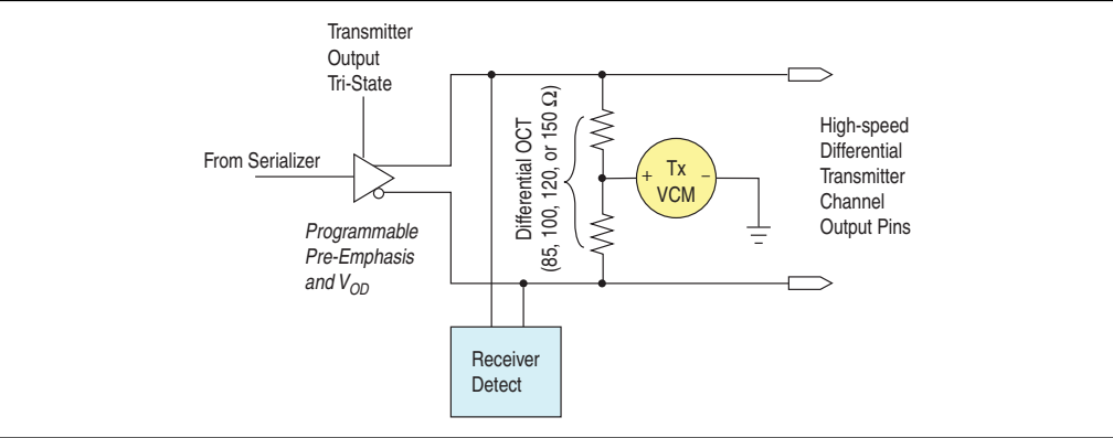
Figure 1-7. Transmitter Buffer in Arria V Devices
