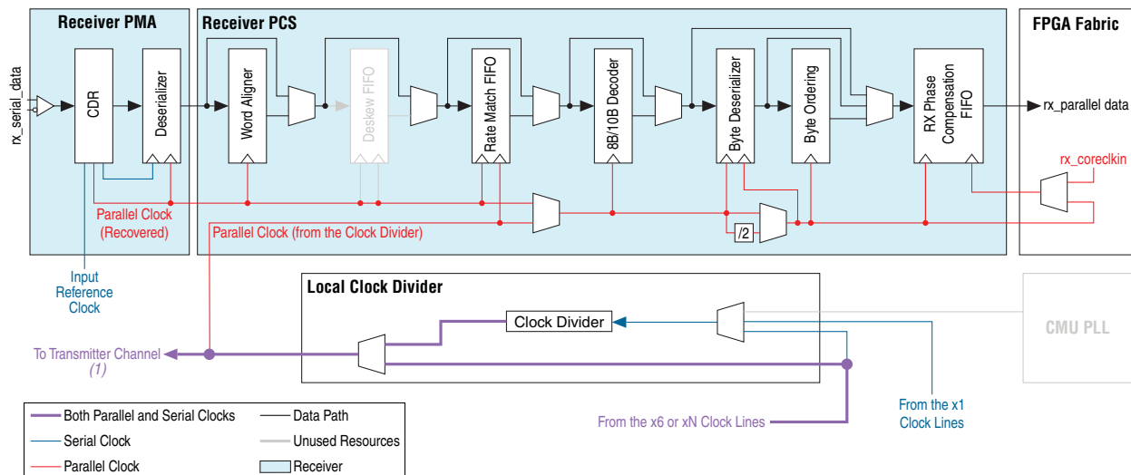
Figure 2-15. Receiver PCS Clocking for 6-Gbps Transceivers
