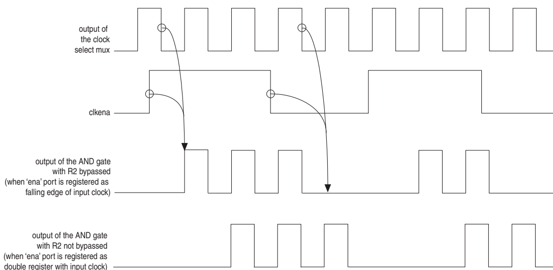
Figure 4-11. clkena Signals (1)
