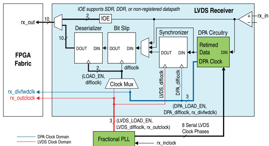
Figure 6-10. Receiver Block Diagram (1) , (2)
