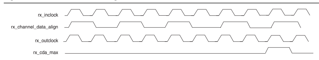
Figure 6-13. Receiver Data Realignment Rollover
