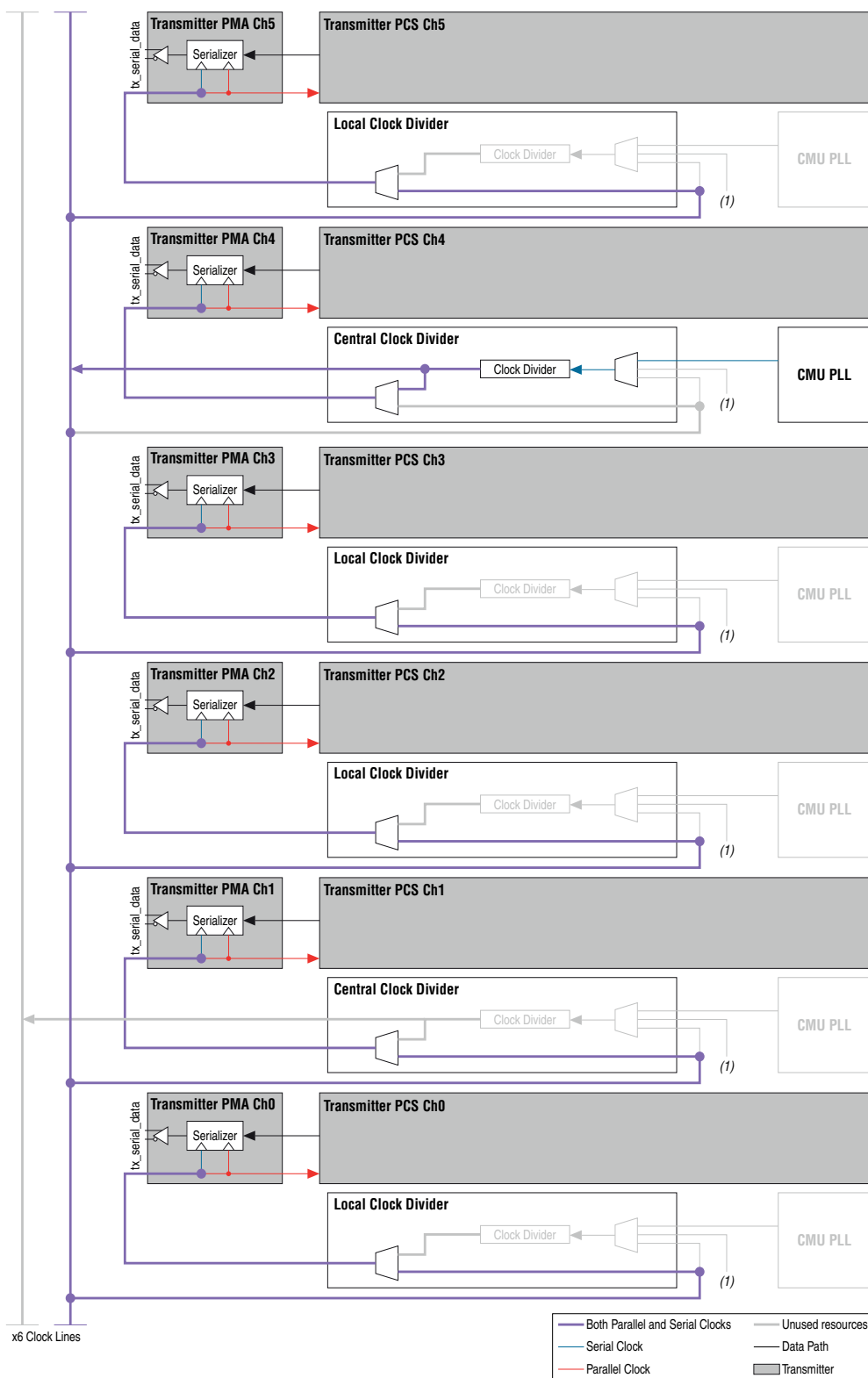
Figure 2-14. Six Transmitter Channels Configured in Bonded Configuration
