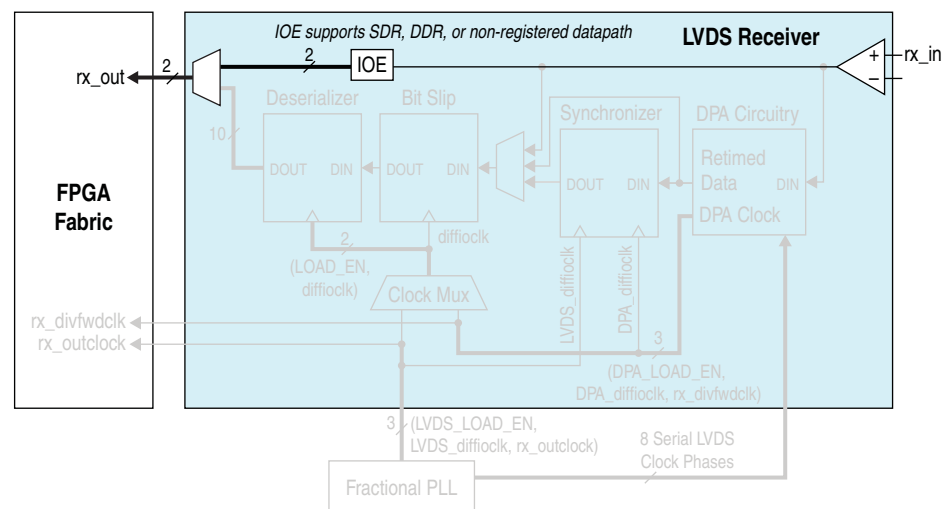
Figure 6-14. Deserializer Bypass (1), (2), (3)
