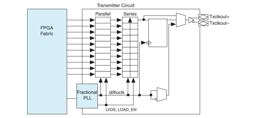
Figure 6–6. Arria V Transmitter in Clock Output Mode
