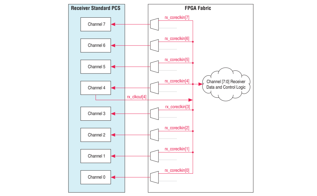
Figure 2–31. Eight Identical Channels with a Single User-Selected Receiver Interface Clock
