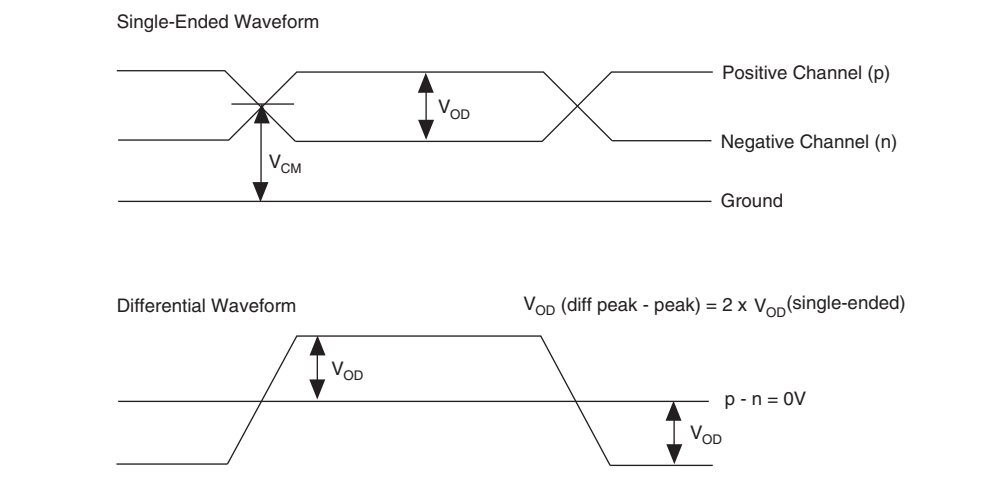
Figure 6-8. Differential V_{OD}
