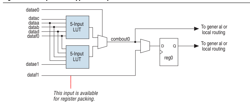
Figure 1-7. Template for Supported 7-Input Functions in Extended LUT Mode in Arria V Devices
