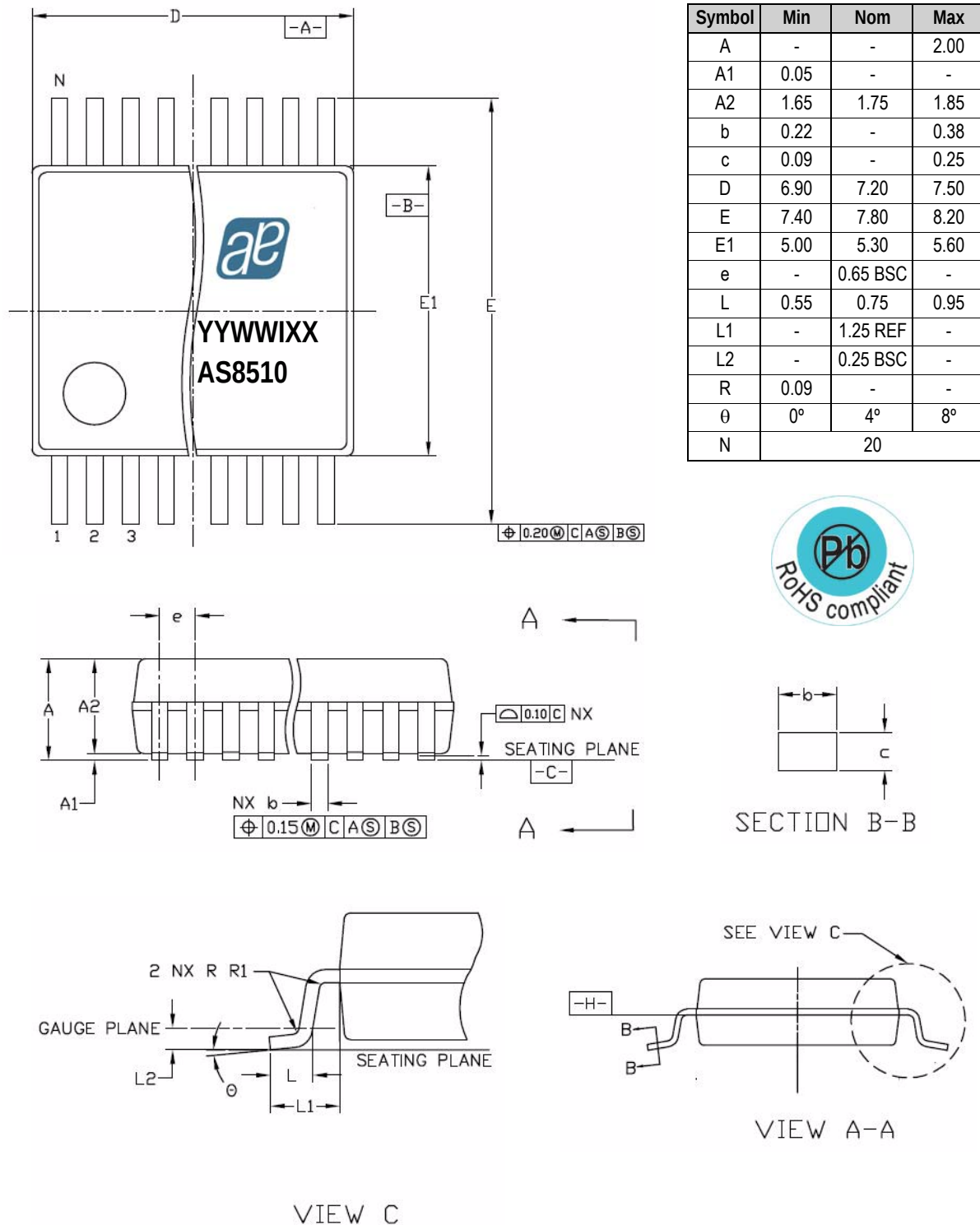
Figure 20. Drawings and Dimensions
