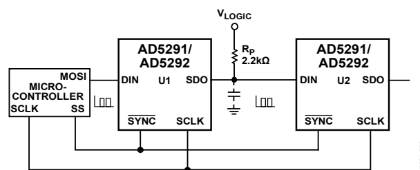
Figure 64. Daisy-Chain Configuration Using SDO
