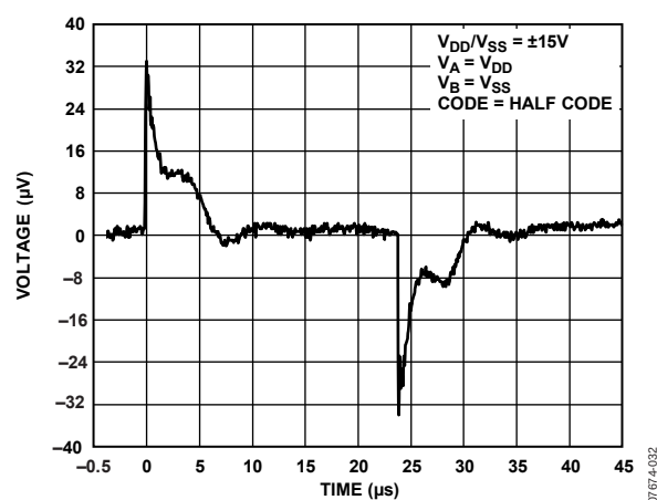
Figure 53. Digital Feedthrough
