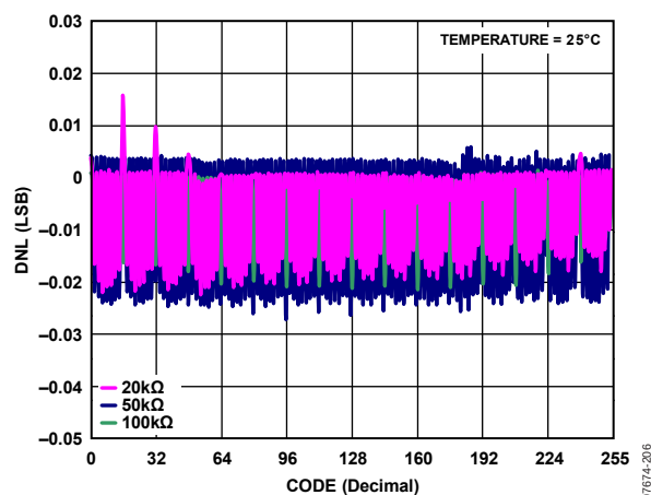
Figure 39. DNL in Normal Mode vs. Code vs. Temperature (AD5291)
