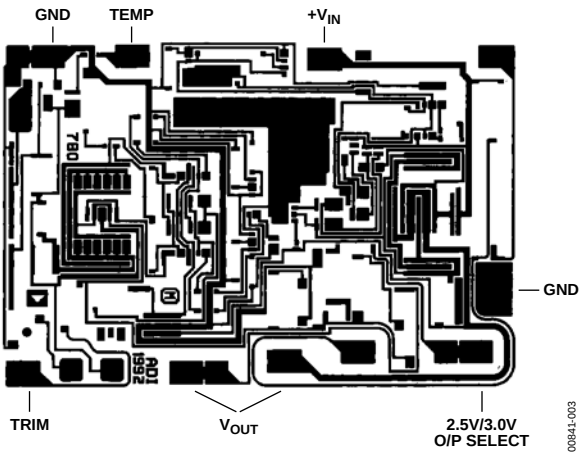
Figure 3. Die Layout
