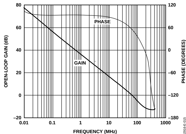
Figure 15. Open-Loop Response
