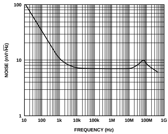
Figure 21. Voltage Noise
