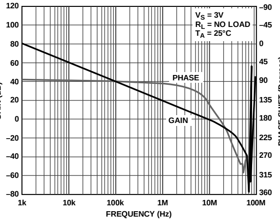
Figure 22. Open-Loop Gain and Phase vs. Frequency
