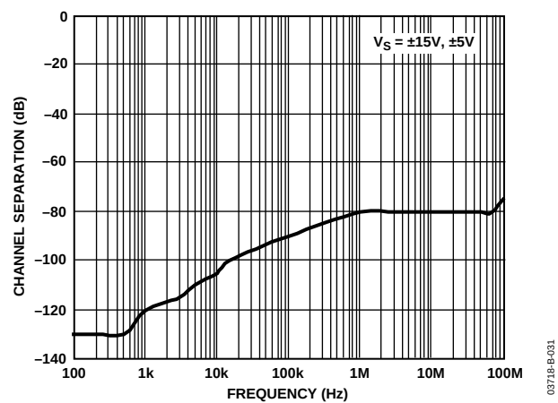
Figure 31. Channel Separation
