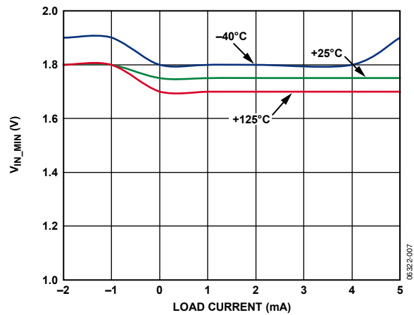
Figure 7. Minimum Input Voltage vs. Load Current, V_{OUT} = 1 V
