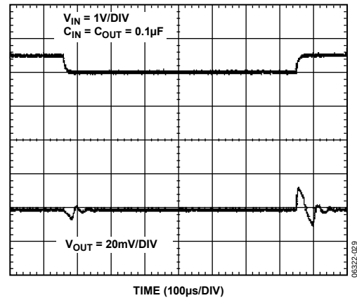
Figure 29. Line Transient Response, V_{OUT} = 1\text{ V}
