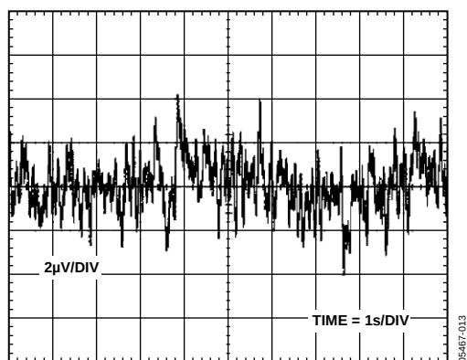
Figure 15. ADR361 0.1 Hz to 10 Hz Noise
