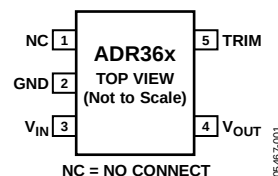
Figure 1. 5-Lead TSOT (UJ)
