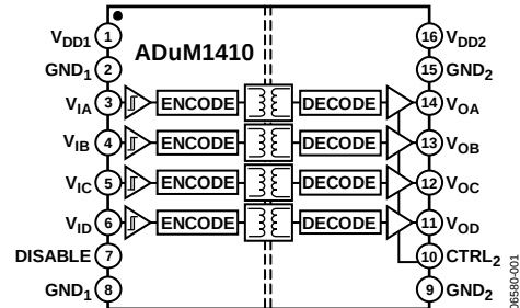
Figure 1. ADuM1410
