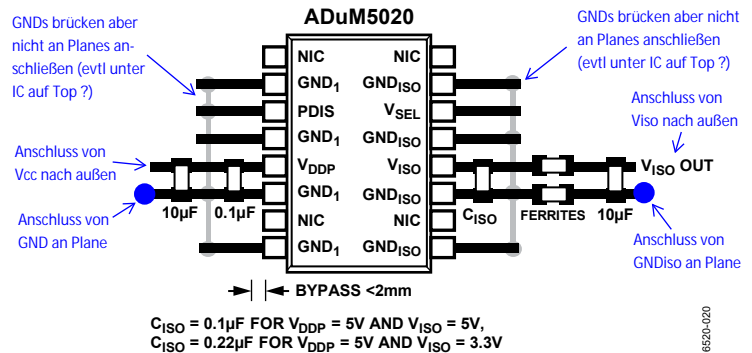
Figure 25. Recommended ADuM5020 PCB Layout
