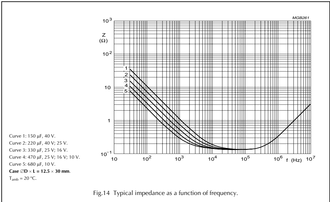
Fig.13 Typical impedance as a function of frequency.
