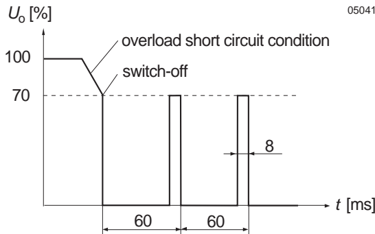
Fig. 14 Overload switch-off (hiccup mode). Frequency of pulses: 16.5 Hz, puls duration: 8.5 ms.
