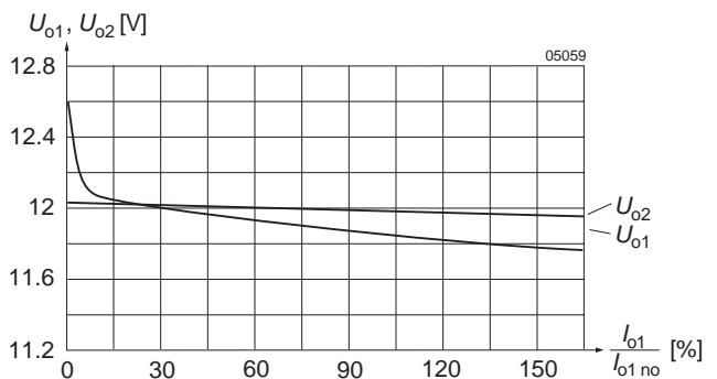
Fig. 13 Flexible load distribution on dual outputs ( 2 \times 12 V) with load variation from 0...150% of P_{o1\text{nom}} on output 1. Output 2 loaded with 25% of P_{o2\text{nom}} .
