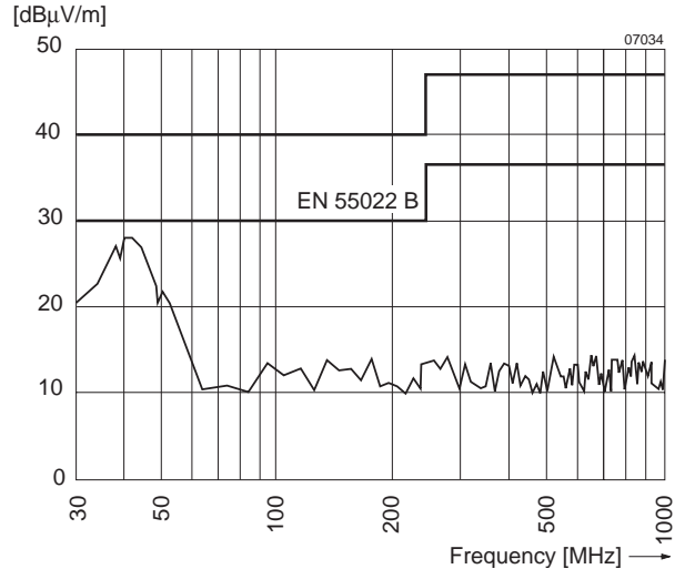
Fig. 17 Typical radio frequency interference voltage at U_{i\text{ nom}} , I_{o\text{ nom}} , measured with an antenna (distance 10 m). Output leads 0.1 m, twisted (40 IMX 4-1515).
