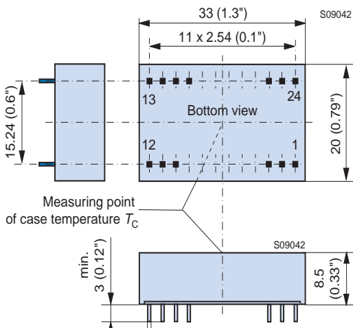
Fig. 18 Standard or alternative pinout (0.5mm pin diameter) Weight: <10 g
