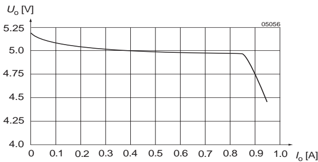
Fig. 10 U_o versus I_o (typ) of single output units (example for 20/40 IMX 4-05)
