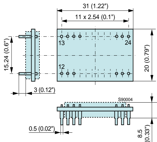
Fig. 19 Open frame (Option Z) Weight: <10 g
