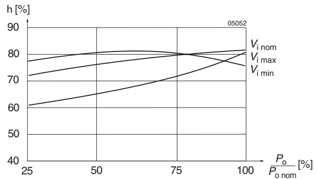
Fig. 11 Efficiency versus input voltage and load. Typical values (40IMX7-12-12).
