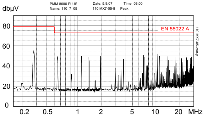
Fig. 16c 110IMX7-05-8: Typical conducted emissions (peak) at the input at V_{i\text{ nom}} and I_{o\text{ nom}} according to EN 55011/22. Output leads 0.1 m, twisted. External input capacitor (0.15 \mu\text{F} ceramic + 4.7 \mu\text{F} electrolytic cap).
