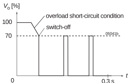
Fig. 6 Overload switch-off (hiccup mode).
