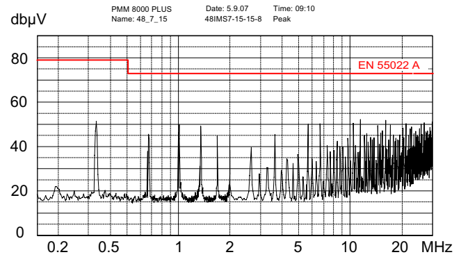
Fig. 17 48IMS7-15-15-8: Typical conducted emissions (peak) at the input at V_{i\text{ nom}} and I_{o\text{ nom}} according to EN 55011/22. Output leads 0.1 m, twisted. External input capacitor (1 \mu\text{F} ceramic + 47 \mu\text{F} electrolytic cap).
