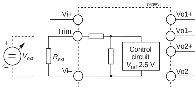
Fig. 15 Output voltage adjust for double-output models
