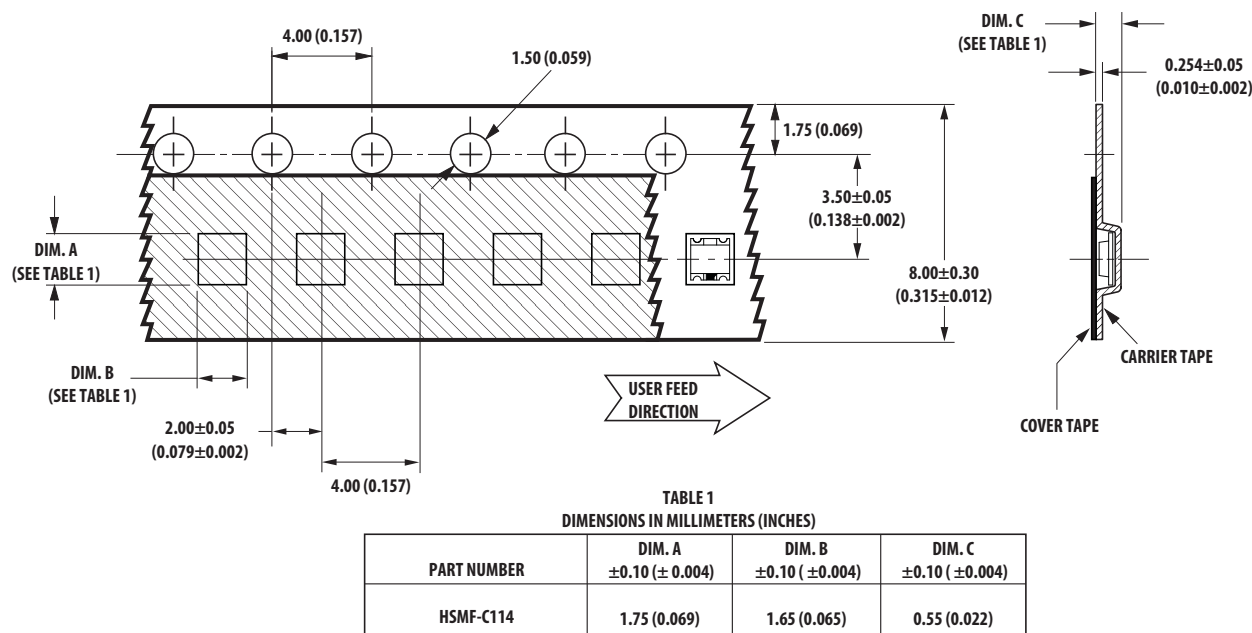
Figure 11. Tape dimensions.
