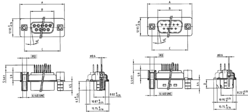
Socket connector
