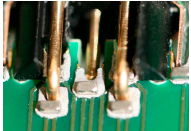
Connector placed into solder paste
