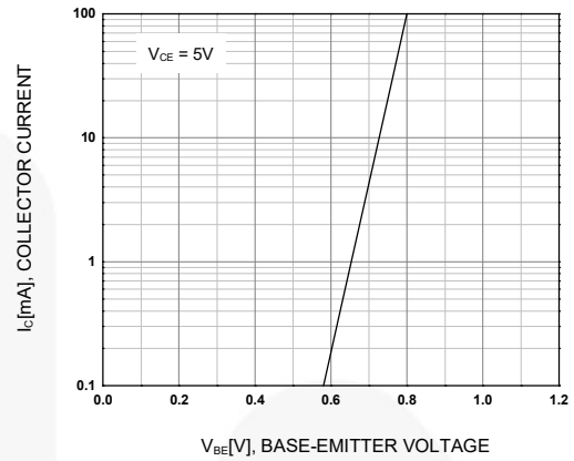
Figure 2. Transfer Characteristic
