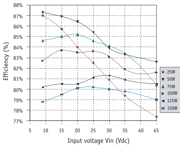
Typical efficiency MGDS-150-H-E at 25°C
