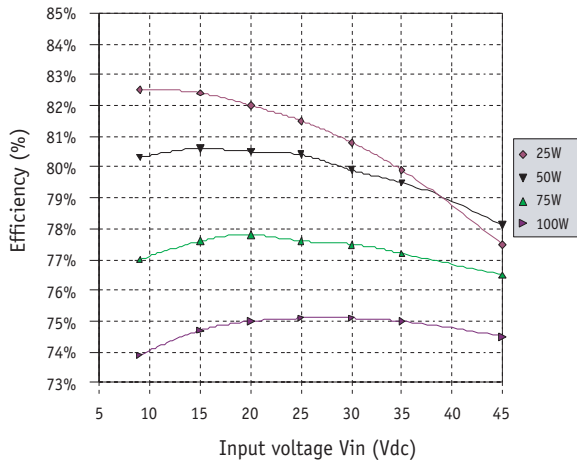
Typical efficiency MGDS-150-H-B at 25°C
