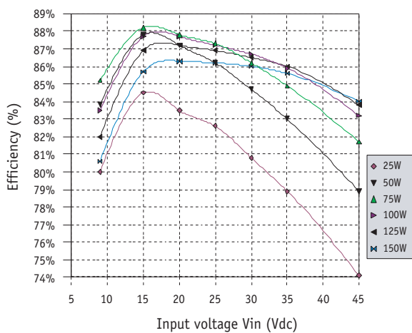
Typical efficiency MGDS-150-H-I at 25°C
