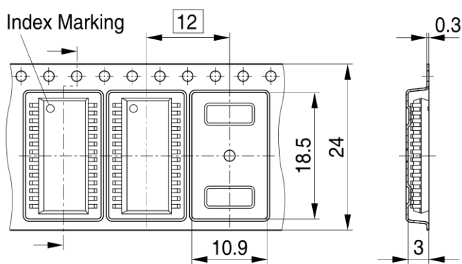
PG-DSO-28-1-6-7-9-11-13-14-16-to-19-21-to-24-26-27-29-to-36-38-41-to-45-73-TP V07
