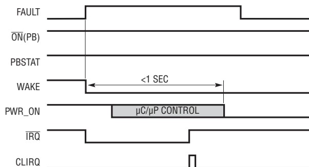
Figure 10. Hard Reset Due to a Fault Condition
