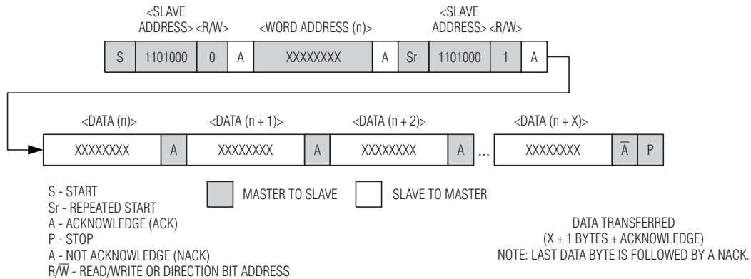
Figure 10. Data Write/Read (Write Pointer, Then Read)—Slave Receive and Transmit
