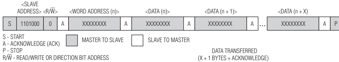
Figure 8. Data Write—Slave Receiver Mode
