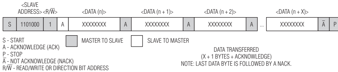
Figure 9. Data Read—Slave Transmitter Mode
