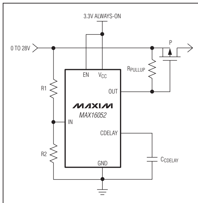
Figure 4. Overvoltage Protection
