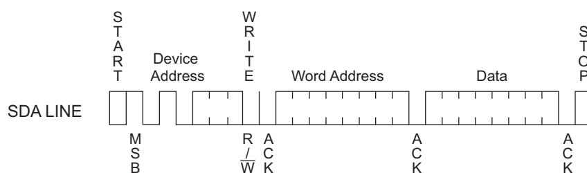
Figure 8-1. Byte Write
