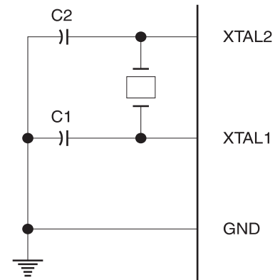
Figure 1. Oscillator Connections
