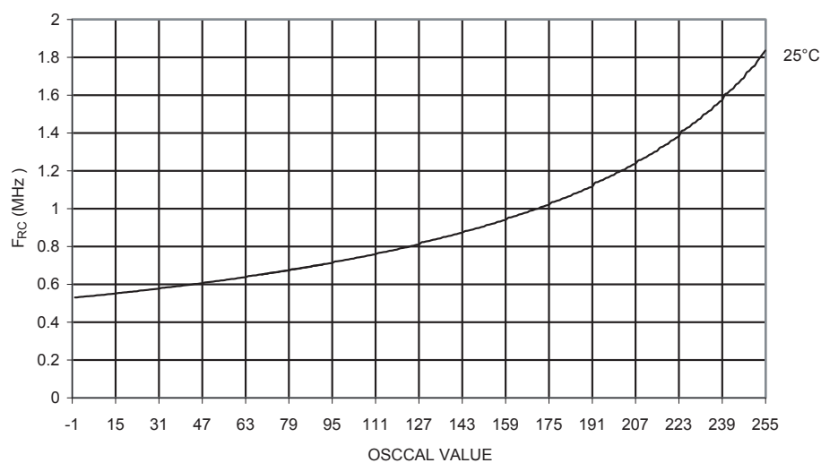
Figure 200. Calibrated 1 MHz RC Oscillator Frequency vs. OSCCAL Value
