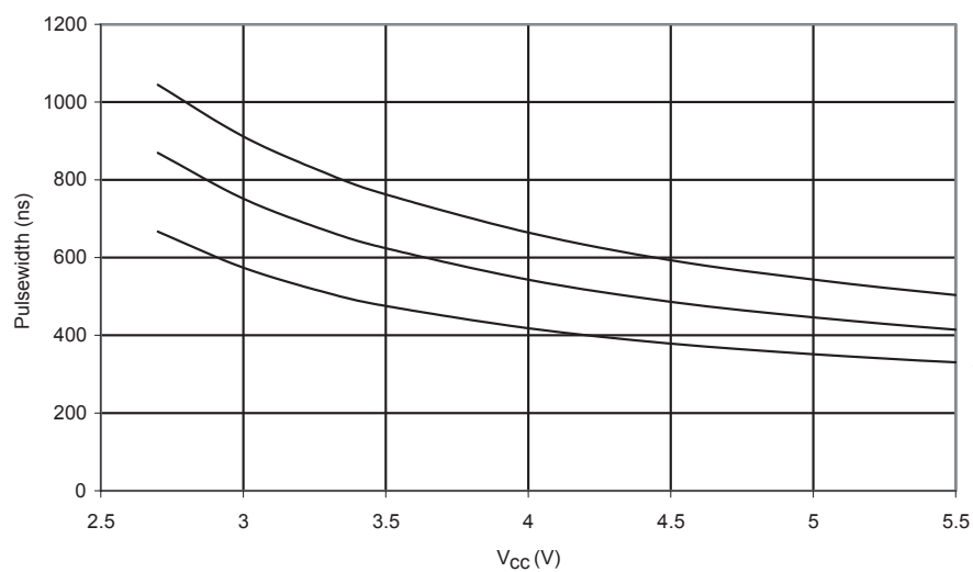
Figure 208. Minimum Reset Pulse Width vs. V_{CC}
