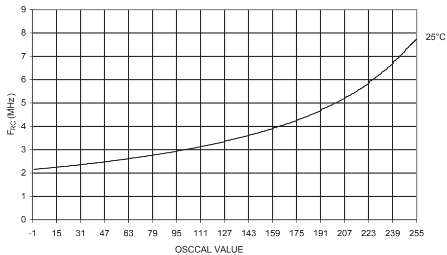
Figure 194. Calibrated 4 MHz RC Oscillator Frequency vs. OSCCAL Value
