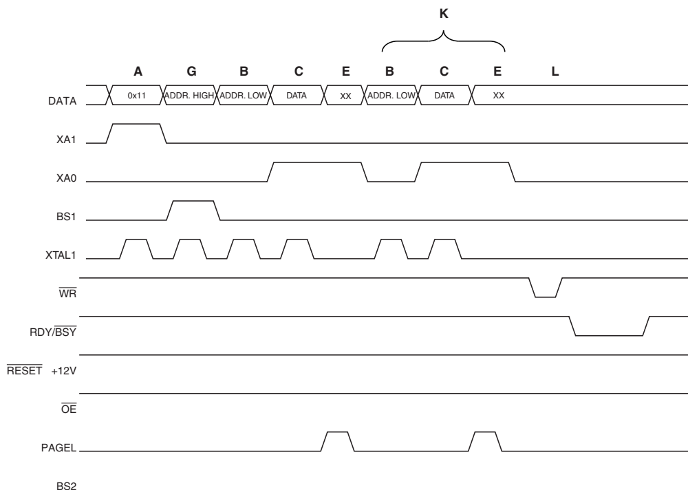
Figure 130. Programming the EEPROM Waveforms
