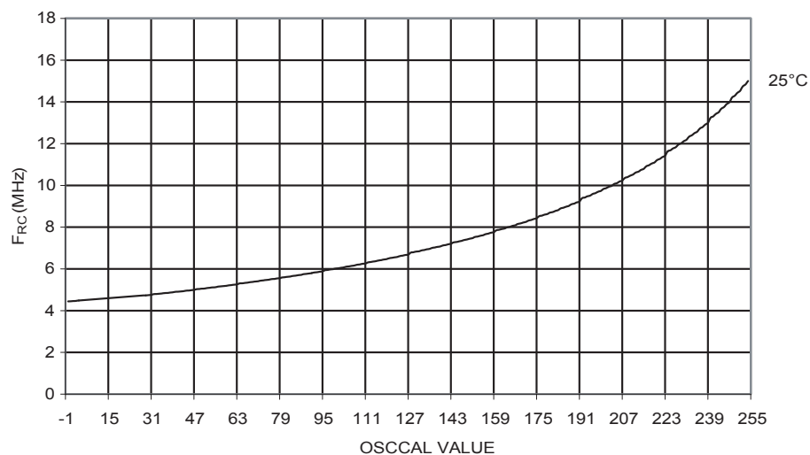
Figure 191. Calibrated 8 MHz RC Oscillator Frequency vs. Oscscal Value
