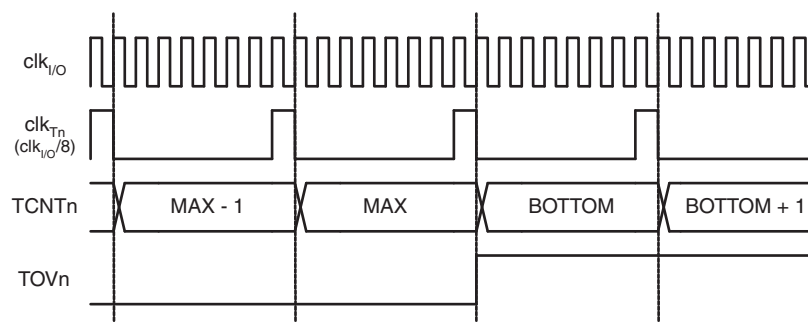
Figure 18-9. Timer/Counter Timing Diagram, with Prescaler ( f_{\text{clk\_I/O}}/8 )
