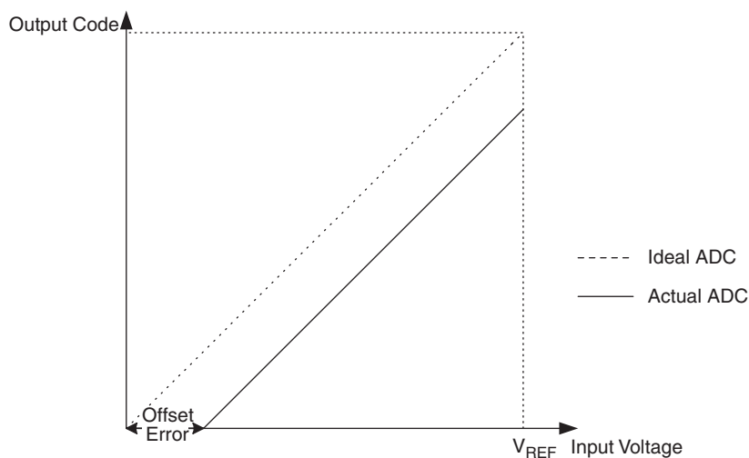
Figure 24-10. Offset Error
