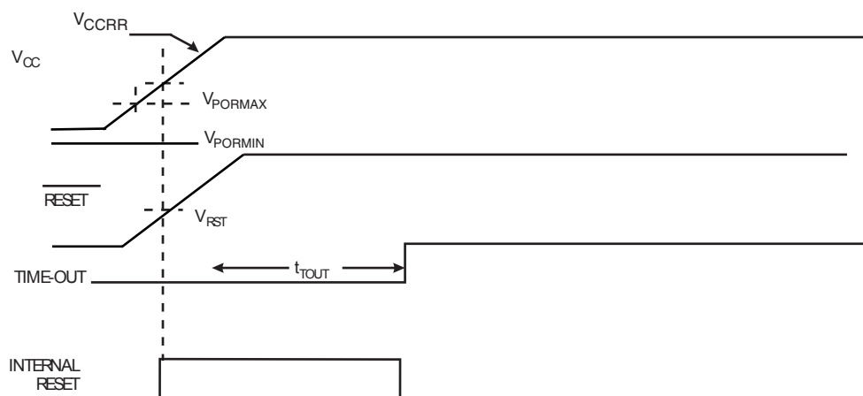
Figure 11-2. MCU Start-up, \overline{\text{RESET}} Tied to V_{CC}
