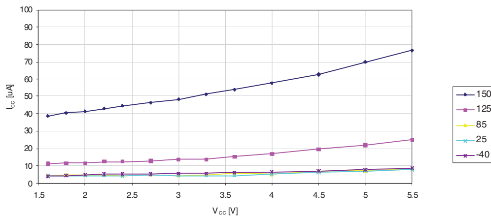
Figure 30-34. Power-Down Supply Current versus V_{CC} (Watchdog Timer Enabled)
