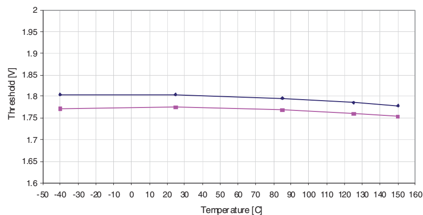
Figure 30-19. BOD Thresholds versus Temperature (BODLEVEL is 1.8V)
