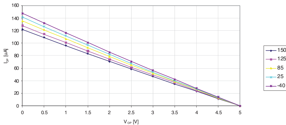
Figure 30-35. I/O Pin Pull-up Resistor Current versus Input Voltage ( V_{CC} = 5.0V )
