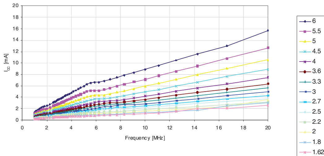
Figure 30-30. Active Supply Current versus Frequency (1-16MHz)
