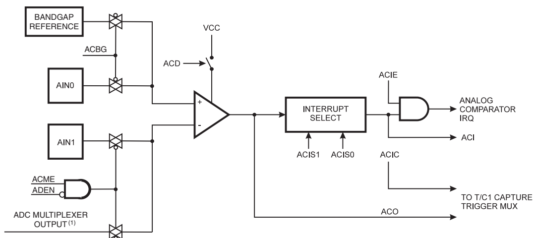
Figure 23-1. Analog Comparator Block Diagram (2)
