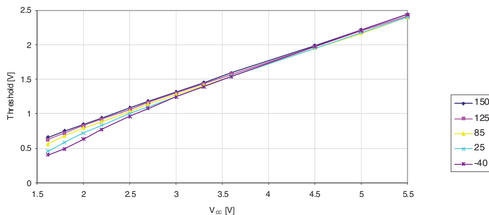
Figure 30-44. I/O Pin Input Threshold Voltage versus V_{CC} ( V_{IL} , I/O Pin read as '0')
