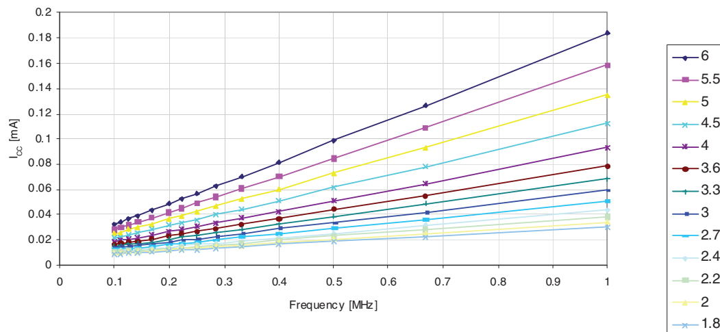
Figure 30-59. Idle Supply Current versus Low Frequency (0.1-1.0MHz)
