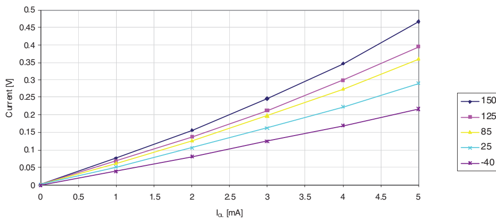
Figure 30-37. I/O Pin Output Voltage versus Sink Current ( V_{CC} = 1.8V )
