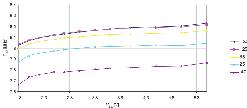
Figure 30-81. Calibrated 8MHz RC Oscillator Frequency versus V_{CC}
