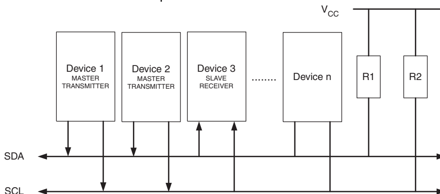
Figure 22-20. An Arbitration Example
