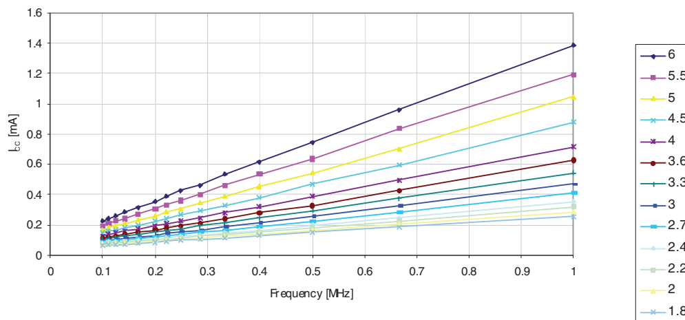
Figure 30-57. Active Supply Current versus Low Frequency (0.1-1.0MHz)
