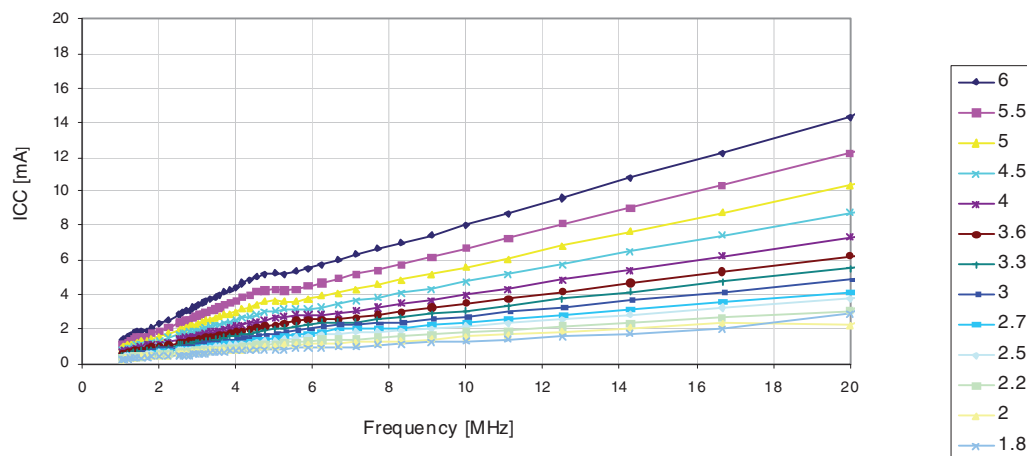
Figure 30-2. Active Supply Current versus Frequency (1-16MHz)
