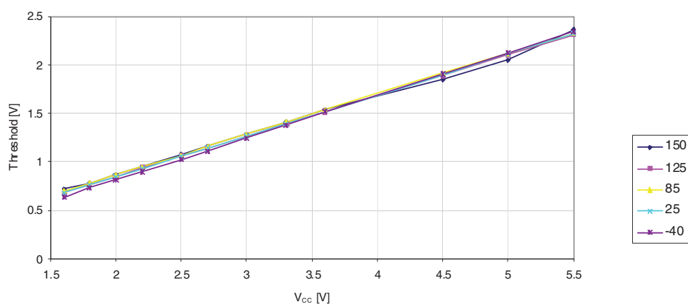
Figure 30-74. Reset Input Threshold Voltage versus V_{CC} ( V_{IL} , I/O Pin read as '0')
