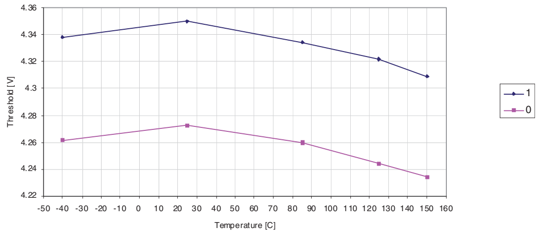
Figure 30-77. BOD Thresholds versus Temperature (BODLEVEL is 4.3V)
