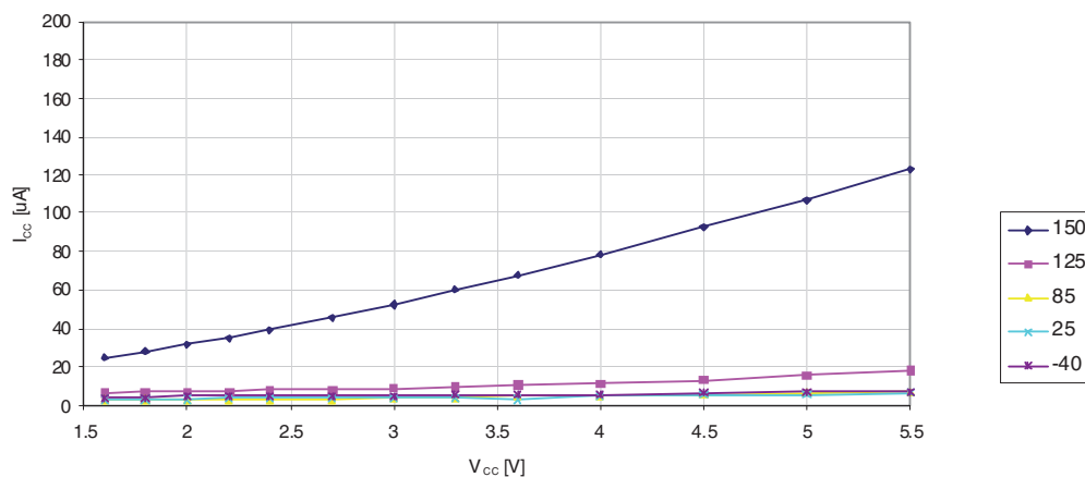
Figure 30-62. Power-Down Supply Current versus V_{CC} (Watchdog Timer Enabled)
