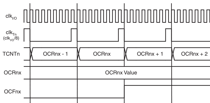
Figure 18-10. Timer/Counter Timing Diagram, Setting of OCF2A, with Prescaler ( f_{\text{clk\_I/O}}/8 )
