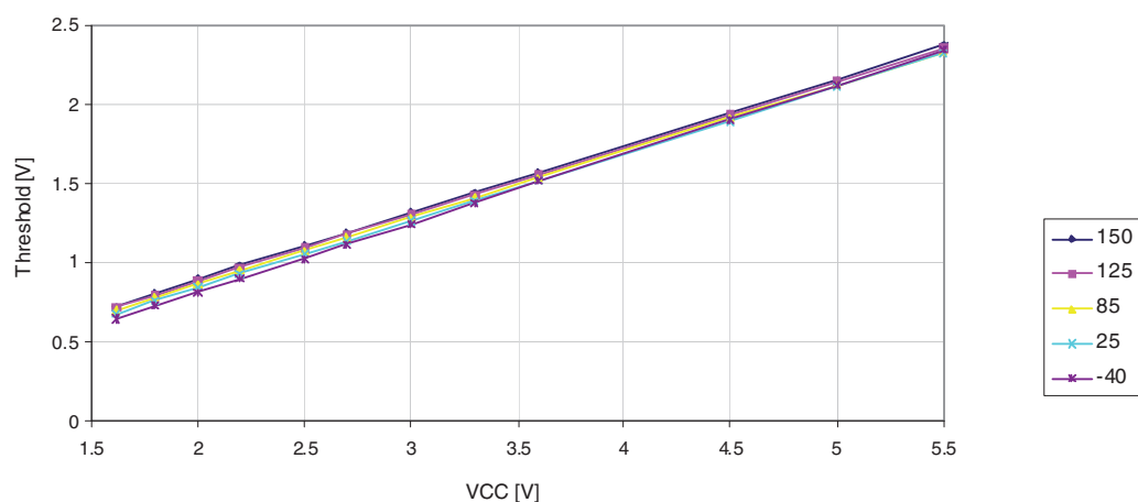
Figure 30-18. Reset Input Threshold Voltage versus V_{CC} ( V_{IL} , I/O Pin read as '0')
