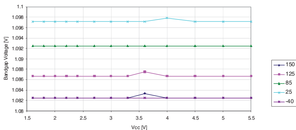
Figure 30-50. Bandgap Voltage versus V_{CC}
