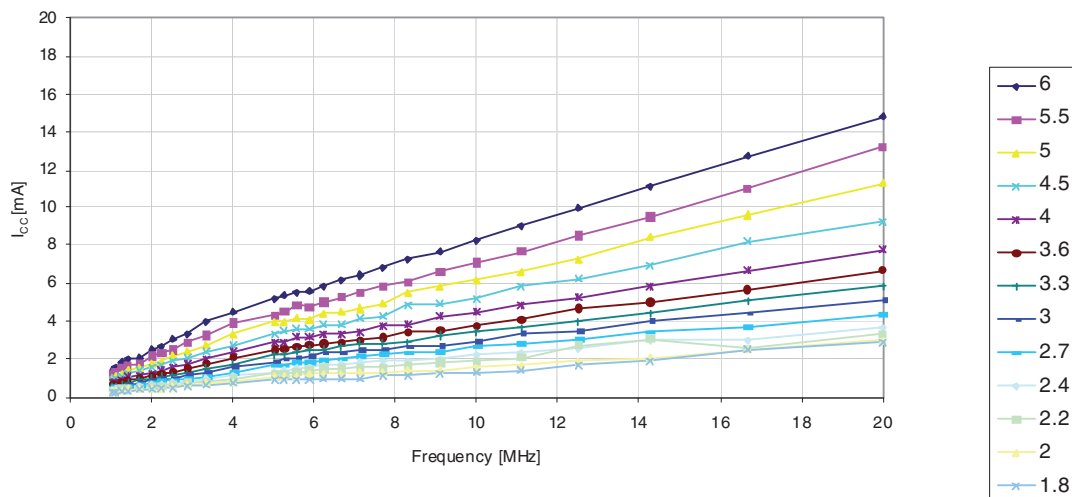
Figure 30-58. Active Supply Current versus Frequency (1-16MHz)
