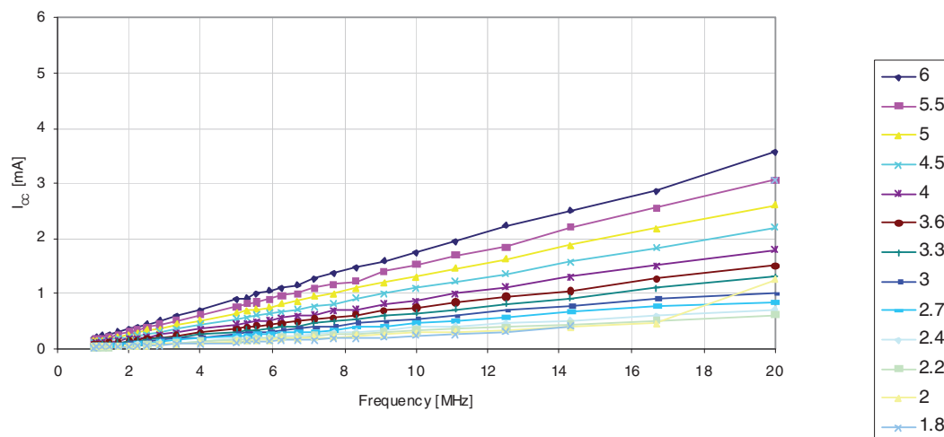
Figure 30-60. Idle Supply Current versus Frequency (1-16MHz)
