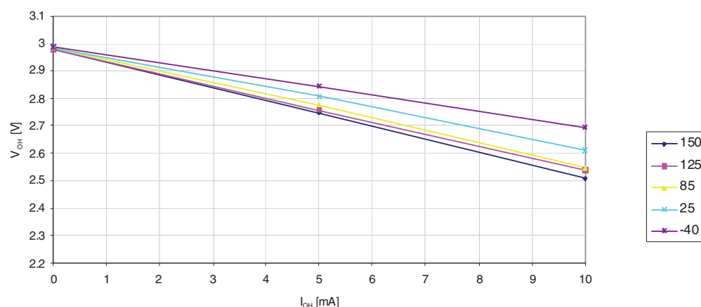
Figure 30-69. I/O Pin Output Voltage versus Source Current ( V_{CC} = 3V )
