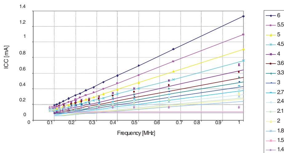
Figure 30-1. Active Supply Current versus Low Frequency (0.1-1.0MHz)
