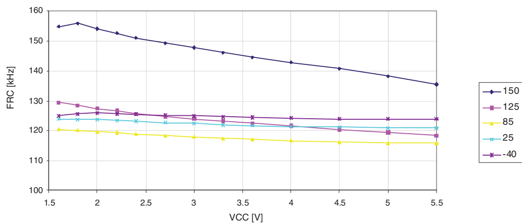
Figure 30-24. Watchdog Oscillator Frequency versus V_{CC}
