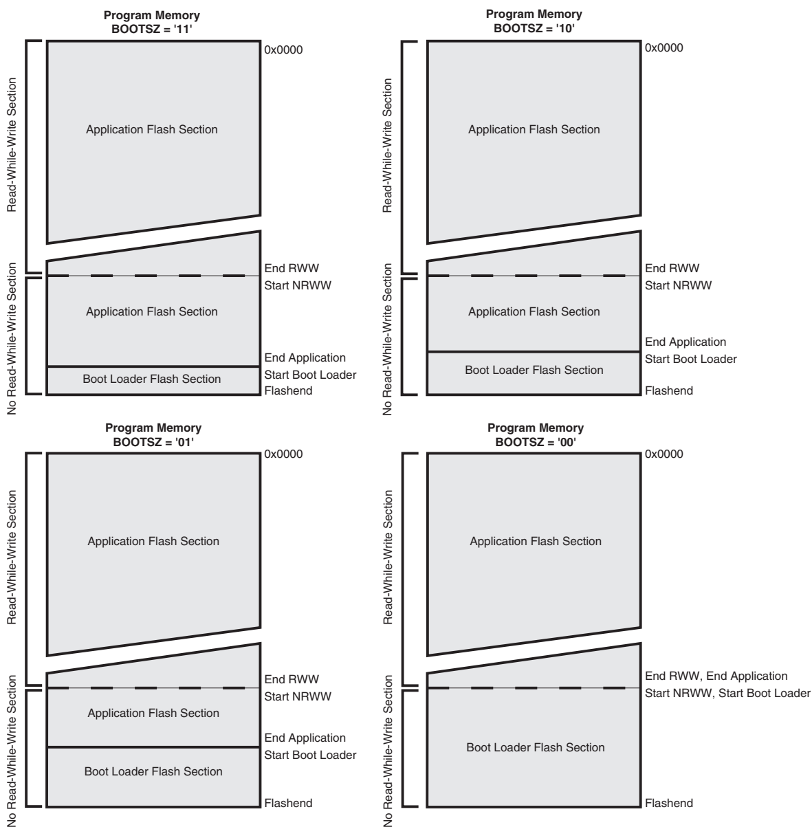
Figure 27-2. Memory Sections
