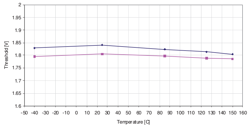
Figure 30-47. BOD Thresholds versus Temperature (BODLEVEL is 1.8V)
