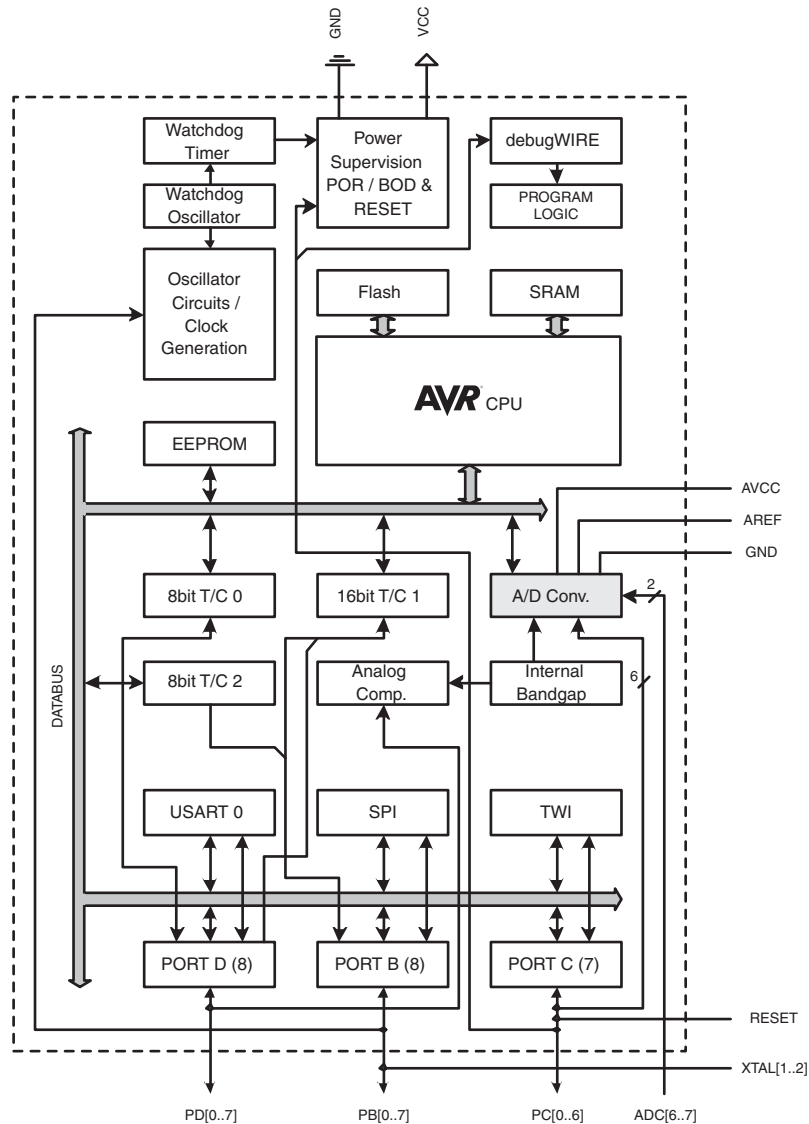
Figure 2-1. Block Diagram
