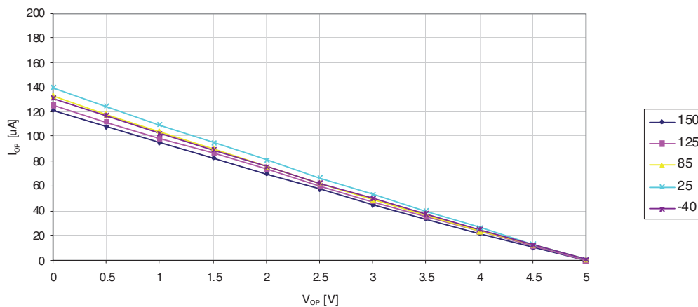
Figure 30-63. I/O Pin Pull-up Resistor Current versus Input Voltage ( V_{CC} = 5.0V )
