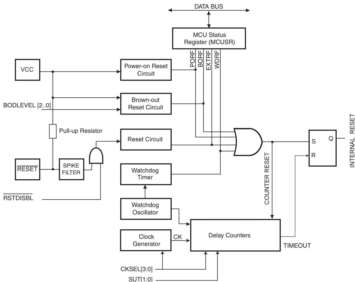
Figure 11-1. Reset Logic
