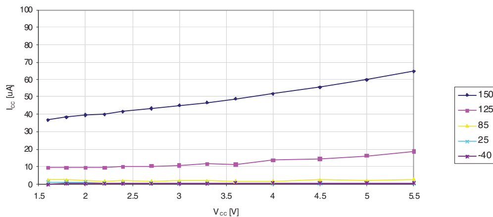
Figure 30-33. Power-Down Supply Current versus V_{CC} (Watchdog Timer Disabled)
