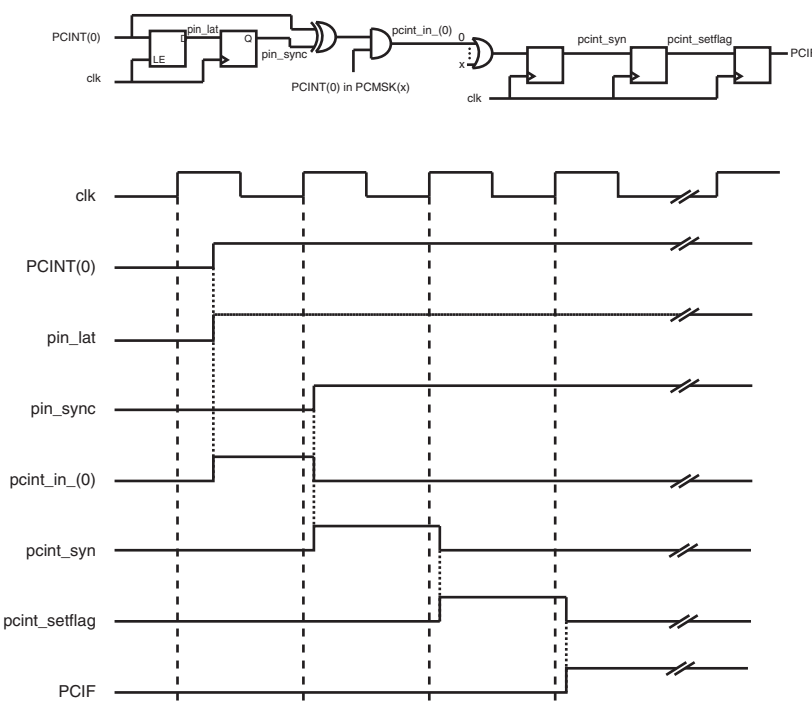
Figure 13-1. Timing of pin change interrupts
