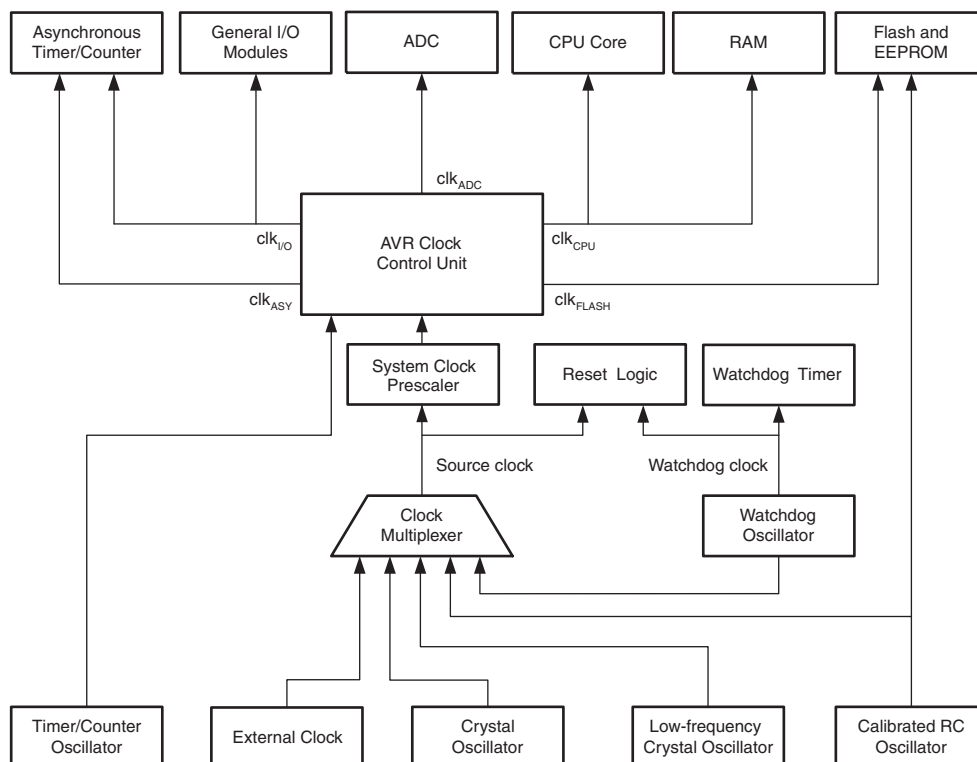
Figure 9-1. Clock Distribution
