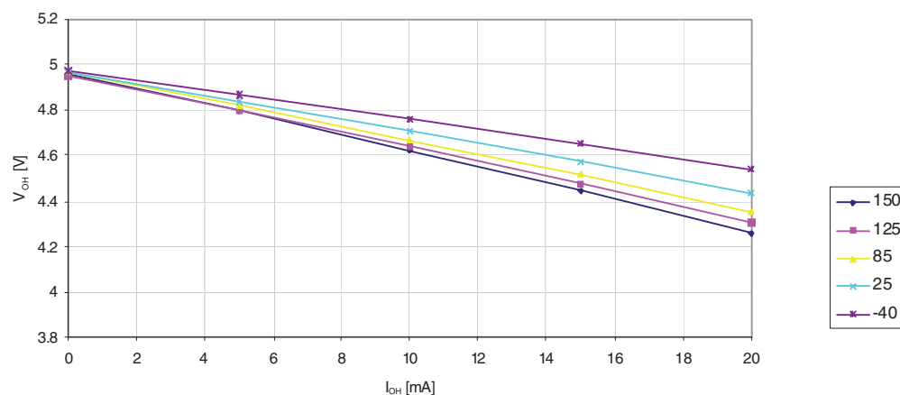
Figure 30-42. I/O Pin Output Voltage versus Source Current ( V_{CC} = 5V )
