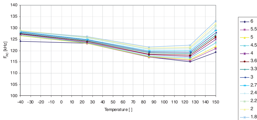
Figure 30-79. Watchdog Oscillator Frequency versus Temperature
