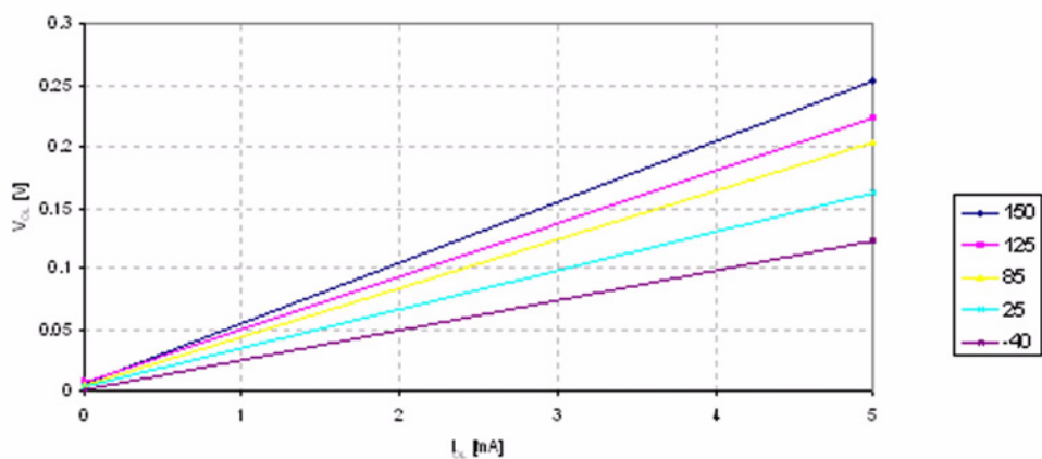
Figure 30-38. I/O Pin Output Voltage versus Sink Current ( V_{CC} = 3V )
