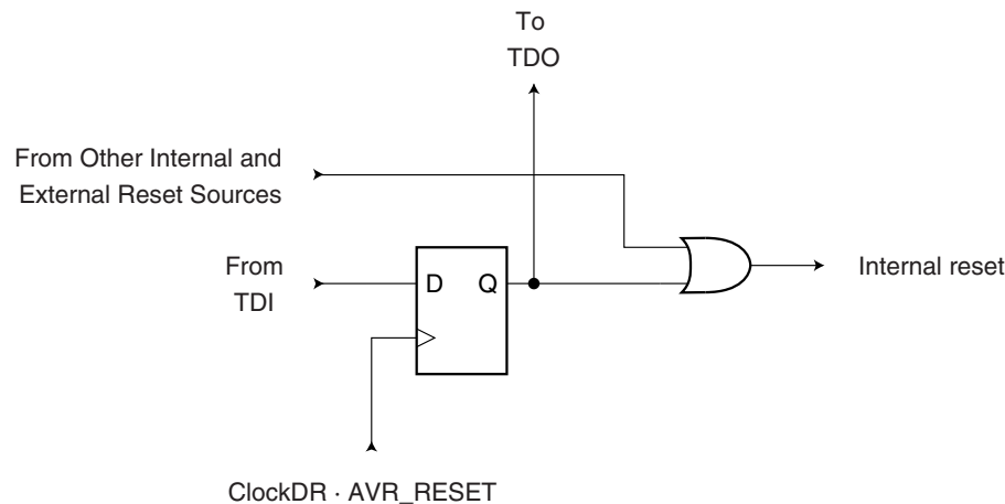
Figure 23-2. Reset Register
