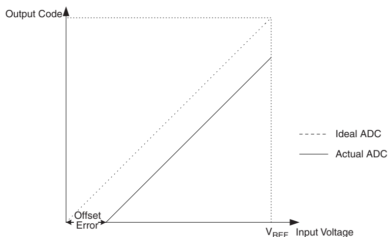
Figure 21-10. Offset Error
