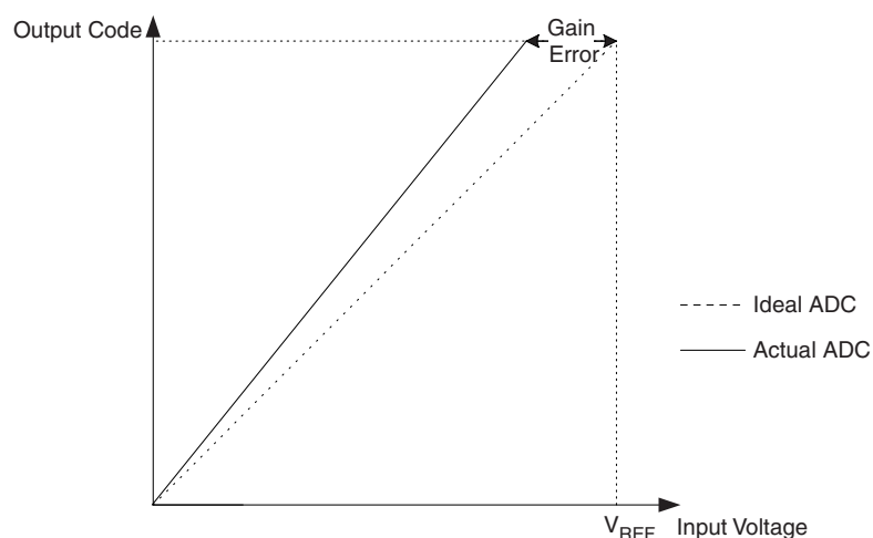
Figure 21-11. Gain Error
