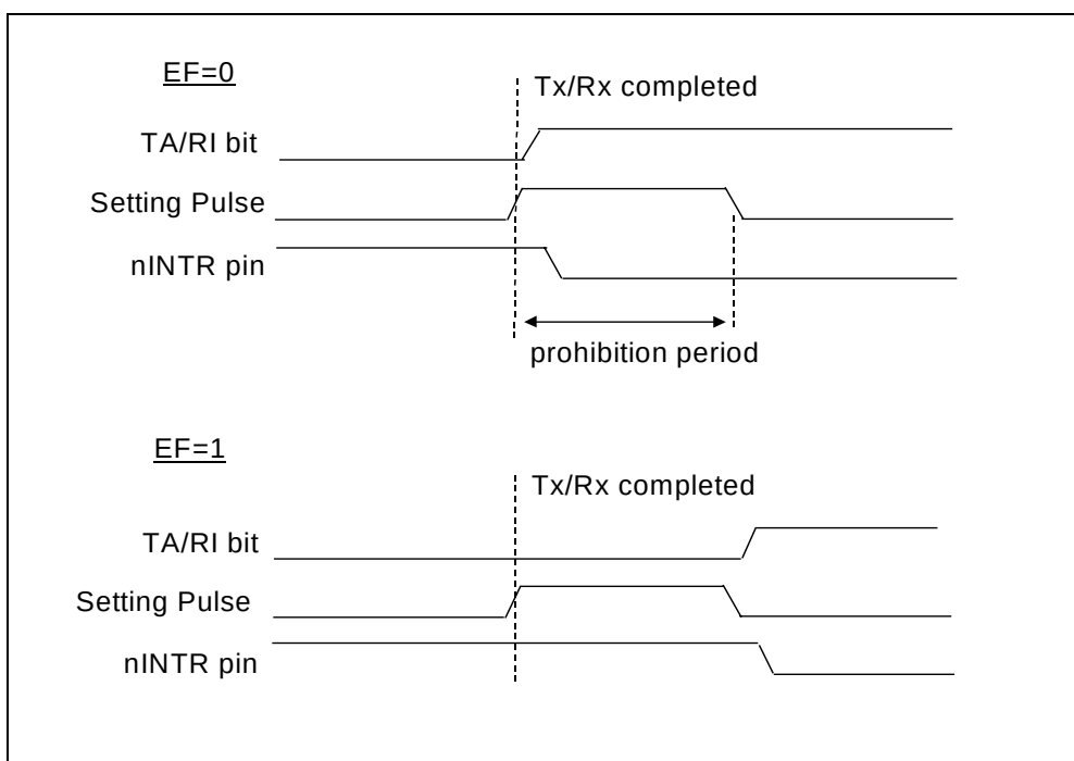
FIGURE 26 - EFFECT OF THE EF BIT ON THE TA/RI BIT
