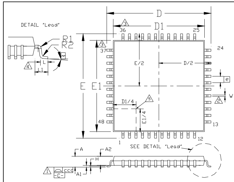
FIGURE 25 - 48 PIN TQFP PACKAGE OUTLINE
