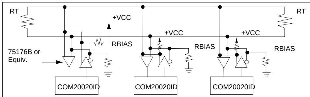
FIGURE 5 - COM20020ID NETWORK USING RS-485 DIFFERENTIAL TRANSCEIVERS
