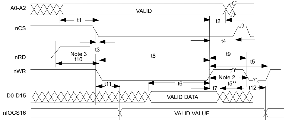
CASE 1: BUSTMG pin = HIGH
