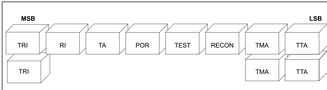
FIGURE 5-3: COMMAND CHAINING STATUS REGISTER QUEUE
