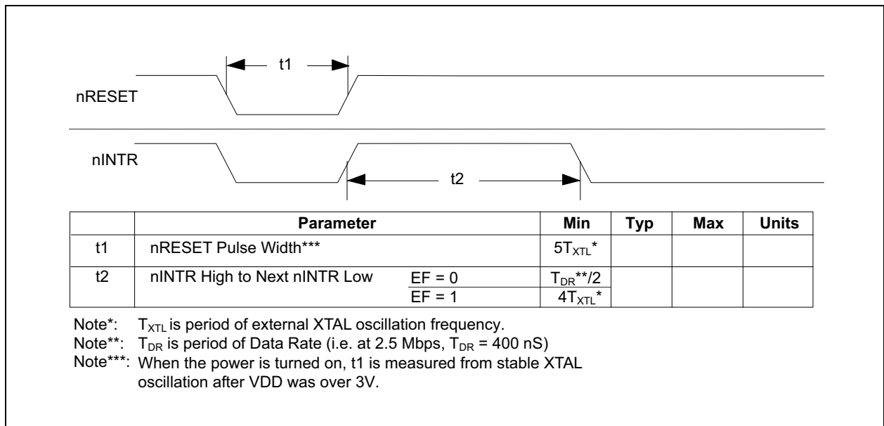
FIGURE 8-16: RESET AND INTERRUPT TIMING
