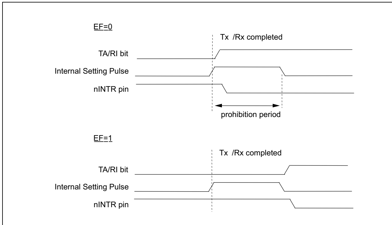
FIGURE A-1: EFFECT OF THE EF BIT ON THE TA/RI BIT
