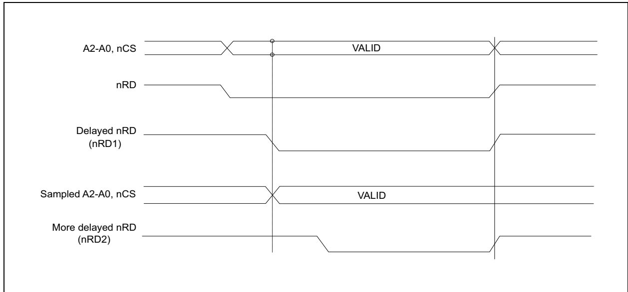
FIGURE 4-3: HIGH-SPEED CPU BUS TIMING – INTEL CPU MODE
