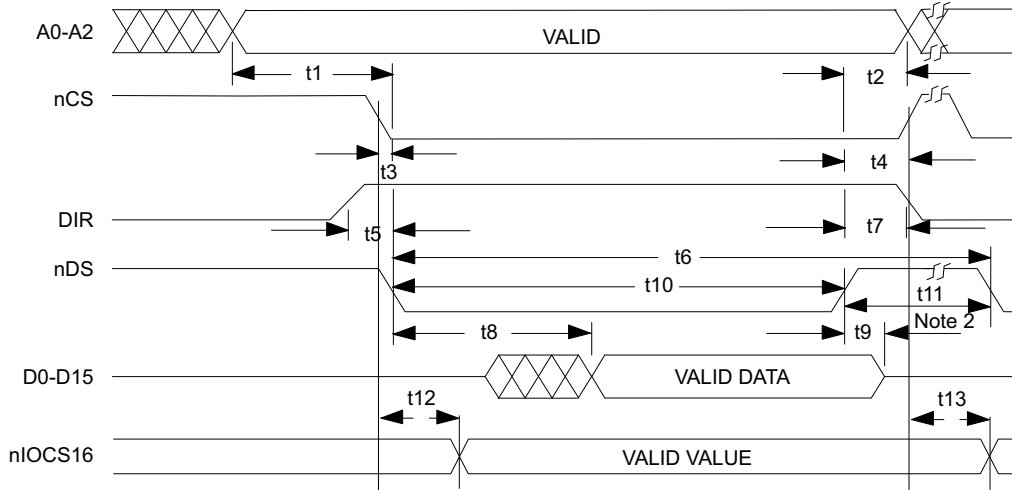
CASE 1: BUSTMG pin = HIGH and RBUSTMG bit = 0
