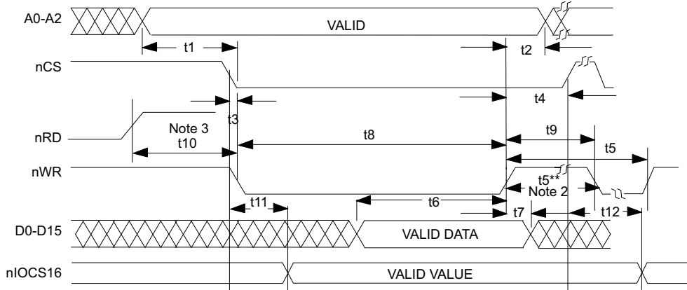
CASE 2: BUSTMG pin = LOW
