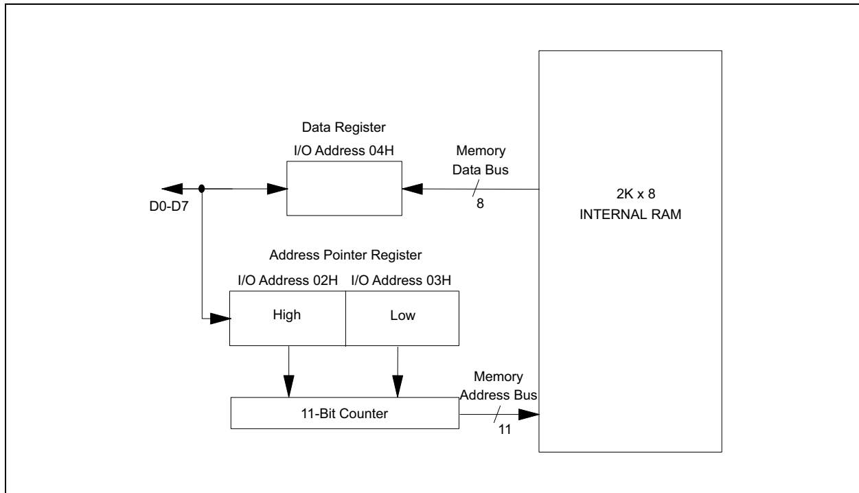
FIGURE 5-1: SEQUENTIAL ACCESS OPERATION
