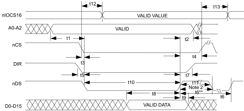
CASE 2: BUSTMG pin = LOW
