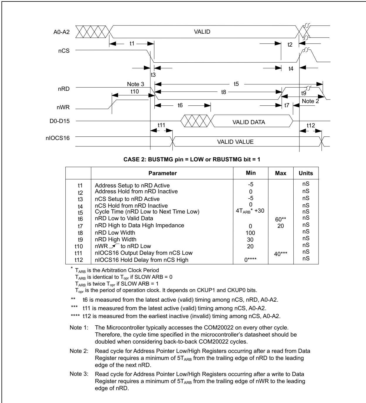
FIGURE 8-6: NON-MULTIPLEXED BUS, 80XX-LIKE CONTROL SIGNALS; READ CYCLE
