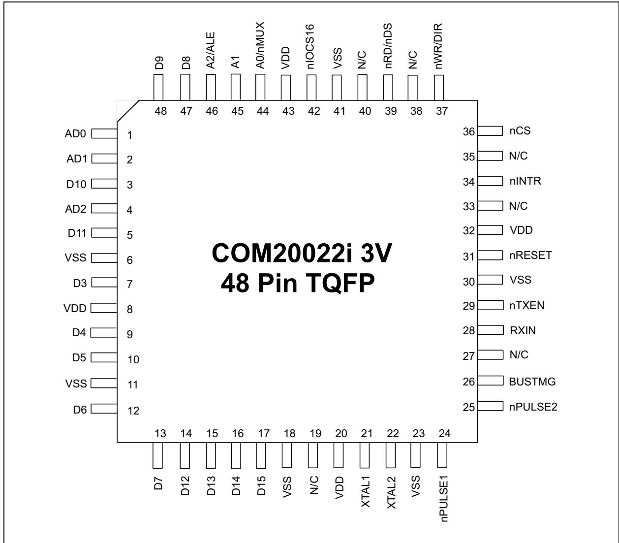
FIGURE 2-1: 48-TQFP PIN ASSIGNMENT
