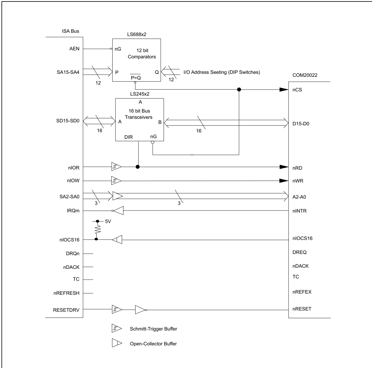
FIGURE B-1: EXAMPLE OF INTERFACE OF CIRCUIT DIAGRAM TO ISA BUS
