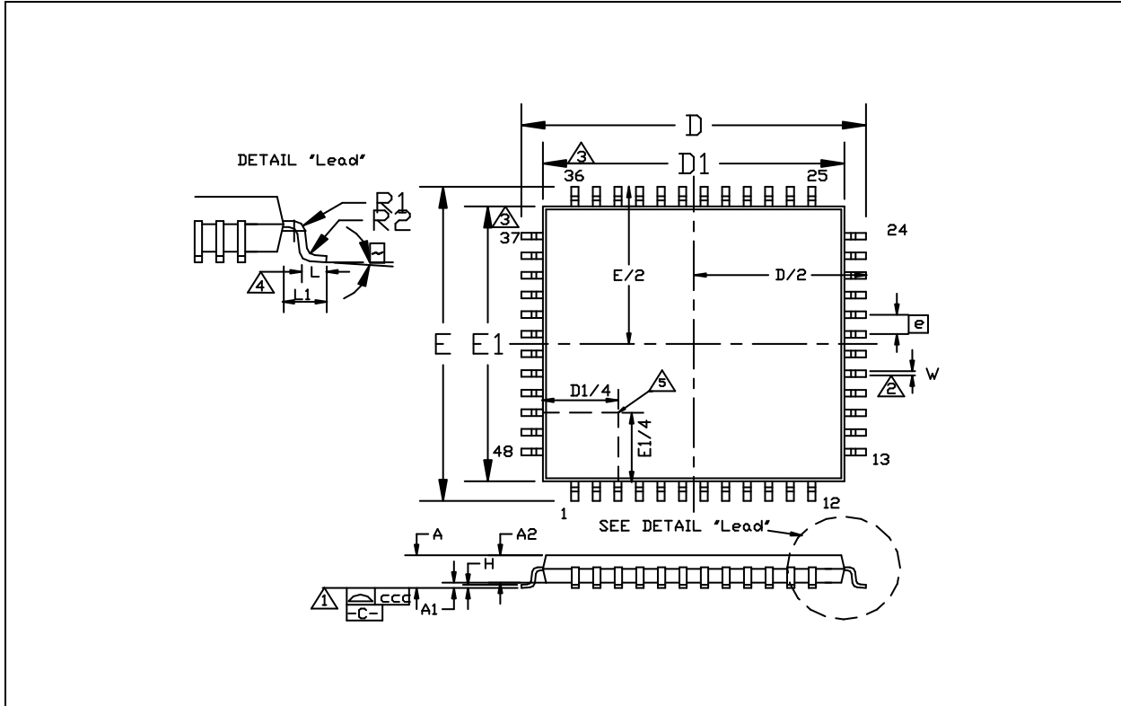
FIGURE 9-1: 48 PIN TQFP PACKAGE OUTLINE
