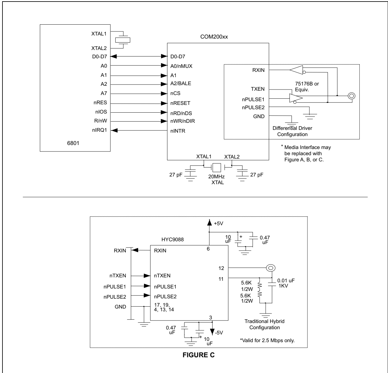
FIGURE 4-2: NON-MULTIPLEXED, 6801-LIKE BUS INTERFACE WITH RS-485 INTERFACE
