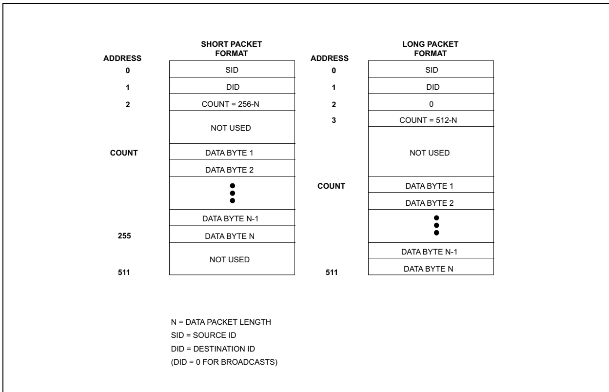
FIGURE 5-2: RAM BUFFER PACKET CONFIGURATION
