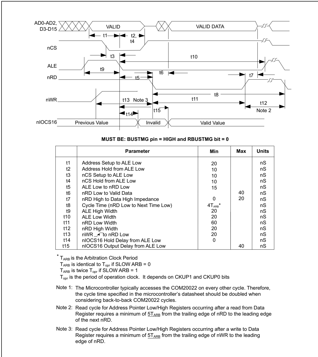
FIGURE 8-2: MULTIPLEXED BUS, 80XX-LIKE CONTROL SIGNALS; READ CYCLE
