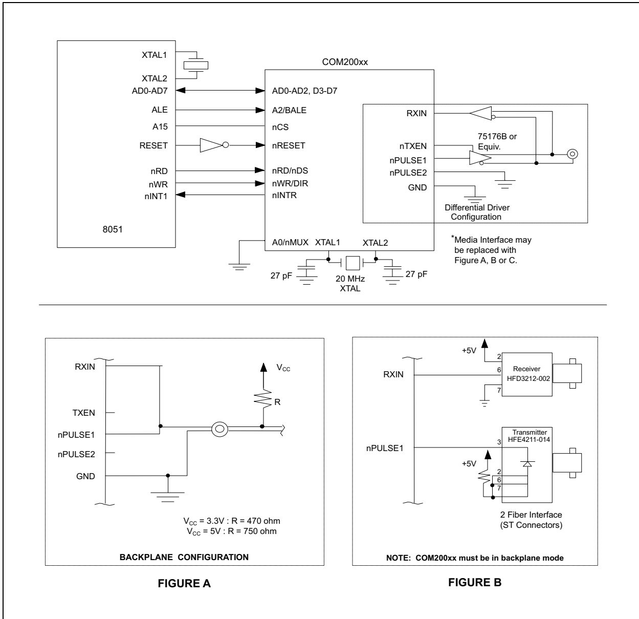
FIGURE 4-1: MULTIPLEXED, 8051-LIKE BUS INTERFACE WITH RS-485 INTERFACE
