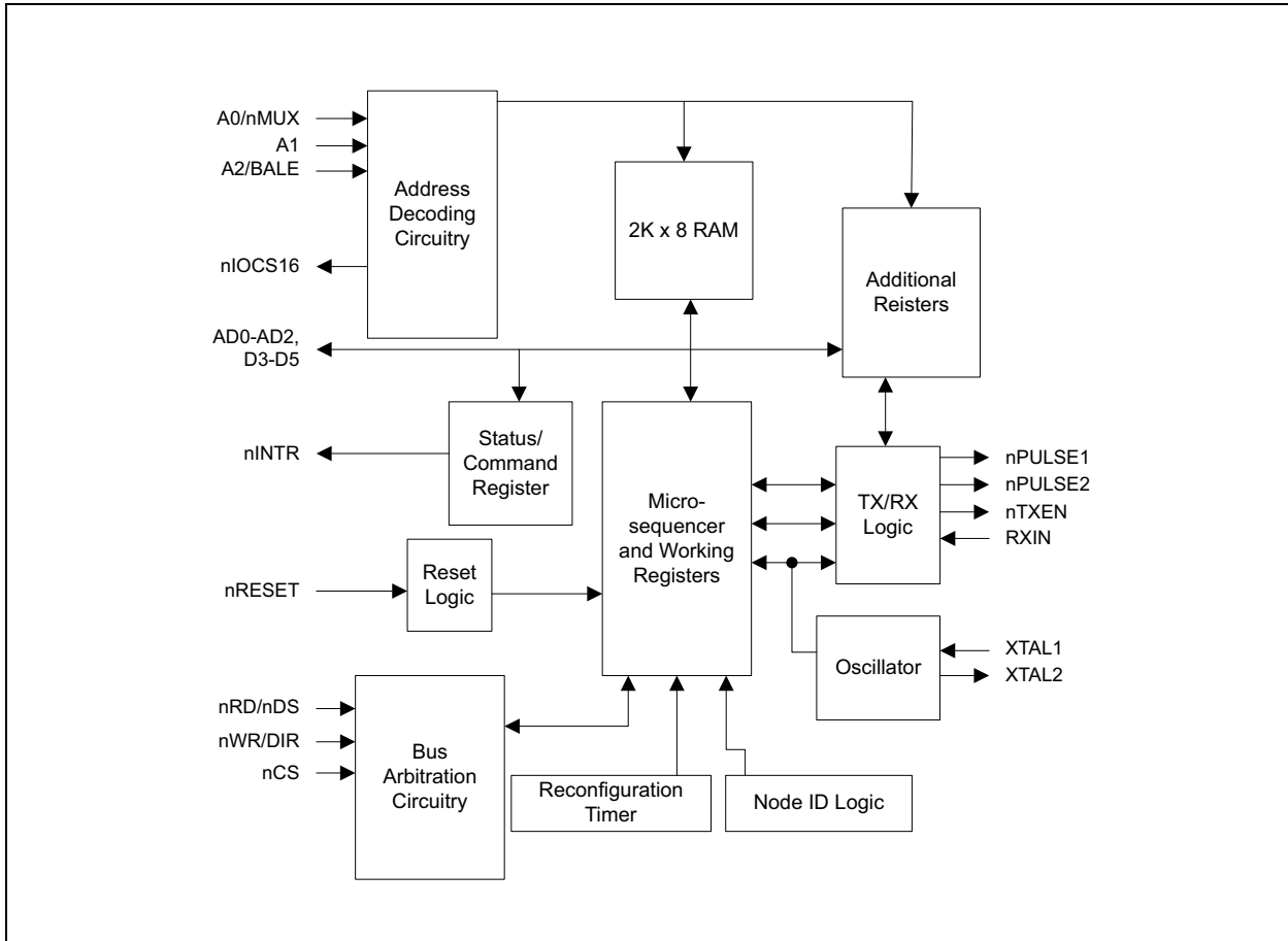
FIGURE 4-6: INTERNAL BLOCK DIAGRAM
