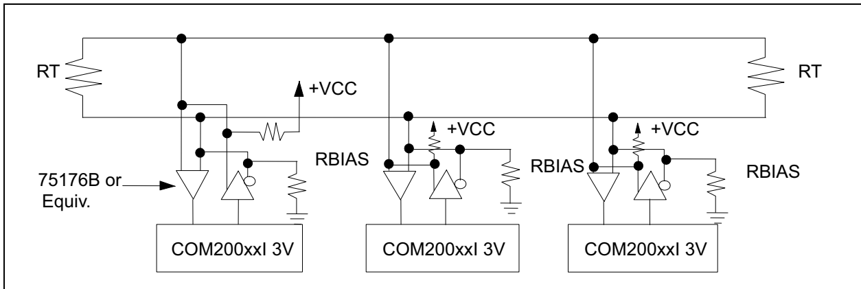
FIGURE 4-4: COM20022i 3V NETWORK USING RS-485 DIFFERENTIAL TRANSCEIVERS
