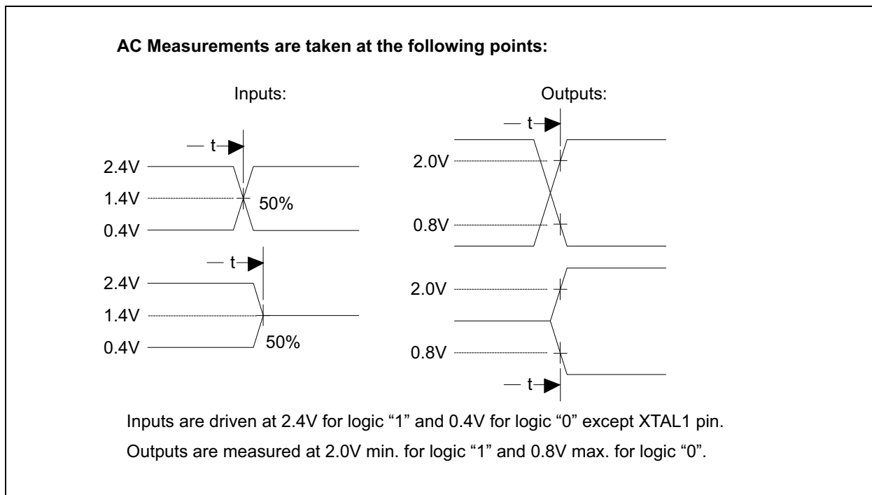
FIGURE 7-1: AC MEASUREMENTS
