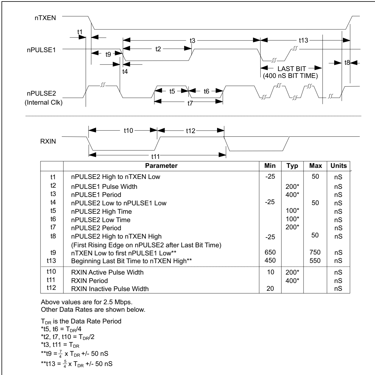
FIGURE 8-14: BACKPLANE MODE TRANSMIT OR RECEIVE TIMING
