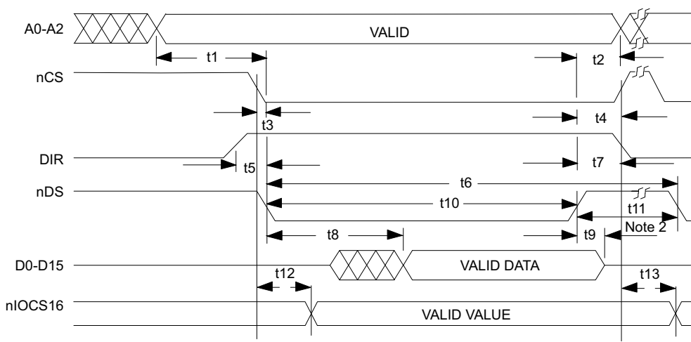
FIGURE 8-8: NON-MULTIPLEXED BUS, 68XX-LIKE CONTROL SIGNALS; READ CYCLE
