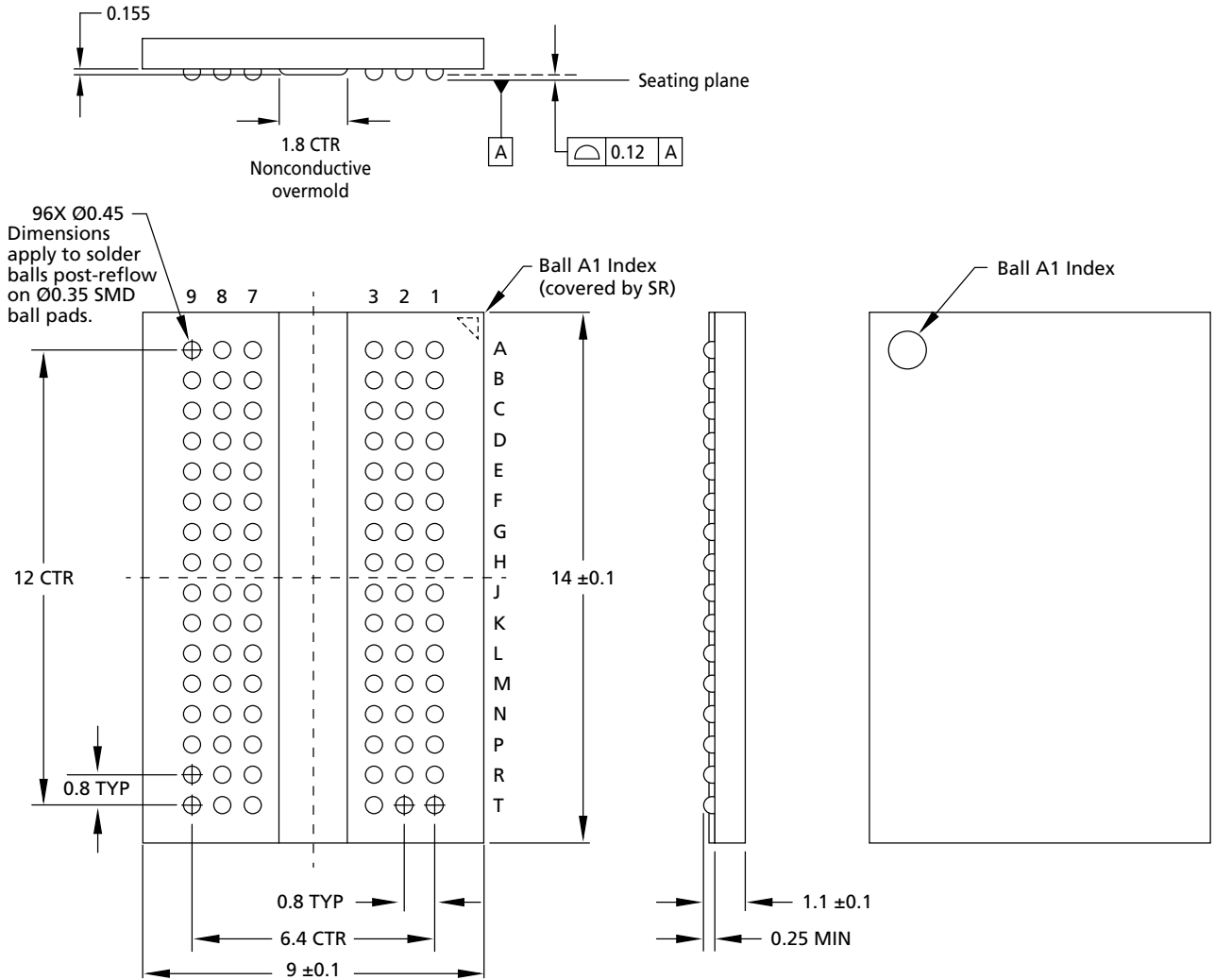
Figure 6: 96-Ball FBGA – x16; "HA"
