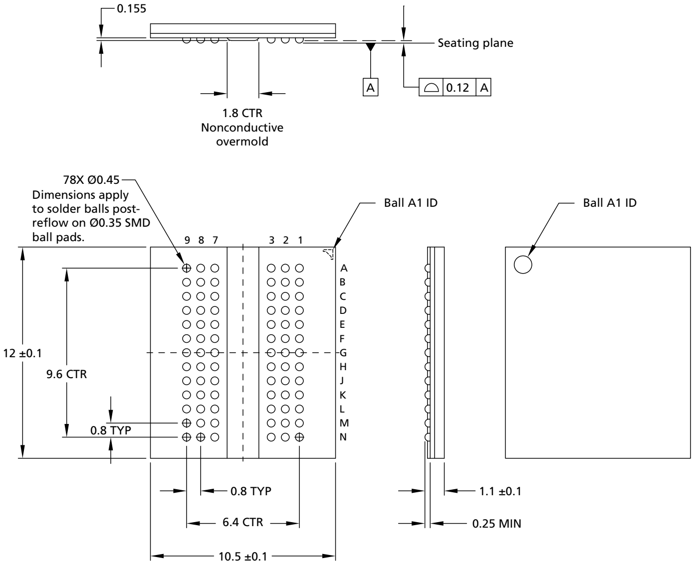
Figure 3: 78-Ball FBGA – x4, x8; "RA"
