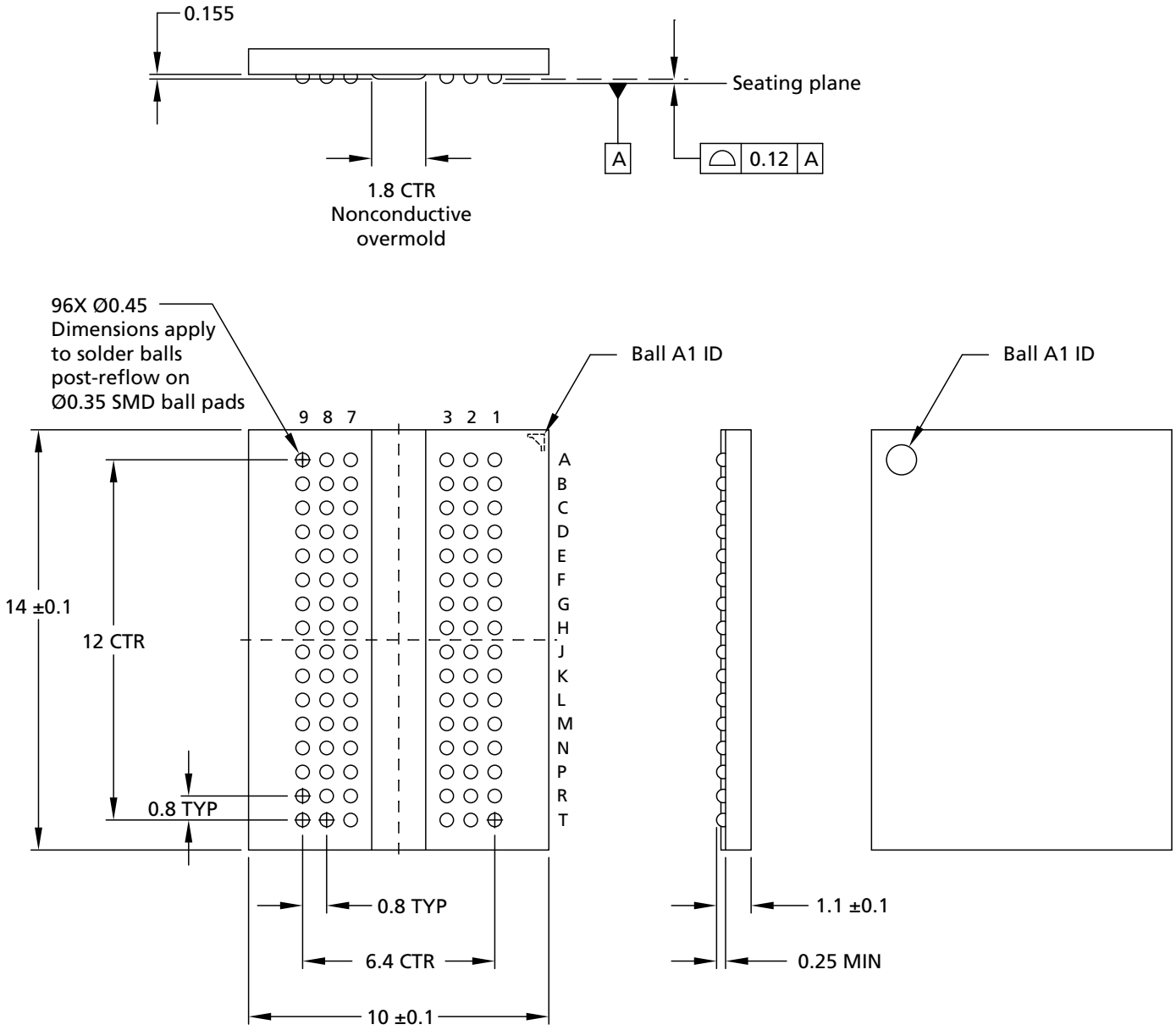
Figure 5: 96-Ball FBGA – x16; "RE"
