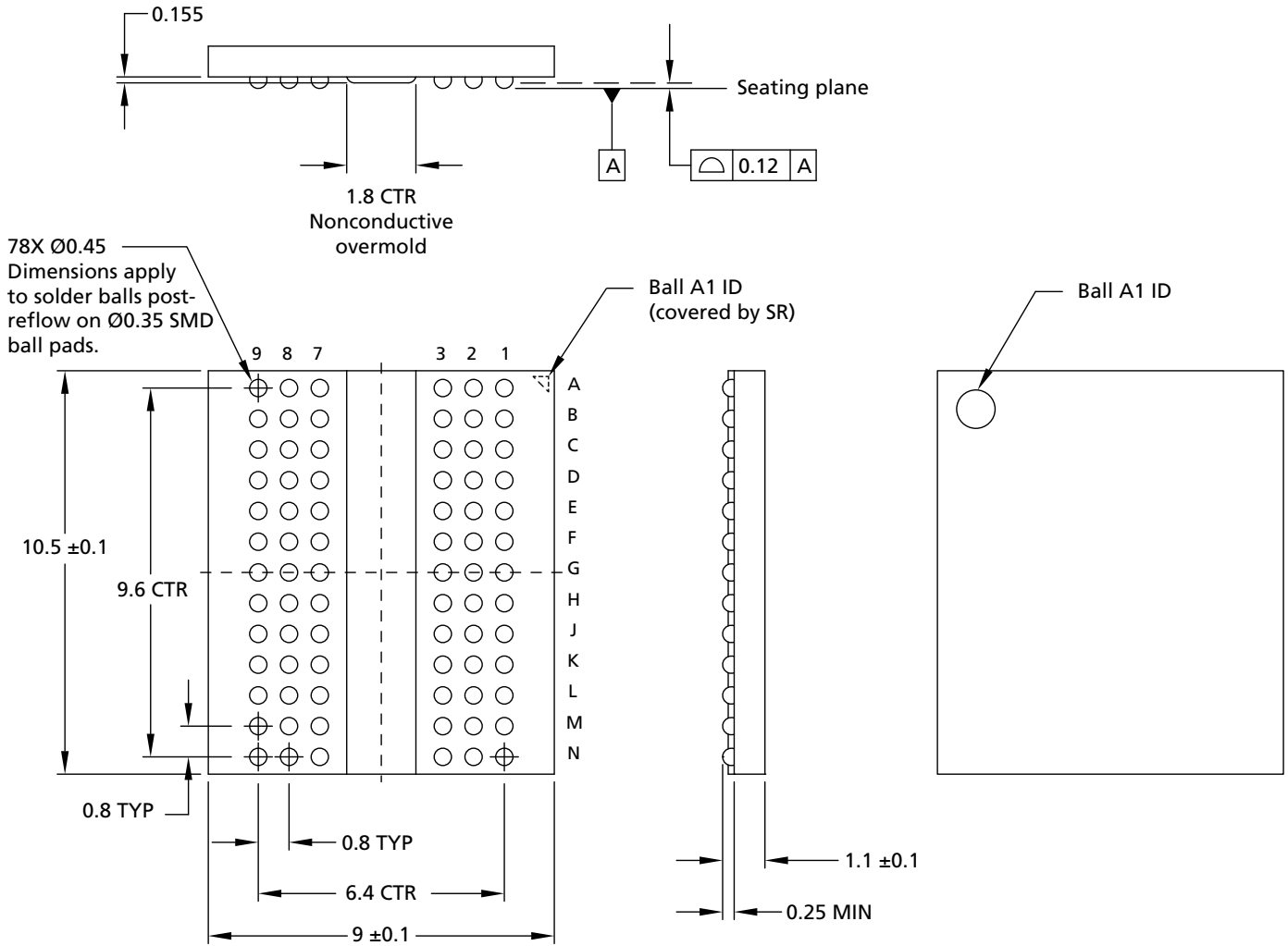
Figure 4: 78-Ball FBGA – x4, x8; "RH"
