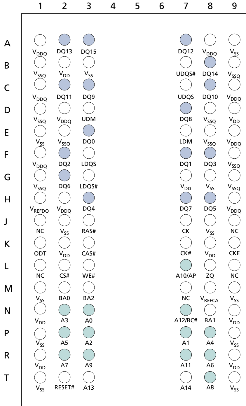
Figure 2: 96-Ball FBGA – x16 (Top View)
