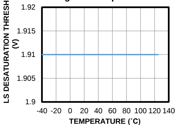
LS Desaturation Threshold Voltage vs. Temperature
