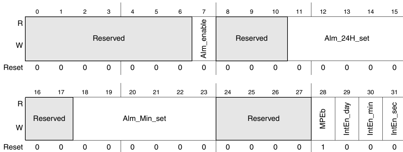
Figure 7-57. RTC Alarm and Interrupt Enable Register
