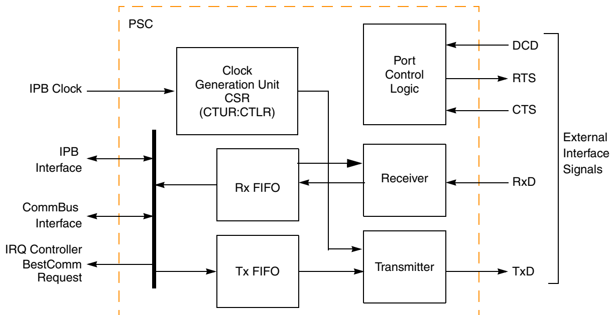
Figure 15-68. PSC UART Block Diagram
