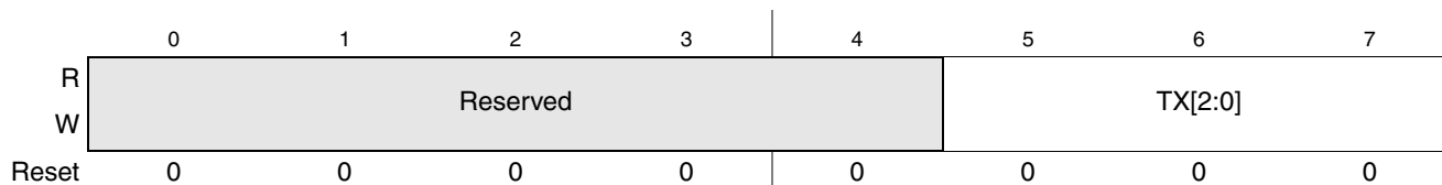
Figure 19-13. MSCAN Transmit Buffer Selection Register
