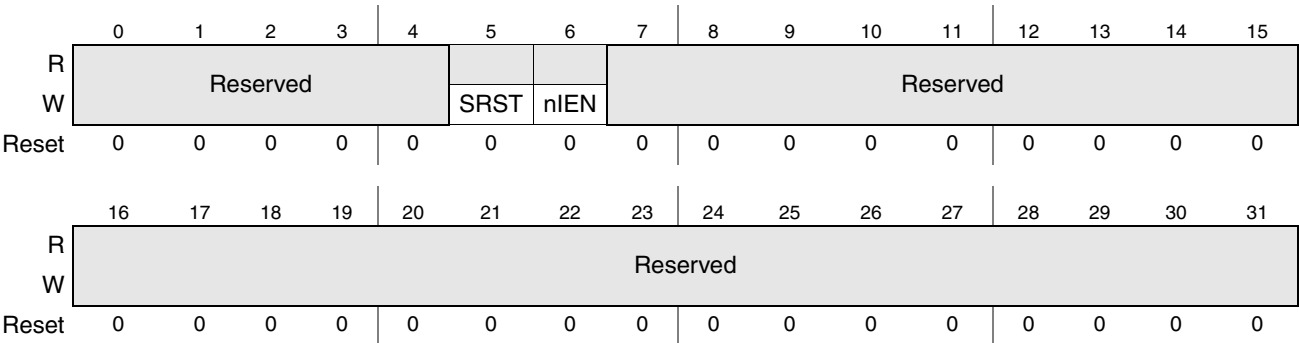
Figure 11-20. ATA Drive Device Control Register
