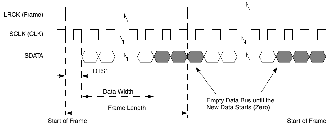
Figure 15-79. I 2 S Data Transmission
