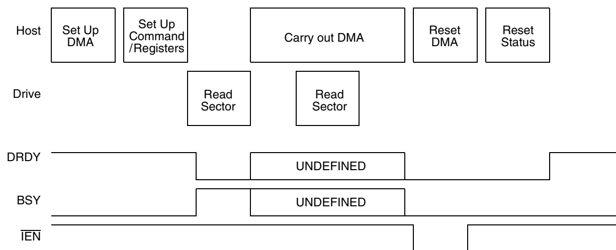
Figure 11-39. Timing Diagram—DMA Command (Class 4)
