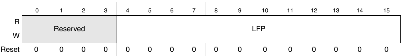
Figure 15-67. Tx FIFO Last Write Frame PTR Register
