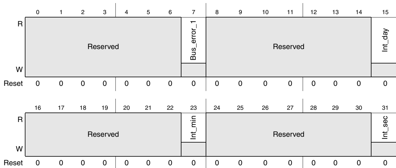
Figure 7-61. RTC Periodic Interrupt and Bus Error Register
