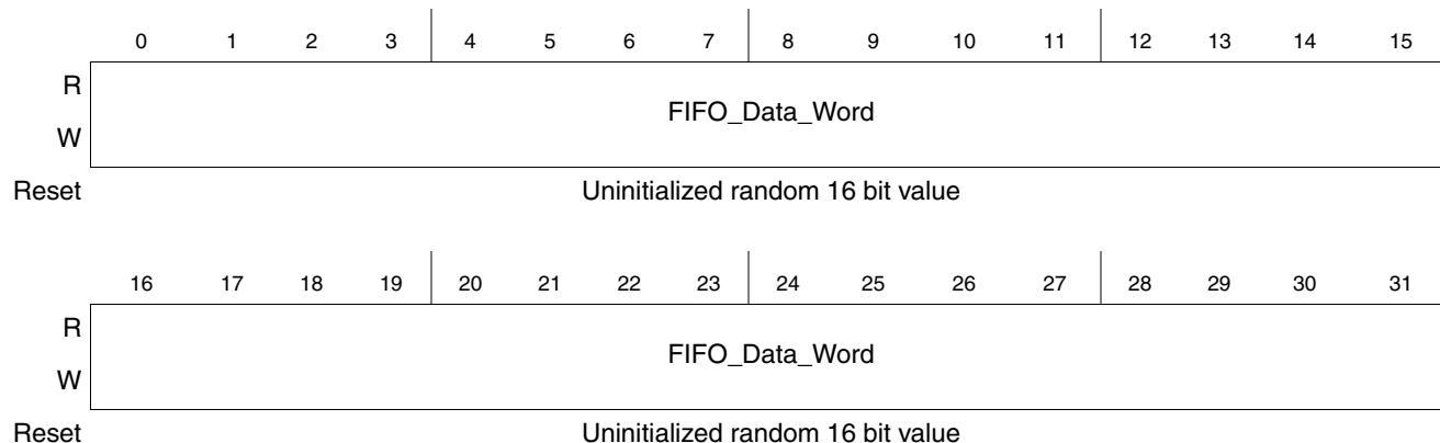
Figure 10-29. Tx FIFO Data Register PCITFDR(RW)
