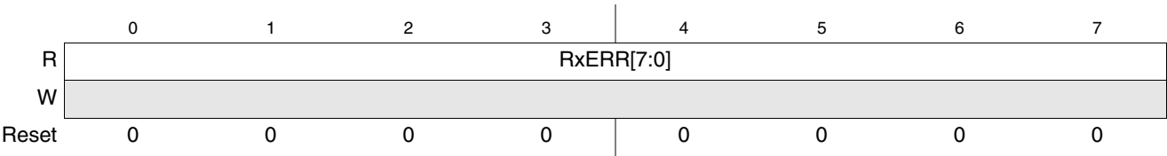
Figure 19-15. MSCAN Receive Error Counter Register
