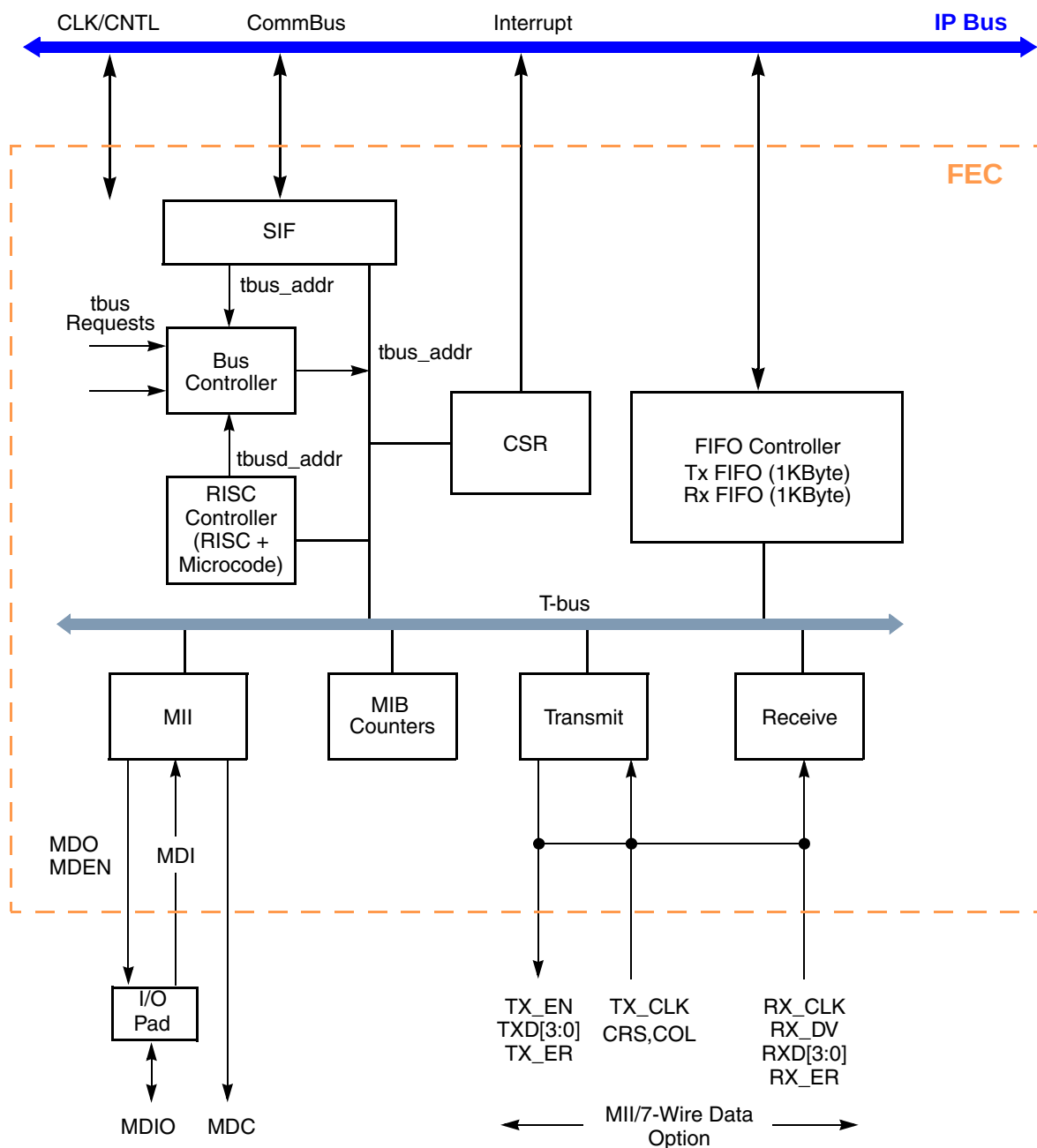
Figure 14-1. Block Diagram—FEC
