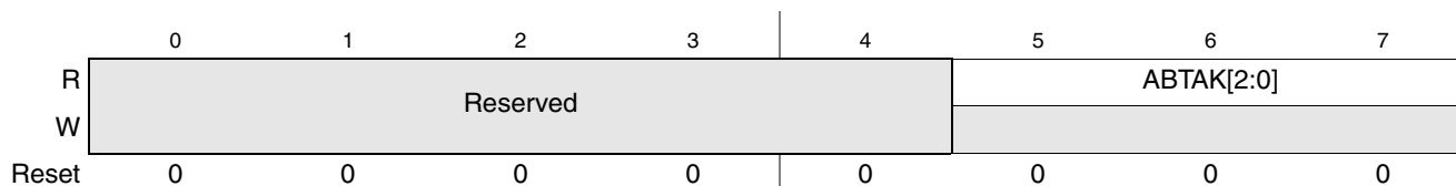
Figure 19-12. MSCAN Transmitter Message Abort Acknowledgement Register
