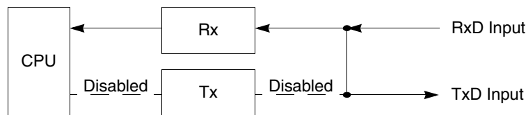
Figure 15-90. Automatic Echo
