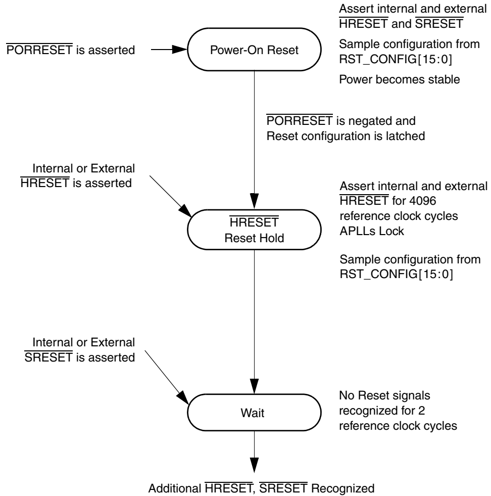
Figure 4-1. Reset sequence
