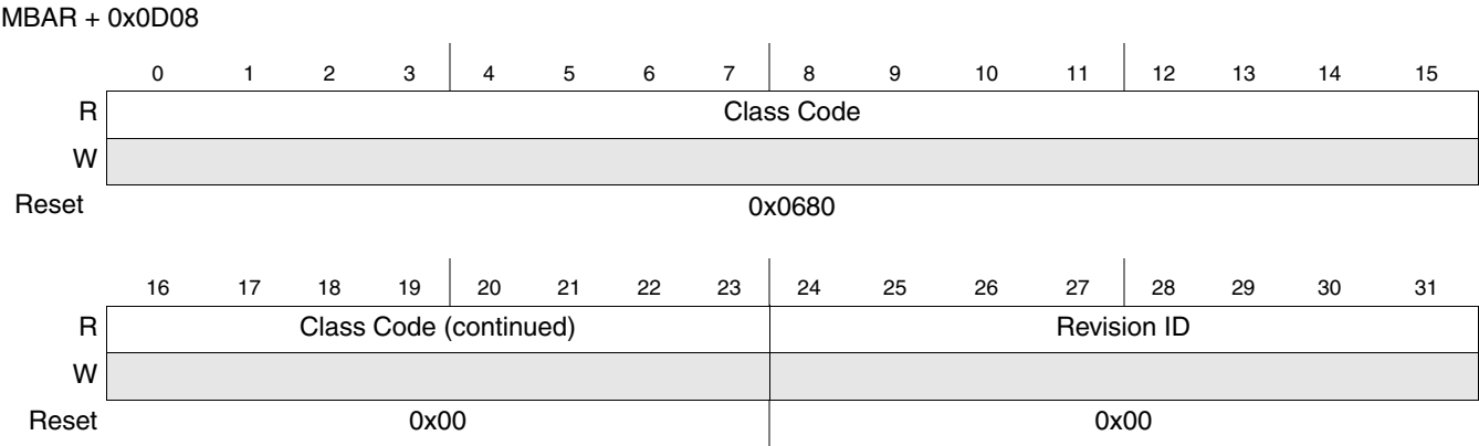
Figure 10-4. Revision ID/ Class Code Registers PCICCRIR(R)
