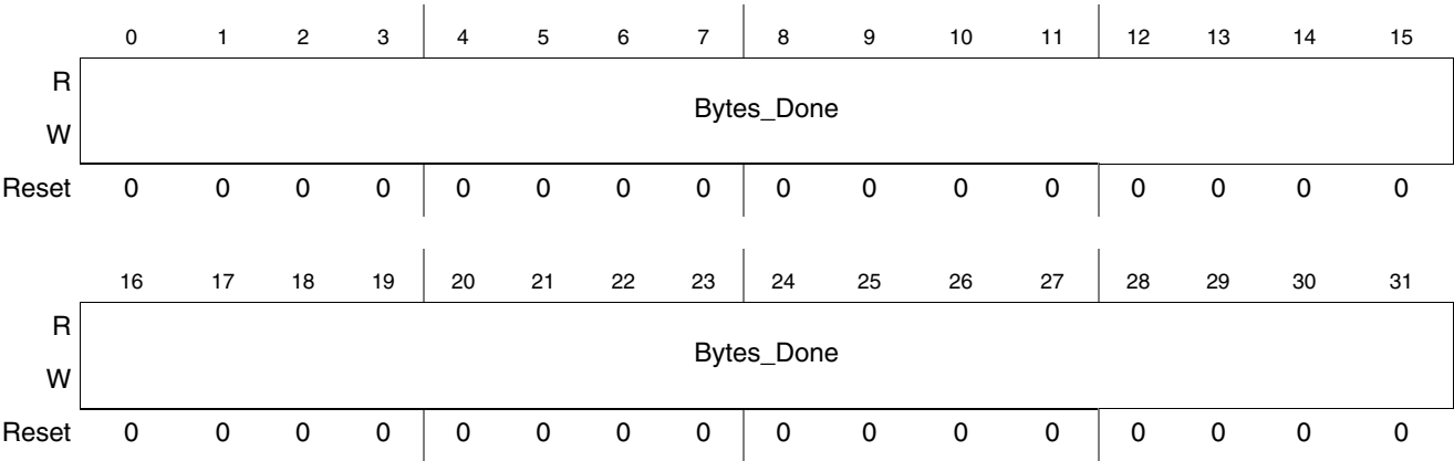
Figure 10-41. Rx Bytes Done Counts PCIRDCCR(R)
