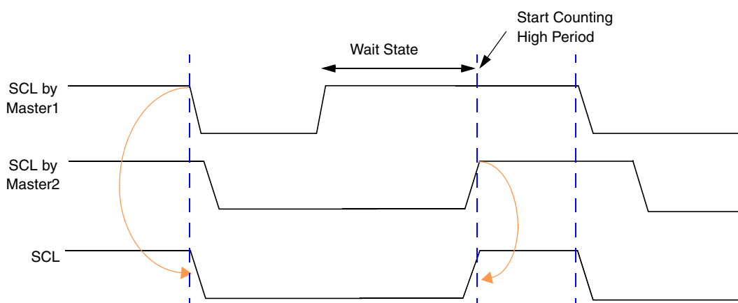
Figure 18-6. Timing Diagram—Clock Synchronization
