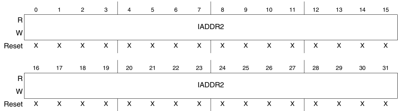
Figure 14-18. FEC Descriptor Individual Address 2 Register
