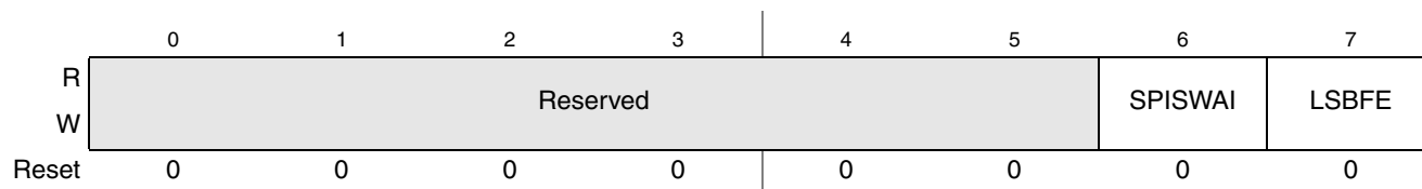
Figure 17-3. SPI Control Register 2
