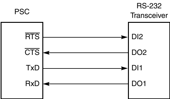
Figure 15-69. Signal Configuration for a PSC/RS-232 interface
