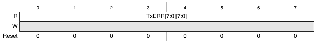
Figure 19-16. MSCAN Transmit Error Counter Register
