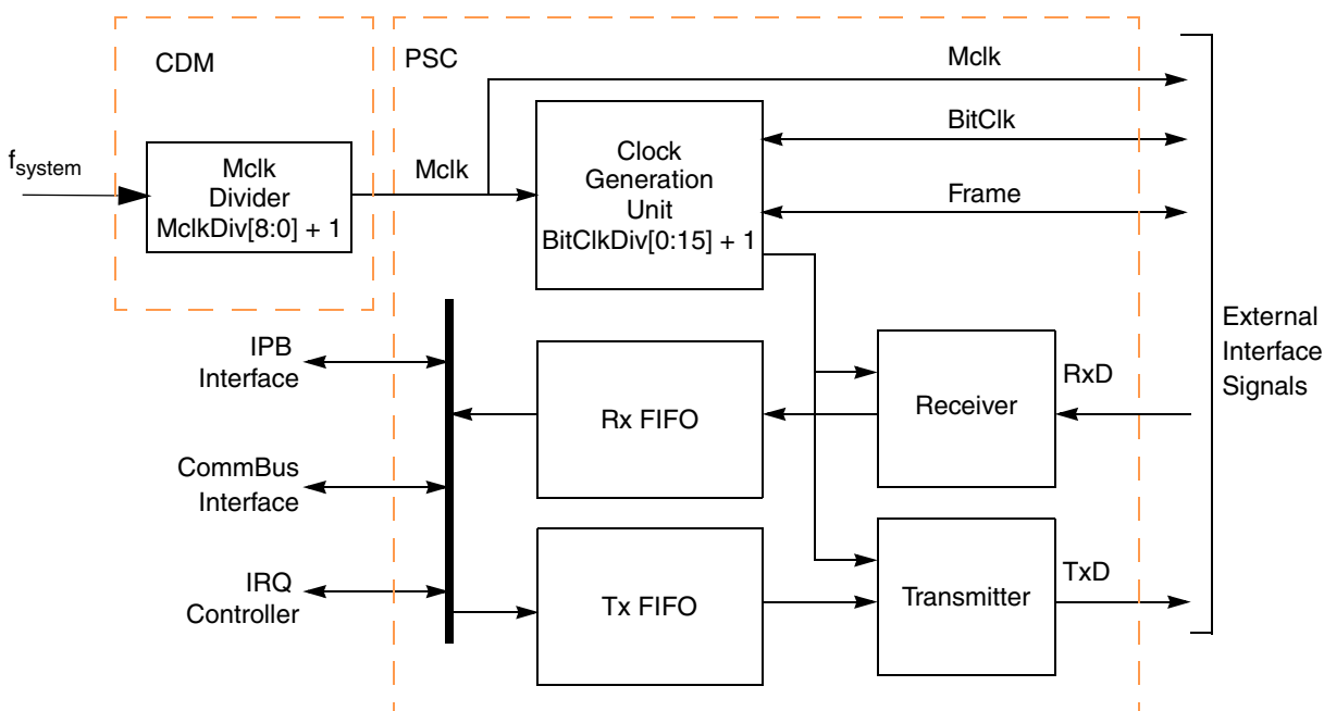
Figure 15-73. PSC Codec Block Diagram
