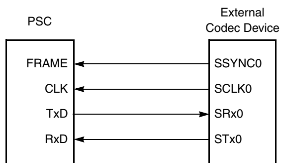
Figure 15-74. PSC Codec Interface in Slave Mode
