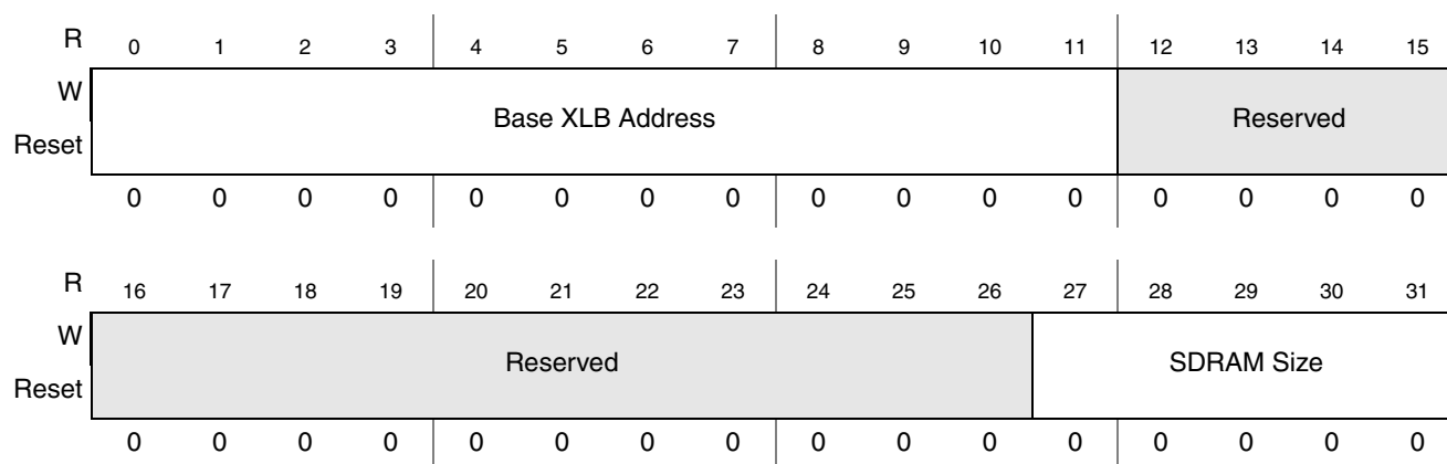
Figure 3-3. SDRAM Chip Select Configuration Register
