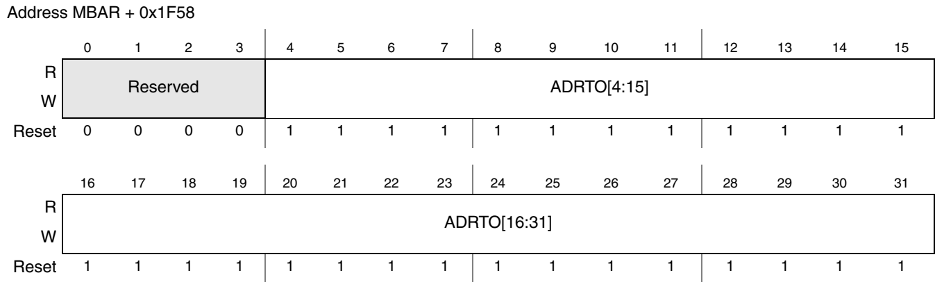
Figure 16-8. Arbiter Address Tenure Time-Out Register
