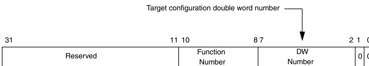
Figure 10-52. Contents of the AD Bus During Address Phase of a Type 0 Configuration Transaction
