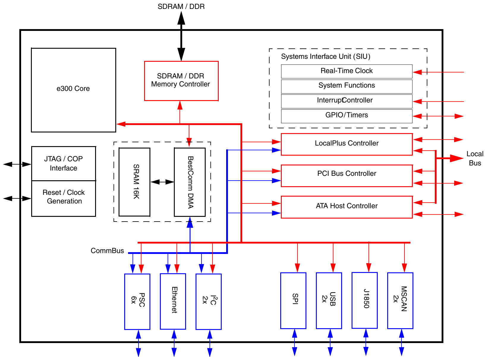
Figure 1-1. Simplified Block Diagram—MPC5200B
