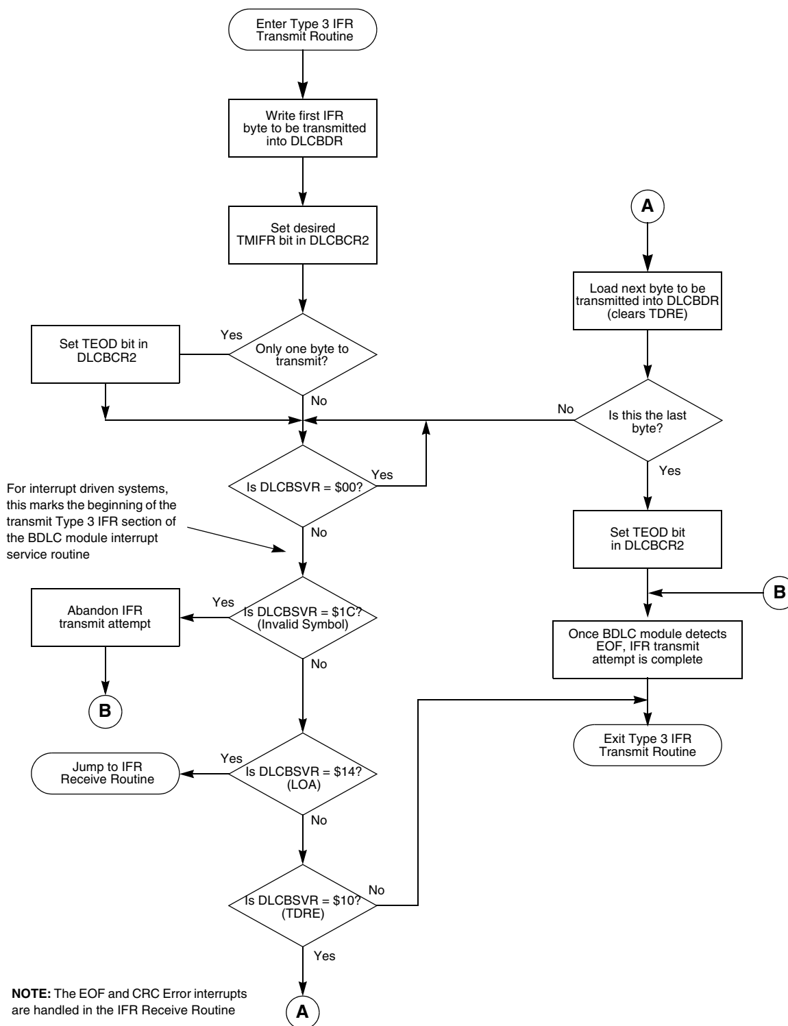
Figure 20-25. Transmitting A Type 3 IFR
