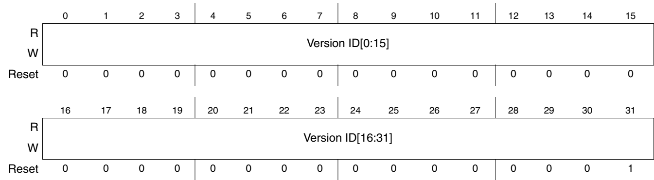
Figure 16-3. Arbiter Version Register
