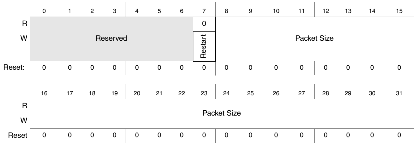
Figure 9-13. SCLPC Packet Size Register
