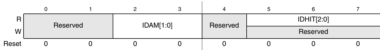
Figure 19-14. MSCAN ID Acceptance Control Register
