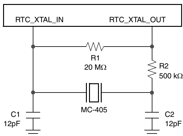
Figure 7-53. Diagram—Suggested Crystal Oscillator Circuit
