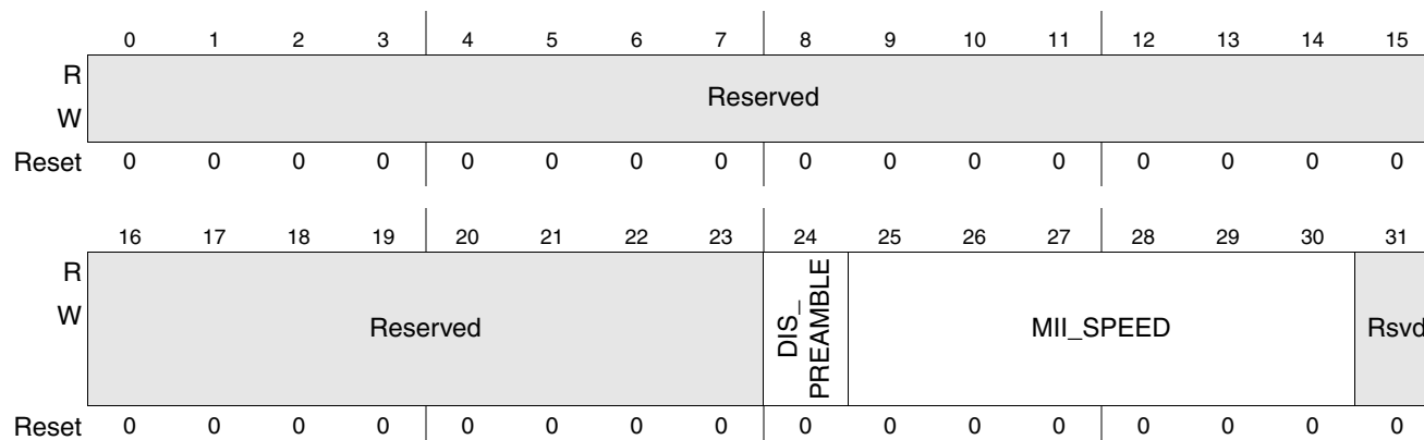
Figure 14-9. FEC MII Speed Control Register
