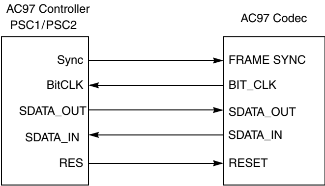
Figure 15-82. PSC—AC97 Interface
