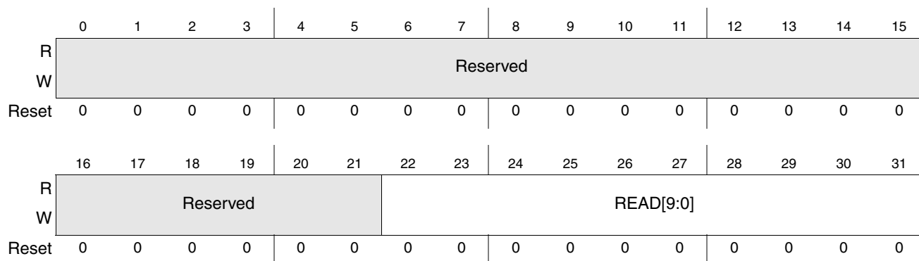
Figure 14-27. FEC Rx/Tx FIFO Read Pointer Register
