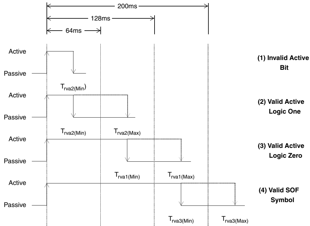
Figure 20-16. J1850 VPW Active Symbols
