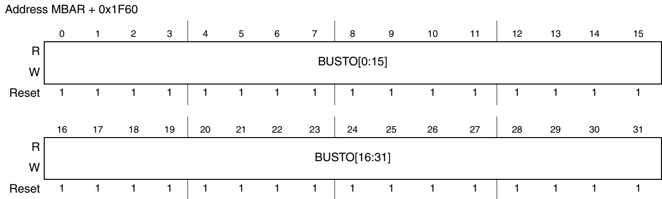
Figure 16-10. Arbiter Bus Activity Time-Out Register
