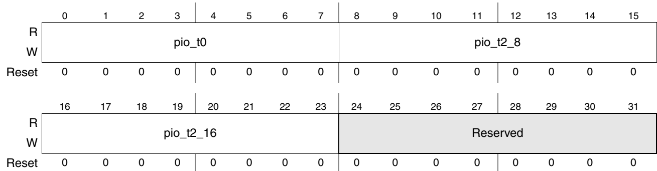
Figure 11-4. ATA PIO Timing 1 Register
