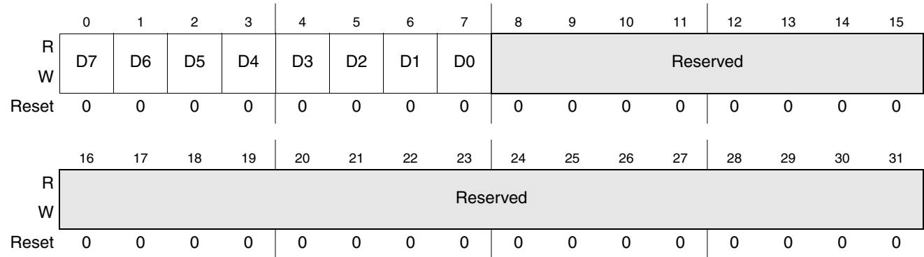
Figure 18-13. I 2 C Data I/O Register
