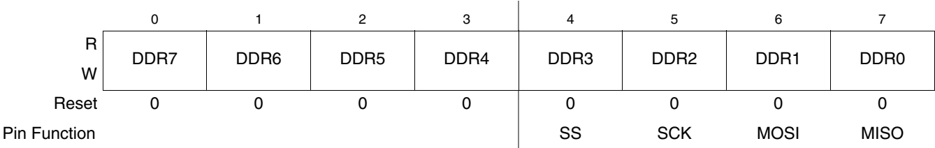
Figure 17-8. SPI Data Direction Register
