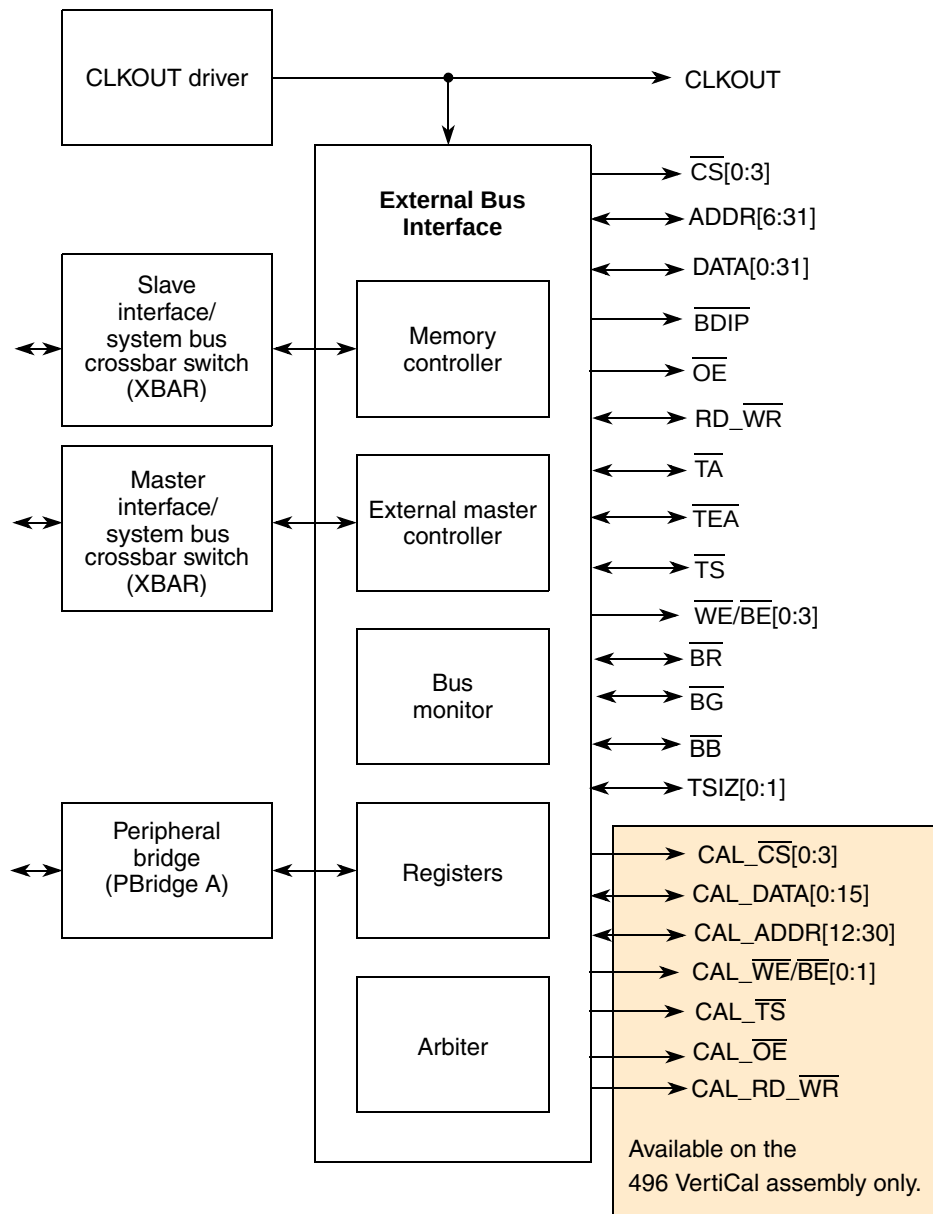
Figure 12-1. EBI Block Diagram
