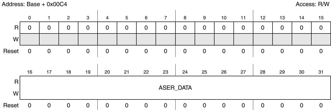
Figure 20-14. DSPI DSI Alternate Serialization Data Register (DSPIx_ASDR)
