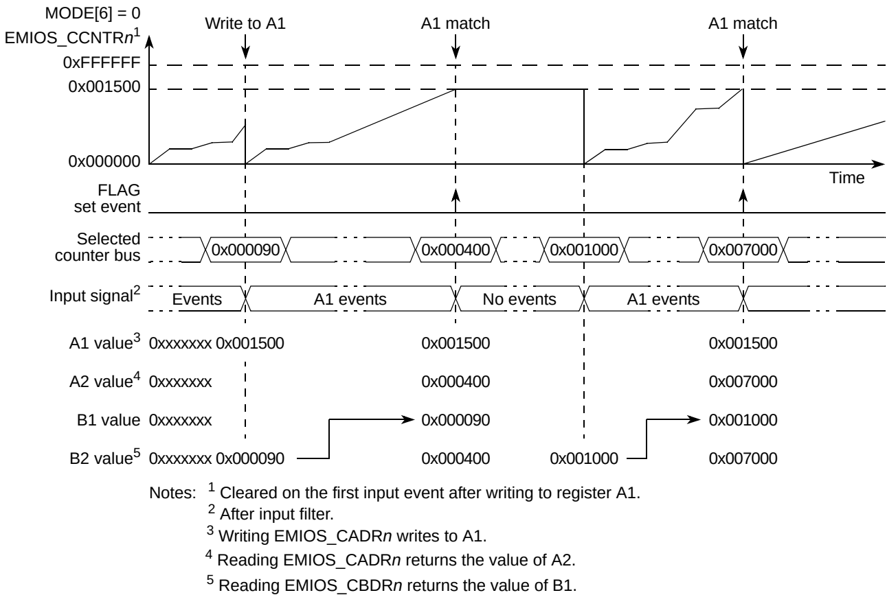
Figure 17-25. Pulse/Edge Accumulation Continuous Mode Example
