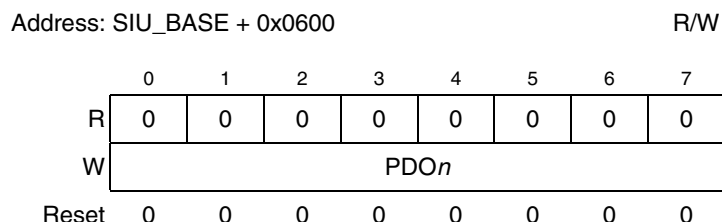
Figure 6-159. General Purpose Data Output (GPDO) Registers 0–213 (SIU_GPDO n )
