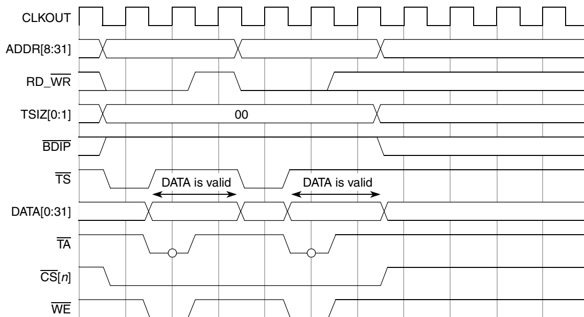
Figure 12-20. Back-to-Back 32-bit Writes to the Same \overline{\text{CS}} Bank
