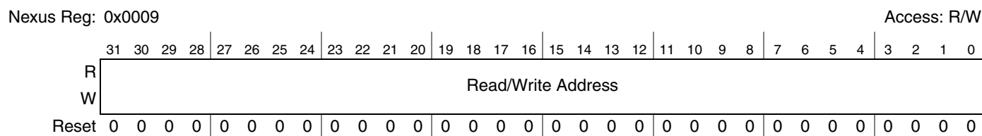
Figure 25-19. Read/Write Access Address Register (RWA)
