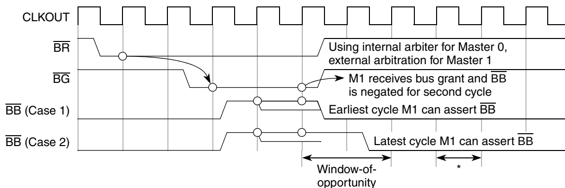
Figure 12-34. Internal Arbitration, Two-Cycle Window-of-Opportunity
