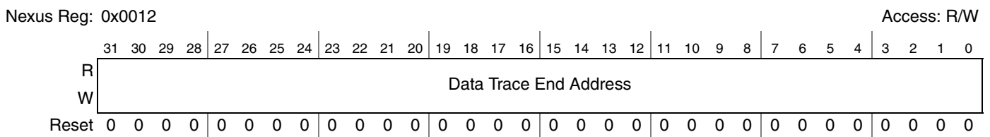
Figure 25-25. Data Trace End Address Register 1 (DTEA1)
