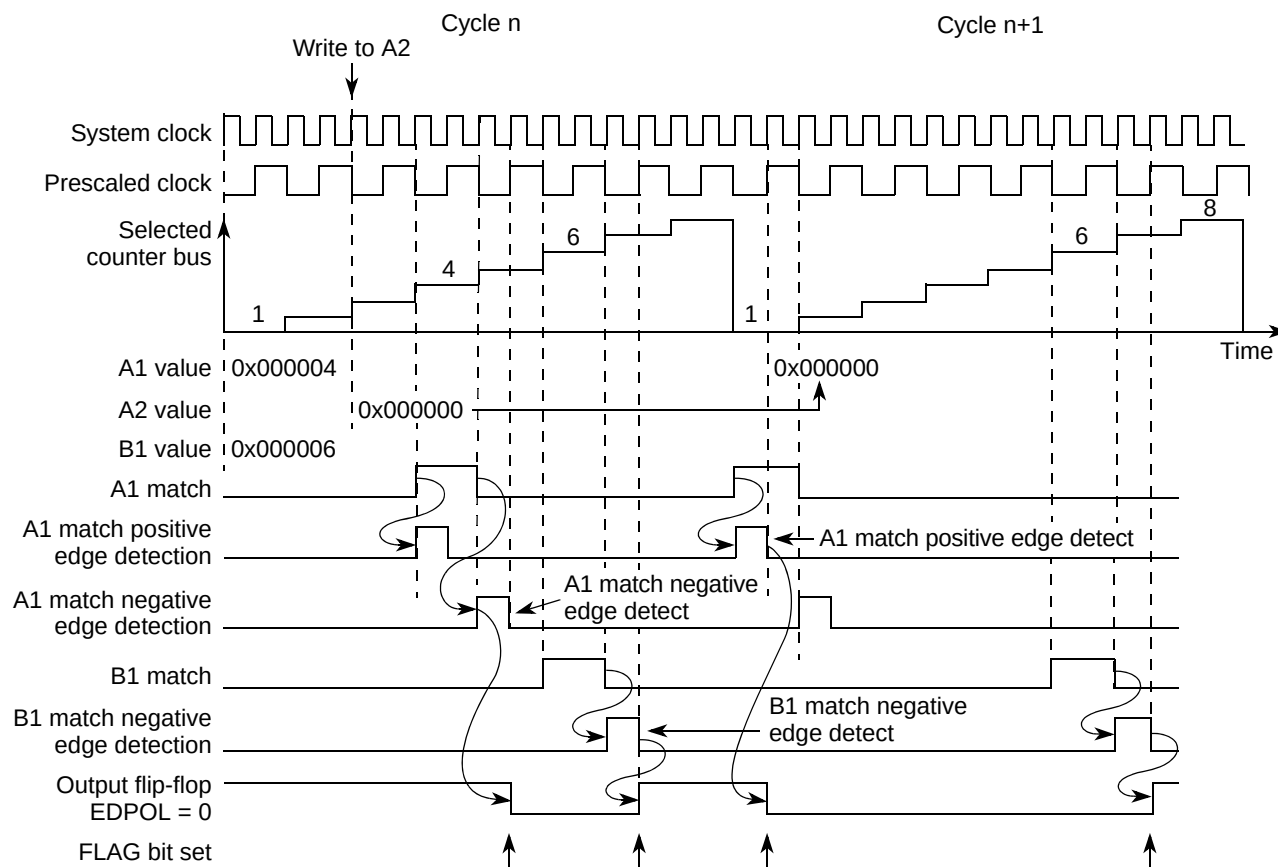
Figure 17-53. eMIOS OPWMB Mode Example — Matches and Flags
