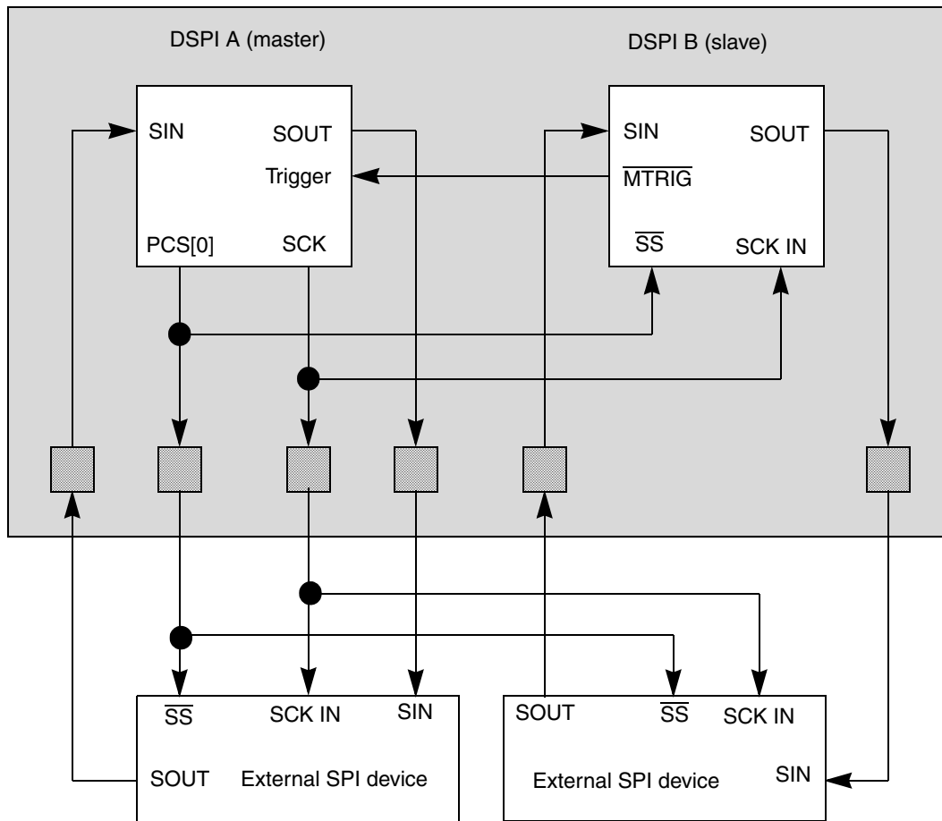
Figure 6-175. DSPI Parallel Chaining
