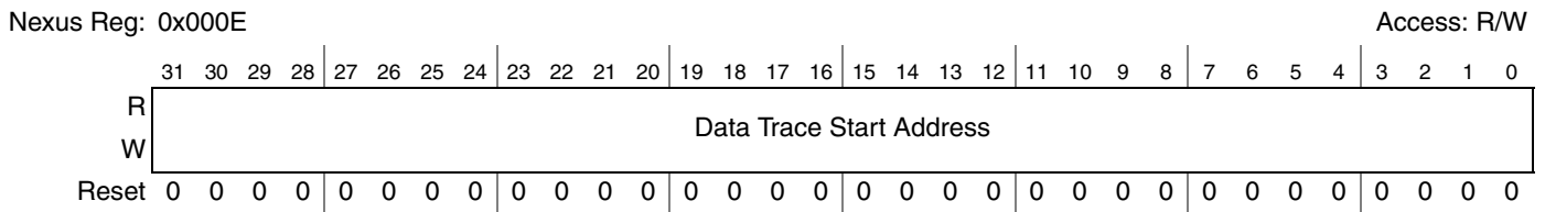
Figure 25-23. Data Trace Start Address Register 1 (DTSA1)
