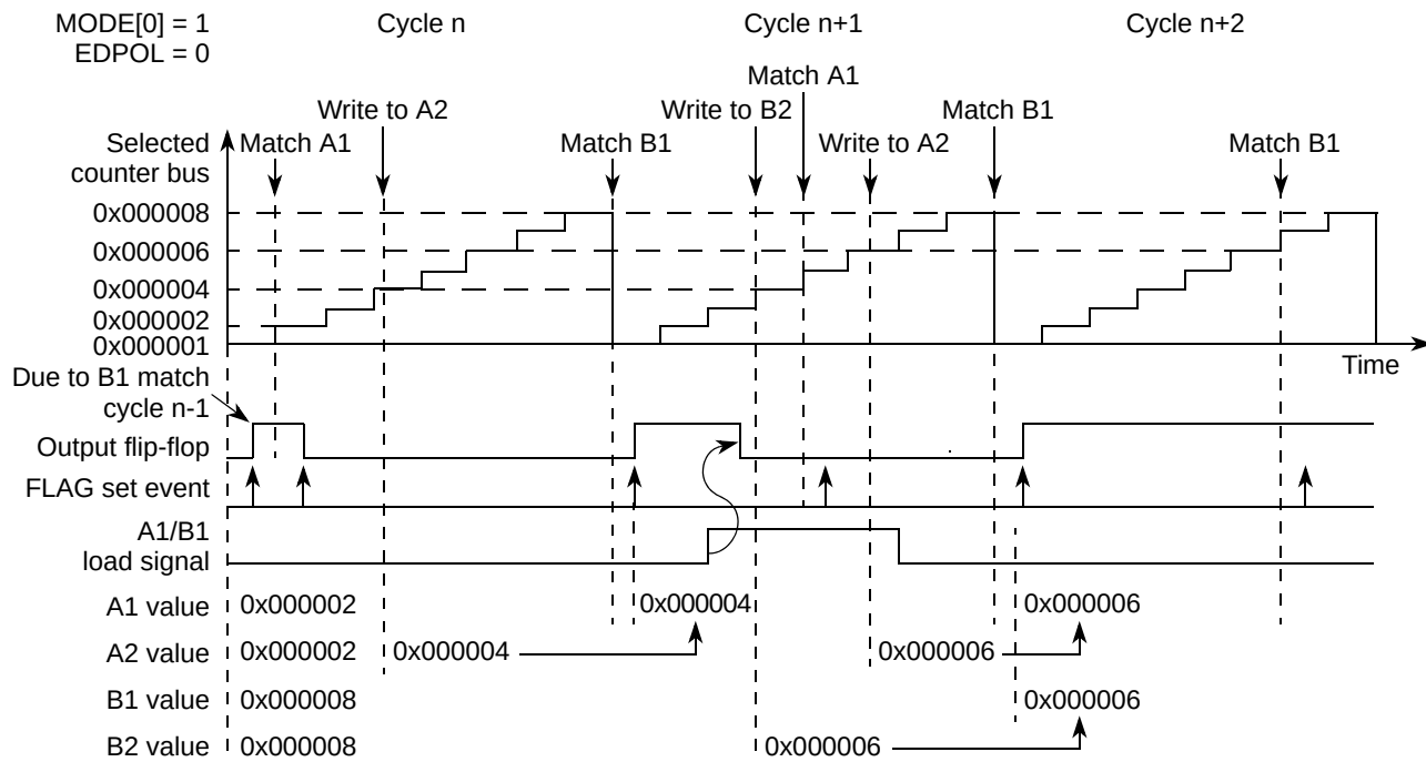
Figure 17-55. eMIOS OPWMB Mode Example — Active Output Disable
