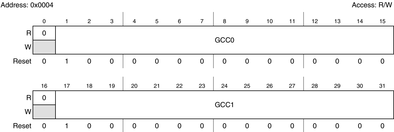
Figure 19-22. ADCn Gain Calibration Constant Registers (ADCn_GCCR)
