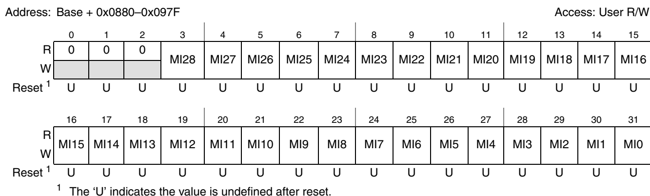
Figure 22-7. RX Individual Mask Registers (CANx_RXIMR0 through CANx_RXIMR63)
