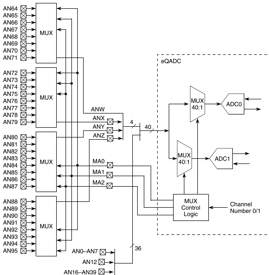
Figure 19-53. Example of External Multiplexing
