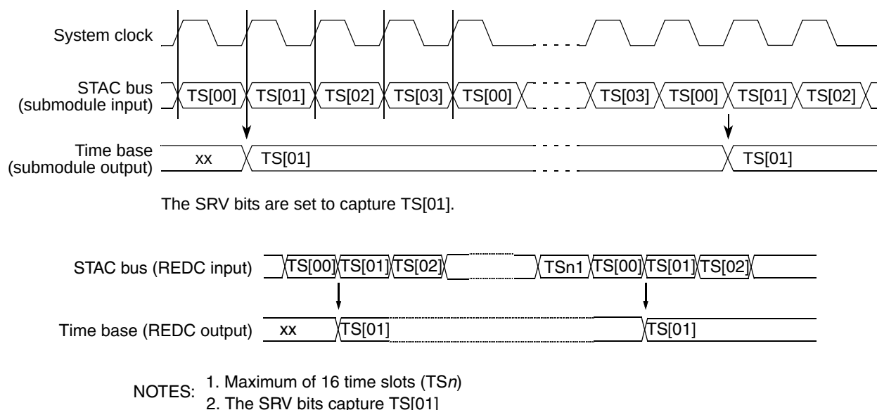
Figure 17-12. Timing Diagram for the STAC Bus and STAC Client Submodule Output
