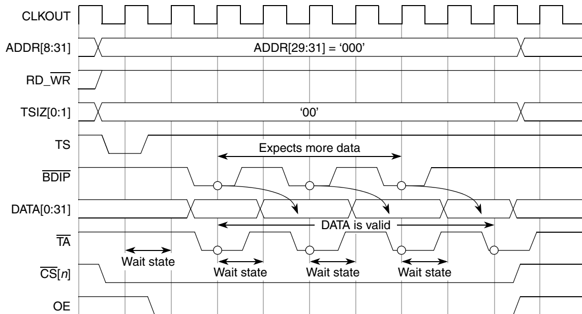
Figure 12-26. Burst 32-bit Read Cycle, One Wait State between Beats, \text{TBDIP} = 1
