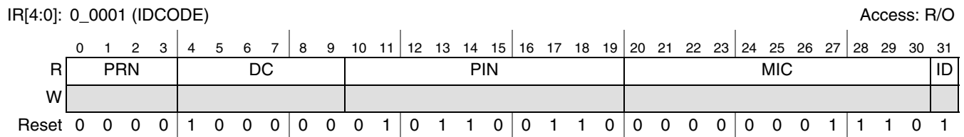
Figure 24-3. Device Identification Register
