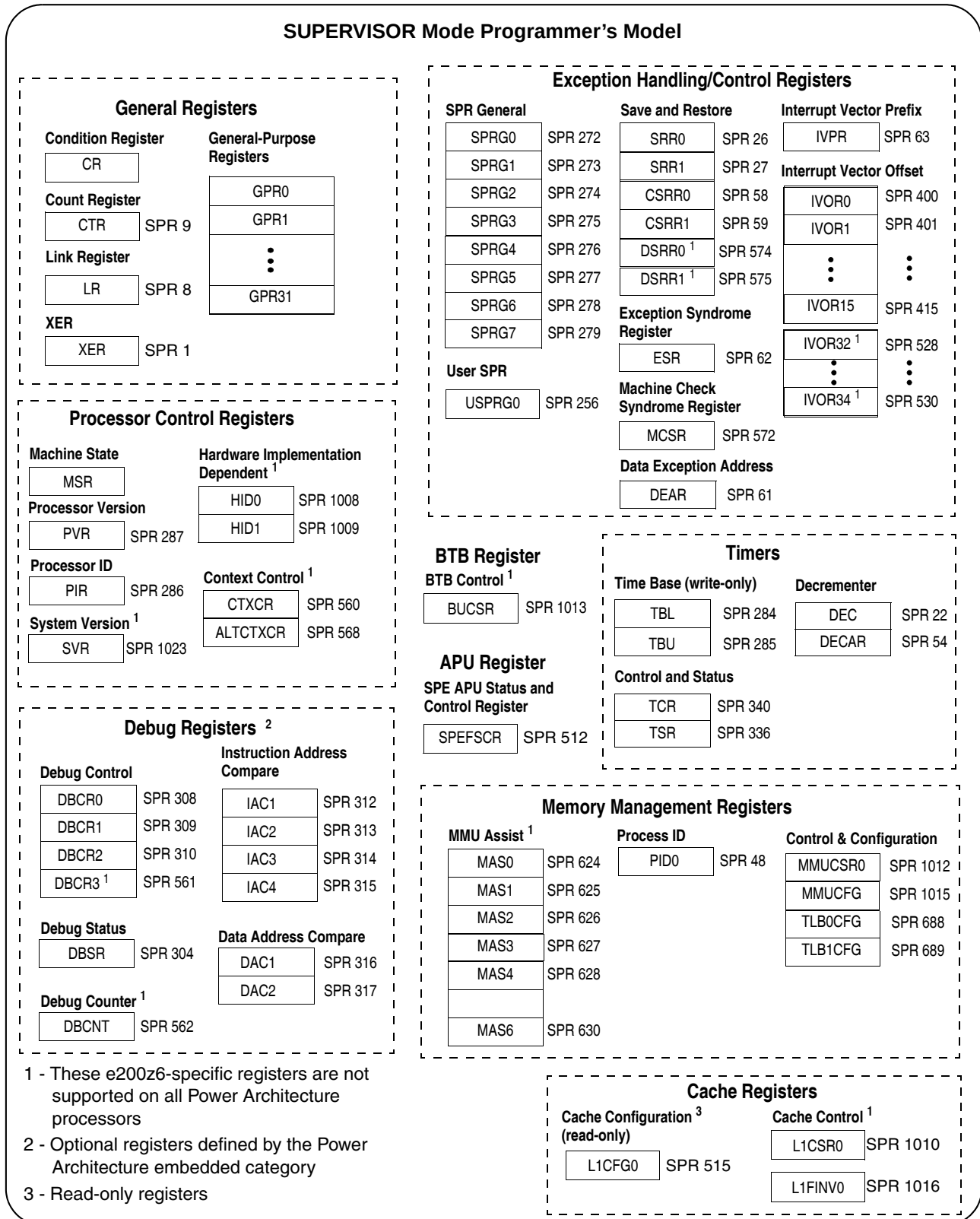
Figure 3-2. Supervisor Mode Programmer's Model
