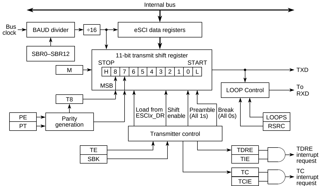
Figure 21-13. eSCI Transmitter Block Diagram
