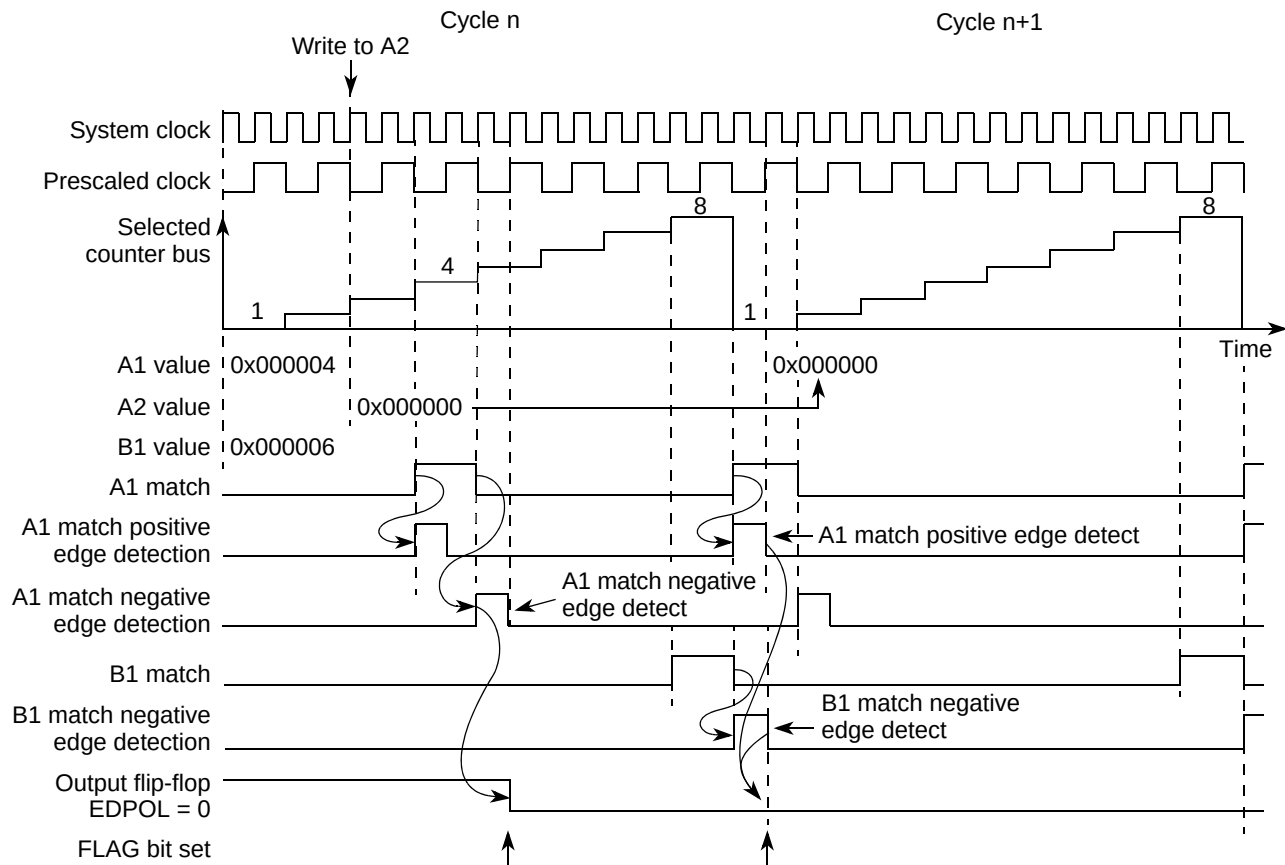
Figure 17-54. eMIOS OPWMB Mode Example — 0% Duty Cycle
