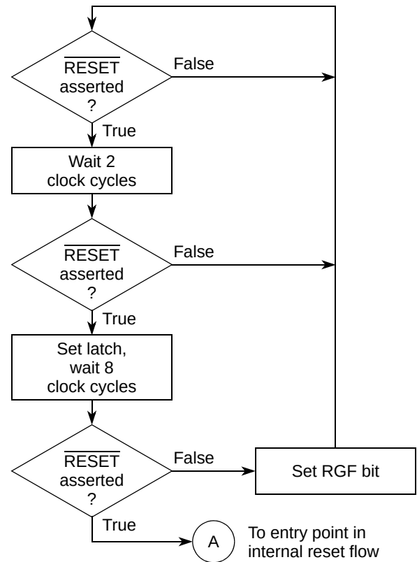
Figure 4-5. External Reset Flow Diagram
