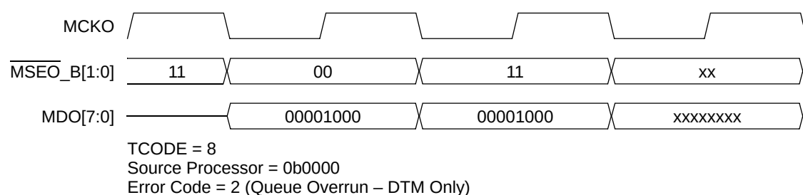
Figure 25-49. Error Message (Data Trace only encoded)
