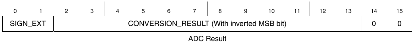
Figure 19-29. ADC Result Format when FMT = 1 (Right Justified Signed)—On-Chip ADC Operation
