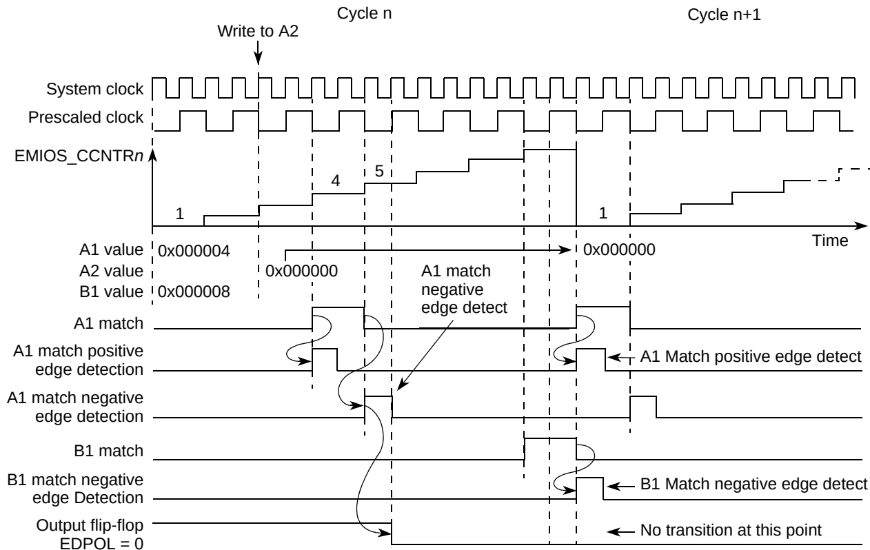
Figure 17-45. eMIOS OPWFMB Mode Example — A1 = 0 (0% Duty Cycle)
