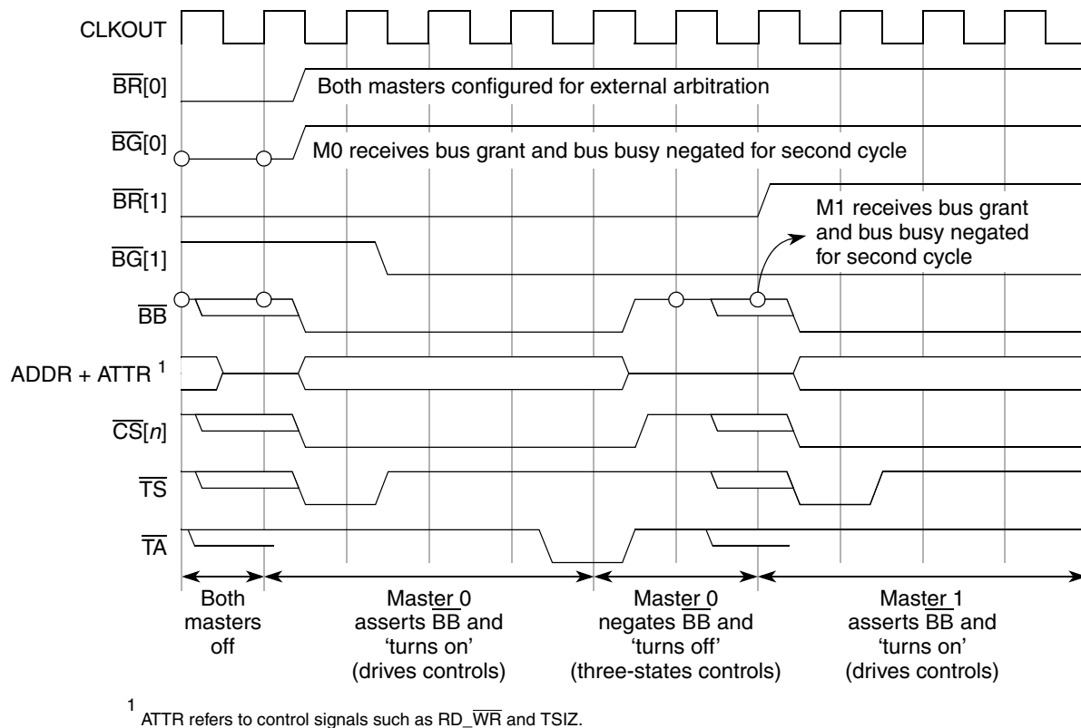
Figure 12-33. Central Arbitration Timing Diagram
