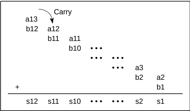
Figure 19-63. RSD Adder
