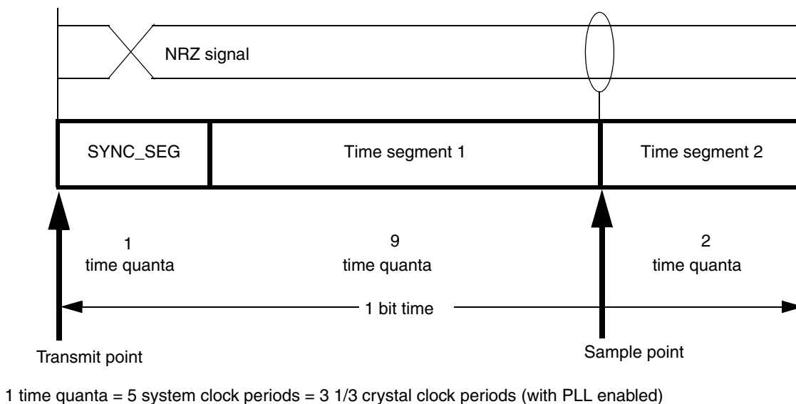
Figure 16-5. FlexCAN Bit Timing
