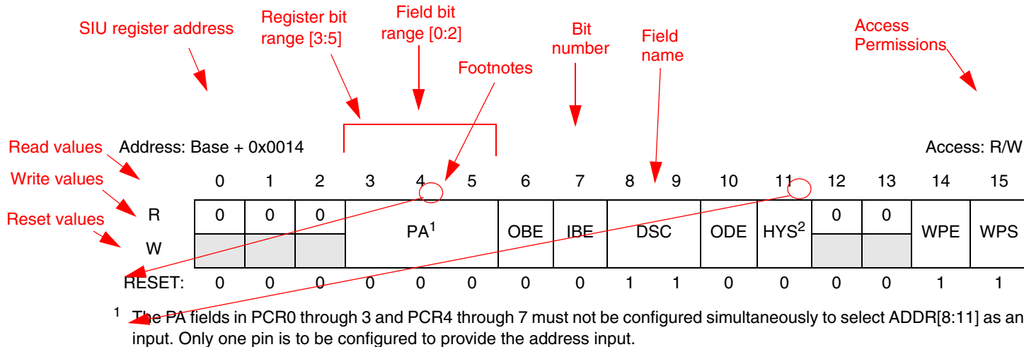
Figure 6-13. Sample PCR Register Description
