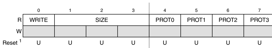
Figure 8-6. Flash ECC Attributes Register (ECSM_FEAT)
