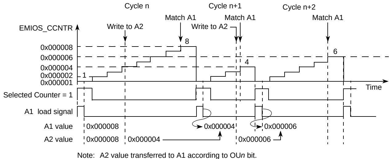
Figure 17-42. eMIOS MCB Mode Example — Up Operation A1 Register Update
