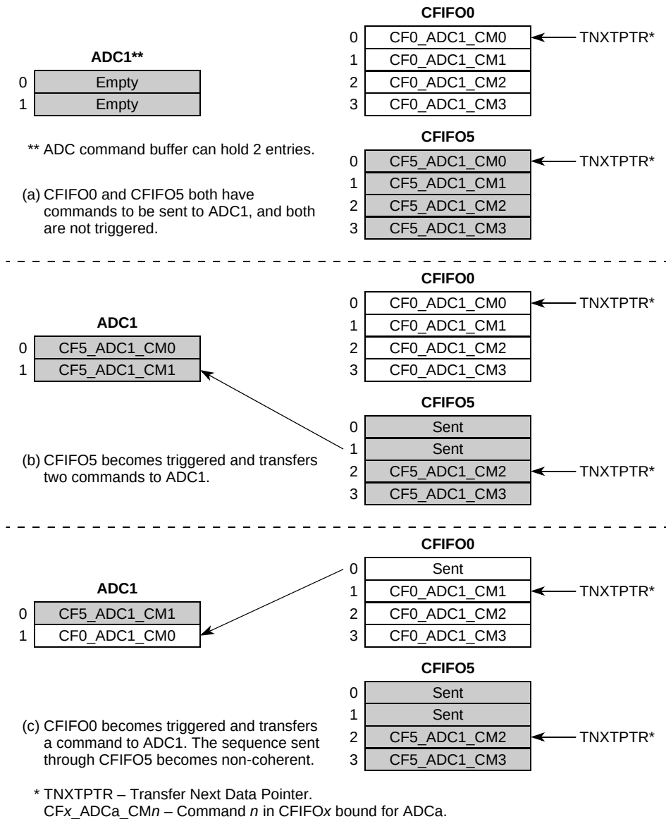
Figure 19-43. Non-Coherency Event When Different CFIFOs Use the Same Buffer
