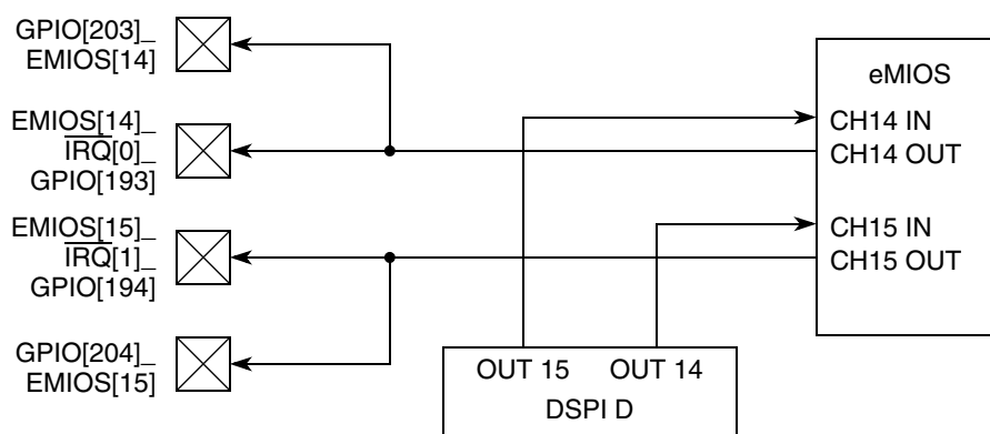
Figure 2-10. EMIO[14:15]—DSPI D I/O Connections
