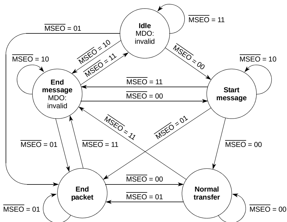
Figure 25-5. \overline{\text{MSEO}} Transfers
