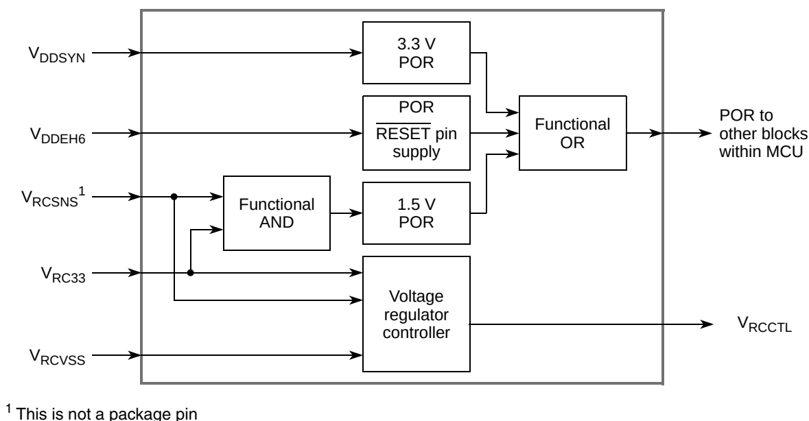
Figure 23-1. Voltage Regulator Controller and POR Blocks
