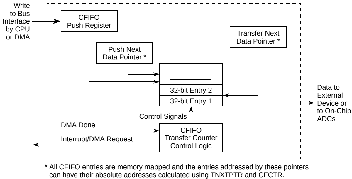
Figure 19-35. CFIFO Diagram
