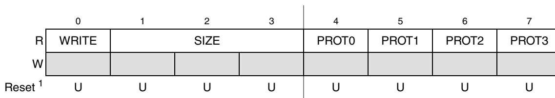
Figure 8-11. RAM ECC Attributes Register (ECSM_REAT)
