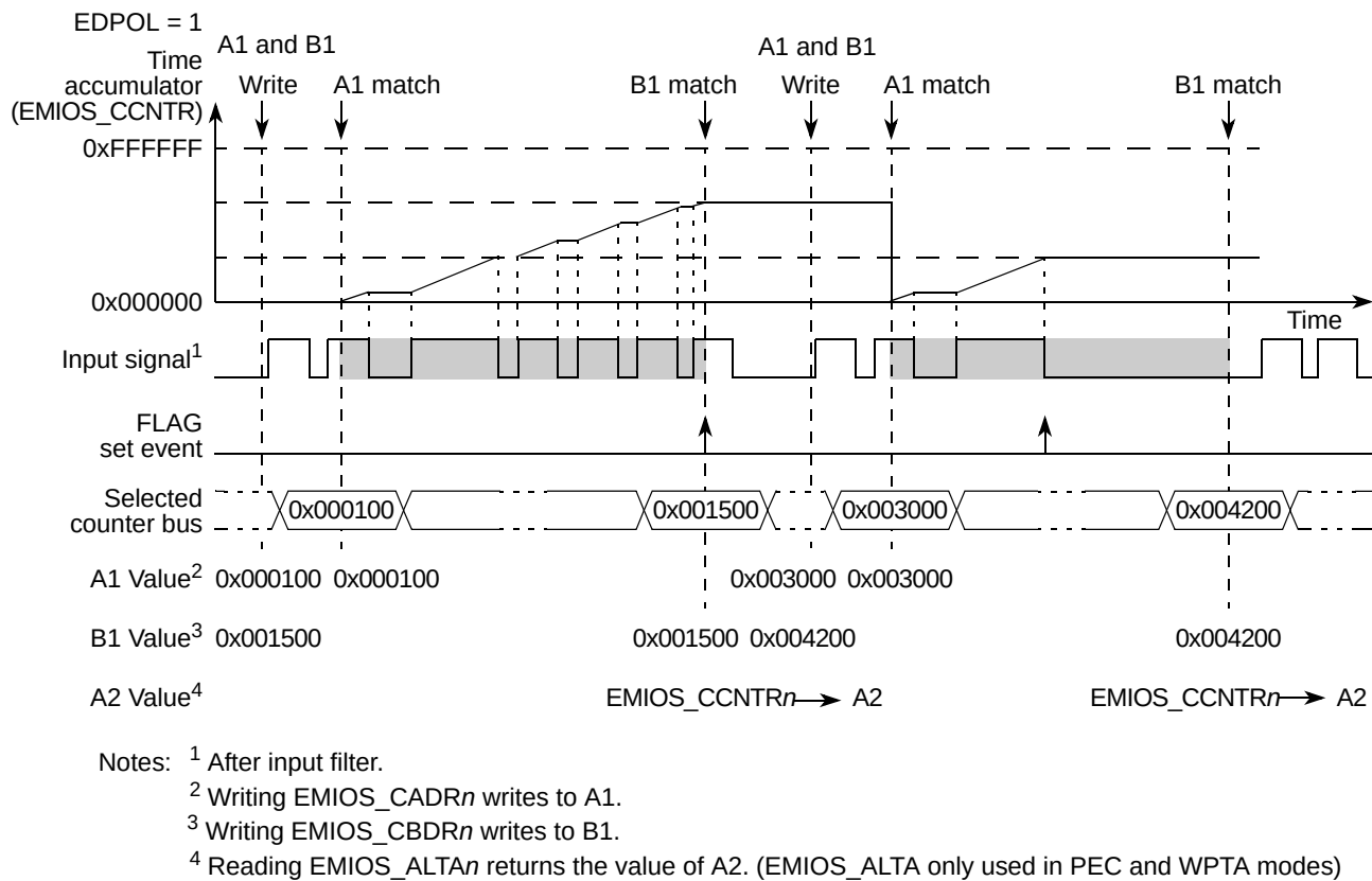
Figure 17-31. Windowed Programmable Time Accumulation Example
