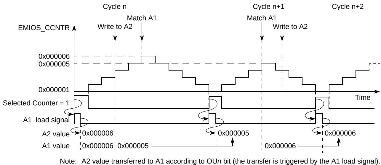
Figure 17-43. eMIOS MCB Mode Example — Up/Down Operation A1 Register Update
