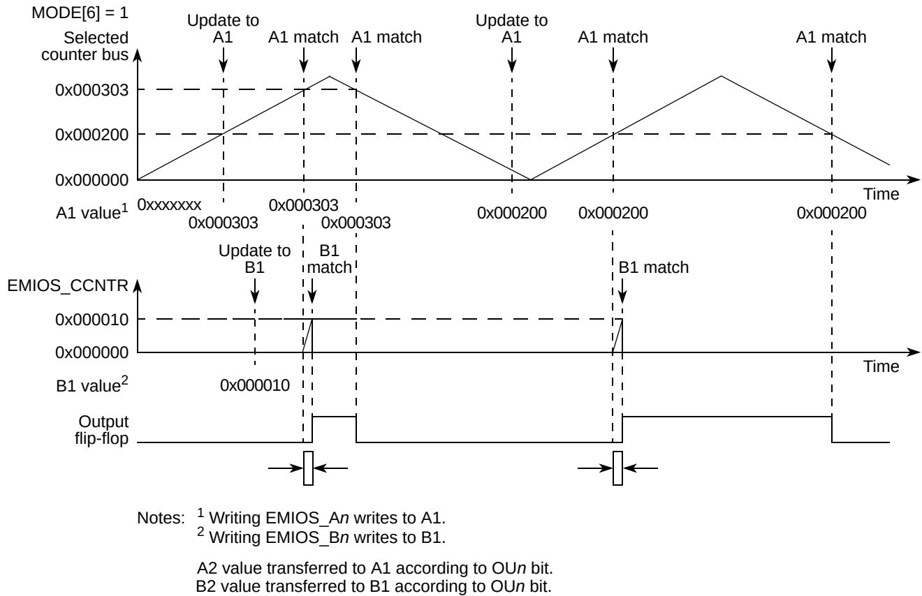
Figure 17-36. Output PWM with Leading Dead-time Insertion
