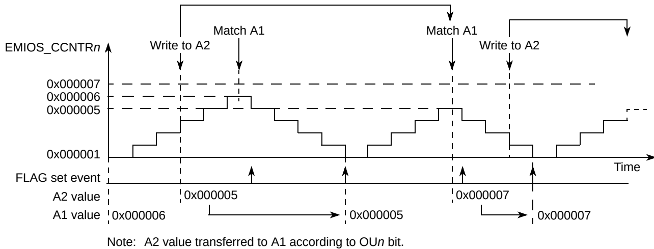
Figure 17-41. eMIOS MCB Mode Example — Up/Down Operation
