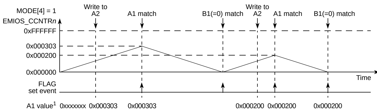
Figure 17-32. Modulus Counter Up Mode Example
