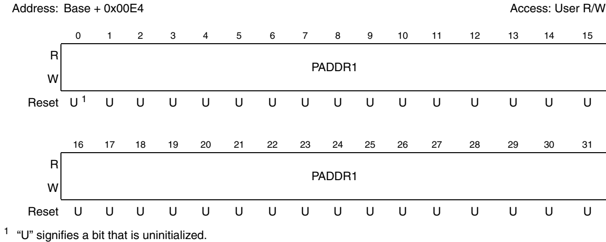
Figure 15-13. Physical Address Low Register (PALR)
