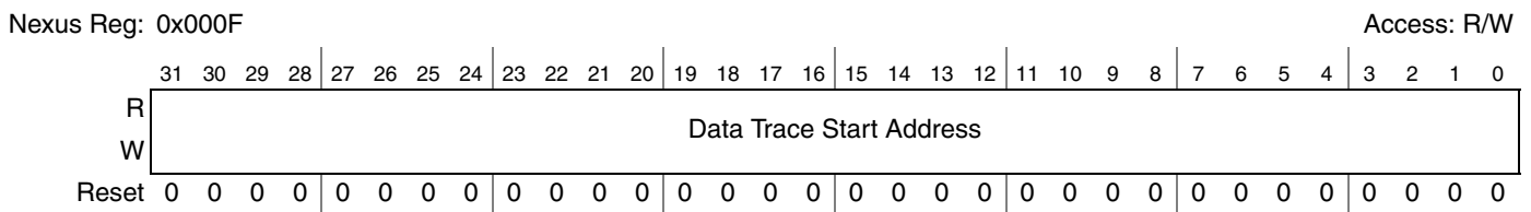
Figure 25-24. Data Trace Start Address Register 2 (DTSA2)
