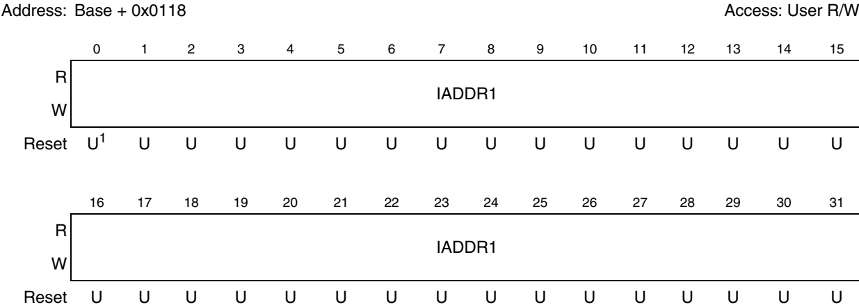
Figure 15-18. Descriptor Individual Upper Address Register (IAUR)
