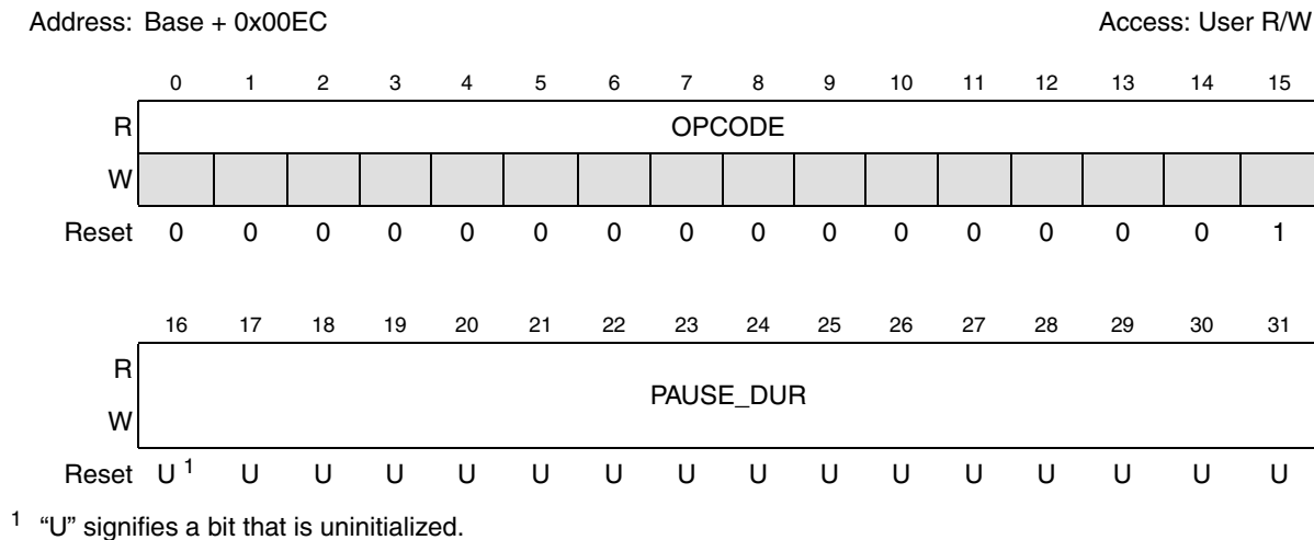
Figure 15-15. Opcode/Pause Duration Register (OPD)
