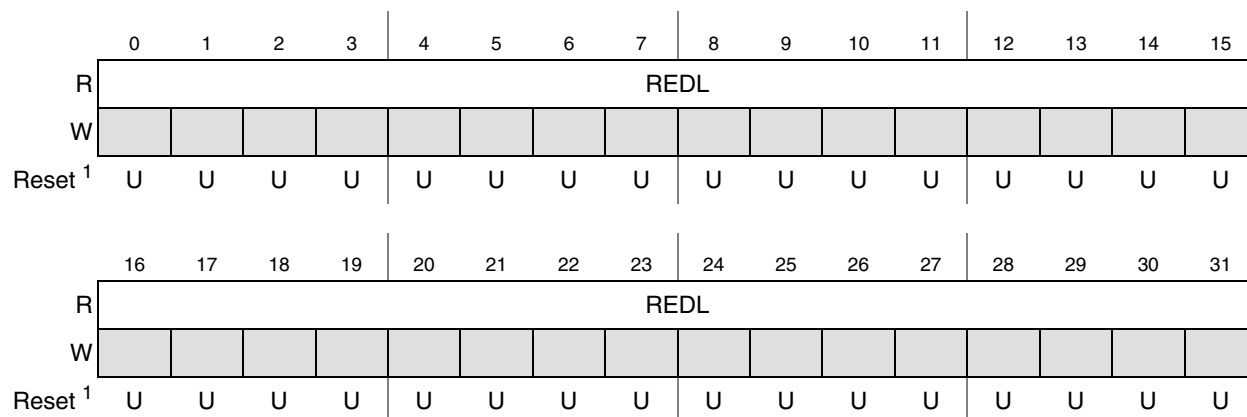
Figure 8-13. RAM ECC Data Low Register (ECSM_REDRL)
