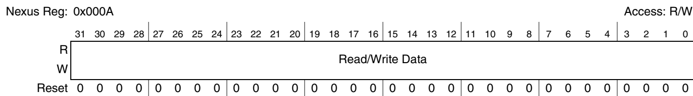
Figure 25-20. Read/Write Access Data Register (RWD)
