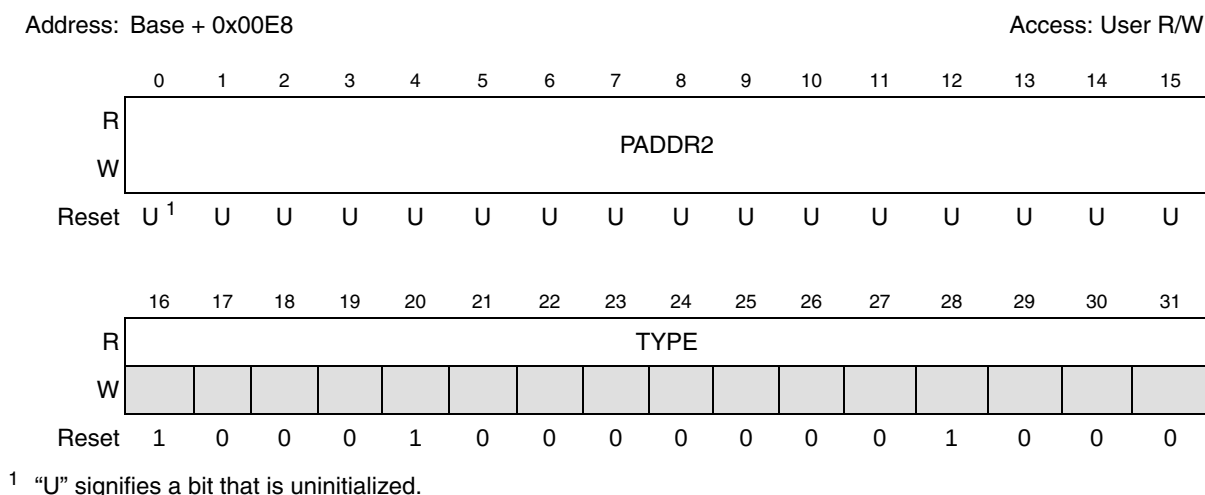
Figure 15-14. Physical Address Upper Register (PAUR)
