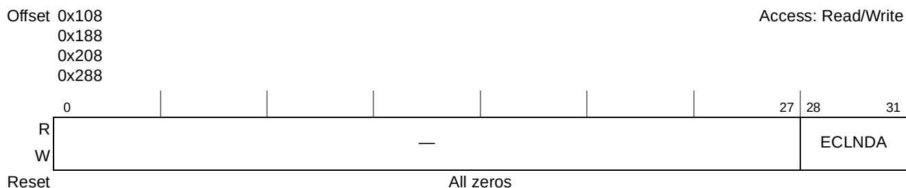
Figure 13-6. Extended Current Link Descriptor Address Registers (ECLNDAR n )
