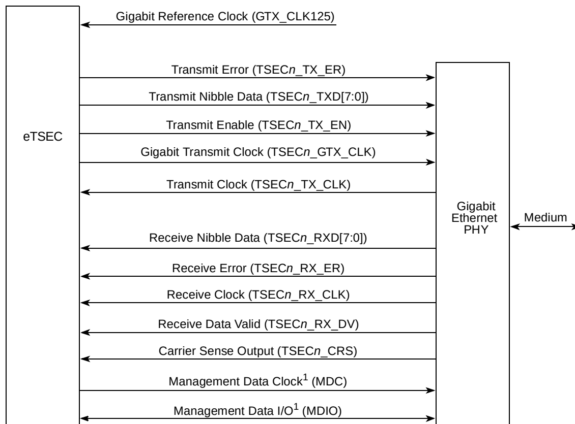
Figure 14-134. eTSEC-GMII Connection
