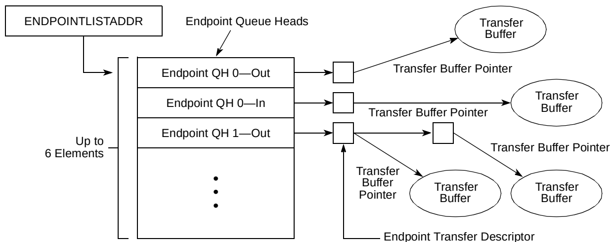
Figure 18-64. Endpoint Queue Head Diagram
