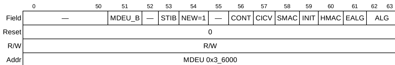
Figure 20-81. MDEU Mode Register in New Configuration
