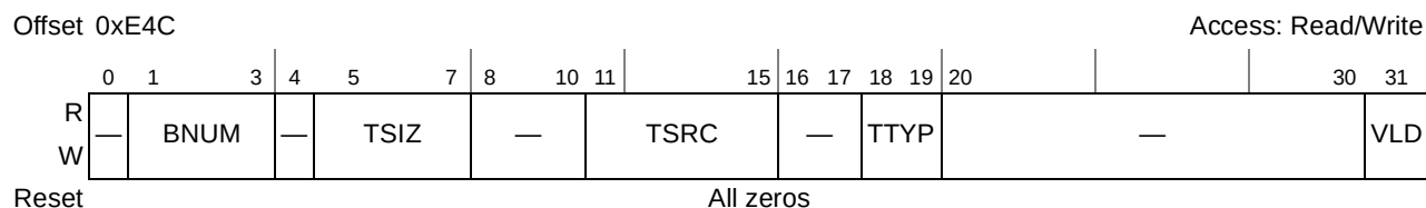
Figure 8-43. Memory Error Attributes Capture Register (CAPTURE_ATTRIBUTES)
