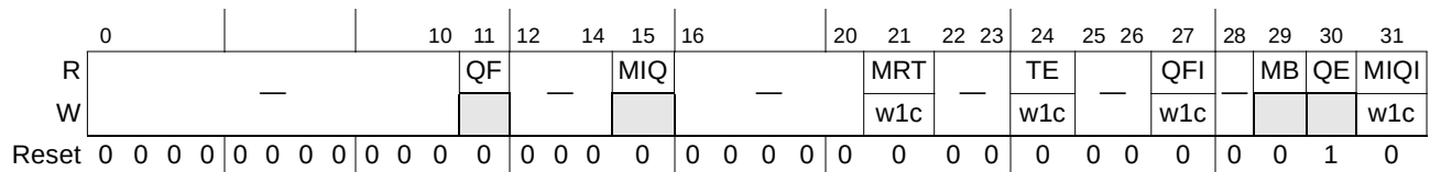
Figure 15-79. Inbound Message n Status Registers (IMnSR)
