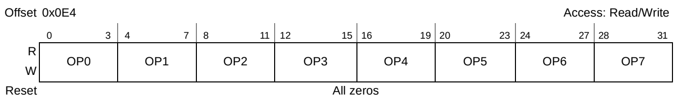
Figure 12-22. Flash Instruction Register
