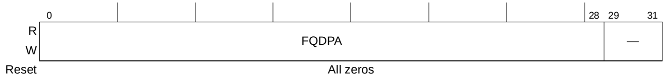
Figure 15-81. Inbound Message n Frame Queue Dequeue Pointer Address Registers (IMnFQDPAR)
