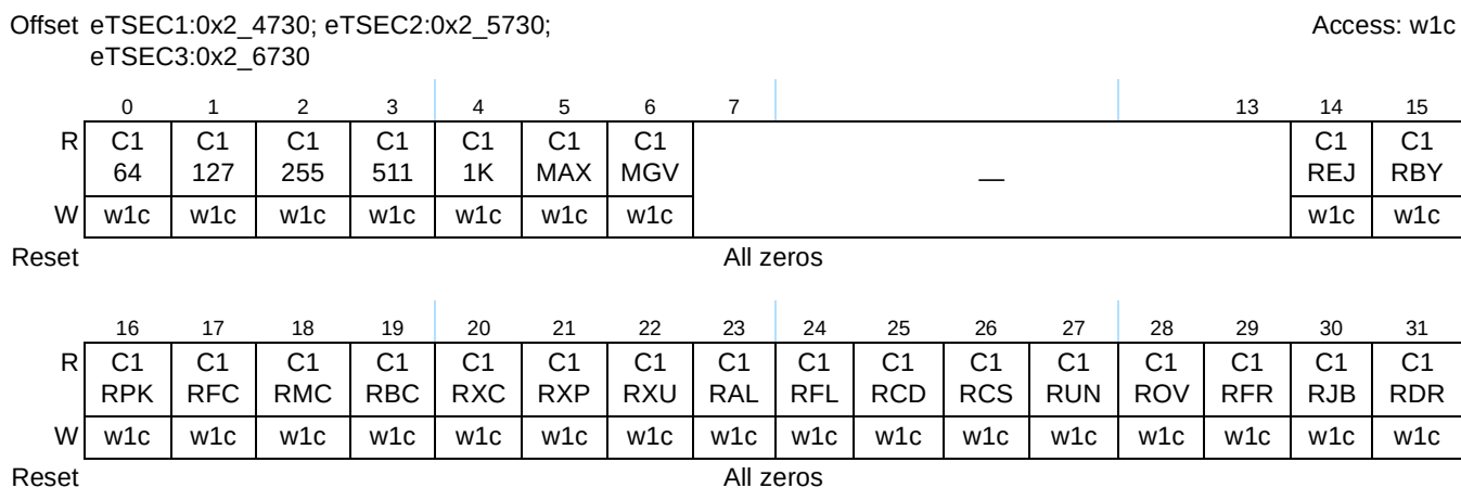
Figure 14-98. Carry Register 1 (CAR1) Register Definition
