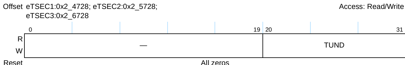
Figure 14-96. Transmit Undersize Frame Counter Register Definition
