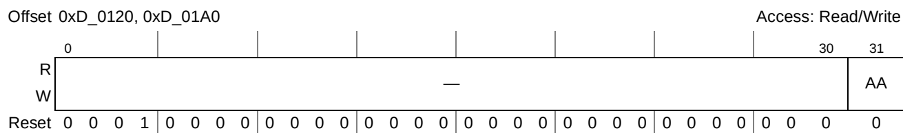
Figure 15-45. Port m Accept-All Configuration Register (PmAACR)
