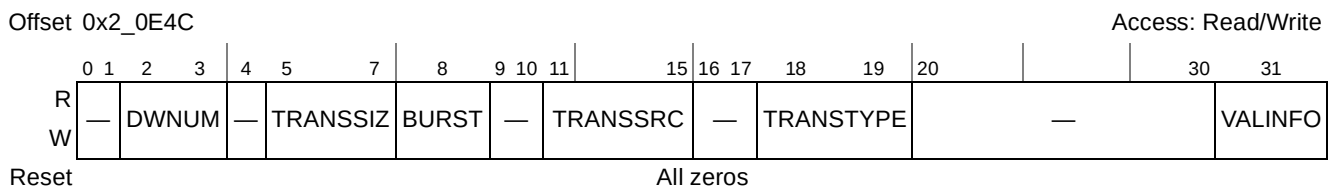
Figure 6-23. L2 Error Attributes Capture Register (L2ERRATTR)
