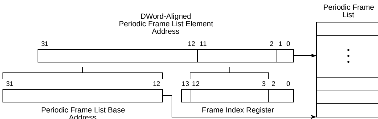
Figure 18-43. Derivation of Pointer into Frame List Array
