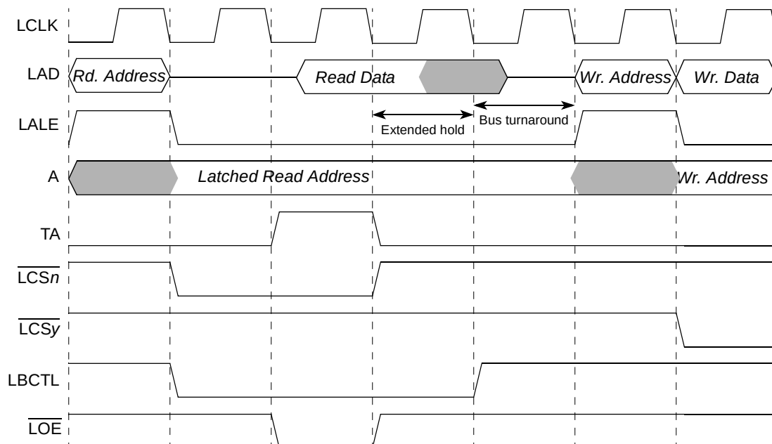
Figure 12-43. GPCM Read Followed by Write (TRLX = 0, EHTR = 1, One-Cycle Extended Hold Time on Reads)
