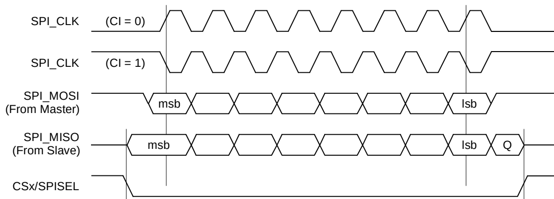
Figure 19-21. eSPI Transfer Format with SPMODEx[CPx] = 0
