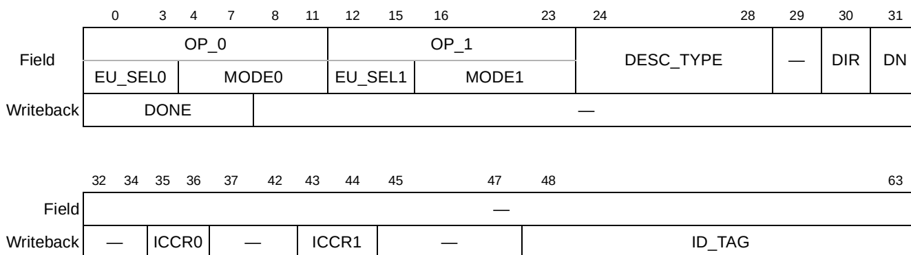
Figure 20-3. Header Dword
