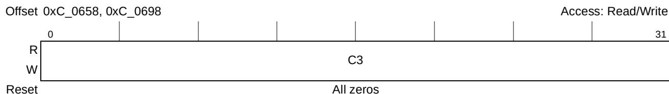
Figure 15-37. Port m Packet Error Capture Command and Status Register 3 ( PmPECCSR3 )
