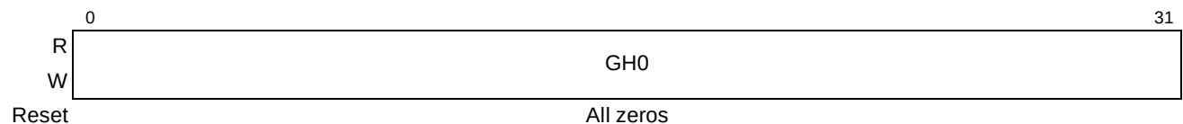
Figure 16-30. PCI Express Error Capture Register 0 (PEX_ERR_CAP_R0) External Source, Inbound Transaction
