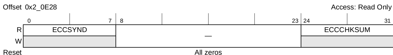
Figure 6-19. L2 Error Syndrome Register (L2CAPTECC)
