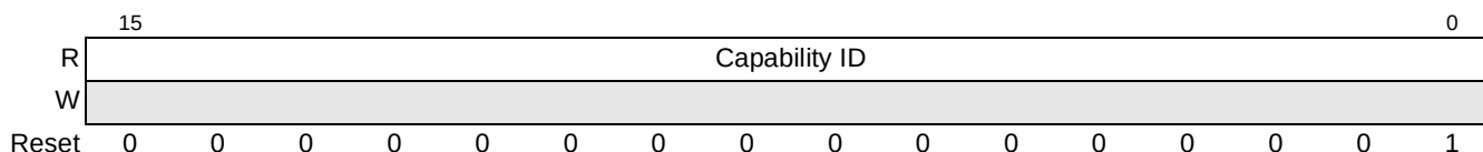
Figure 16-104. PCI Express Advanced Error Reporting Capability ID Register
