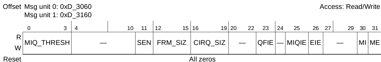
Figure 15-78. Inbound Message n Mode Registers (IMnMR)
