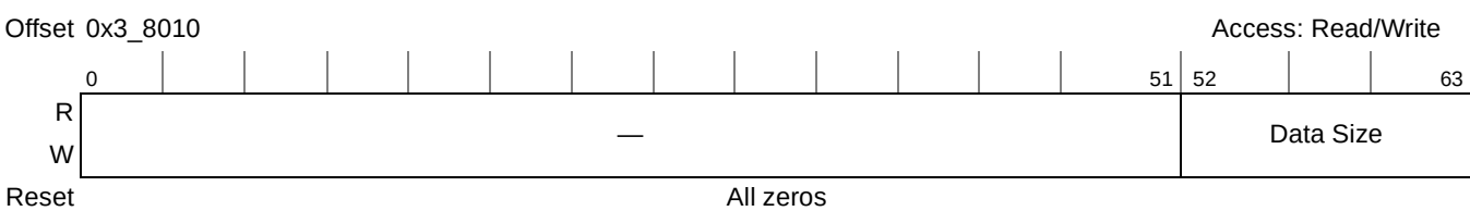
Figure 20-34. AFEU Context/Data Size Register
