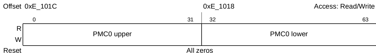
Figure 23-7. Performance Monitor Counter Register 0 (PMC0)
