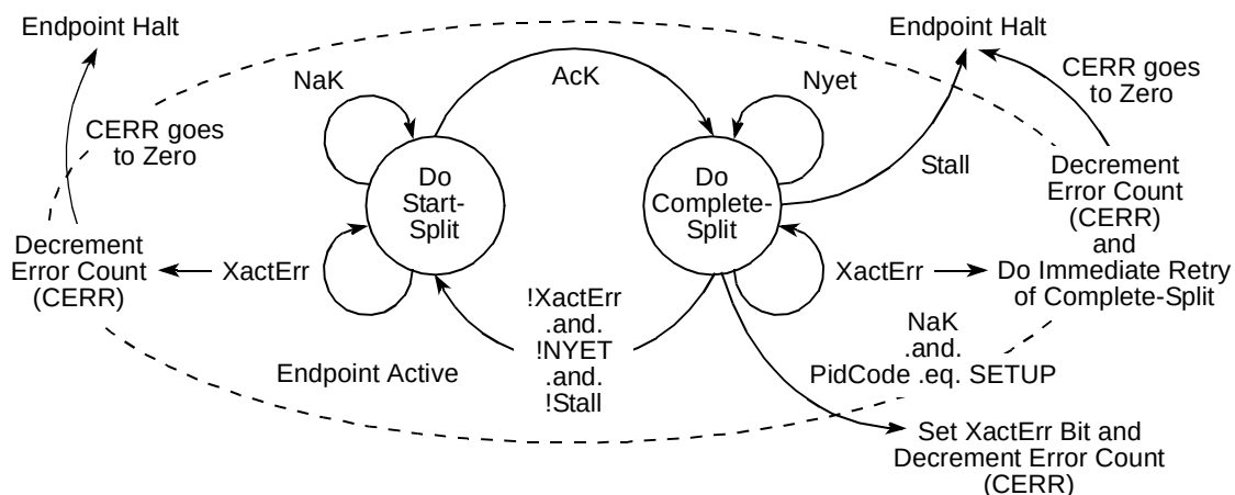
Figure 18-52. Host Controller Asynchronous Schedule Split-Transaction State Machine
