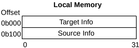
Figure 15-105. Doorbell Entry Format
