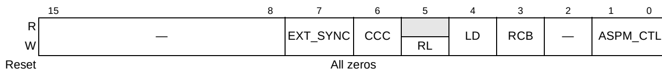
Figure 16-91. PCI Express Link Control Register
