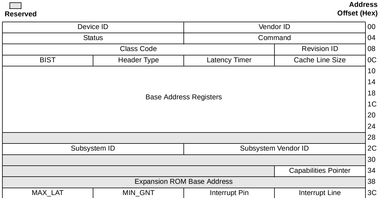
Figure 16-39. PCI Express PCI-Compatible Configuration Header—Type 0
