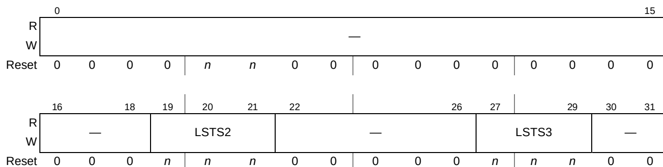
Figure 22-26. SRDS Control Register 4(SRDSCR4)
