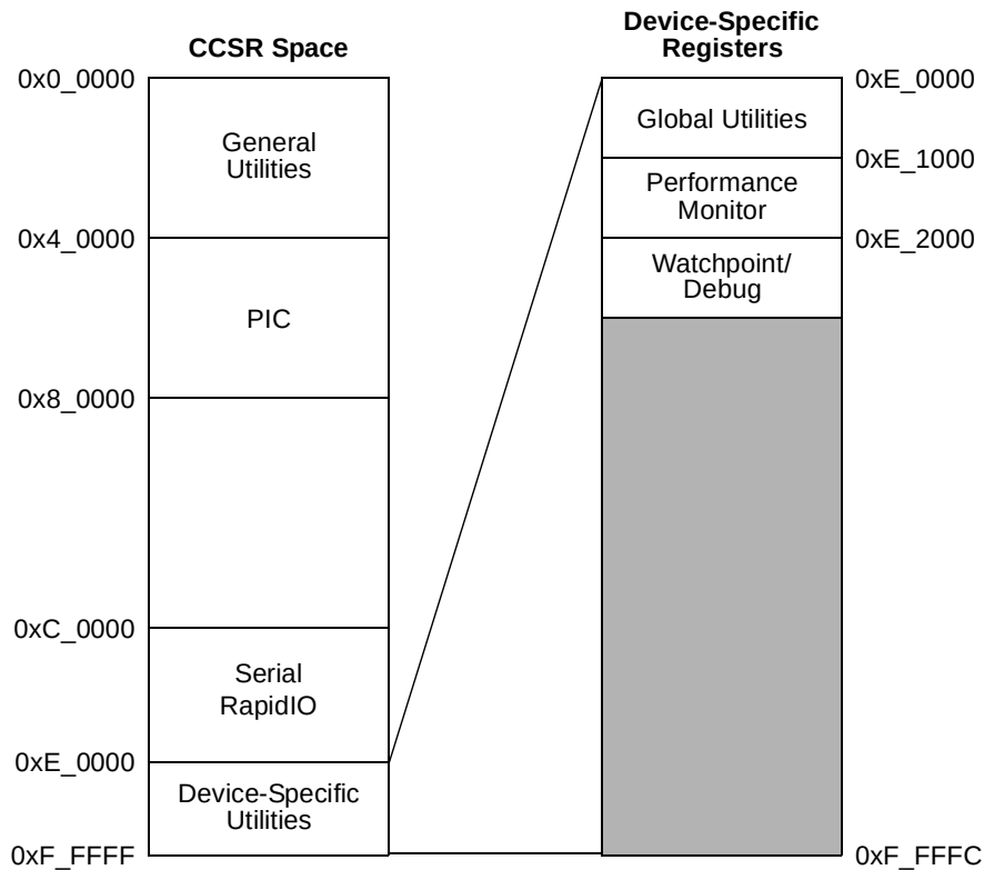
Figure 2-6. Device-Specific Register Map within CCSR Space
