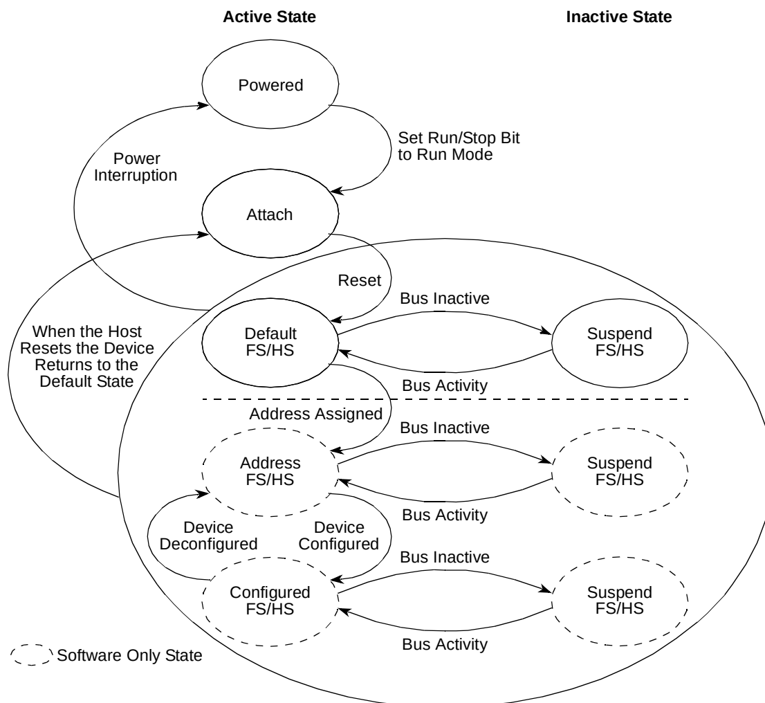
Figure 18-63. USB 2.0 Device States
