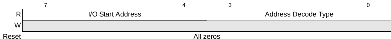
Figure 16-65. PCI Express I/O Base Register
