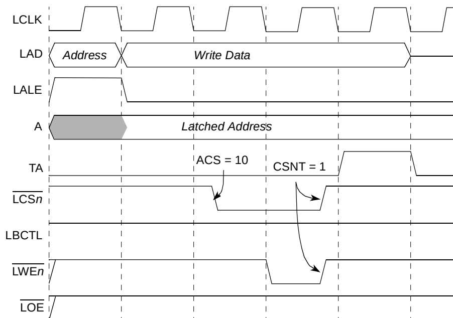
Figure 12-40. GPCM Relaxed Timing Write (XACS = 0, ACS = 10, SCY = 0, CSNT = 1, TRLX = 1)
