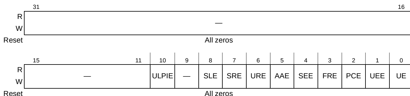
Figure 18-11. USB Interrupt Enable (USBINTR)
