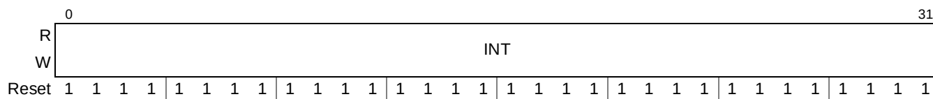
Figure 9-26. Performance Monitor Mask Registers 1 (PMnMR1)
