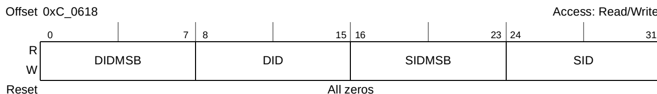
Figure 15-29. Logical/Transport Layer Device ID Capture Command and Status Register (LTLDIDCCSR)
