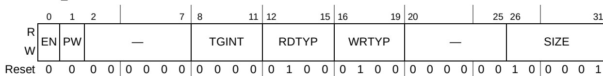
Figure 15-62. Port m RapidIO Inbound Window Attributes Register 1–4
