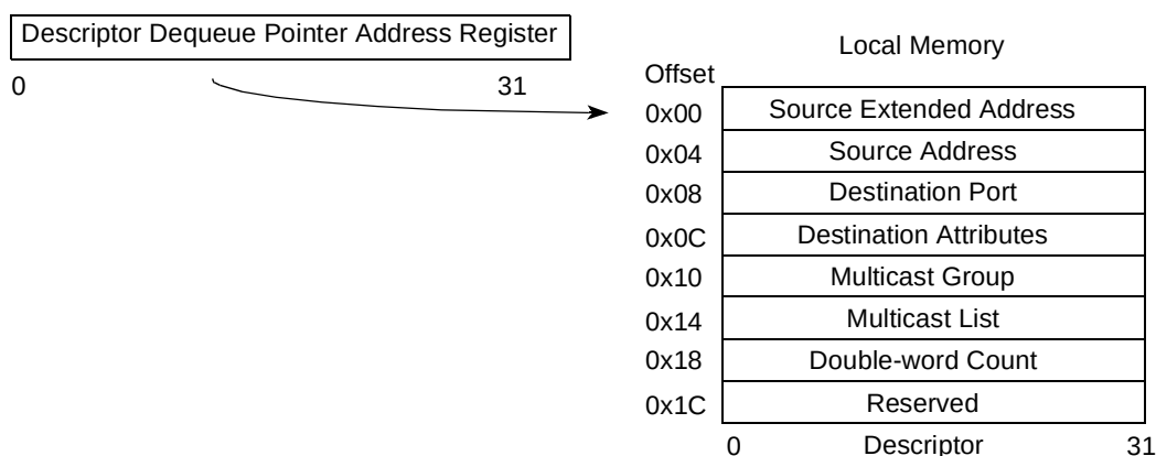
Figure 15-102. Descriptor Dequeue Pointer and Descriptor
