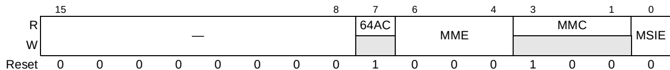
Figure 16-99. PCI Express MSI Message Control Register
