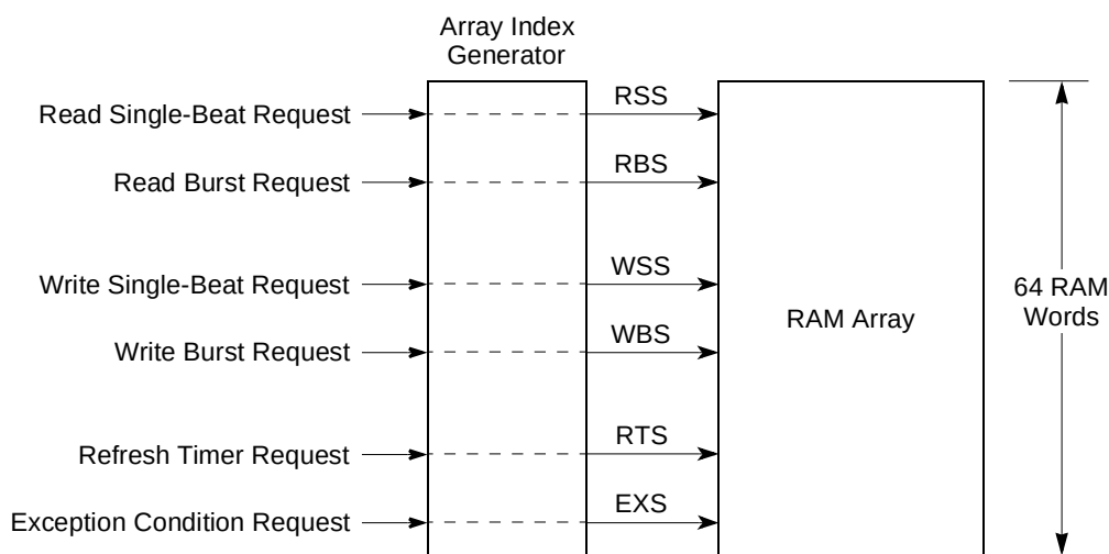
Figure 12-62. RAM Array Indexing
