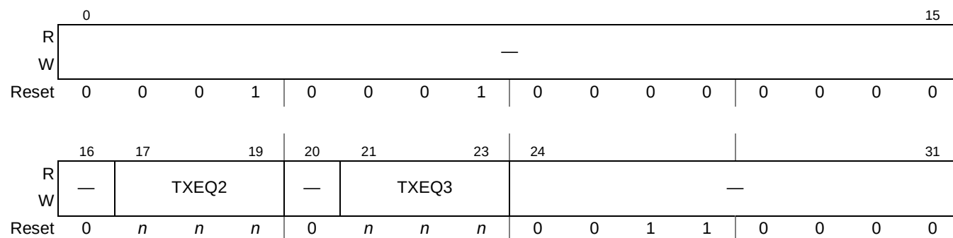
Figure 22-24. SRDS Control Register 1 (SRDSCR1)
