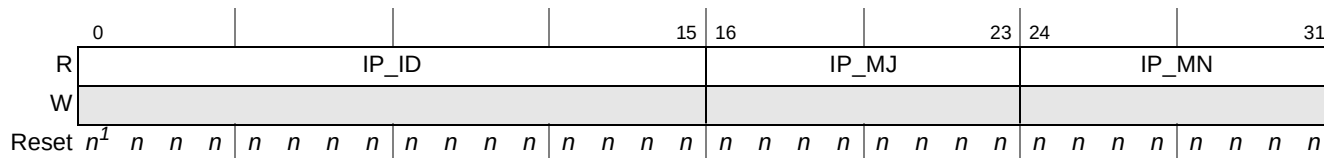
Figure 8-32. DDR IP Block Revision 1 (DDR_IP_REV1)
