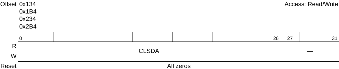
Figure 13-17. Current List Descriptor Address Registers (CLSDARn)
