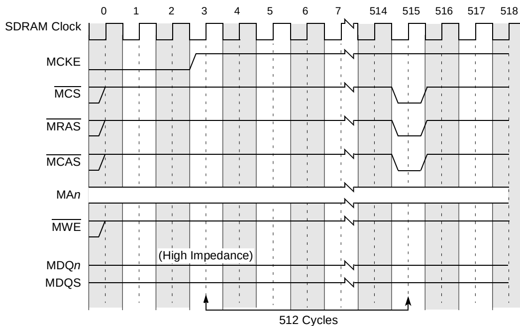
Figure 8-60. DDR SDRAM Self-Refresh Exit Timing (DDR3)
