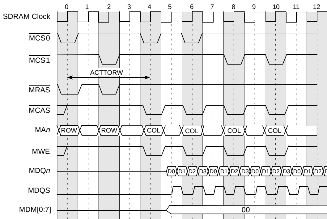
Figure 8-53. DDR SDRAM 4-Beat Burst Write Timing—ACTTORW = 4
