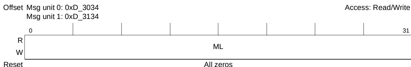
Figure 15-77. Outbound Message n Multicast List Registers (OMnMLR)
