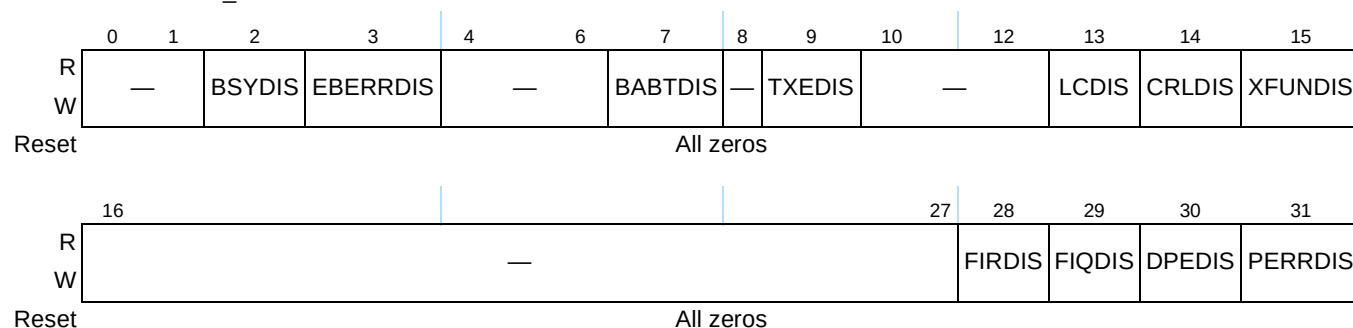
Figure 14-6. EDIS Register Definition
