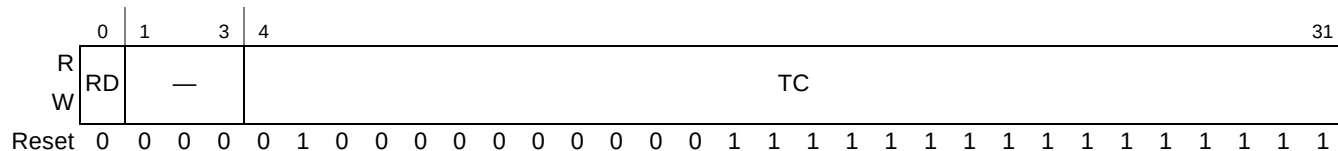
Figure 16-5. PCI Express Configuration Retry Timeout Register (PEX_CONF_RTY_TOR)
