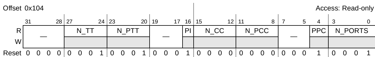
Figure 18-5. Host Controller Structural Parameters (HCSPARAMS)
