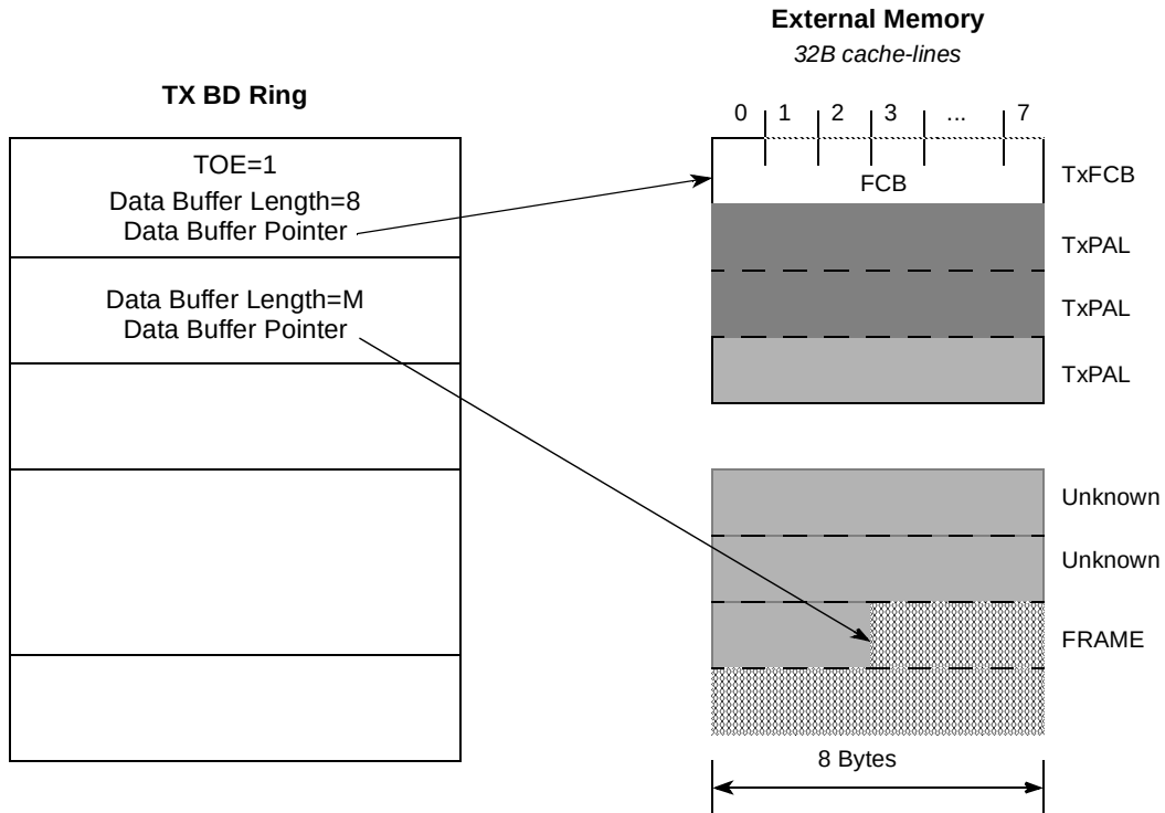
Figure 14-151. Buffer Format for Transmit Time-Stamp Insertion
