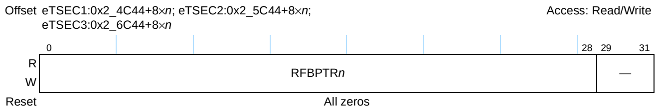
Figure 14-108. RFBPTR0–RFBPTR7 Register Definition
