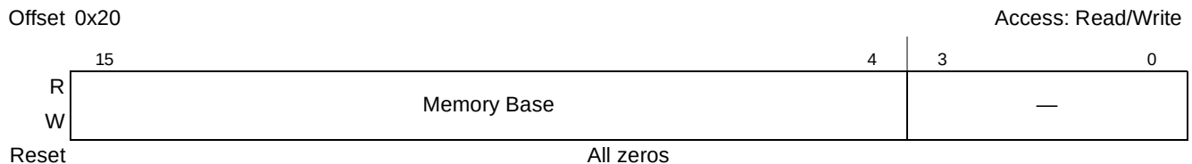
Figure 16-68. PCI Express Memory Base Register
