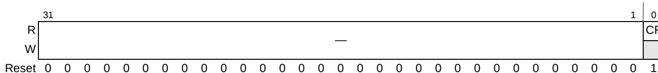
Figure 18-20. Configure Flag Register (CONFIGFLAG)
