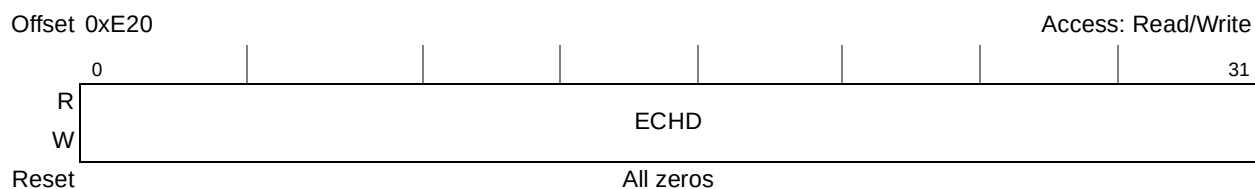
Figure 8-37. Memory Data Path Read Capture High Register (CAPTURE_DATA_HI)
