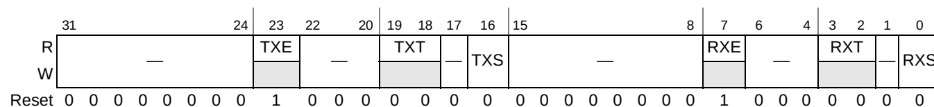
Figure 18-28. Endpoint Control 0 (ENDPTCTRL0)
