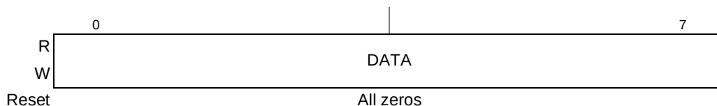
Figure 10-6. I 2 C Data Register (I2CDR)
