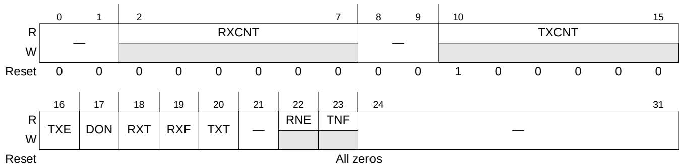
Figure 19-4. eSPI Event Register (SPIE)
