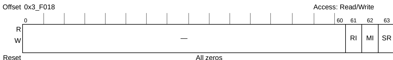
Figure 20-43. CRCU Reset Control Register
