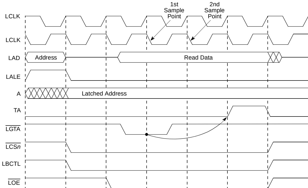
Figure 12-45. External Termination of GPCM Access (PLL Bypass Mode)
