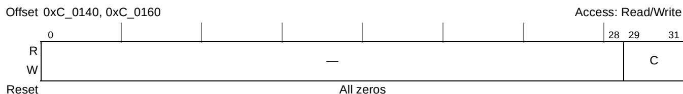
Figure 15-20. Port m Link Maintenance Request Command and Status Register (PmLMREQCSR)
