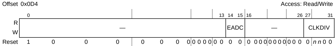
Figure 12-20. Clock Ratio Register (LCRR)
