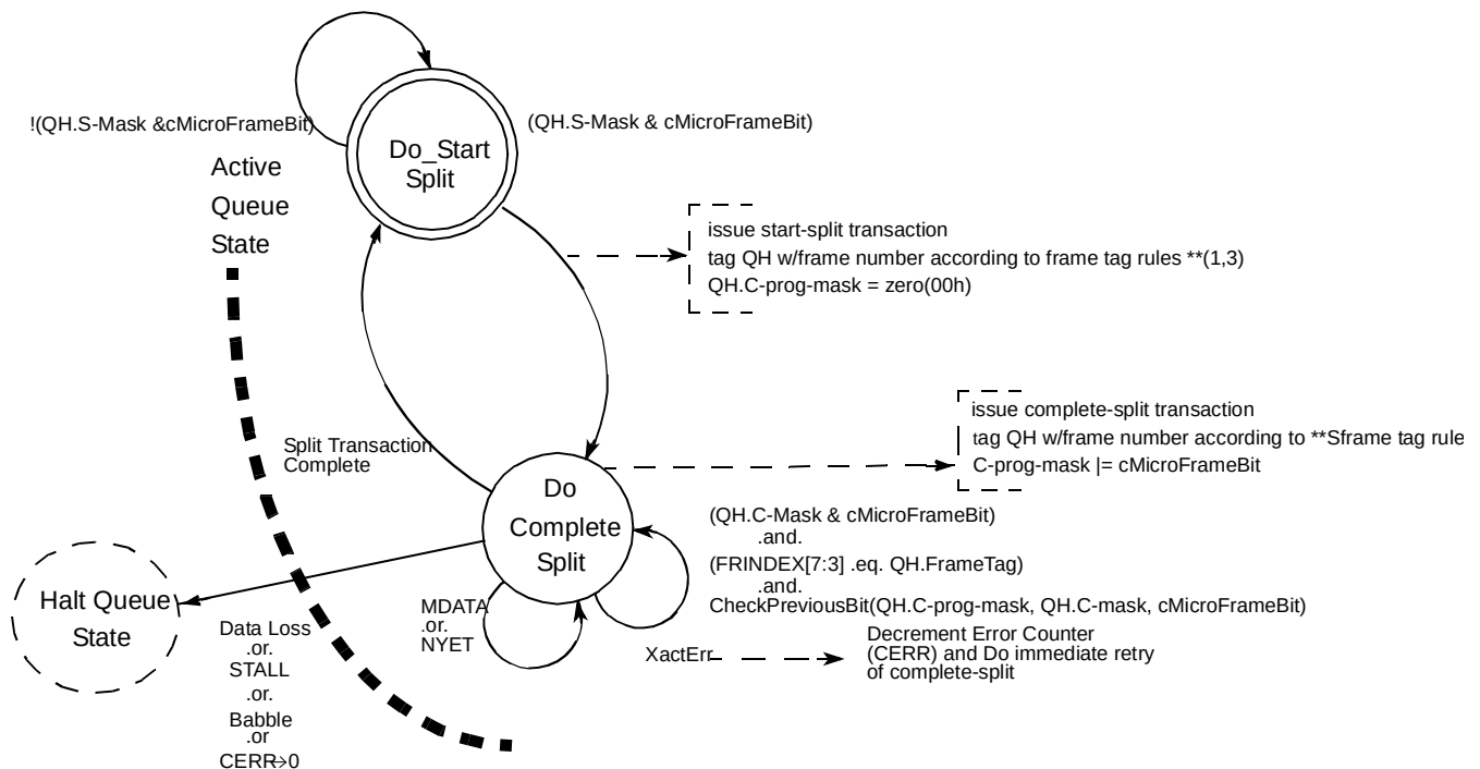
Figure 18-56. Split Transaction State Machine for Interrupt
