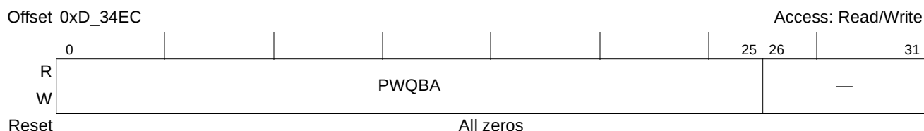
Figure 15-100. Inbound Port-Write Queue Base Address Register (IPWQBAR)
