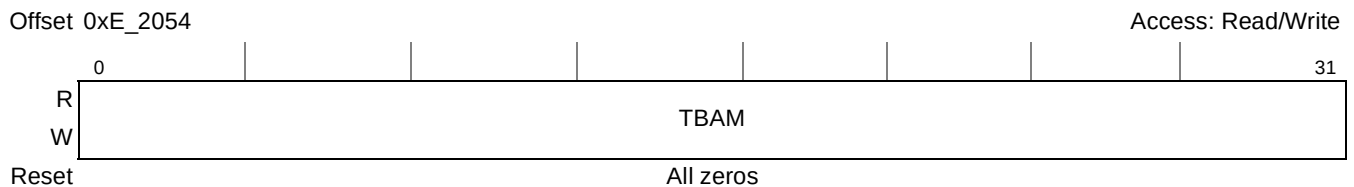
Figure 24-11. Trace Buffer Address Mask Register (TBAMR)
