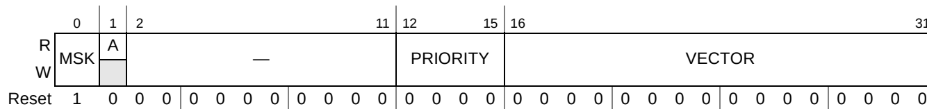
Figure 9-9. Interprocessor Interrupt Vector/Priority Register (IPIVPR n )
