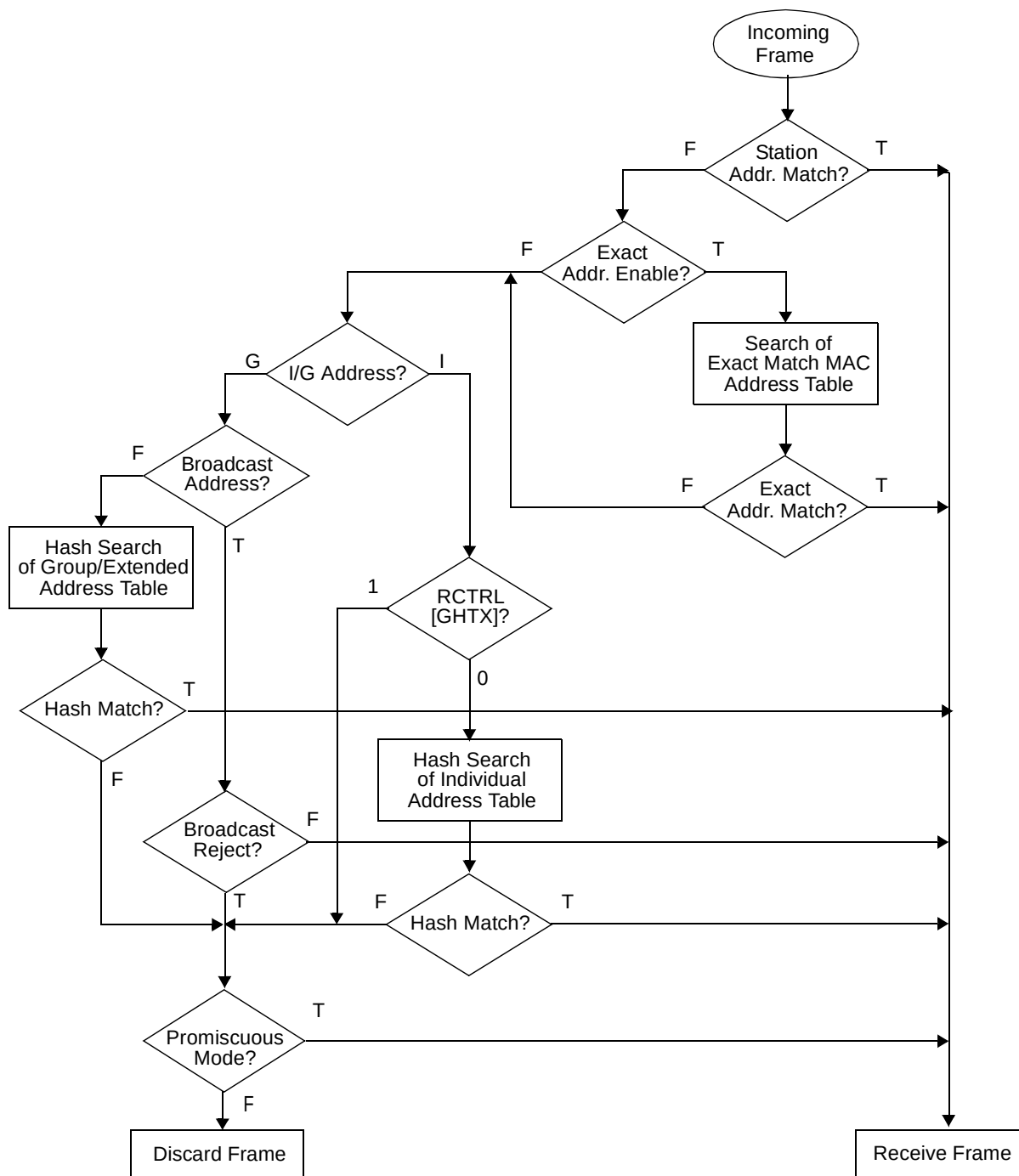
Figure 14-141. Ethernet Address Recognition Flowchart
