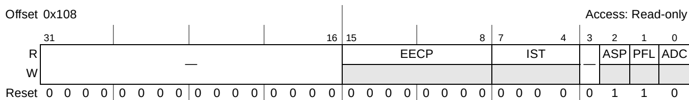
Figure 18-6. Host Control Capability Parameters (HCCPARAMS)
