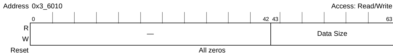
Figure 20-83. MDEU Data Size Register
