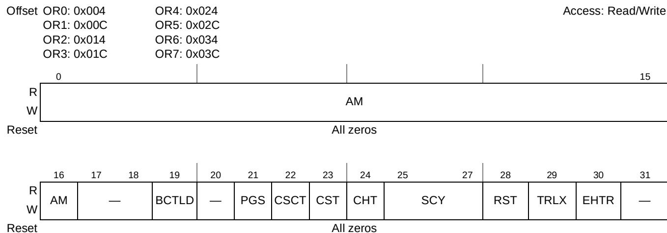
Figure 12-4. Option Registers (OR n ) in FCM Mode
