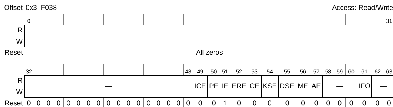
Figure 20-47. CRCU Interrupt Mask Register
