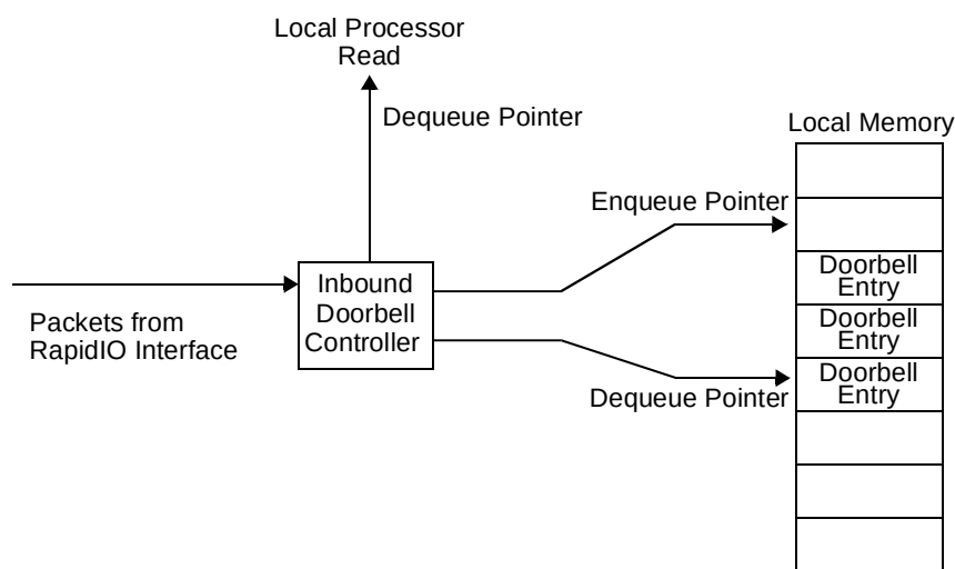
Figure 15-104. Inbound Doorbell Queue and Pointer Structure
