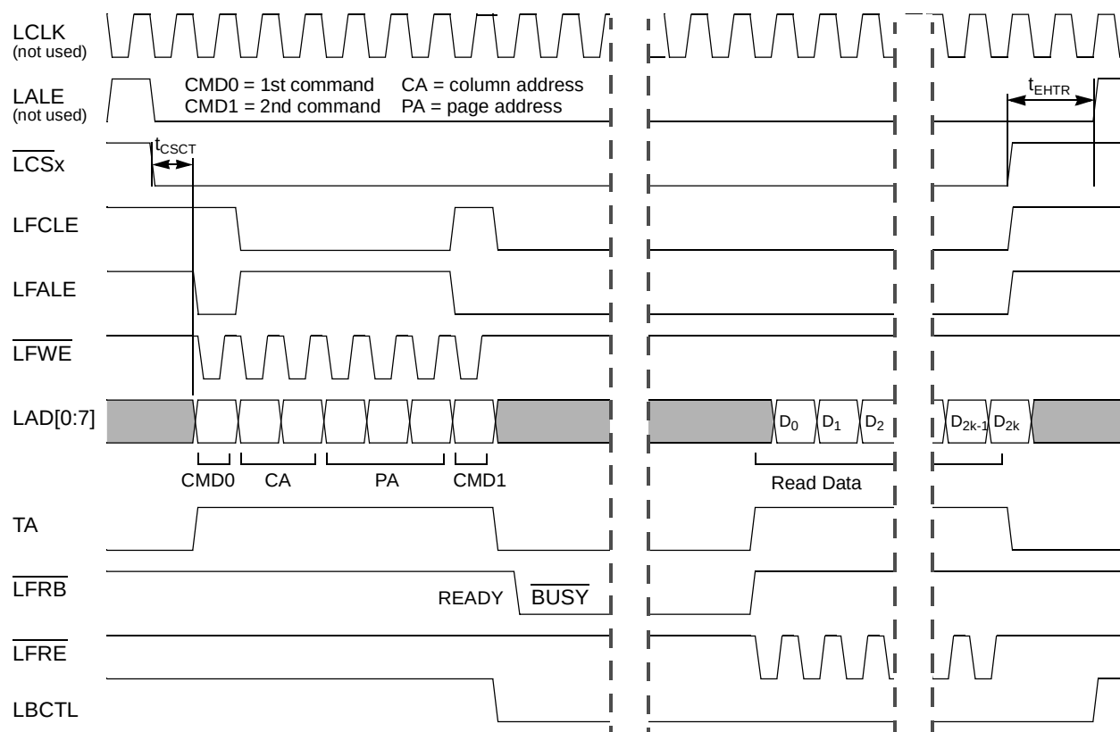
Figure 12-47. FCM Basic Page Read Timing (PGS = 1, CSCT = 0, CST = 0, CHT = 1, RST = 1, SCY = 0, TRLX = 0, EHTR = 1)
