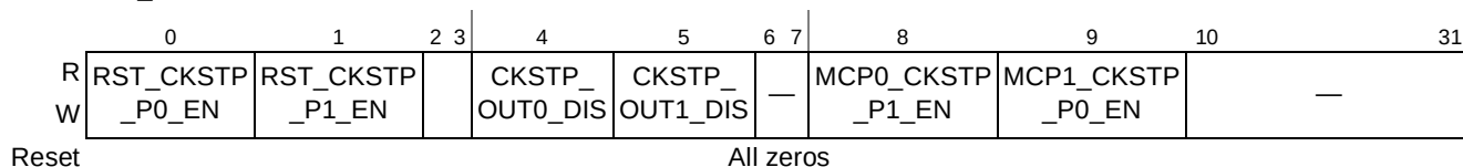
Figure 22-13. Exception Reset Control Register (ECTRSTCR)
