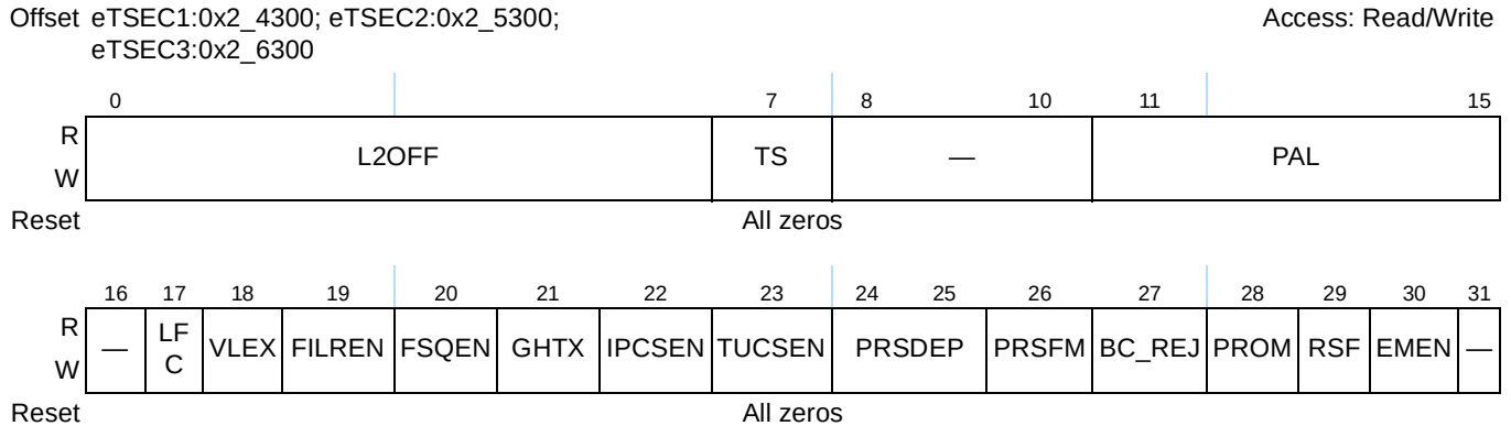
Figure 14-24. RCTRL Register Definition
