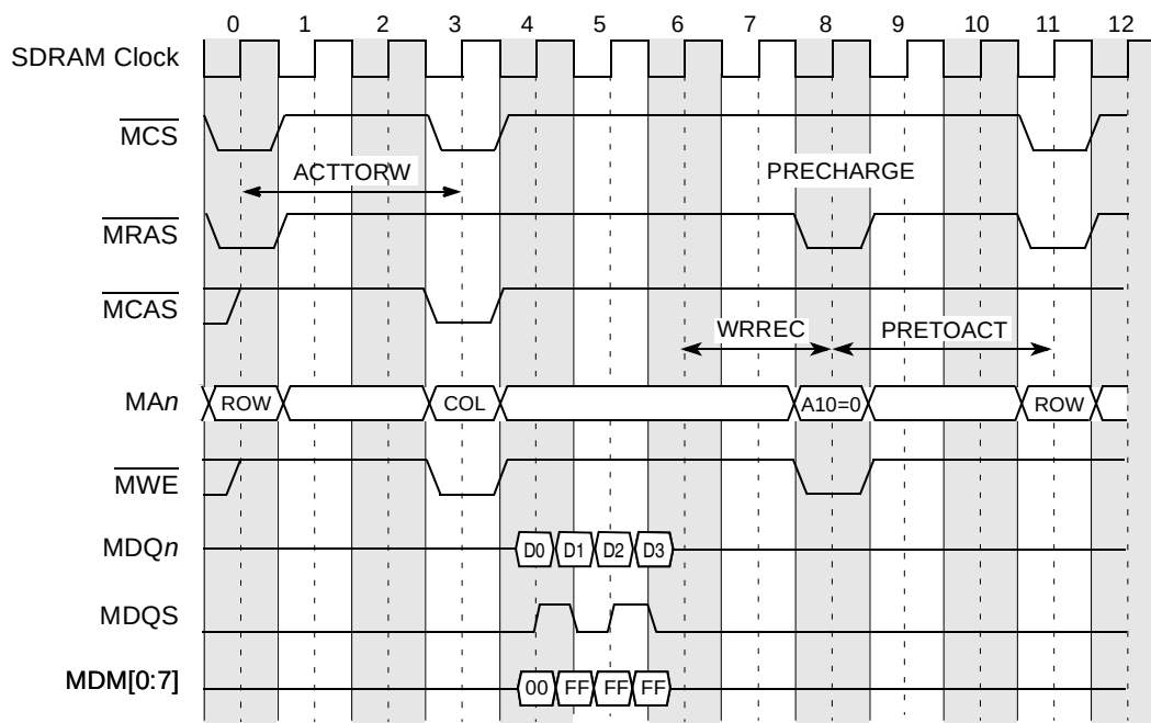
Figure 8-52. DDR SDRAM Single-Beat (Double Word) Write Timing—ACTTORW = 3
