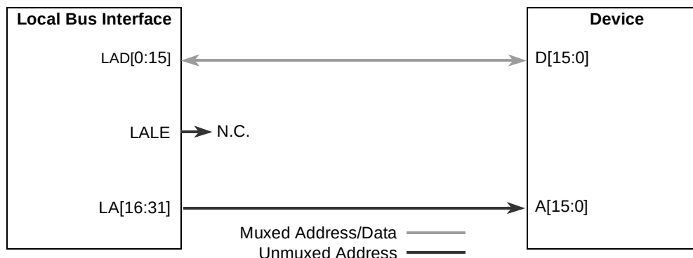
Figure 12-71. Non-Multiplexed Address and Data Buses
