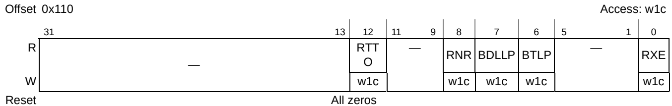
Figure 16-108. PCI Express Correctable Error Status Register
