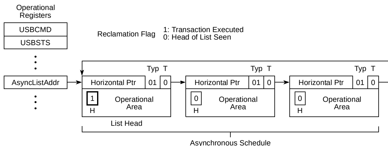
Figure 18-50. Asynchronous Schedule List with Annotation to Mark Head of List
