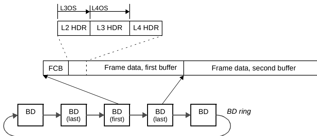
Figure 14-143. Location of Frame Control Blocks for TOE Parameters
