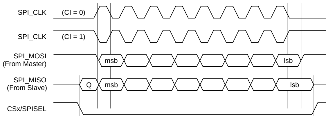
Figure 19-22. eSPI Transfer Format with SPMODEx[CPx] = 1
