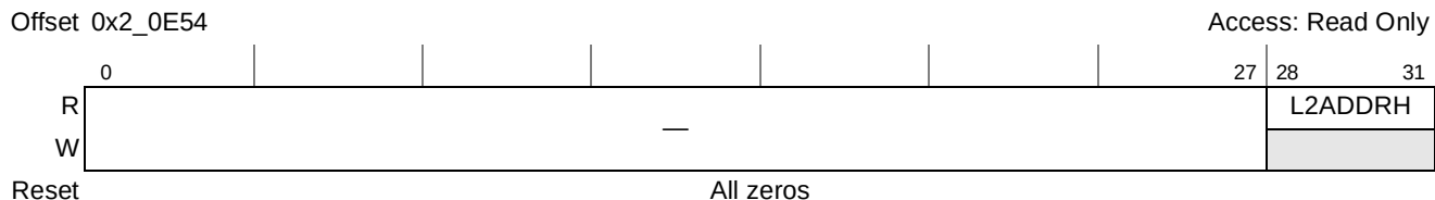
Figure 6-25. L2 Error Address Capture Register (L2ERRADDRH)
