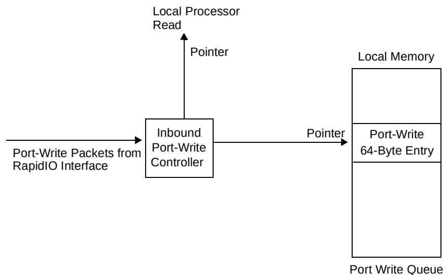
Figure 15-106. Inbound Port-Write Structure
