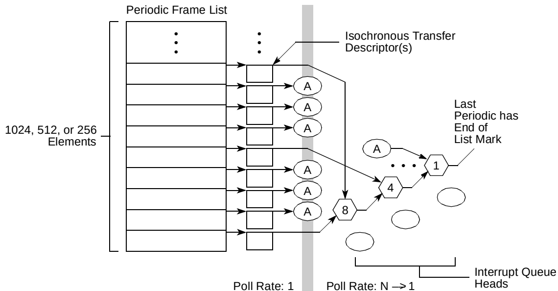
Figure 18-47. Example Periodic Schedule
