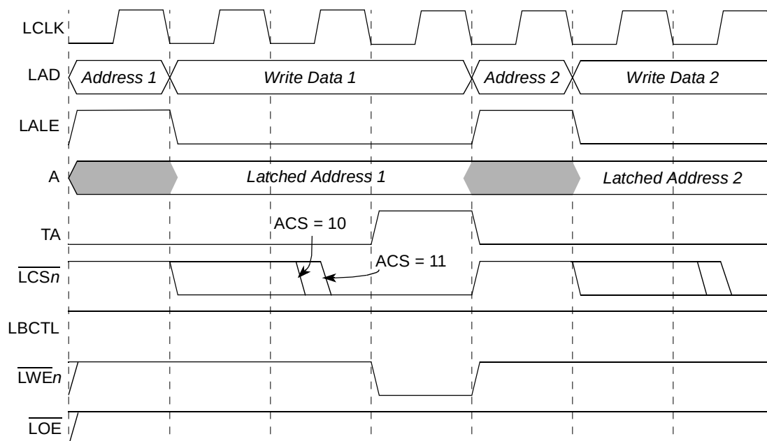
Figure 12-39. GPCM Relaxed Timing Back-to-Back Writes with PLL Bypass (XACS = 0, ACS = 1x, SCY = 0, CSNT = 0, TRLX = 1)
