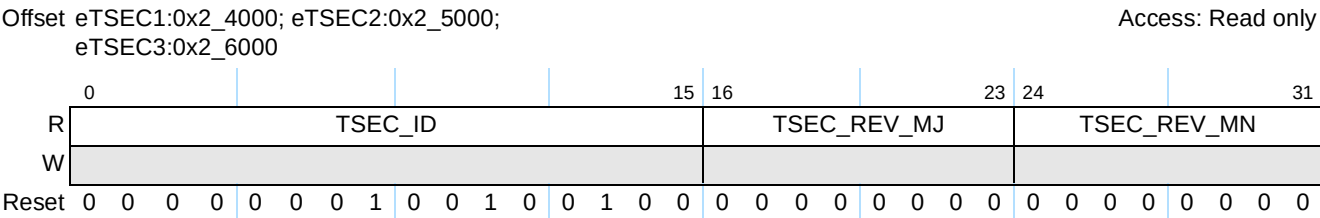
Figure 14-2. TSEC_ID Register
