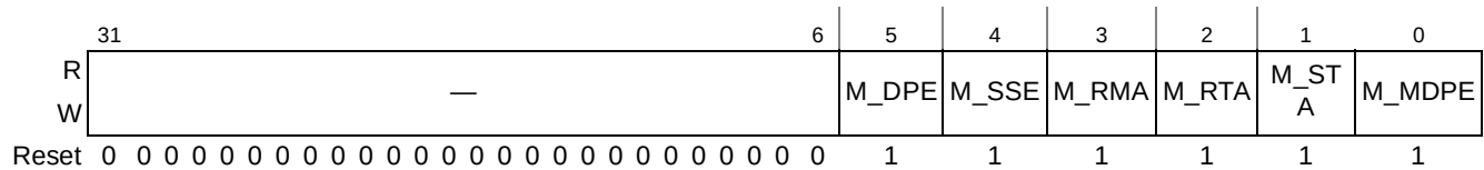
Figure 16-124. PCI Express PCI Interrupt Mask Register (PEX_SS_INTR_MASK)
