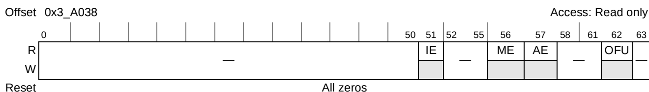
Figure 20-105. RNGU Interrupt Mask Register
