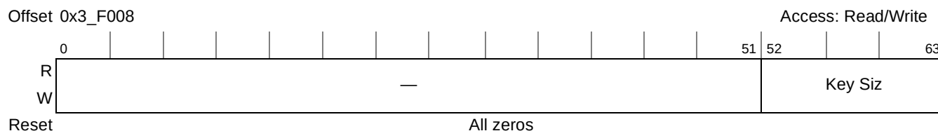
Figure 20-41. CRCU Key Size Register
