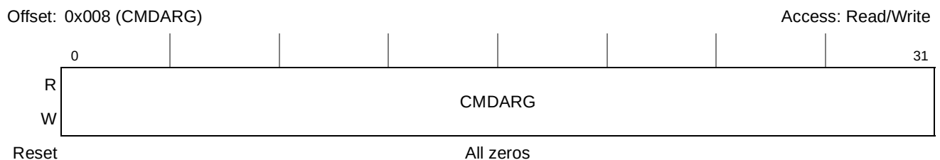
Figure 17-5. Command Argument Register (CMDARG)
