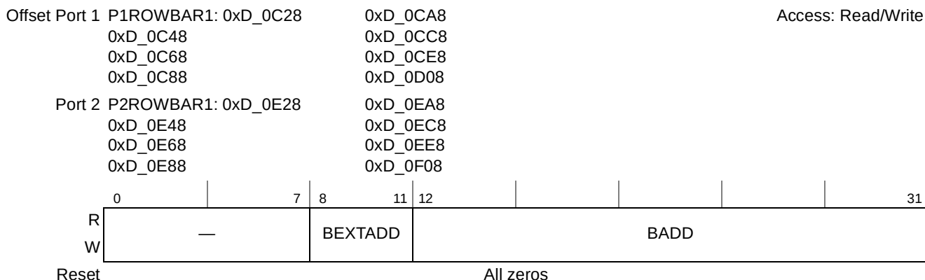
Figure 15-57. Port m RapidIO Outbound Window Base Address Registers 1–8
