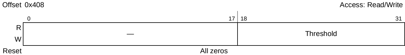
Figure 18-31. Age Count Threshold (AGE_CNT_THRESH)
