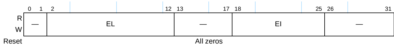
Figure 14-106. ATTRELI Register Definition
