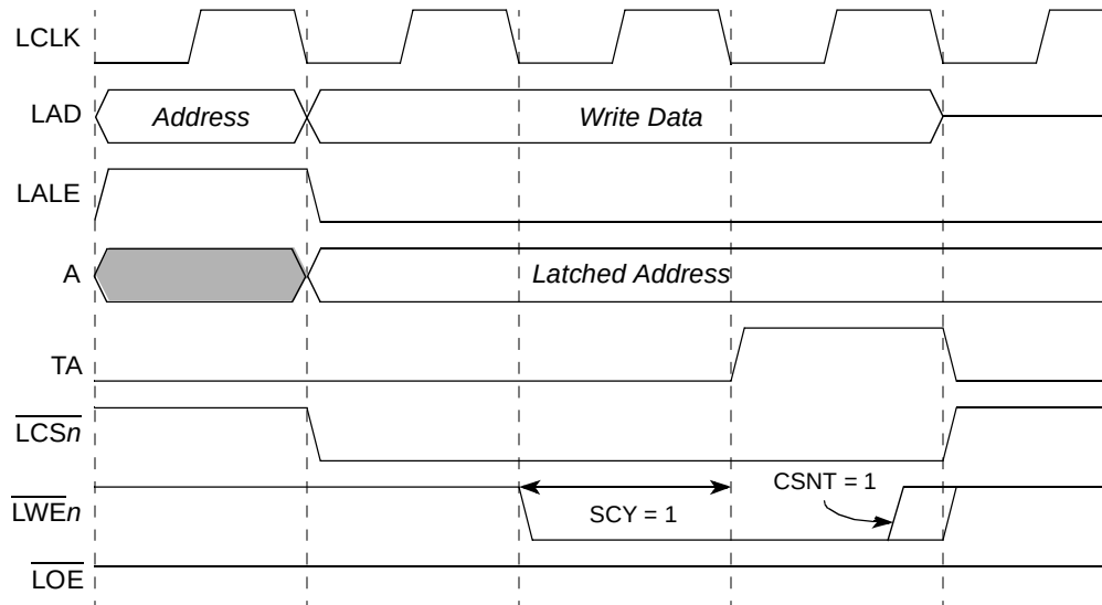
Figure 12-37. GPCM Basic Write Timing (XACS = 0, ACS = 00, CSNT = 1, SCY = 1, TRLX = 0)
