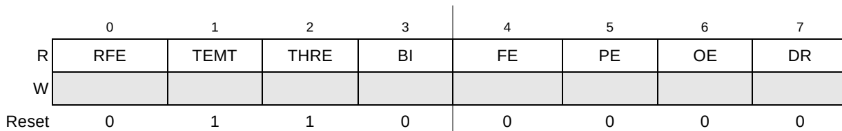
Figure 11-12. Line Status Register (ULSR)
