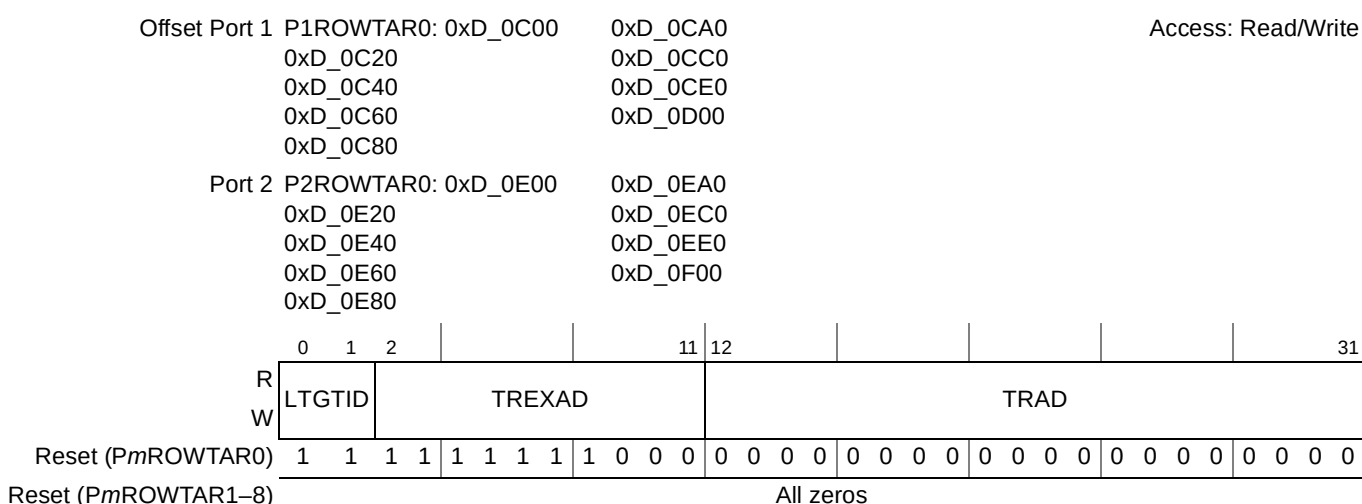
Figure 15-55. Port m RapidIO Outbound Window Translation Address Registers 0–8 (PmROWTARn)
