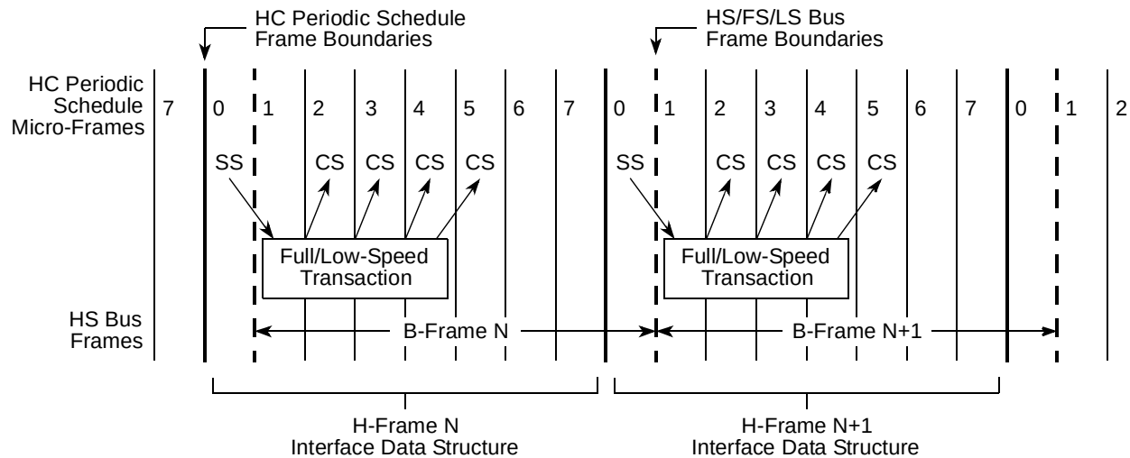
Figure 18-46. Relationship of Periodic Schedule Frame Boundaries to Bus Frame Boundaries
