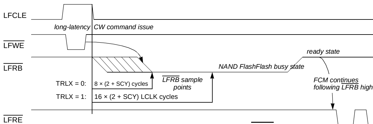
Figure 12-57. FCM Delay Prior to Sampling \overline{LFRB} State
