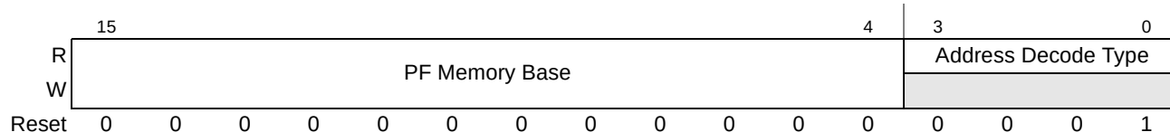
Figure 16-70. PCI Express Prefetchable Memory Base Register
