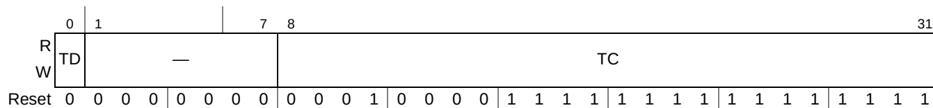
Figure 16-4. PCI Express Outbound Completion Timeout Register (PEX_OTB_CPL_TOR)
