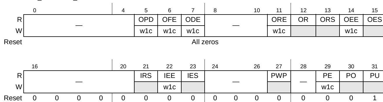
Figure 15-23. Port m Error and Status Command and Status Register (PmESCSR)
