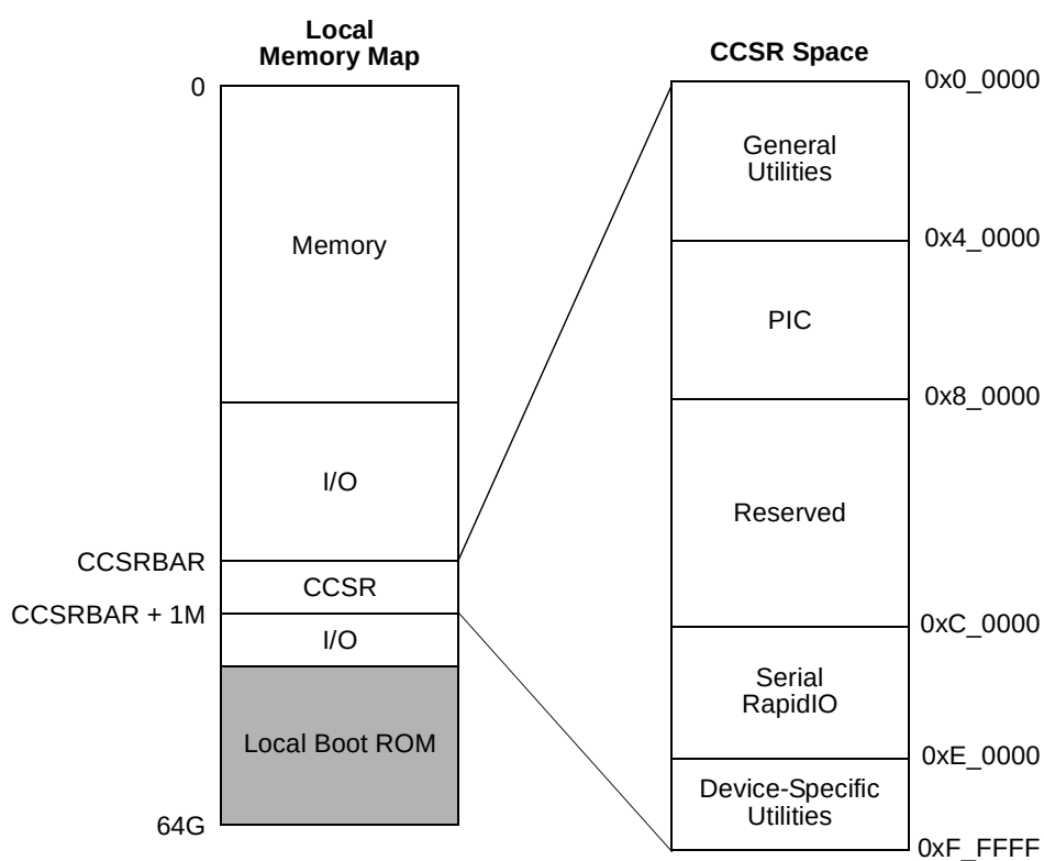
Figure 2-1. CCSR Space
