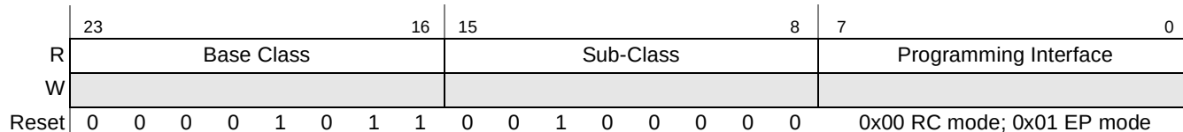
Figure 16-45. PCI Express Class Code Register
