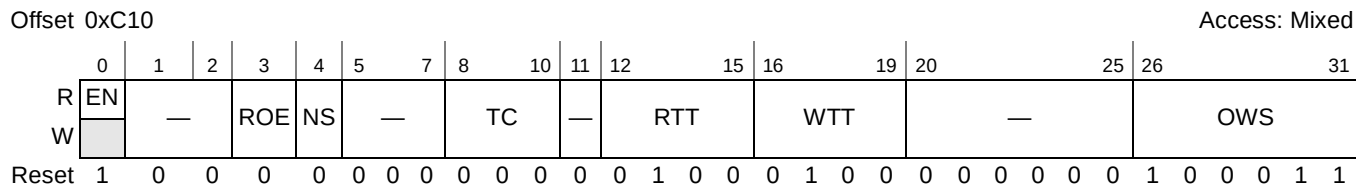
Figure 16-17. PCI Express Outbound Window Attributes Register0 (PEXOWAR0)
