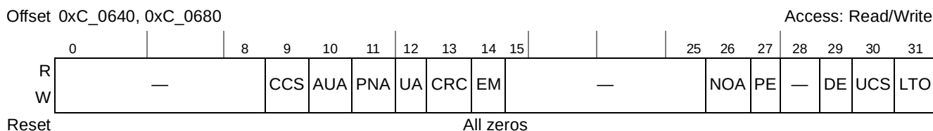
Figure 15-31. Port m Error Detect Command and Status Register (PmEDCSR)
