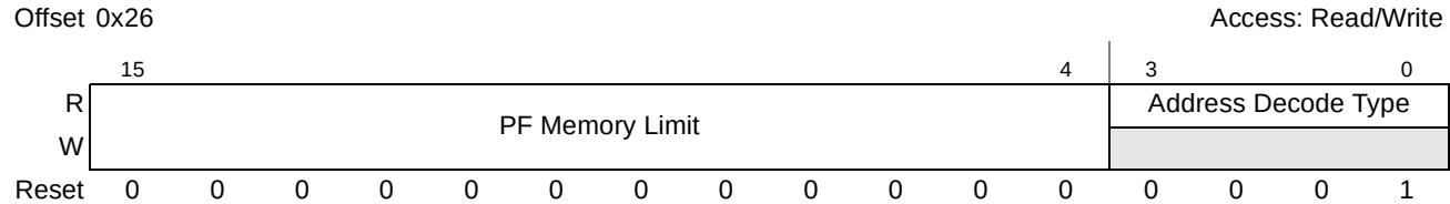
Figure 16-71. PCI Express Prefetchable Memory Limit Register
