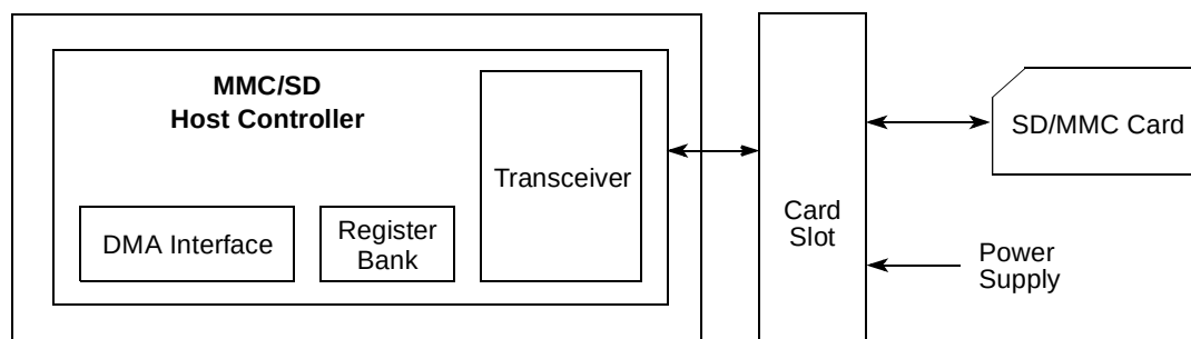
Figure 17-1. System Connection of the eSDHC
