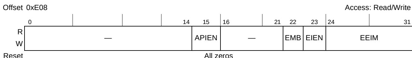
Figure 8-36. Memory Data Path Error Injection Mask ECC Register (ERR_INJECT)
