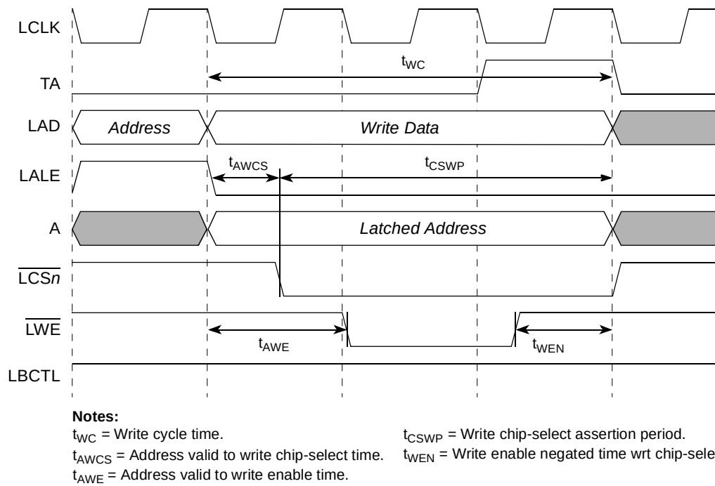
Figure 12-36. GPCM General Write Timing Parameters
