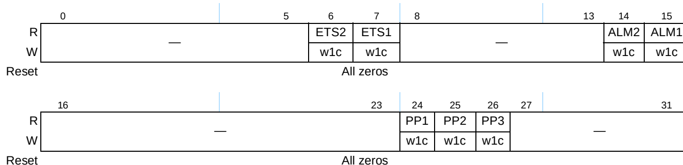
Figure 14-110. TMR_TEVENT Register Definition
