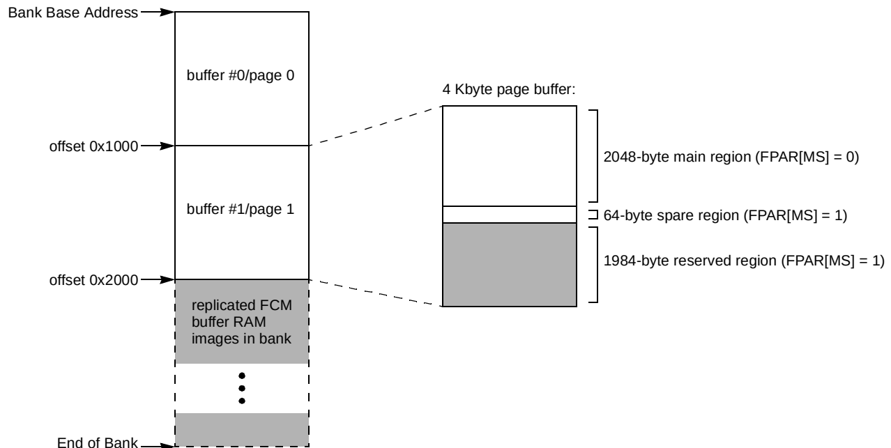
Figure 12-49. FCM Buffer RAM Memory Map for Large-Page (2-Kbyte Page) NAND Flash Devices
