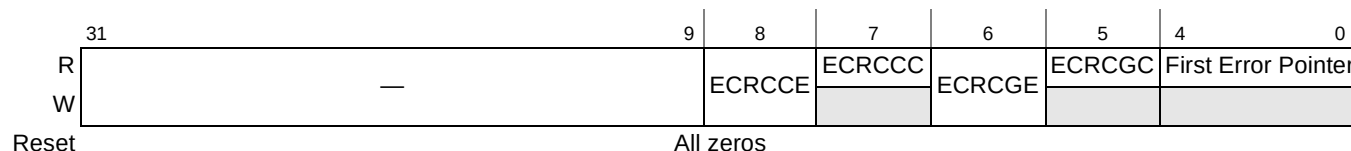
Figure 16-110. PCI Express Advanced Error Capabilities and Control Register
