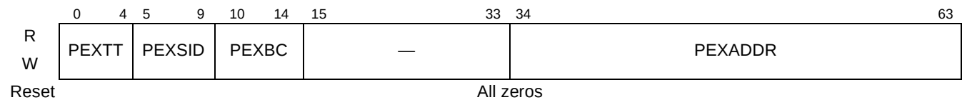
Figure 24-21. PCI Express Trace Buffer Entry
