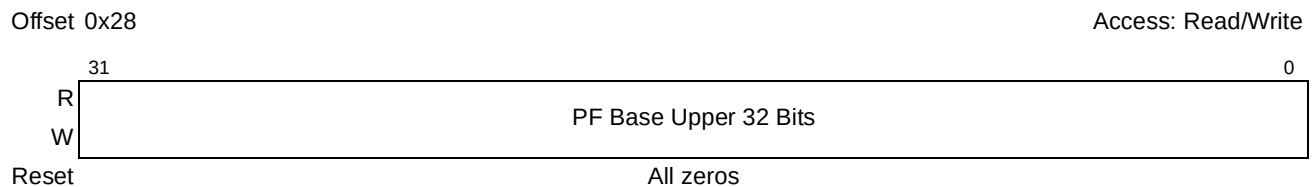
Figure 16-72. PCI Express Prefetchable Base Upper 32 Bits Register
