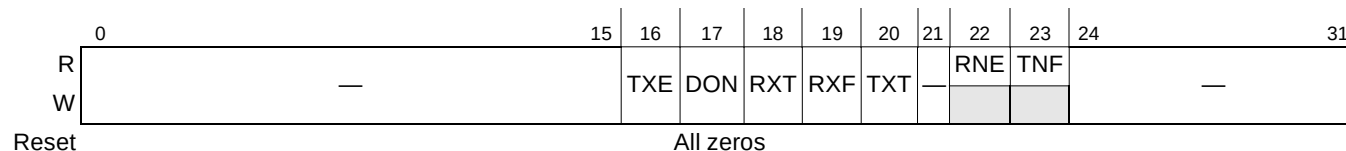
Figure 19-5. eSPI Mask Register (SPIM)
