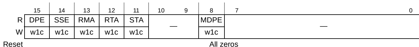
Figure 16-67. PCI Express Secondary Status Register
