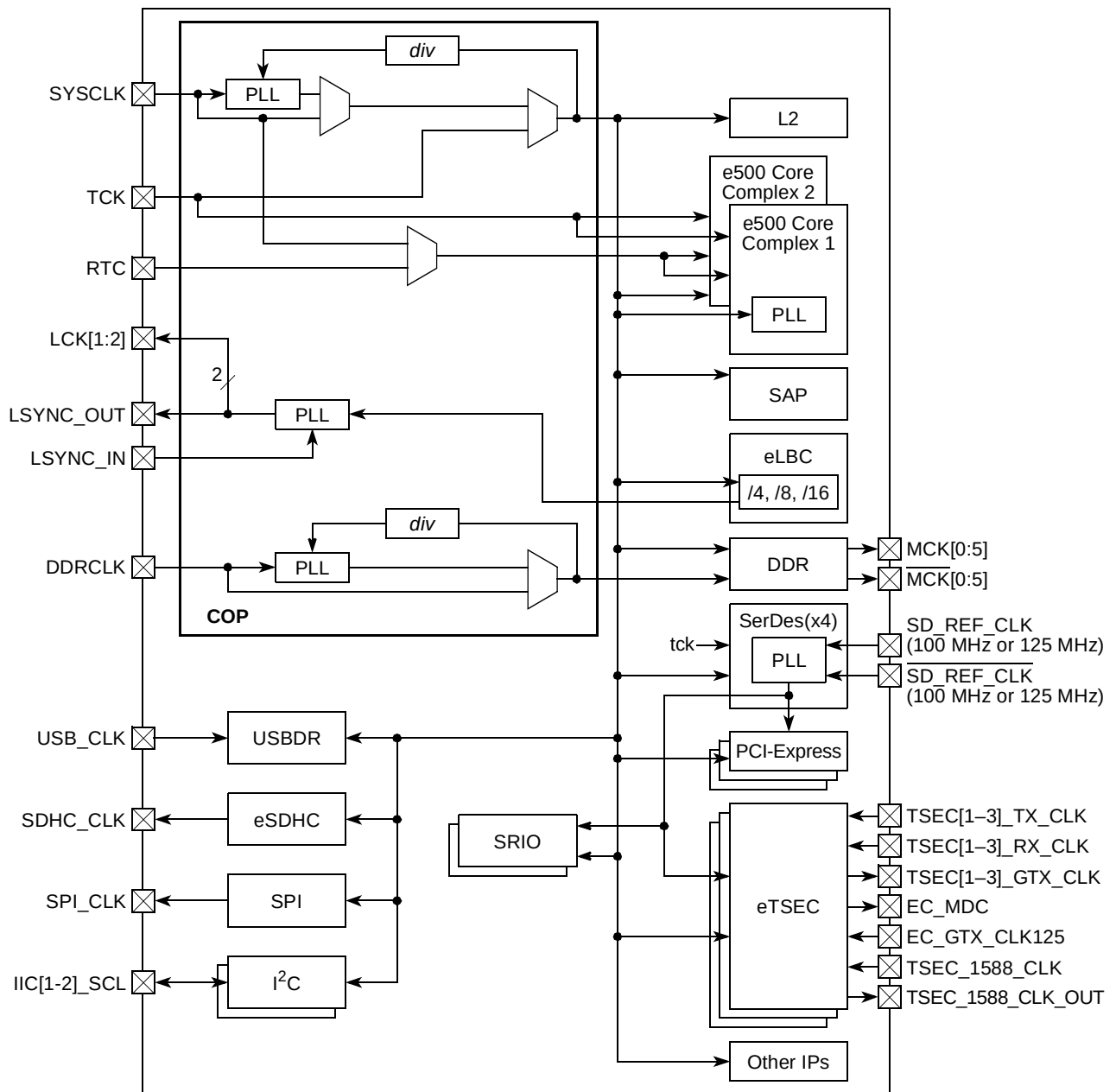
Figure 4-6. P2020 Clock Subsystem Block Diagram
