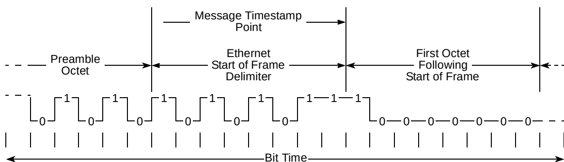
Figure 14-149. Ethernet Sampling Points for 1588
