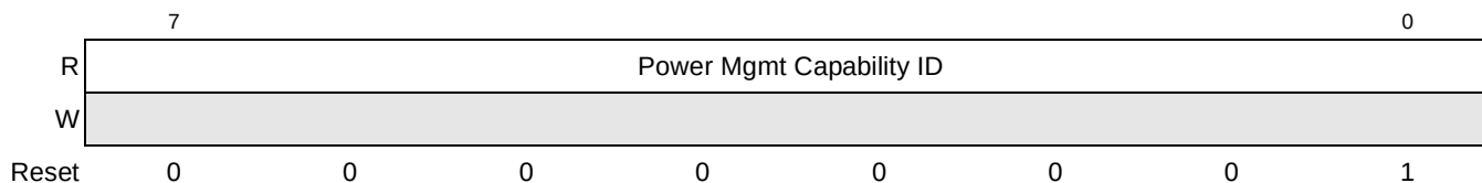
Figure 16-81. PCI Express Power Management Capability ID Register
