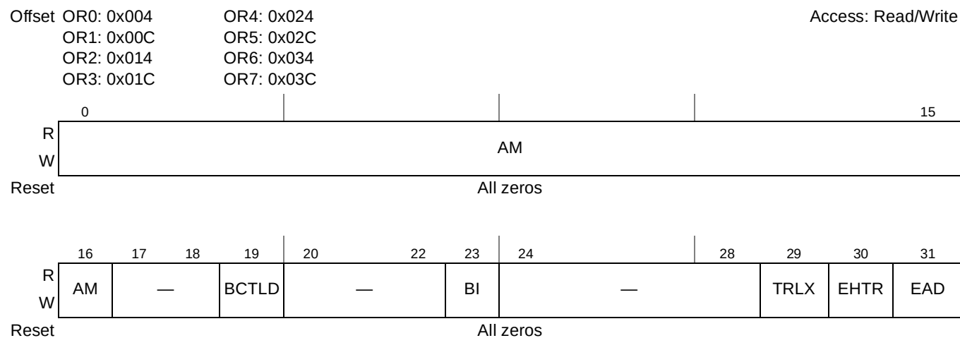
Figure 12-5. Option Registers (OR n ) in UPM Mode
