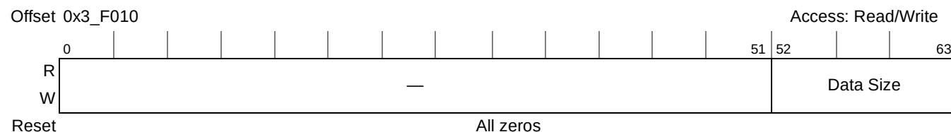
Figure 20-42. CRCU Data Size Register
