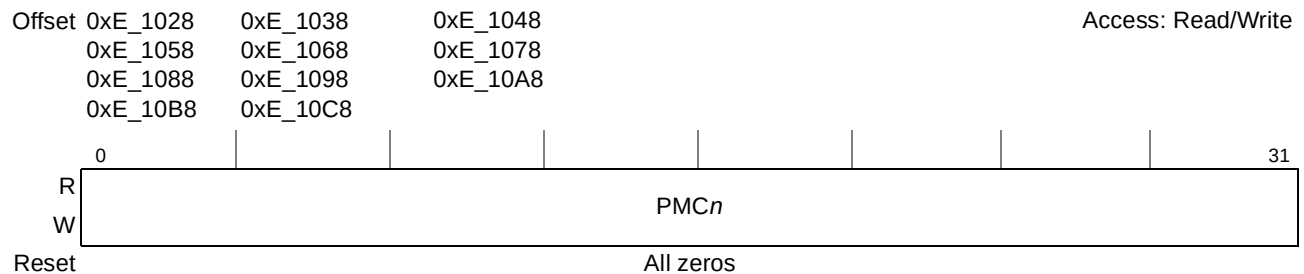
Figure 23-8. Performance Monitor Counter Register (PMC1–PMC11)
