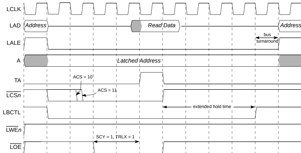
Figure 12-38. GPCM Relaxed Timing Back-to-Back Reads with PLL Bypass (XACS = 0, ACS = 1x, SCY = 1, CSNT = 0, TRLX = 1, EHTR = 0)
