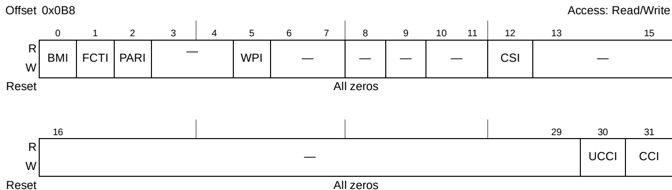
Figure 12-15. Transfer Error Interrupt Enable Register (LTEIR)
