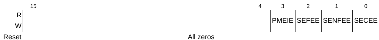
Figure 16-96. PCI Express Root Control Register
