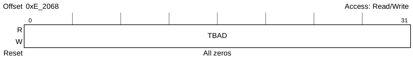
Figure 24-16. Trace Buffer Access Data Register (TBADR)
