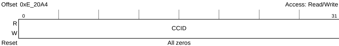
Figure 24-18. Current Context ID Register (CCIDR)
