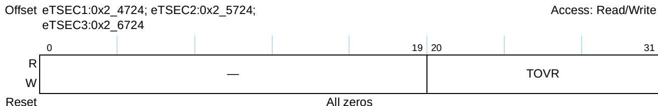
Figure 14-95. Transmit Oversized Frame Counter Register Definition
