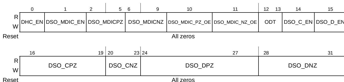
Figure 8-30. DDR Control Driver Register 1 (DDRCDDR_1)
