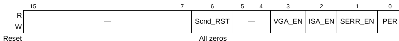
Figure 16-79. PCI Express Bridge Control Register
