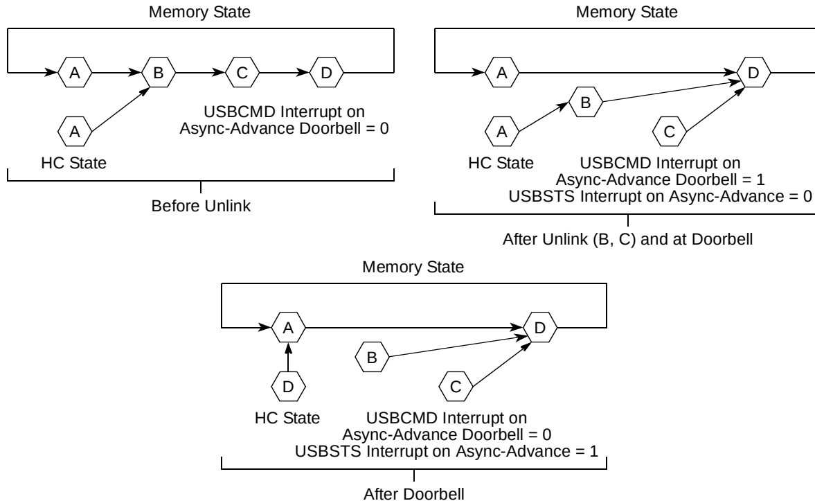
Figure 18-49. Generic Queue Head Unlink Scenario
