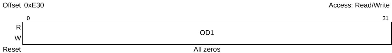
Figure 16-33. PCI Express Error Capture Register 2 (PEX_ERR_CAP_R2) Internal Source, Outbound Transaction
