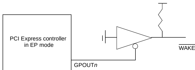
Figure 16-135. WAKE Generation Example
