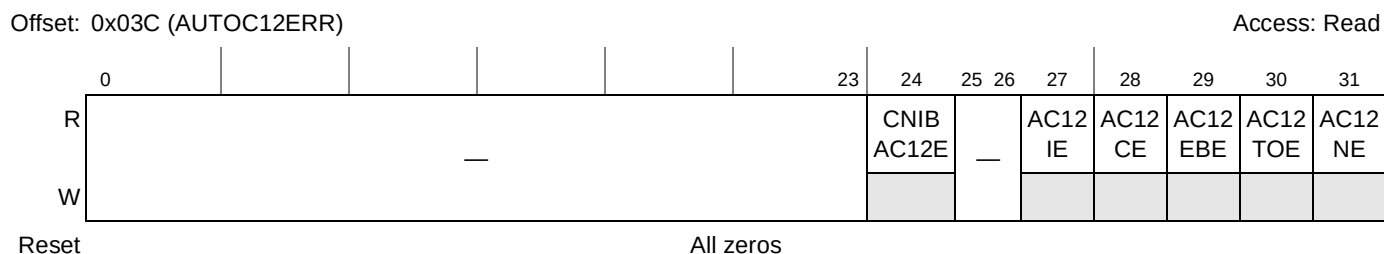
Figure 17-15. Auto CMD12 Error Status Register (AUTOC12ERR)
