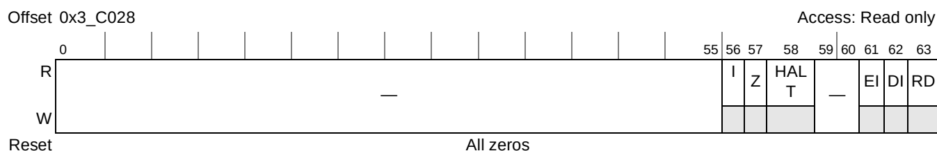
Figure 20-96. PKEU Status Register
