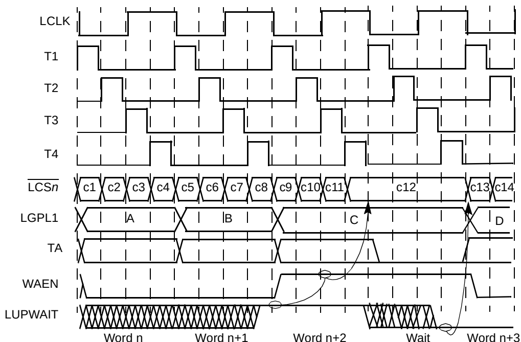
Figure 12-69. Effect of LUPWAIT Signal with PLL Bypass
