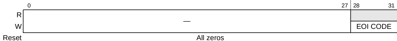
Figure 9-49. End of Interrupt Registers (EOIn)
