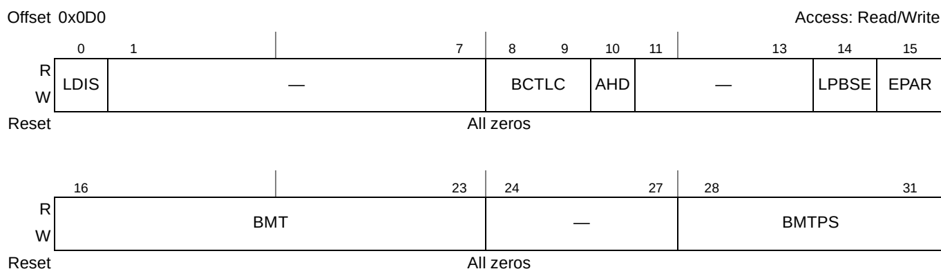
Figure 12-19. Local Bus Configuration Register
