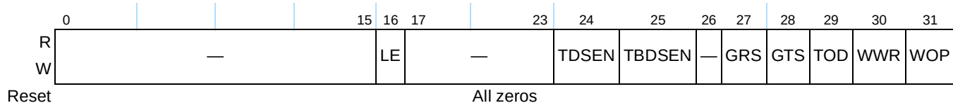
Figure 14-9. DMACTRL Register
