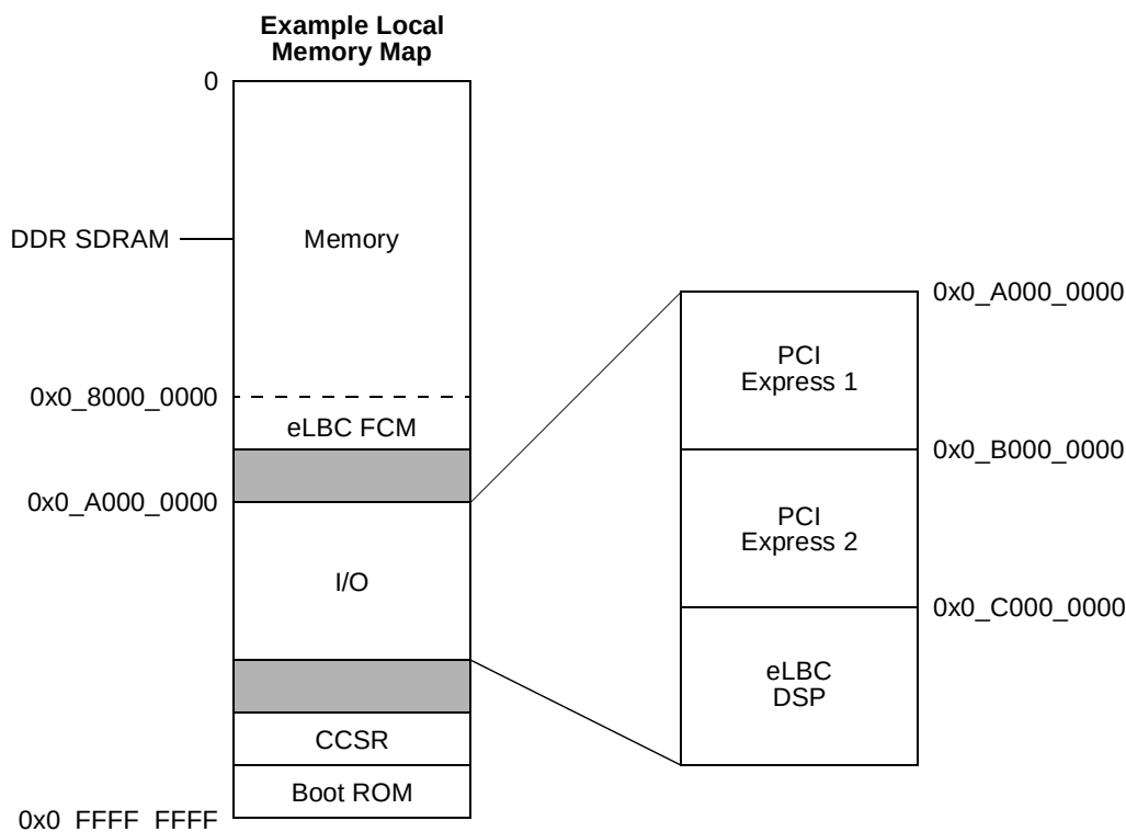
Figure 2-9. Local Address Map Example
