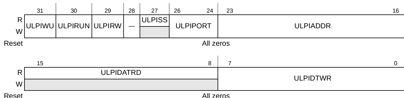
Figure 18-19. ULPI Register Access (ULPI VIEWPORT)
