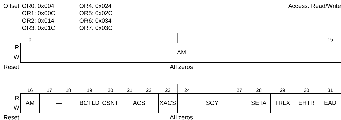
Figure 12-3. Option Registers (OR n ) in GPCM Mode
