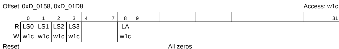
Figure 15-49. Port m Serial Link Command and Status Register (PmSLCSR)
