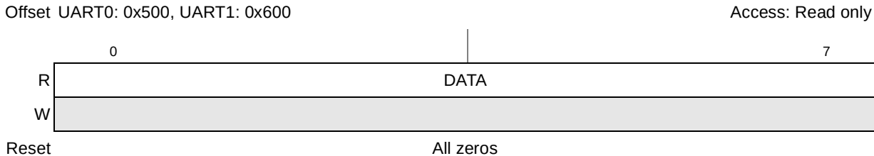
Figure 11-2. Receiver Buffer Registers (URBRn)
