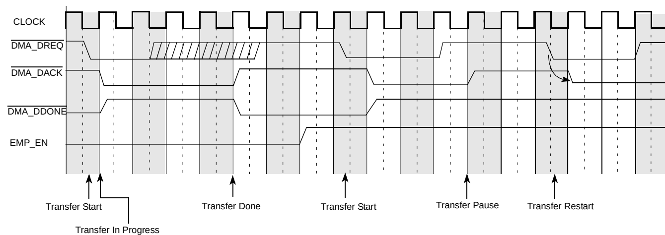
Figure 13-24. External Control Interface Timing
