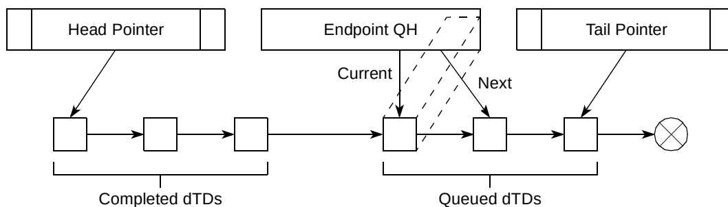
Figure 18-65. Software Link Pointers
