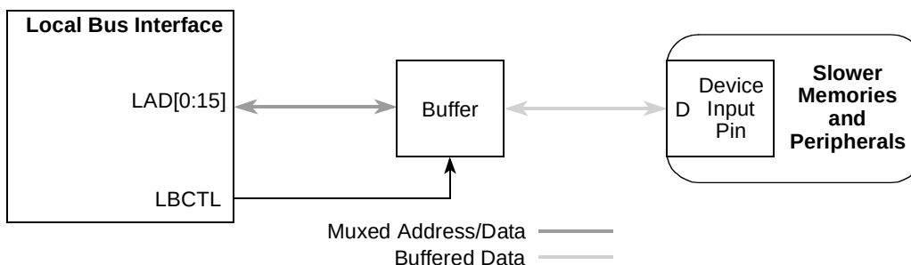
Figure 12-74. GPCM Data Timings
