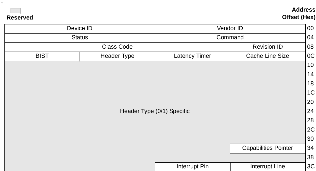
Figure 16-38. PCI Express PCI-Compatible Configuration Header Common Registers
