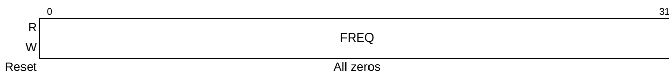
Figure 9-11. Timer Frequency Reporting Registers (TFRR x )
