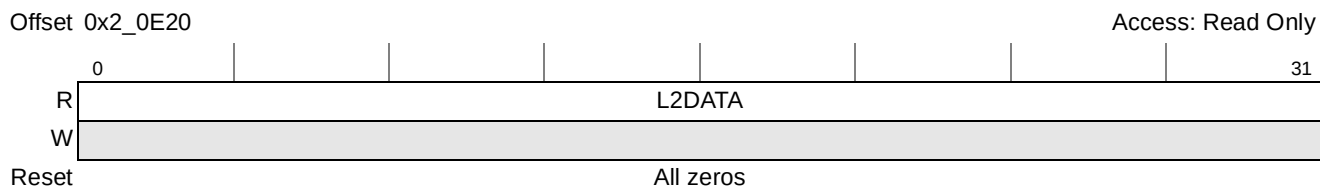
Figure 6-17. L2 Error Capture Data High Register (L2CAPTDATAHI)
