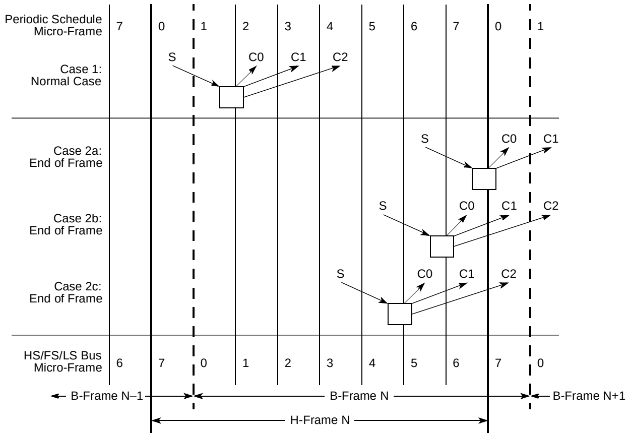
Figure 18-53. Split Transaction, Interrupt Scheduling Boundary Conditions
