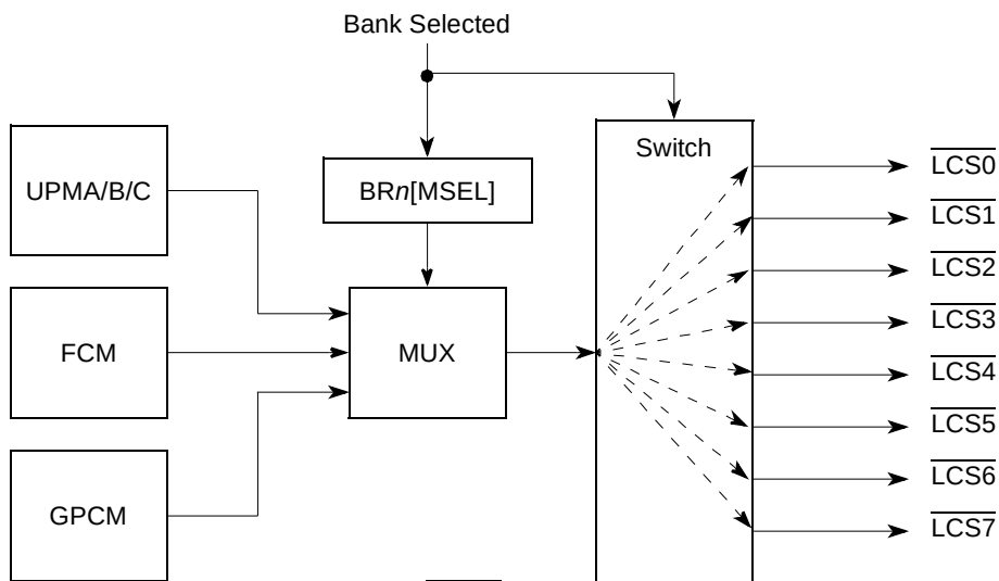
Figure 12-67. \overline{LCS}_n Signal Selection
