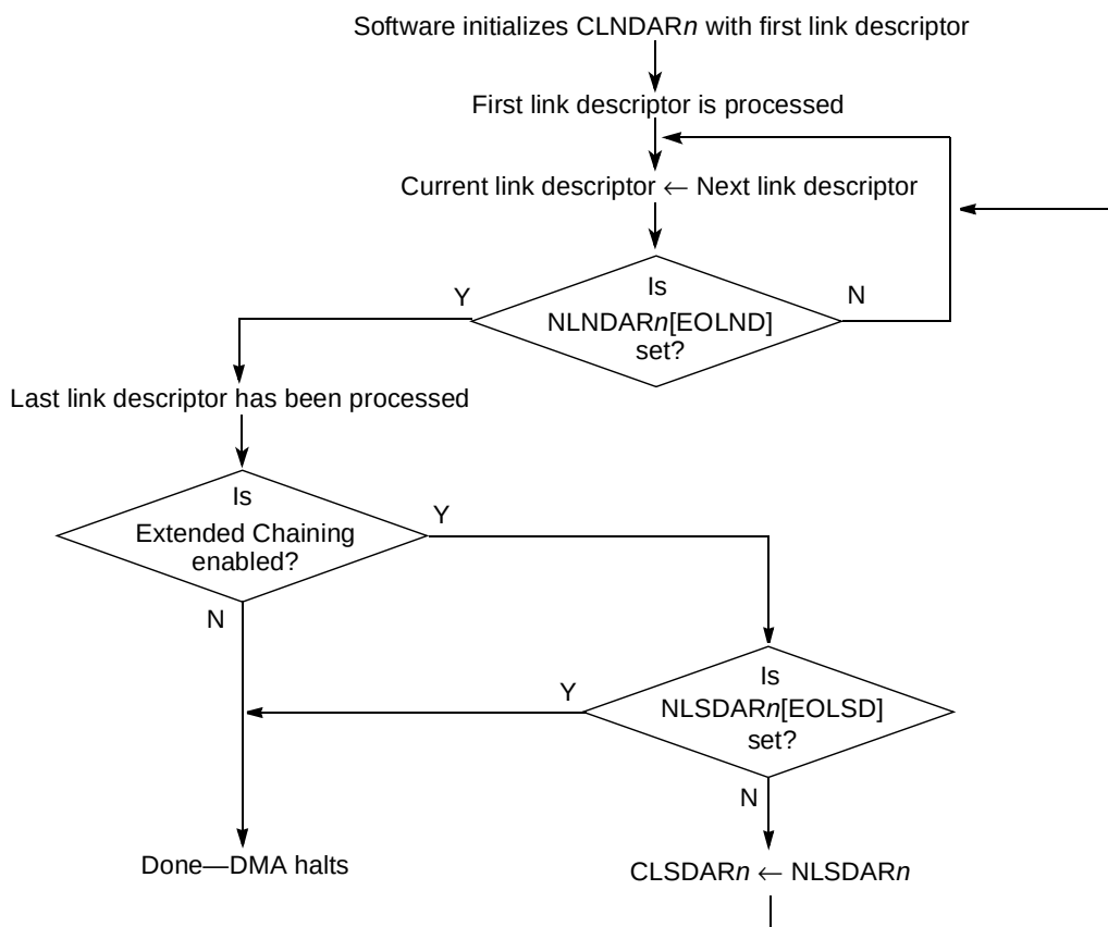
Figure 13-7. Basic Chaining Mode Flow Chart
