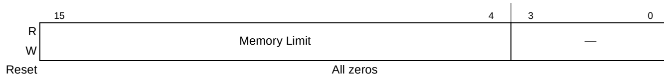
Figure 16-69. PCI Express Memory Limit Register
