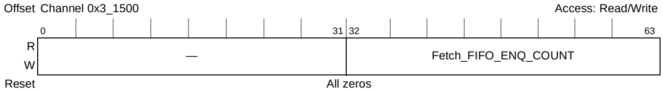
Figure 20-7. Fetch FIFO Enqueue Counter
