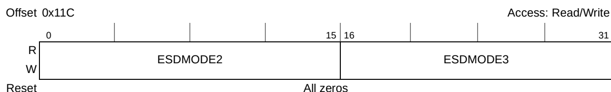
Figure 8-12. DDR SDRAM Mode 2 Configuration Register (DDR_SDRAM_MODE_2)
