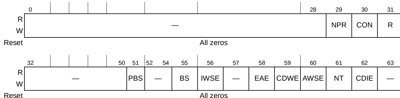
Figure 20-11. Channel Configuration Register (CCR)
