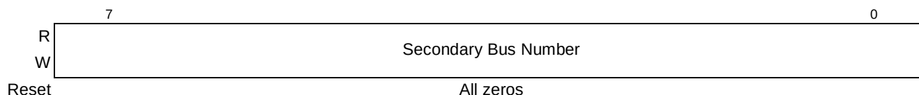
Figure 16-63. PCI Express Secondary Bus Number Register
