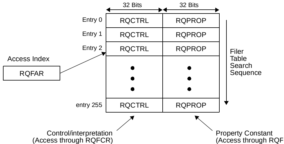
Figure 14-146. Structure of the Receive Queue Filer Table
