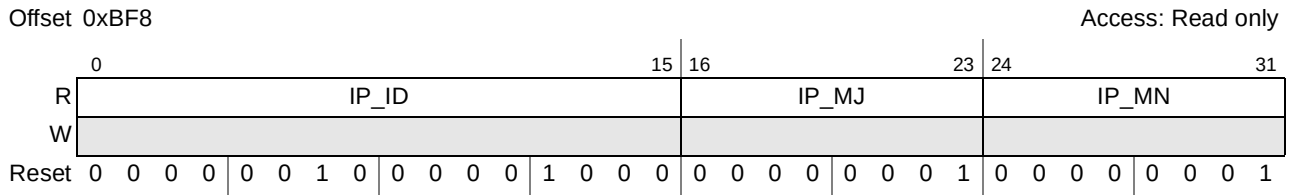
Figure 16-11. IP Block Revision Register 1
