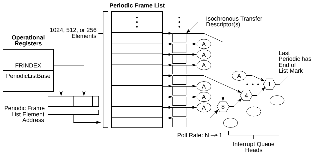
Figure 18-35. Periodic Schedule Organization
