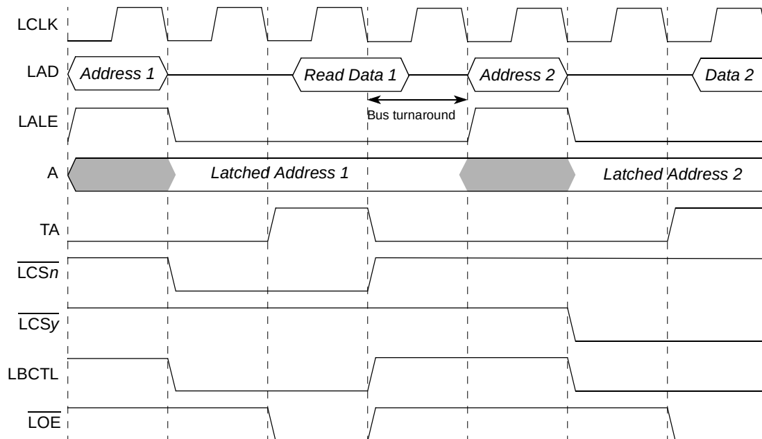
Figure 12-42. GPCM Read Followed by Read (TRLX = 0, EHTR = 0, Fastest Timing)
