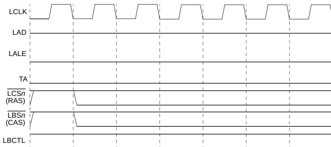
Figure 12-79. Refresh Cycle (CBR) to FPM DRAM
