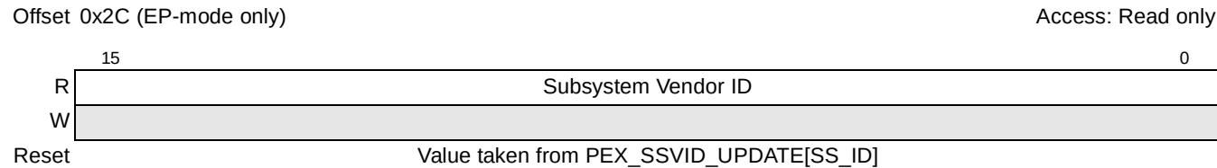
Figure 16-53. PCI Express Subsystem Vendor ID Register
