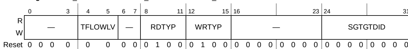
Figure 15-59. Port m RapidIO Outbound Window Segment 1–3 Registers 1–8 (PmROWSnRp)
