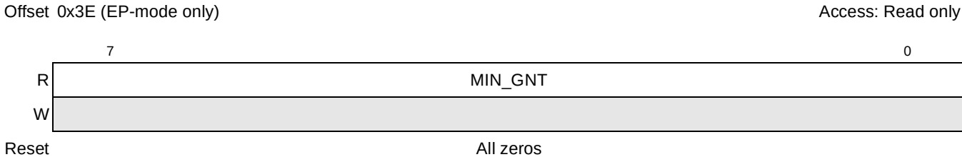
Figure 16-58. PCI Express Maximum Grant Register (MAX_GNT)
