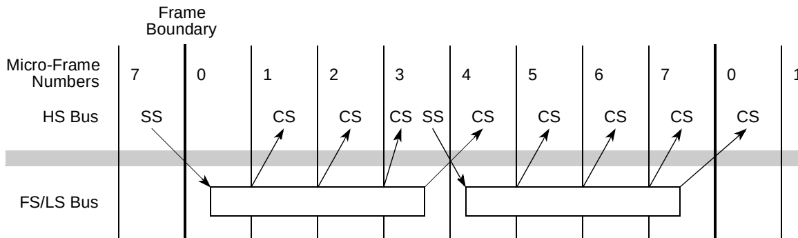
Figure 18-45. Frame Boundary Relationship Between HS Bus and FS/LS Bus
