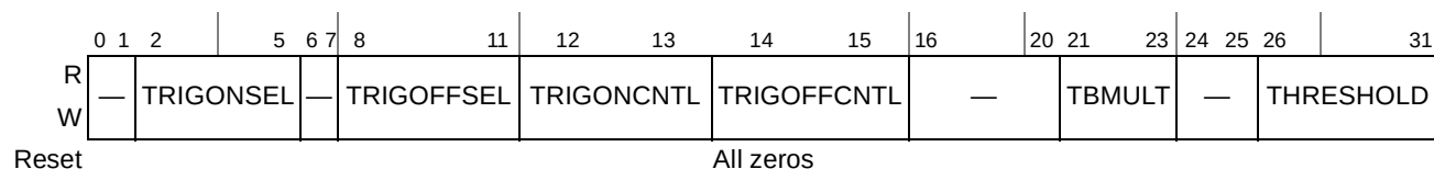
Figure 23-6. Performance Monitor Local Control Register B (PMLCB1–PMLCB11)
