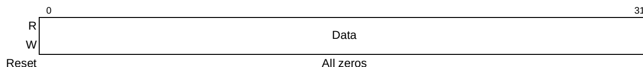
Figure 16-3. PCI Express Configuration Data Register (PEX_CONFIG_DATA)
