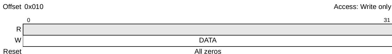
Figure 19-7. eSPI Transmit Data Register (SPITF)
