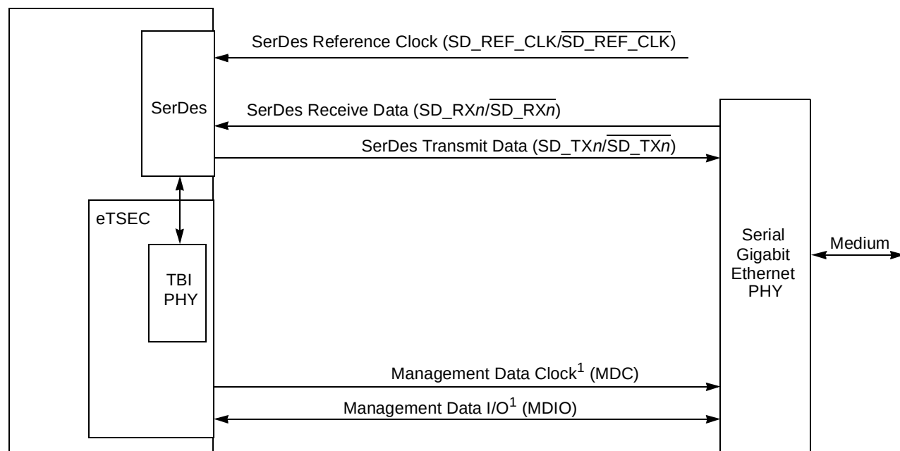
Figure 14-138. eTSEC-SGMII Connection
