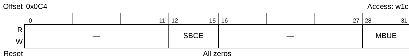
Figure 12-18. Transfer Error ECC Register (LTECCR)
