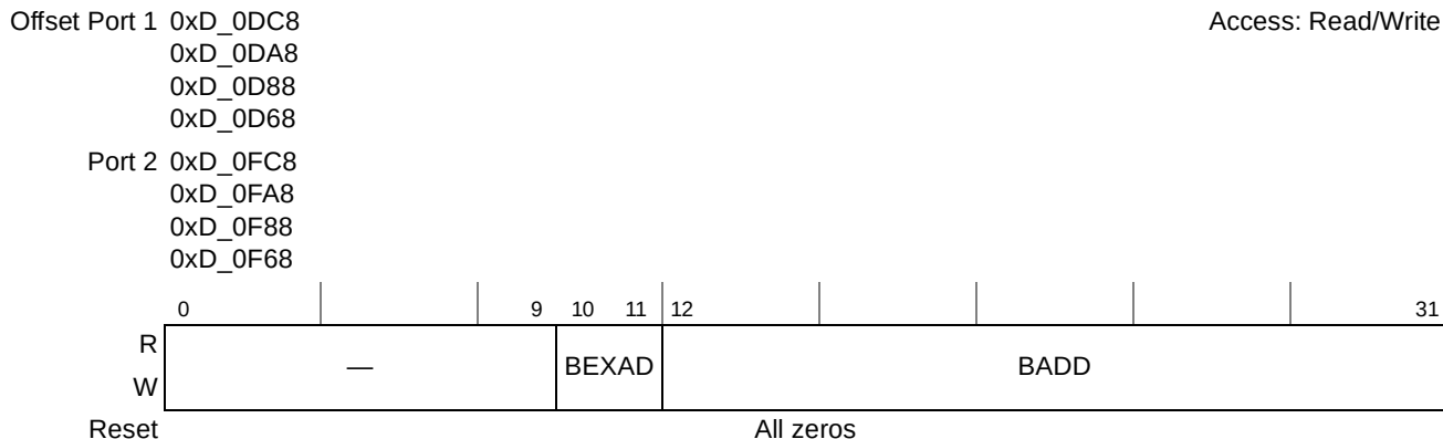
Figure 15-61. Port m RapidIO Inbound Window Base Address Registers 1–4
