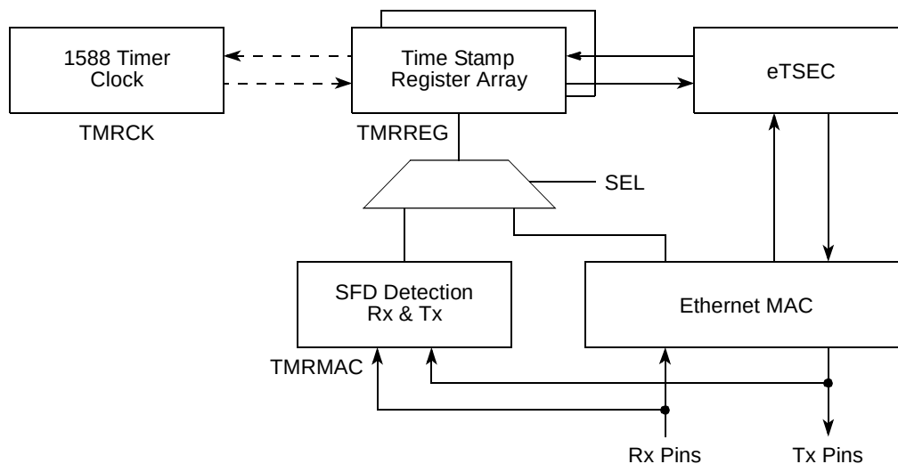
Figure 14-147. 1588 Timer Design Partition
