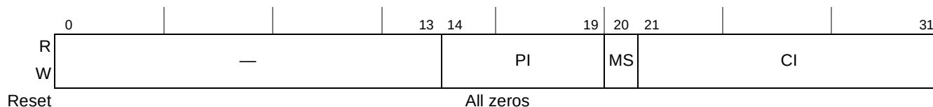
Figure 12-26. Flash Page Address Register, Large Page Device (ORx[PGS] = 1)
