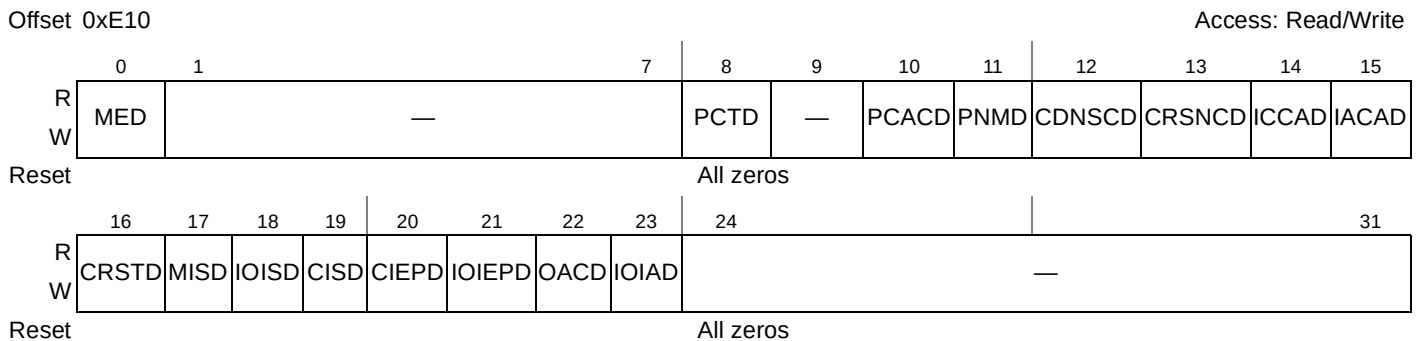
Figure 16-27. PCI Express Error Disable Register (PEX_ERR_DISR)
