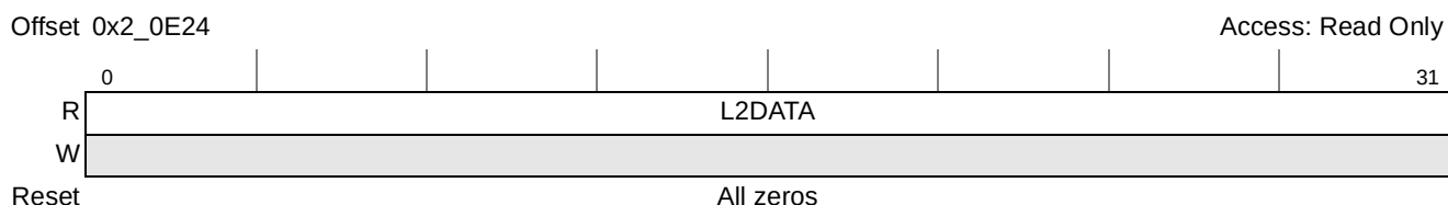
Figure 6-18. L2 Error Capture Data Low Register (L2CAPTDATALO)
