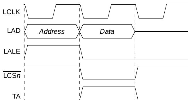
Figure 12-31. Basic eLBC Bus Cycle with LALE, TA, and \overline{LCSn} (PLL Bypass)
