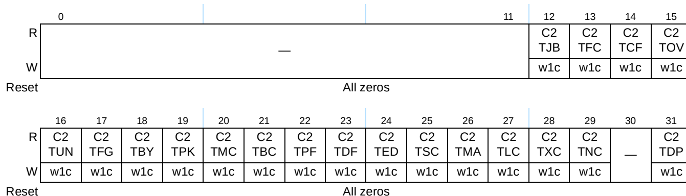
Figure 14-99. Carry Register 2 (CAR2) Register Definition
