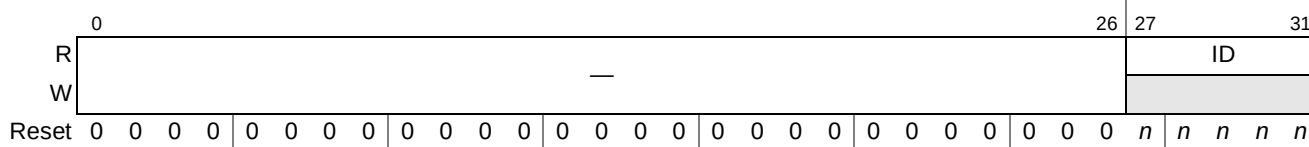
Figure 9-47. Processor Core Who Am I Registers (WHOAMIn)
