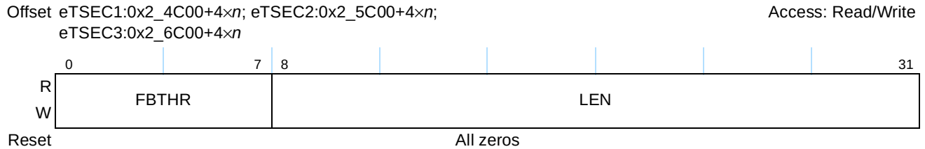
Figure 14-107. RQPRM Register Definition
