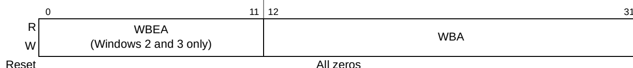
Figure 16-22. PCI Express Inbound Window Base Address Registers (PEXIWBARN)
