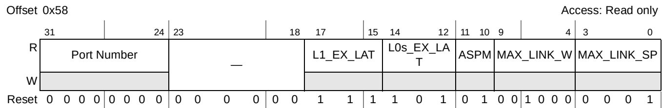
Figure 16-90. PCI Express Link Capabilities Register
