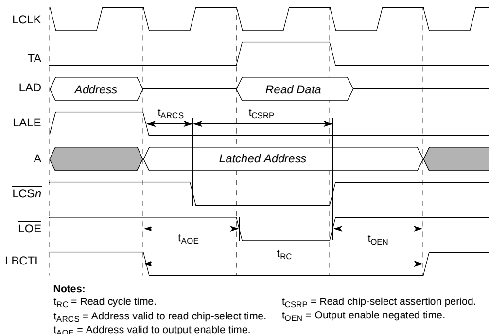
Figure 12-35. GPCM General Read Timing Parameters with PLL Bypass
