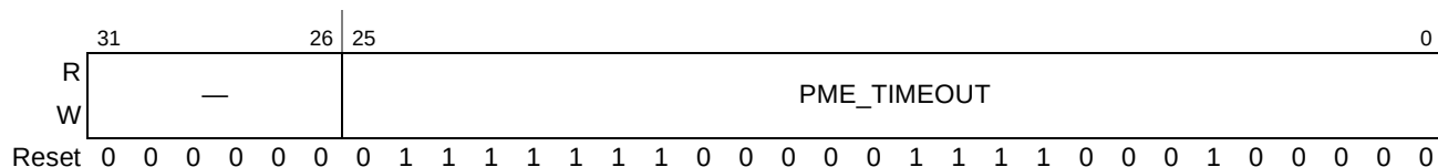
Figure 16-120. PCI Express PME Time-Out Register (PEX_PME_TIMEOUT)
