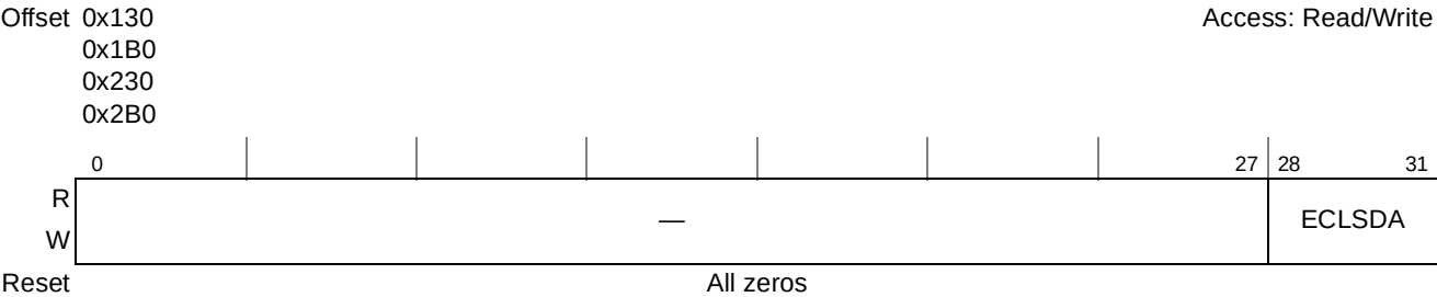
Figure 13-16. Extended Current List Descriptor Address Registers (ECLSDARn)
