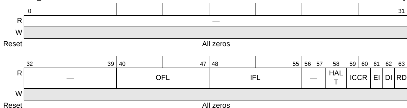
Figure 20-68. KEU Status Register
