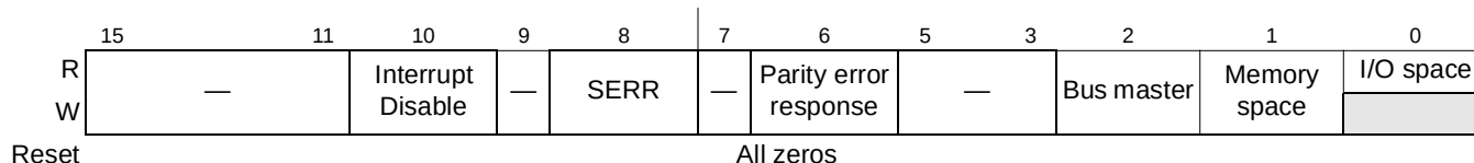
Figure 16-42. PCI Express Command Register
