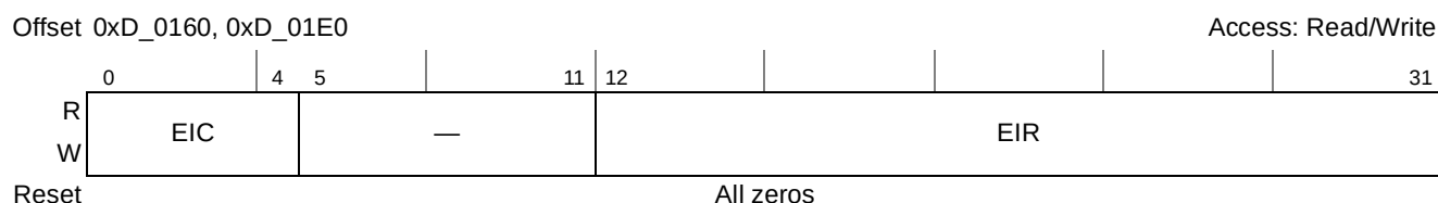
Figure 15-50. Port m Serial Link Error Injection Configuration Register (PmSLEICR)
