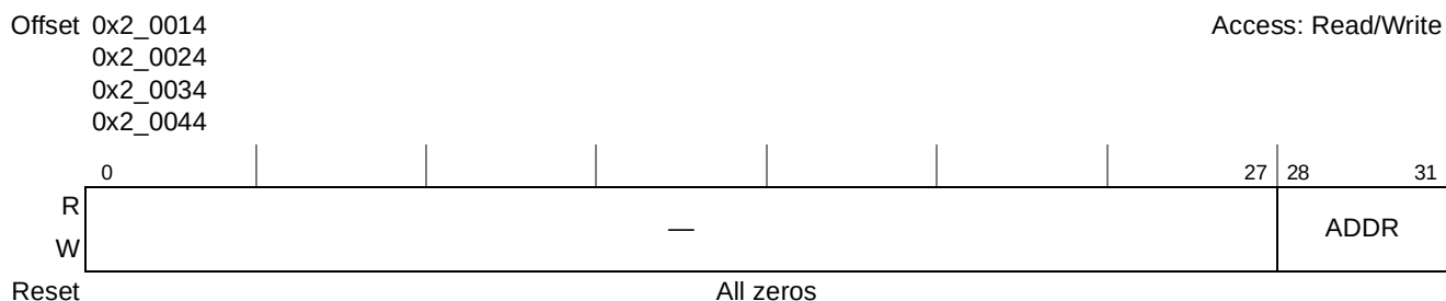
Figure 6-10. Cache External Write Address Registers Extended Address (L2CEWAREAn)
