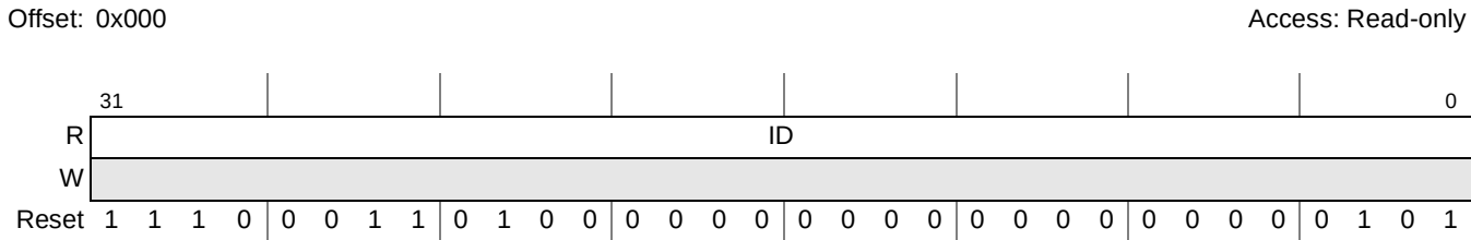
Figure 18-2. ID Register
