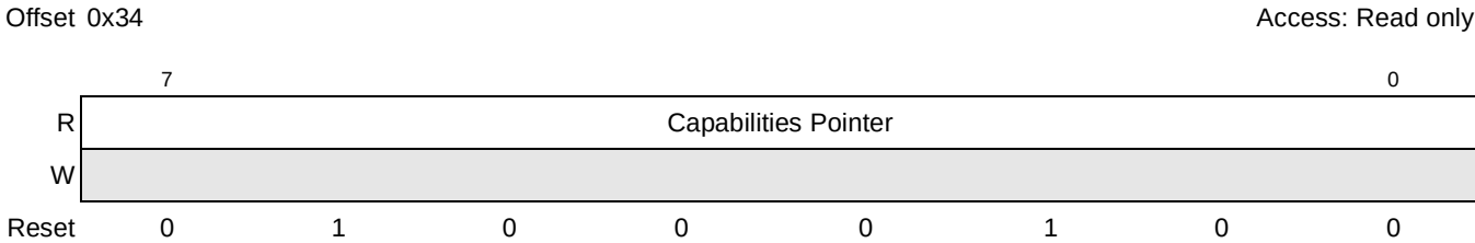
Figure 16-55. Capabilities Pointer Register
