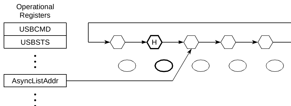
Figure 18-44. General Format of Asynchronous Schedule List
