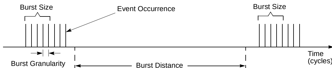
Figure 23-10. Burst Size, Distance, Granularity, and Burstiness Counting
