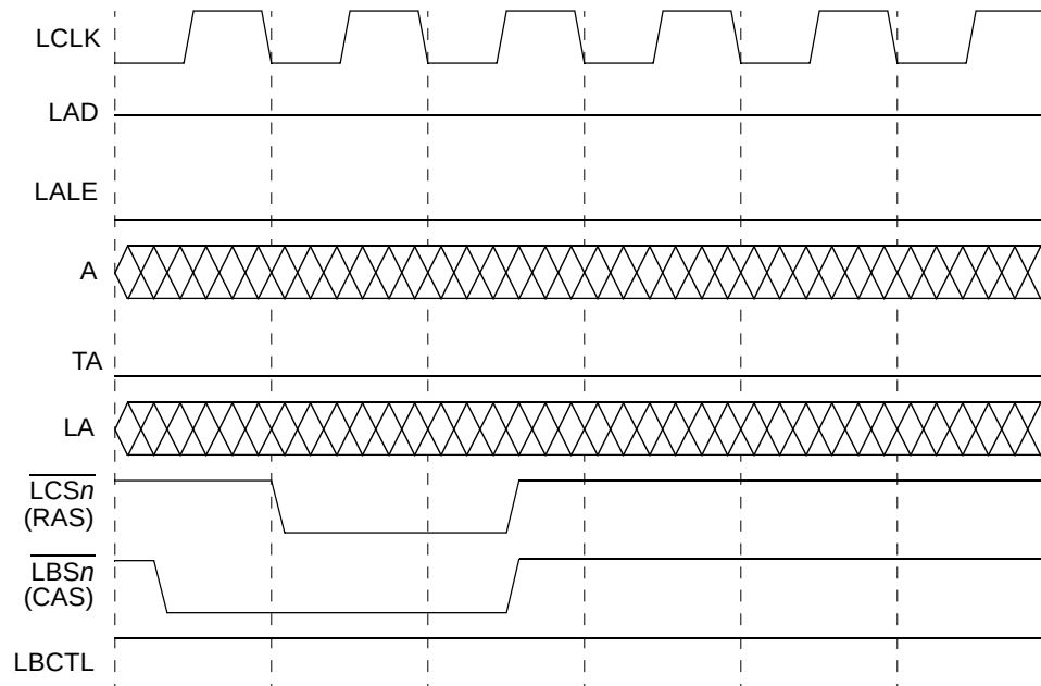
Figure 12-78. Burst Read Access to FPM DRAM Using LOOP (Two Beats Shown)
