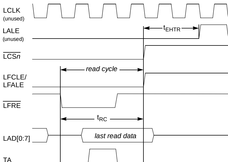
Figure 12-59. FCM Read Data Timing with Extended Hold Time (for TRLX = 0 , EHTR = 1 , RST = 1 , SCY = 1 )
