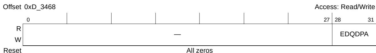
Figure 15-92. Extended Inbound Doorbell Queue Dequeue Pointer Address Registers (EIDQDPAR)
