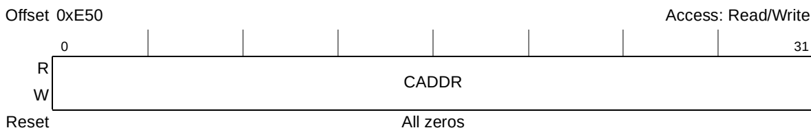
Figure 8-44. Memory Error Address Capture Register (CAPTURE_ADDRESS)
