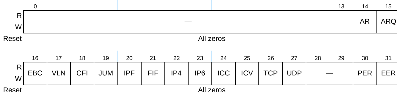
Figure 14-32. Receive Queue Filer Table Property ID1 Register Definition
