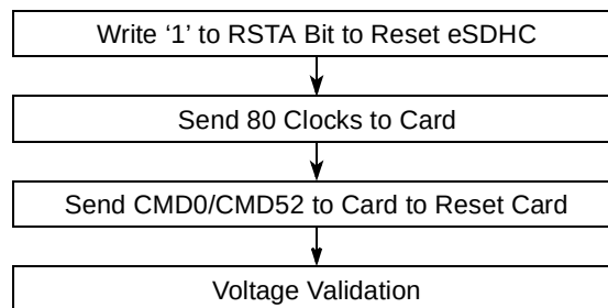
Figure 17-26. Flow Chart for Reset of eSDHC and SD I/O Card
