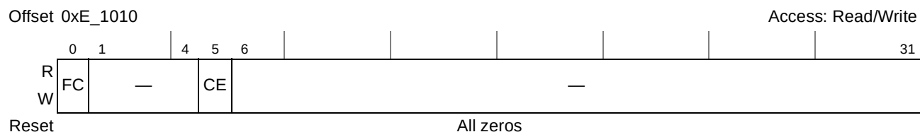
Figure 23-3. Performance Monitor Local Control Register A0 (PMLCA0)
