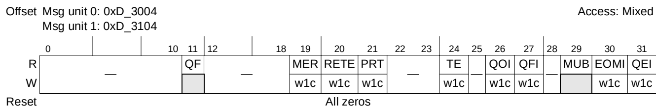
Figure 15-65. Outbound Message n Status Registers (OMnSR)
