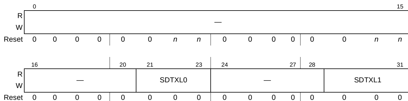
Figure 22-27. SRDS Control Register 5(SRDSCR5)
