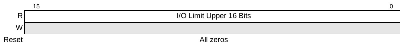
Figure 16-75. PCI Express I/O Limit Upper 16 Bits Register
