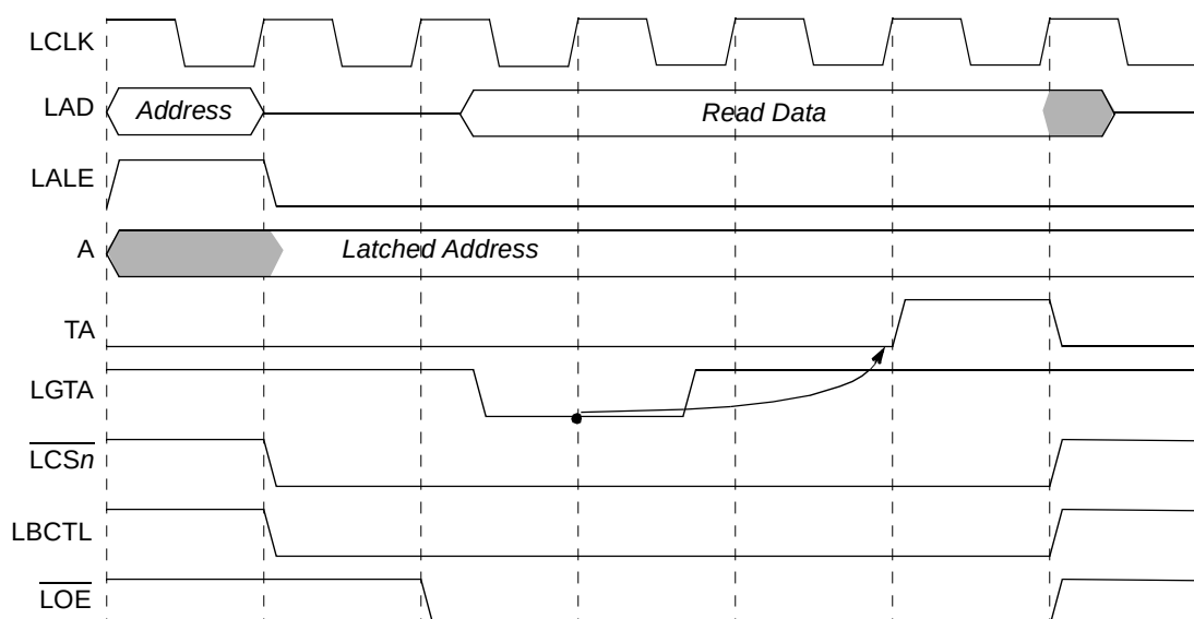
Figure 12-44. External Termination of GPCM Access (PLL Enabled Mode)
