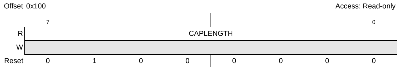
Figure 18-3. Capability Registers Length (CAPLENGTH)
