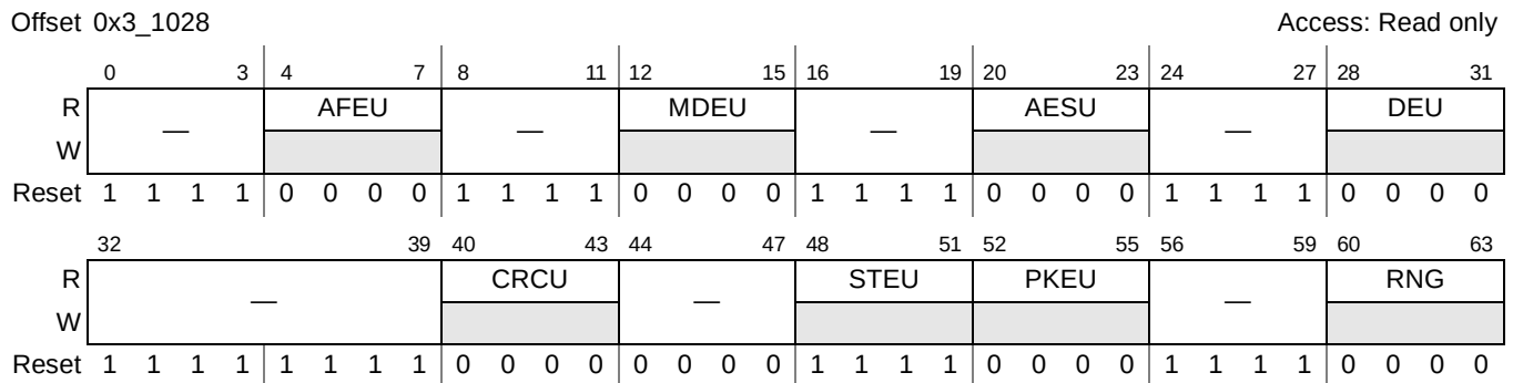
Figure 20-16. EU Assignment Status Register (EUASR)
