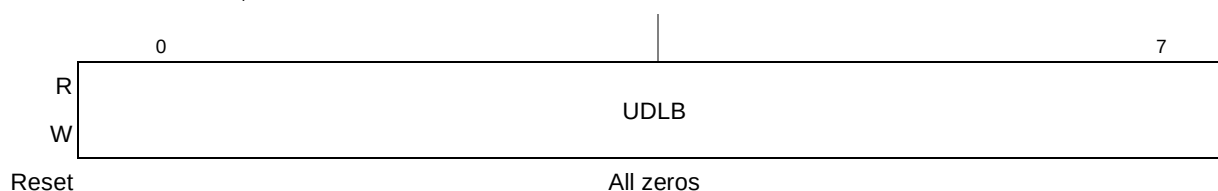
Figure 11-5. Divisor Least Significant Byte Registers (UDLBn)
