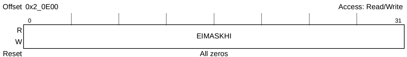
Figure 6-14. L2 Error Injection Mask High Register (L2ERRINJHI)
