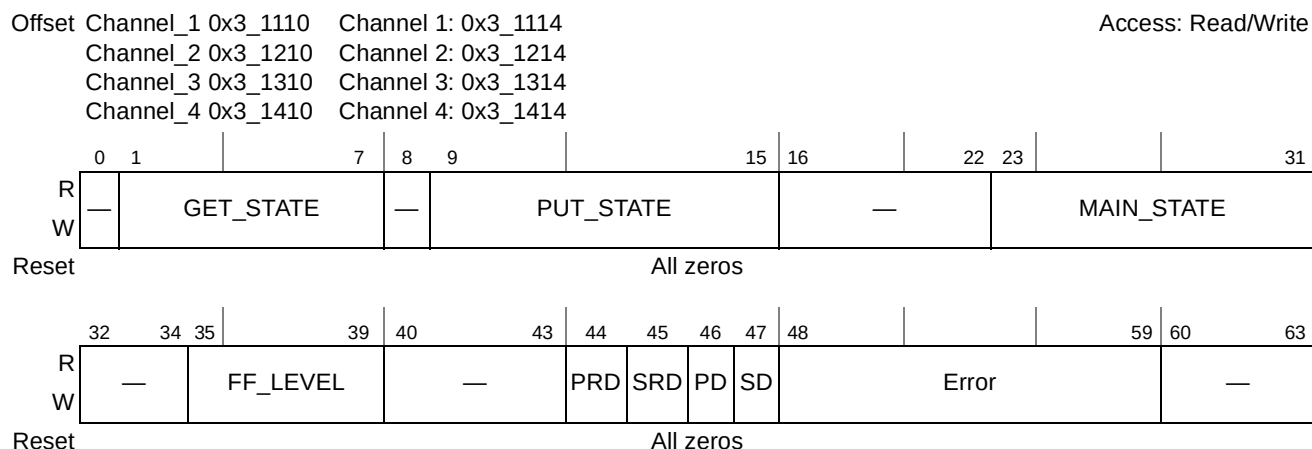
Figure 20-12. Channel Status Register (CSR)
