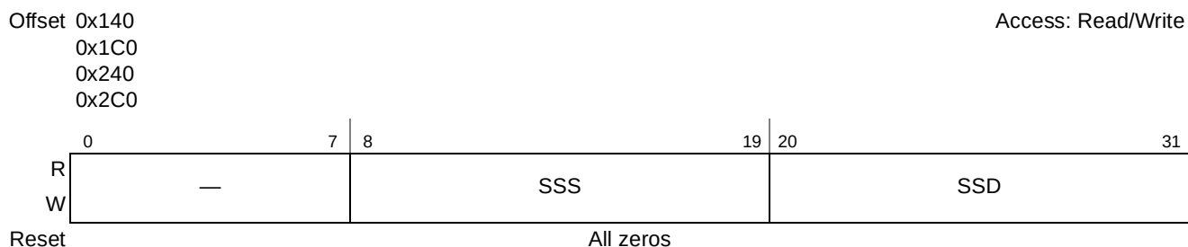
Figure 13-20. Source Stride Registers (SSR n )
