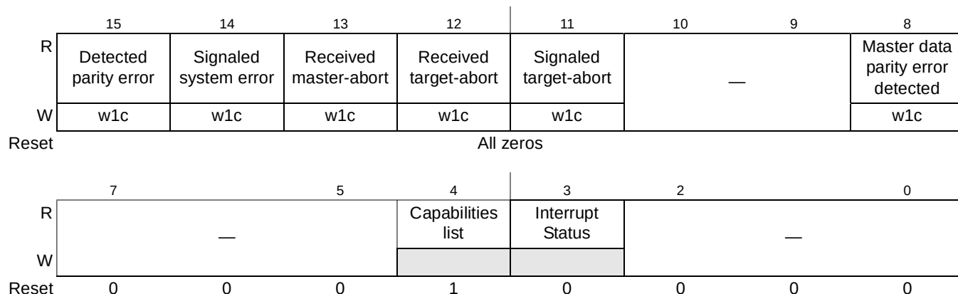
Figure 16-43. PCI Express Status Register
