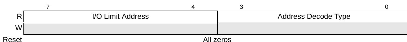
Figure 16-66. PCI Express I/O Limit Register
