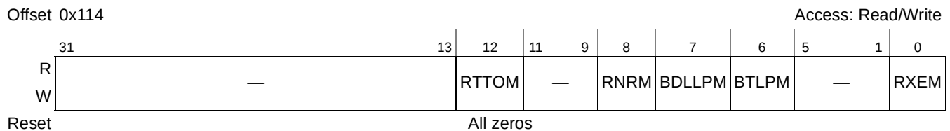
Figure 16-109. PCI Express Correctable Error Mask Register
