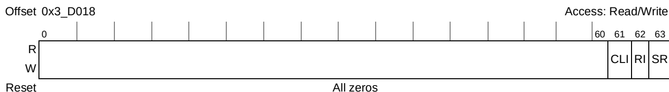
Figure 20-110. STEU Reset Control Register
