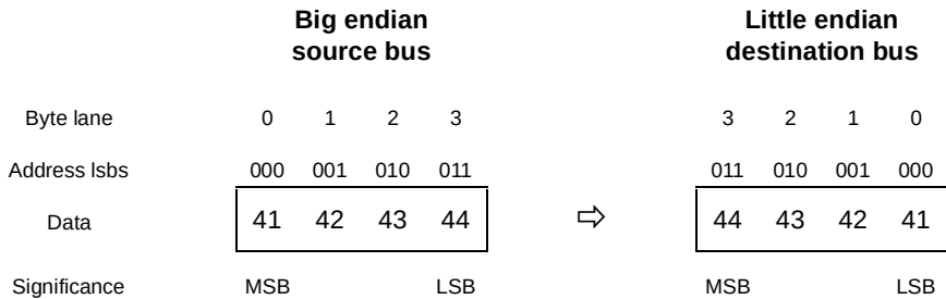
Figure 16-128. Address Invariant Byte Ordering—4 bytes Outbound
