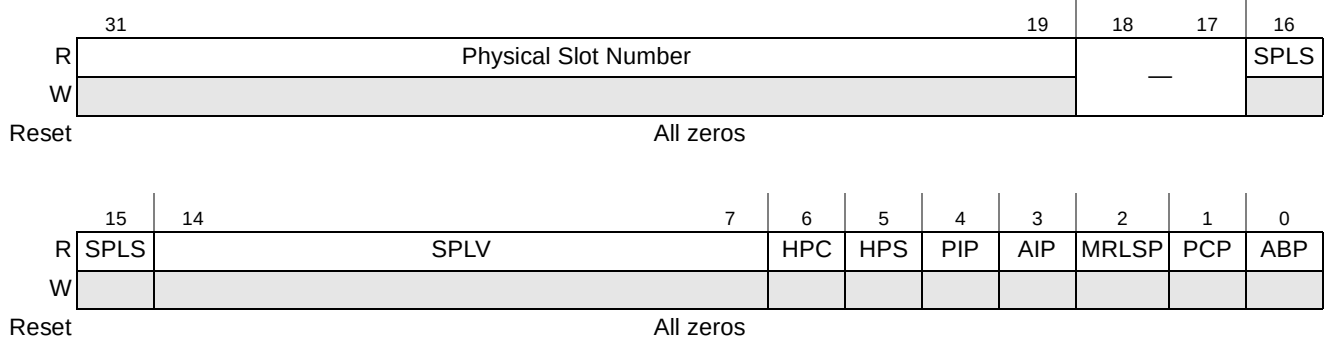
Figure 16-93. PCI Express Slot Capabilities Register
