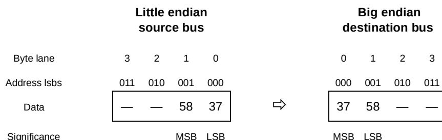
Figure 16-131. Address Invariant Byte Ordering—2 bytes Inbound
