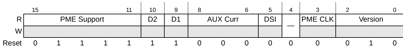
Figure 16-82. PCI Express Power Management Capabilities Register
