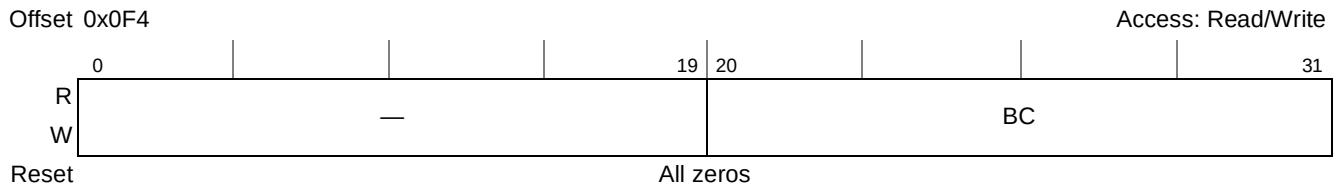
Figure 12-27. Flash Byte Count Register
