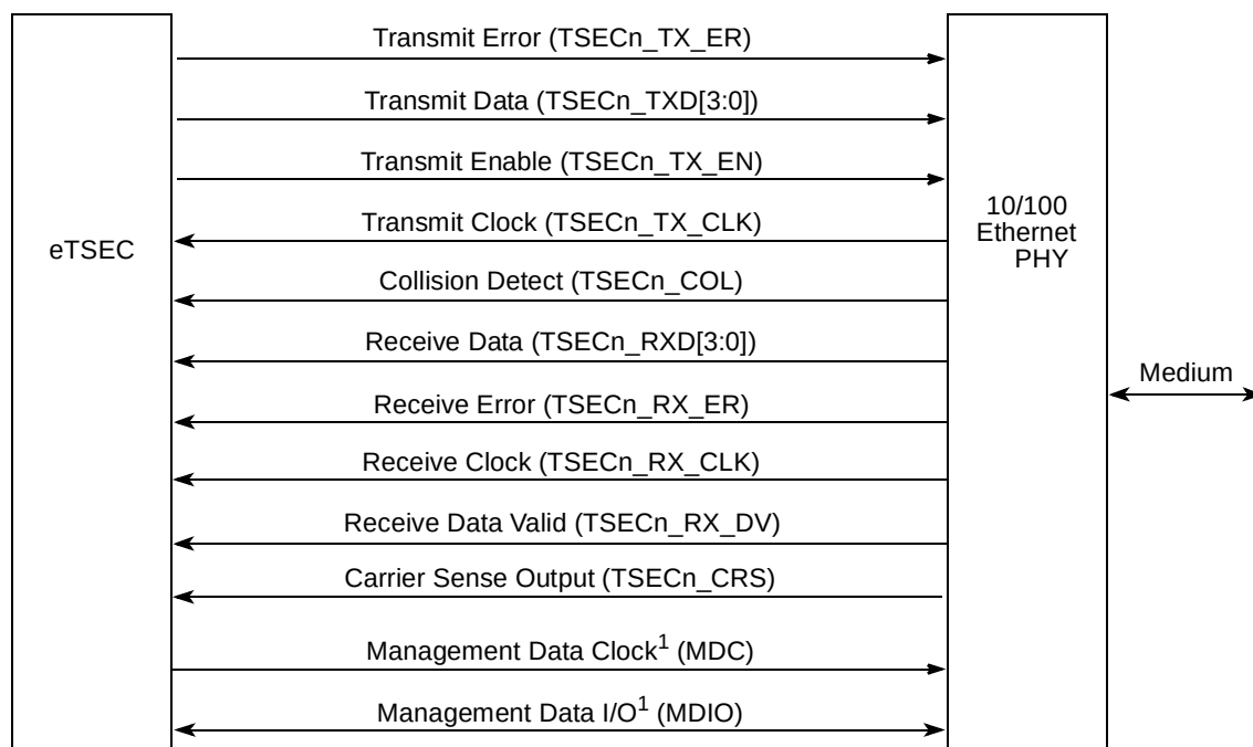
Figure 14-132. eTSEC-MII Connection
