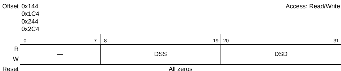
Figure 13-21. Destination Stride Registers (DSR n )
