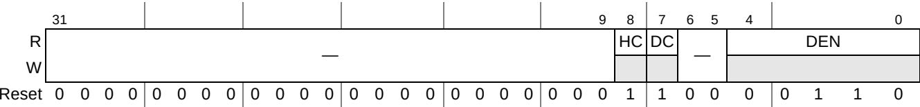
Figure 18-8. Device Control Capability Parameters (DCCPARAMS)
