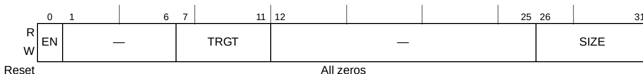
Figure 2-8. Local Access Window Attributes Registers (LAWAR0 to LAWAR9)
