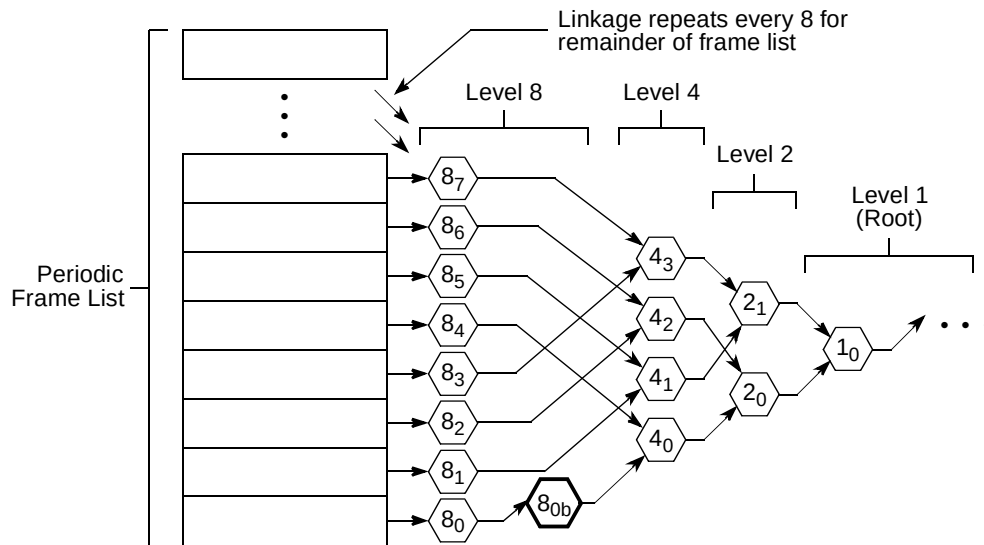
Figure 18-54. General Structure of EHCI Periodic Schedule Utilizing Interrupt Spreading
