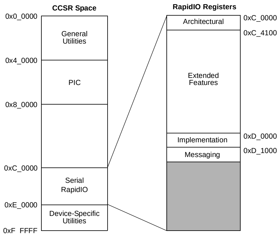
Figure 2-5. Serial RapidIO Register Map within CCSR Space
