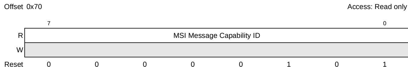
Figure 16-98. PCI Express Capability ID Register
