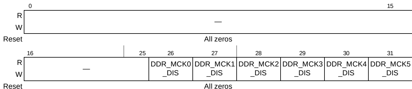
Figure 22-19. DDR Clock Disable Register (DDRCLKDR)
