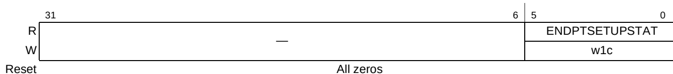
Figure 18-23. Endpoint Setup Status (ENDPTSETUPSTAT)
