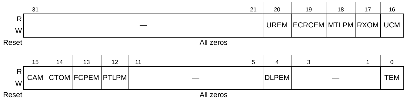
Figure 16-106. PCI Express Uncorrectable Error Mask Register
