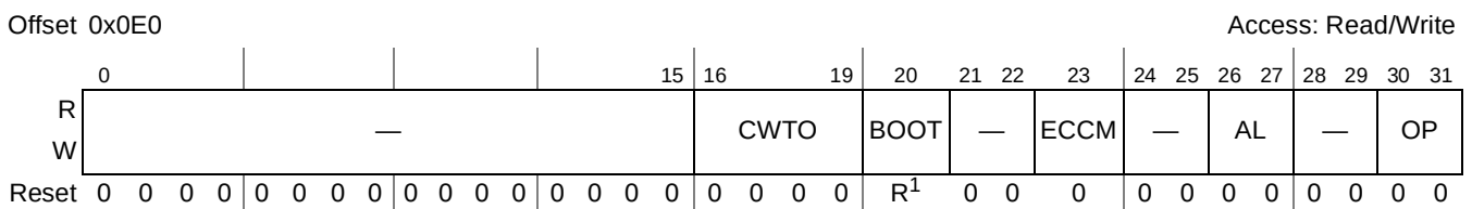
Figure 12-21. Flash Mode Register
