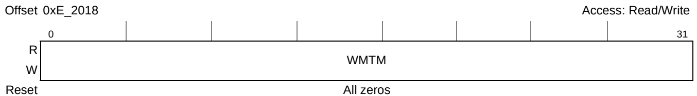
Figure 24-6. Watchpoint Monitor Transaction Mask Register (WMTMR)
