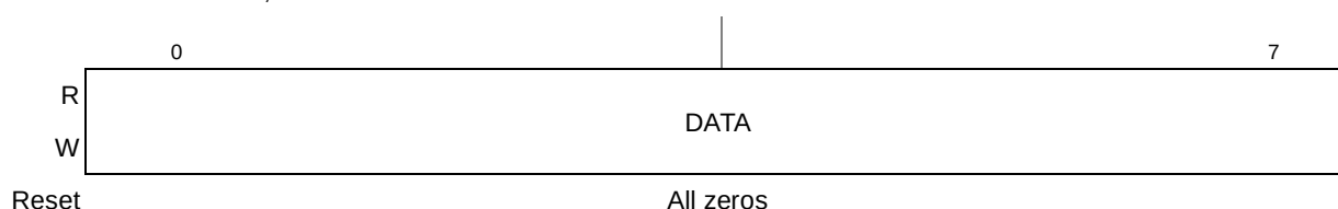
Figure 11-14. Scratch Register (USCR)
