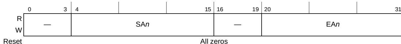
Figure 8-2. Chip Select Bounds Registers (CS n _BNDS)
