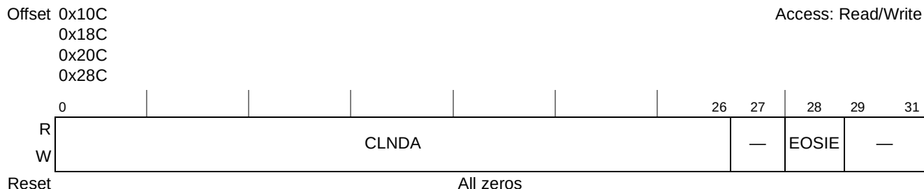
Figure 13-8. Current Link Descriptor Address Registers (CLNDAR n )
