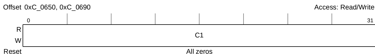
Figure 15-35. Port m Packet Error Capture Command and Status Register 1 (PmPECCSR1)
