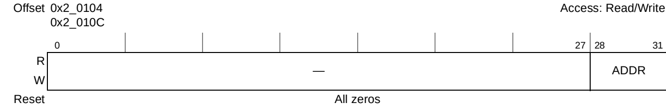
Figure 6-13. L2 Memory-Mapped SRAM Base Address Registers Extended Address 0–1 (L2SRBAREAn)
