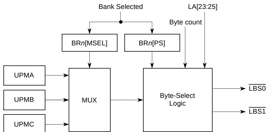
Figure 12-68. LBS Signal Selection
