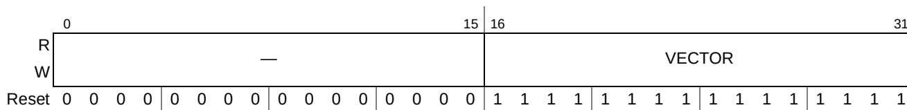
Figure 9-10. Spurious Vector Register (SVR)
