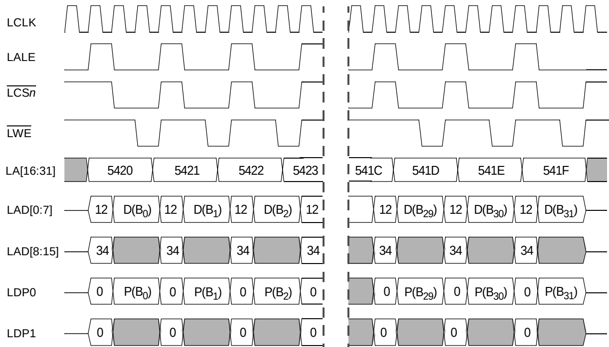
Figure 12-30. Example of 8-Bit GPCM Writing 32 Bytes to Address 0x1234_5420
