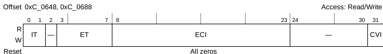
Figure 15-33. Port m Error Capture Attributes Command and Status Register ( PmECACSR )
