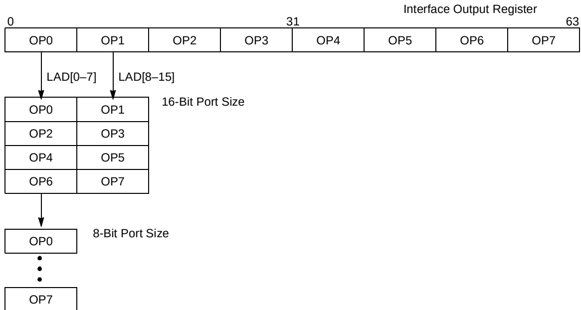
Figure 12-75. Interface to Different Port-Size Devices
