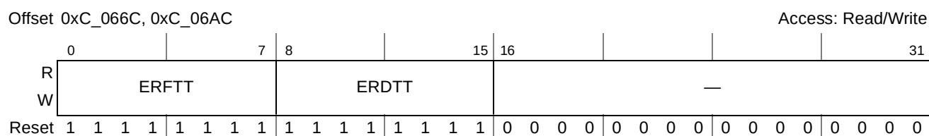
Figure 15-39. Port m Error Rate Threshold Command and Status Register (PmERTCSR)
