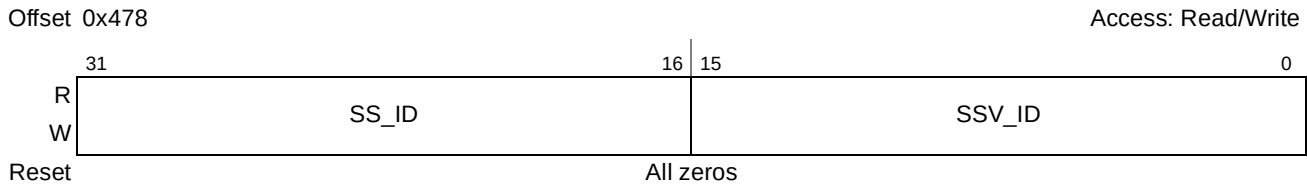
Figure 16-121. PCI Express Subsystem Vendor ID Update Register (PEX_SSVID_UPDATE)
