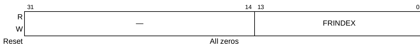
Figure 18-12. USB Frame Index (FRINDEX)
