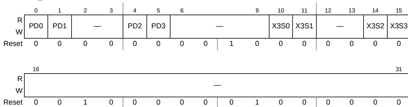
Figure 22-25. SRDS Control Register 2 (SRDSCR2)
