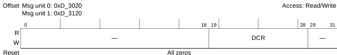
Figure 15-74. Outbound Message n Double Word Count Registers (OM n DCR)
