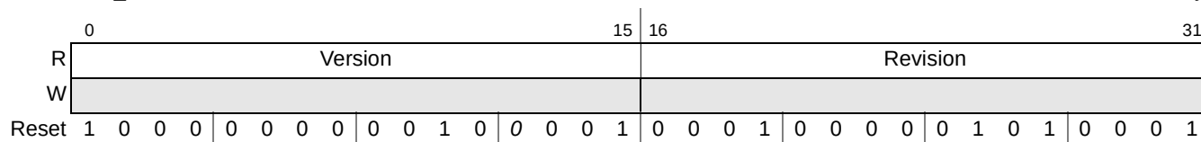
Figure 22-15. Processor Version Register (PVR)
