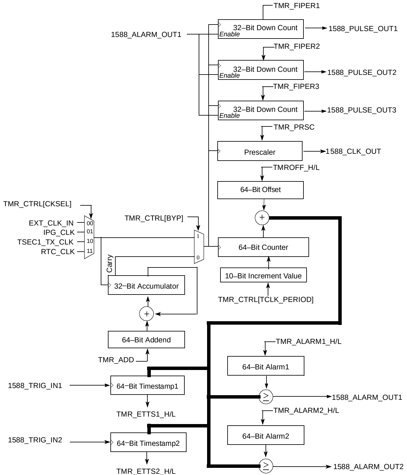
Figure 14-148. 1588 Current Time Control
