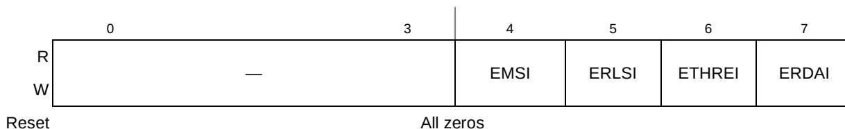
Figure 11-6. Interrupt Enable Register (UIER)
