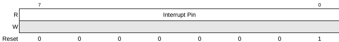
Figure 16-57. PCI Express Interrupt Pin Register
