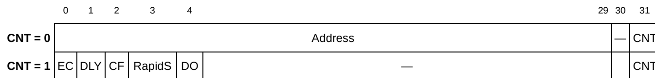
Figure 4-12. Config Address Fields
