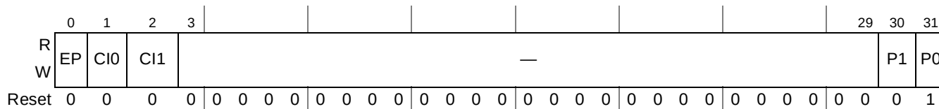
Figure 9-39. External Interrupt Destination Registers (EIDRs)
