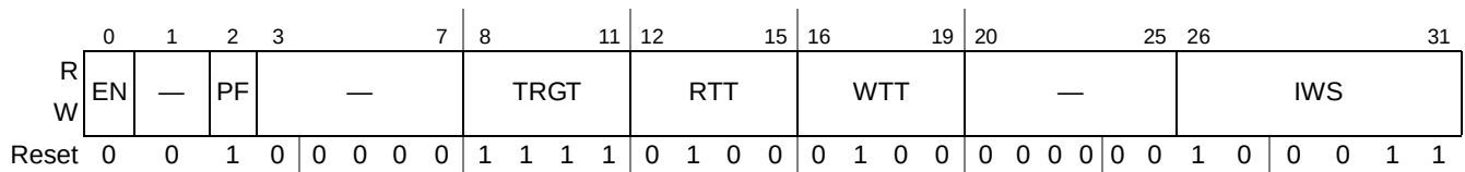
Figure 16-24. PCI Express Inbound Window Attributes Registers (PEXIWARn)
