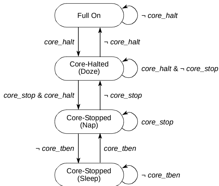
Figure 22-29. e500 Cores Power Management State Diagram
