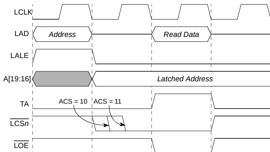
Figure 12-34. GPCM Basic Read Timing (XACS = 0, ACS = 1x, TRLX = 0)
