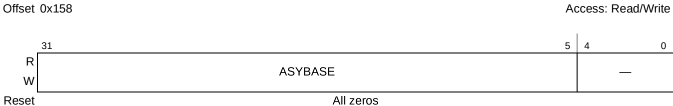
Figure 18-15. Current Asynchronous List Address (ASYNCLISTADDR)
