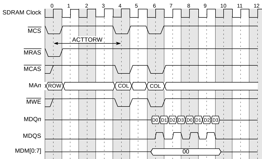
Figure 8-54. Registered DDR SDRAM DIMM Burst Write Timing
