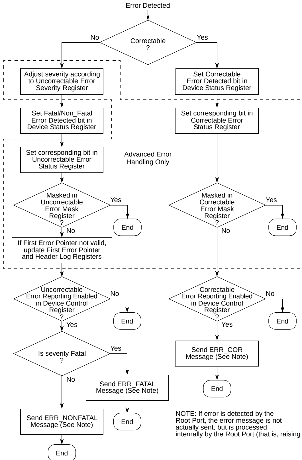
Figure 16-134. PCI Express Device Error Signaling Flowchart
