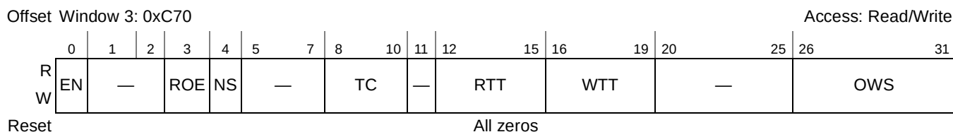
Figure 16-19. PCI Express Outbound Window Attributes Register 3 (PEXOWAR3)
