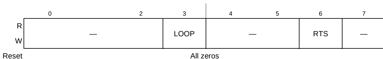
Figure 11-11. Modem Control Register (UMCR)
