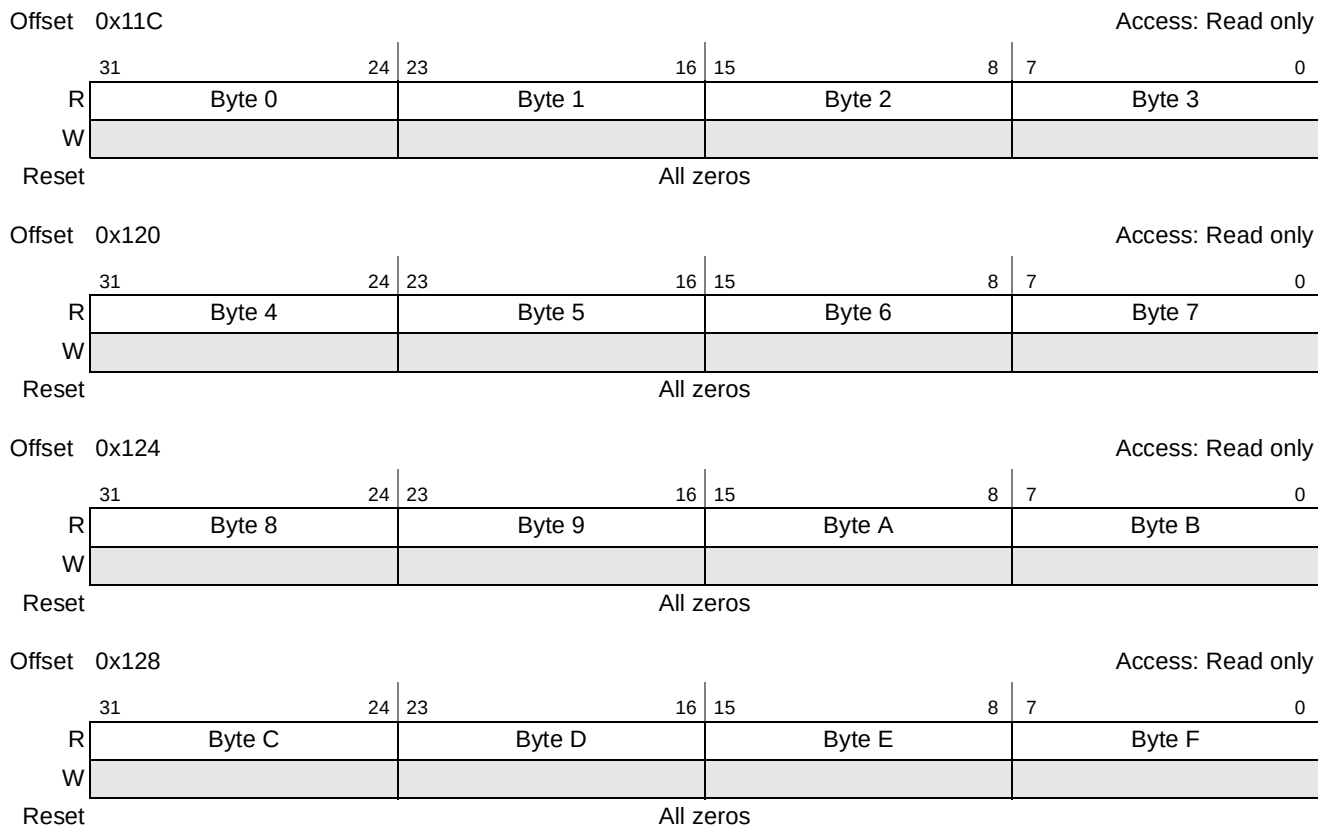
Figure 16-111. PCI Express Header Log Register
