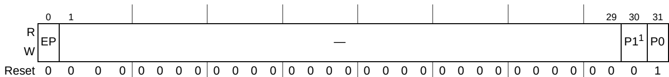
Figure 9-35. Shared Message Signaled Interrupt Destination Registers (MSIDRn)
