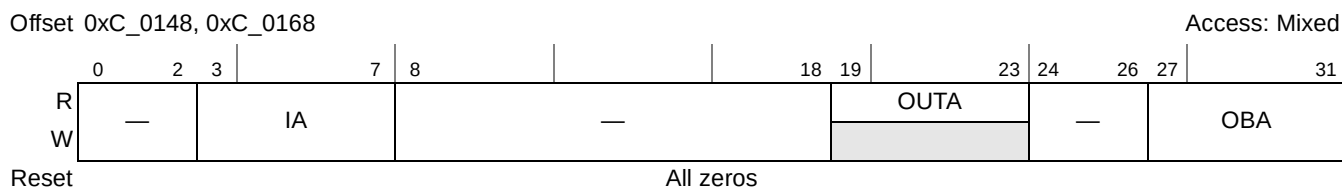
Figure 15-22. Port m Local ackID Status Command and Status Register (PmLASCSR)
