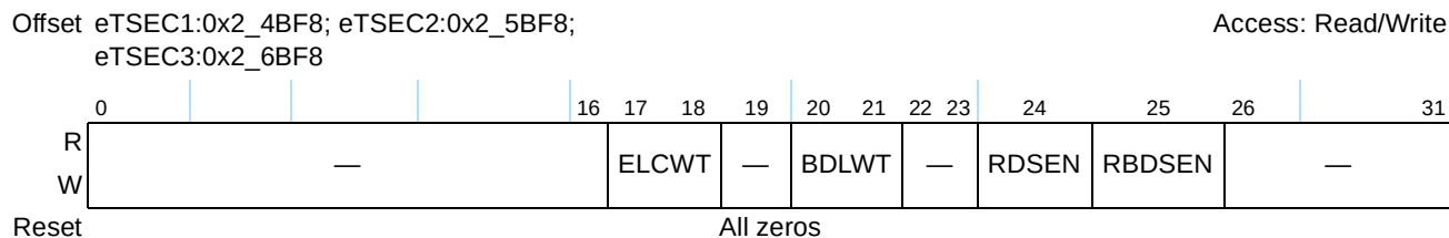
Figure 14-105. ATTR Register Definition
