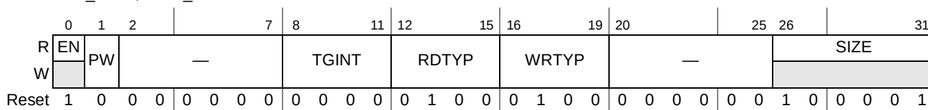
Figure 15-63. Port m RapidIO Inbound Window Attributes Register 0
