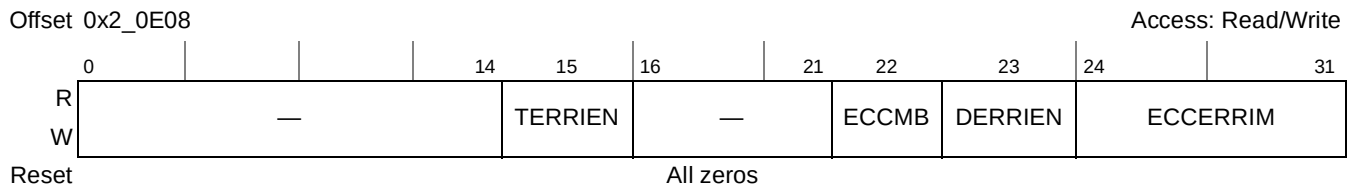
Figure 6-16. L2 Error Injection Mask Control Register (L2ERRINJCTL)
