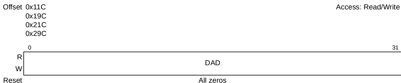
Figure 13-12. Destination Address Registers (DAR n )
