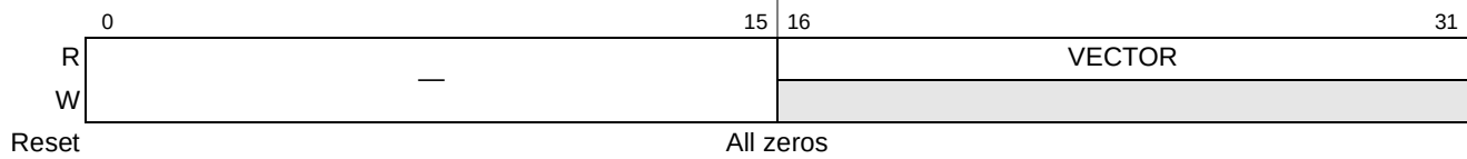
Figure 9-48. Processor Core Interrupt Acknowledge Registers (IACKn)
