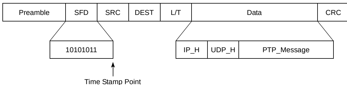
Figure 14-150. PTP Packet Format
