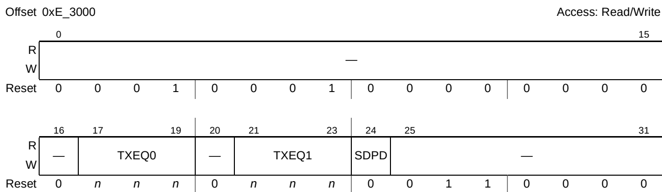
Figure 22-23. SRDS Control Register 0 (SRDSCR0)
