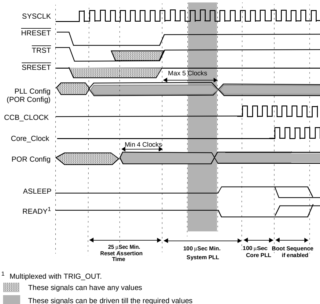
Figure 4-5. Power-On Reset Sequence
