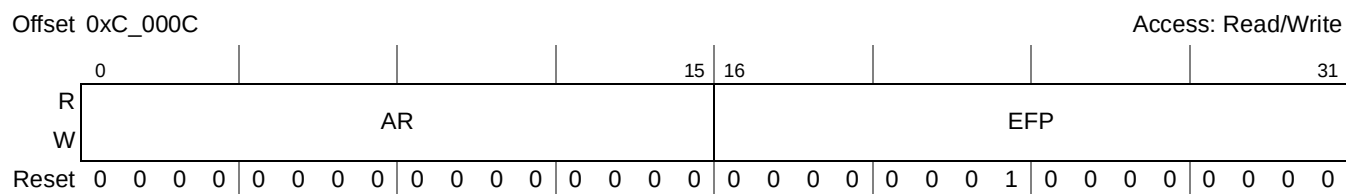
Figure 15-5. Assembly Information Capability Register (AICAR)
