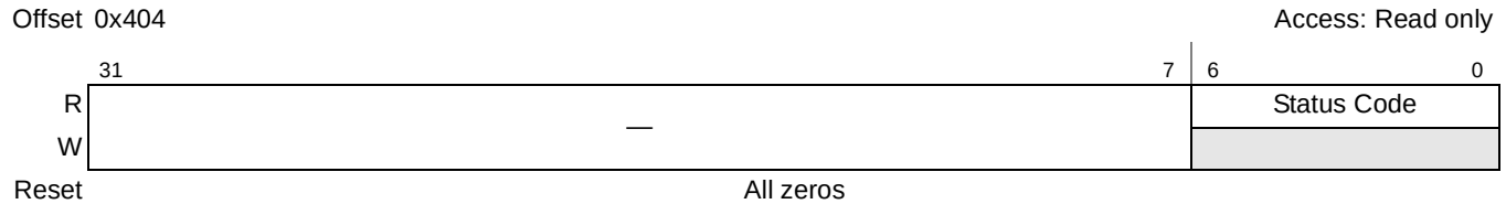
Figure 16-117. PCI Express LTSSM State Status Register (PEX_LTSSM_STAT)
