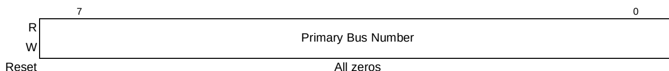
Figure 16-62. PCI Express Primary Bus Number Register
