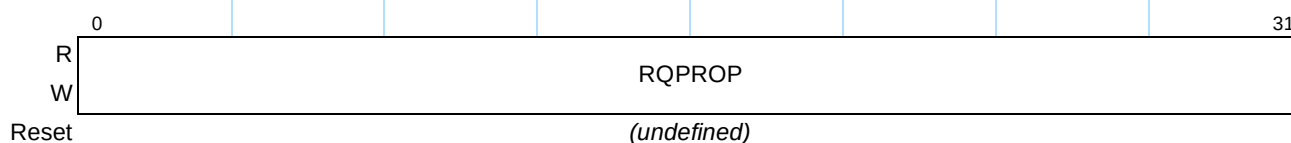
Figure 14-31. Receive Queue Filer Table Property IDs 0, 2–15 Register Definition
