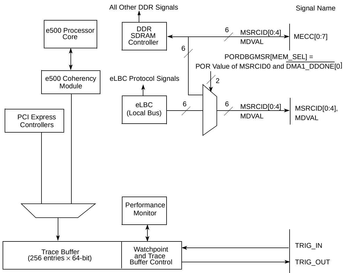
Figure 24-1. Debug and Watchpoint Monitor Block Diagram
