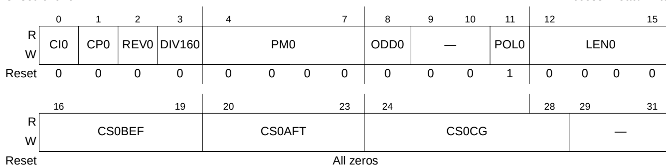
Figure 19-17. eSPI CS0 Mode Register (SPMODE0)
