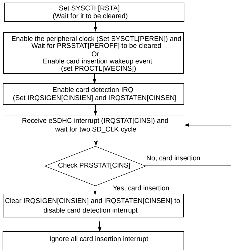
Figure 17-25. Flow Diagram for Card Detection
