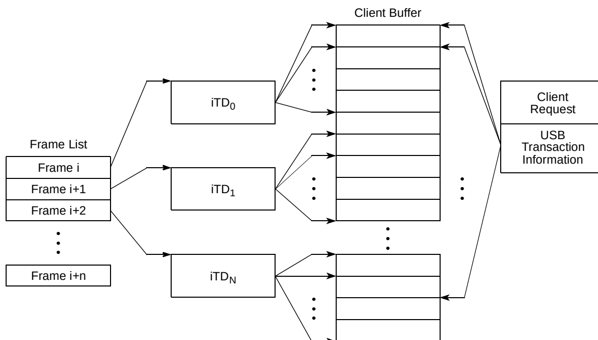
Figure 18-48. Example Association of iTDs to Client Request Buffer
