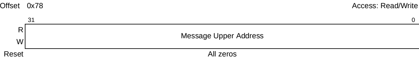
Figure 16-101. PCI Express MSI Message Upper Address Register
