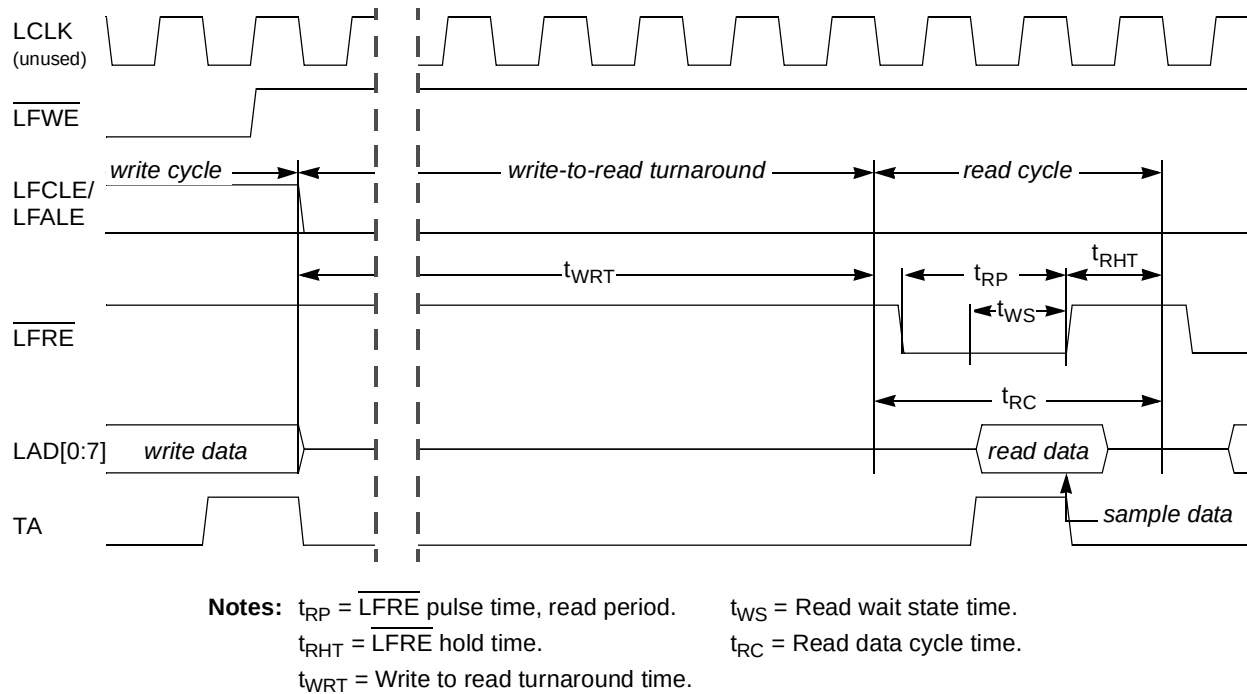
Figure 12-58. FCM Read Data Timing (for \text{TRLX} = 0 , \text{RST} = 0 , \text{SCY} = 1 )
