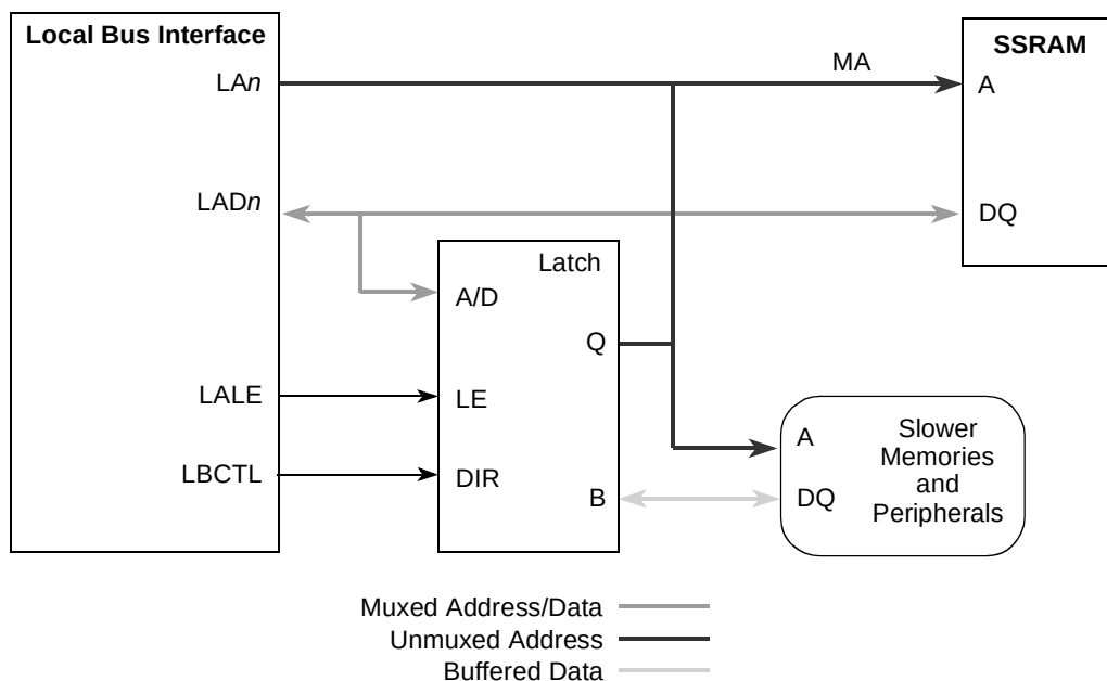
Figure 12-72. Local Bus Peripheral Hierarchy for High Bus Speeds
