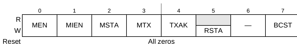
Figure 10-4. I 2 C Control Register (I2CCR)
