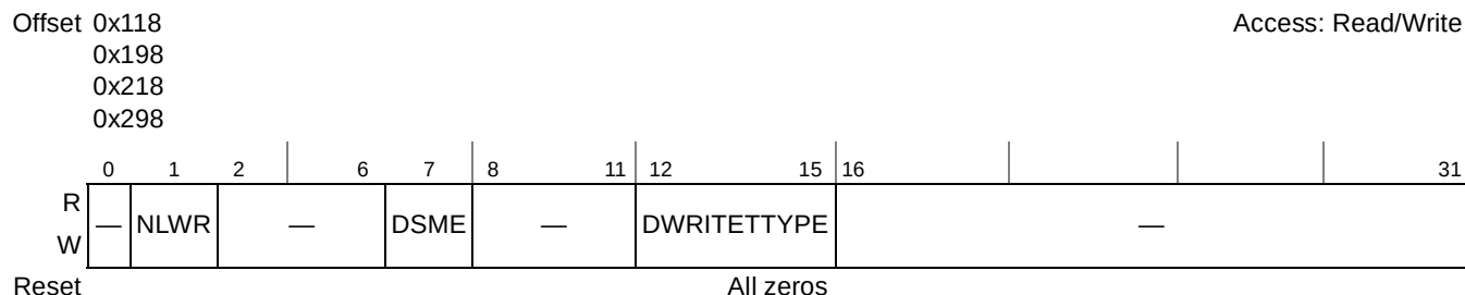
Figure 13-11. Destination Attributes Registers (DATR n )
