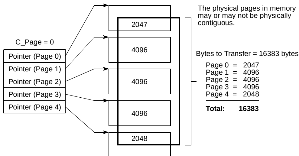
Figure 18-51. Example Mapping of qTD Buffer Pointers to Buffer Pages
