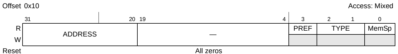
Figure 16-61. PCI Express Base Address Register 0 (PEXCSRBAR)
