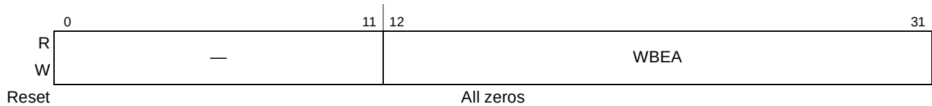
Figure 16-23. PCI Express Inbound Window Base Extended Address Registers (PEXIWBENr)
