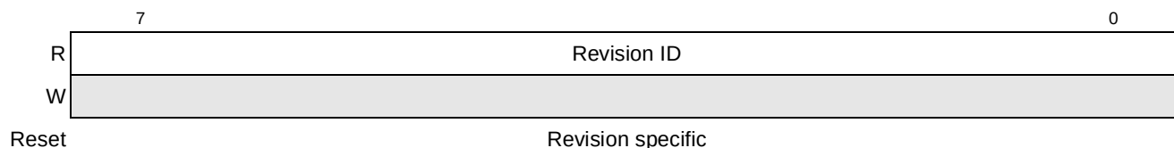
Figure 16-44. PCI Express Revision ID Register
