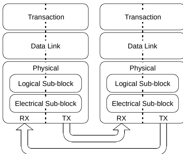
Figure 16-126. PCI Express High-Level Layering
