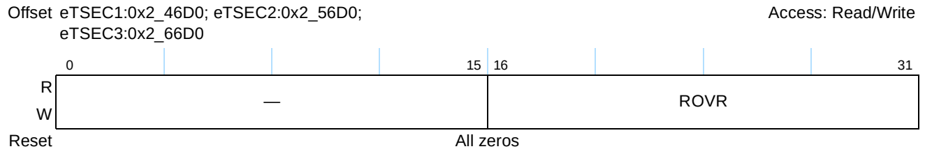
Figure 14-75. Receive Oversize Packet Counter Register Definition
