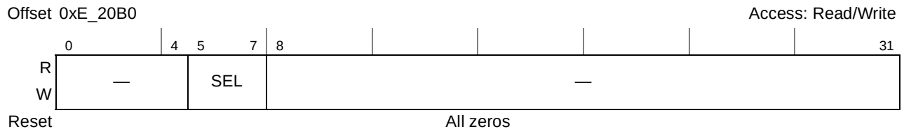
Figure 24-19. Trigger Out Source Register (TOSR)
