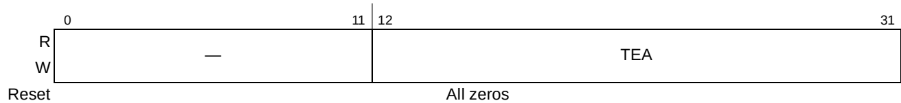
Figure 16-15. PCI Express Outbound Translation Extended Address Registers (PEXOTEAR n )
