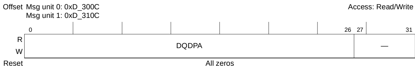
Figure 15-67. Outbound Message n Descriptor Queue Dequeue Pointer Address Registers (OM n DQDPAR)
