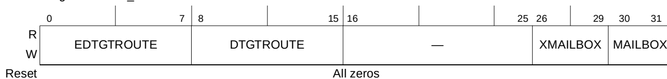
Figure 15-72. Outbound Message n Destination Port Registers (OMnDPR)
