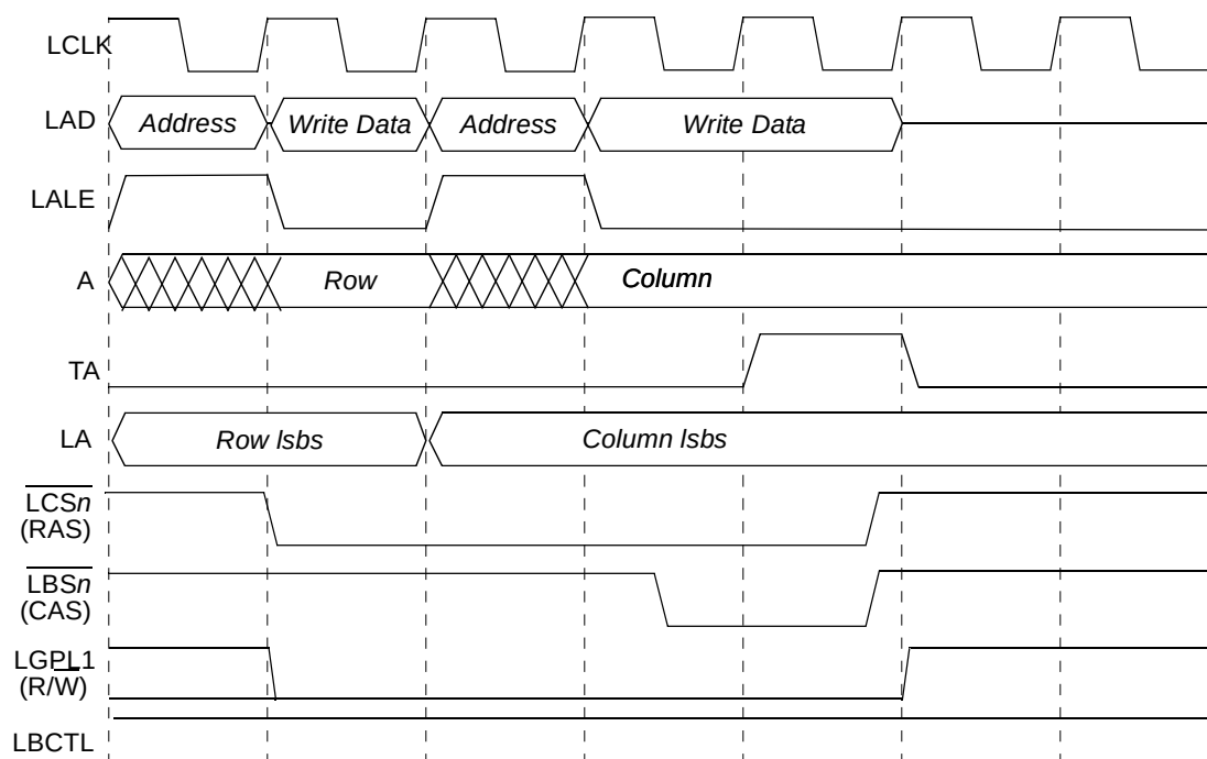
Figure 12-77. Single-Beat Write Access to FPM DRAM
