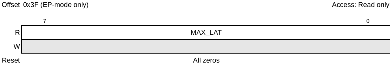
Figure 16-59. PCI Express Maximum Latency Register (MAX_LAT)
