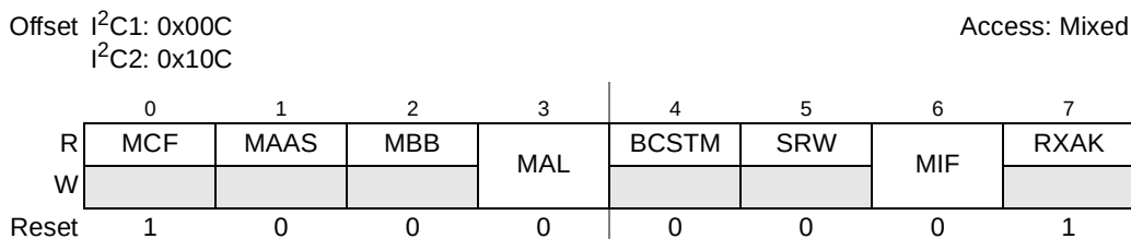
Figure 10-5. I 2 C Status Register (I2CSR)
