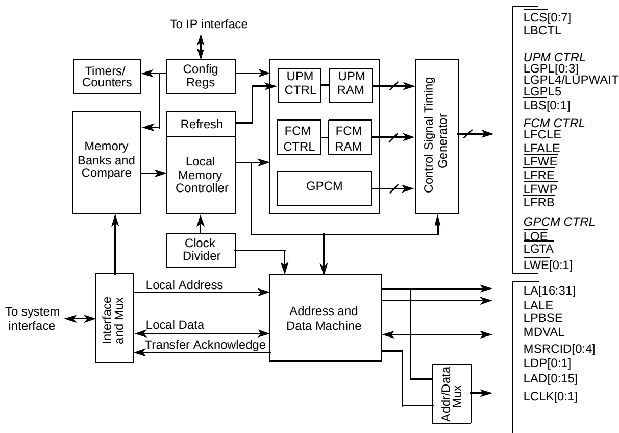
Figure 12-1. Enhanced Local Bus Controller Block Diagram
