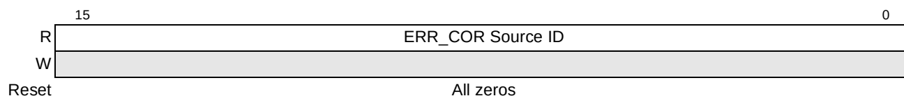
Figure 16-114. PCI Express Correctable Error Source ID Register
