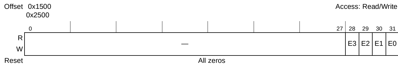
Figure 9-29. Message Enable Register (MER)
