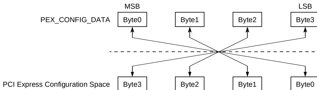
Figure 16-132. PEX_CONFIG_DATA Byte Ordering
