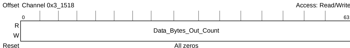
Figure 20-10. Data Bytes Out Counter
