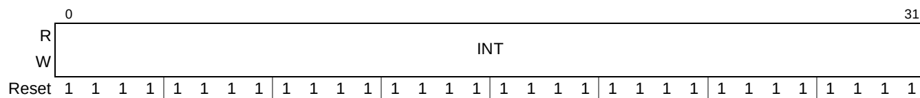
Figure 9-27. Performance Monitor Mask Registers 2 (PMnMR2)
