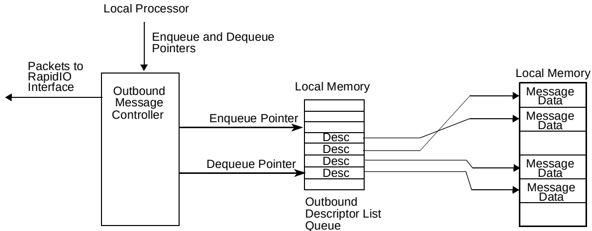
Figure 15-101. Outbound Frame Queue Structure
