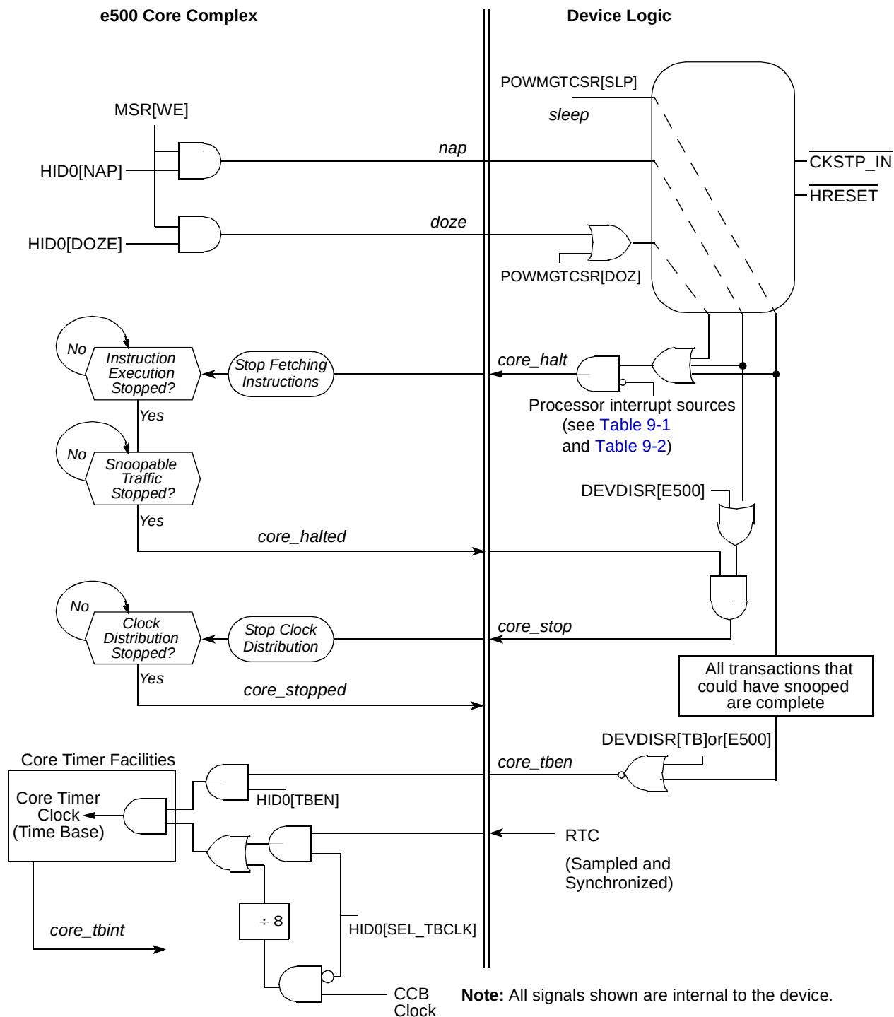
Figure 22-30. P2020 Power Management Handshaking Signals
