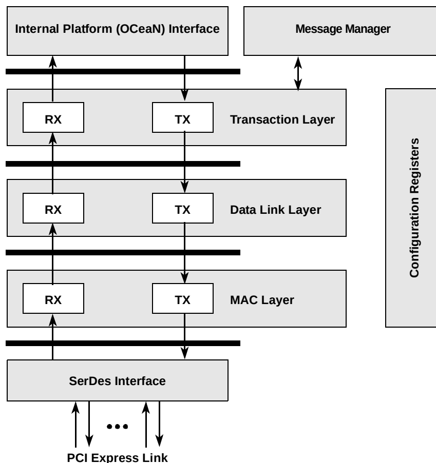
Figure 16-1. PCI Express Controller Block Diagram
