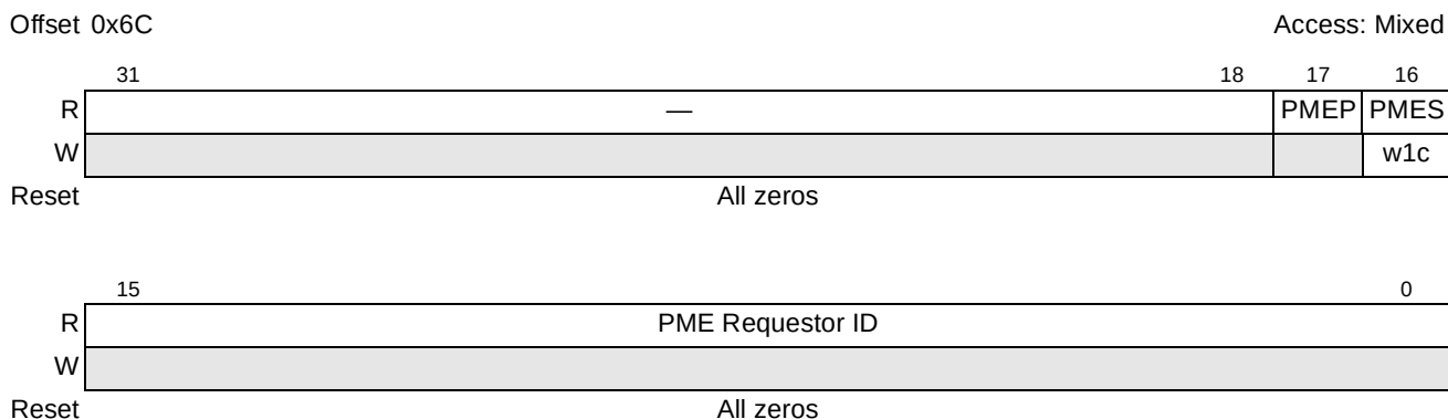
Figure 16-97. PCI Express Root Status Register
