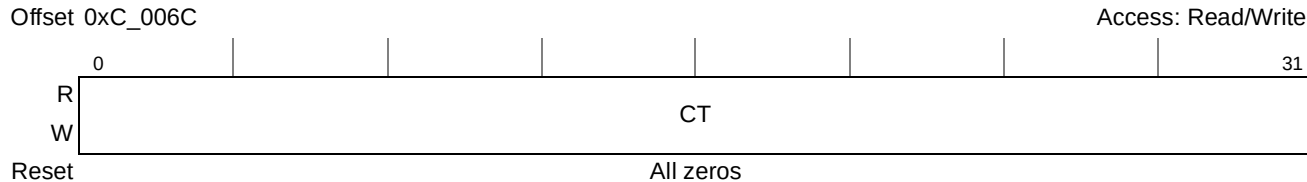
Figure 15-15. Component Tag Command and Status Register (CTCSR)
