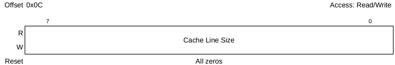
Figure 16-46. PCI Express Bus Cache Line Size Register
