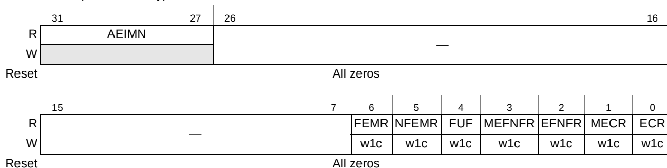
Figure 16-113. PCI Express Root Error Status Register
