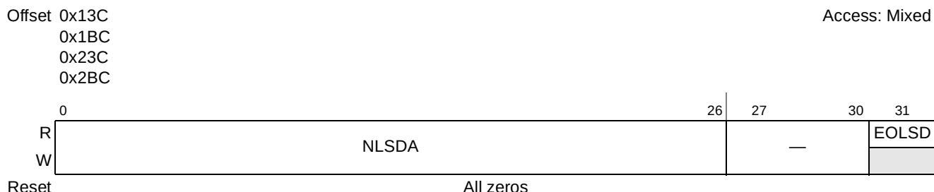
Figure 13-19. Next List Descriptor Address Registers (NLSDAR n )
