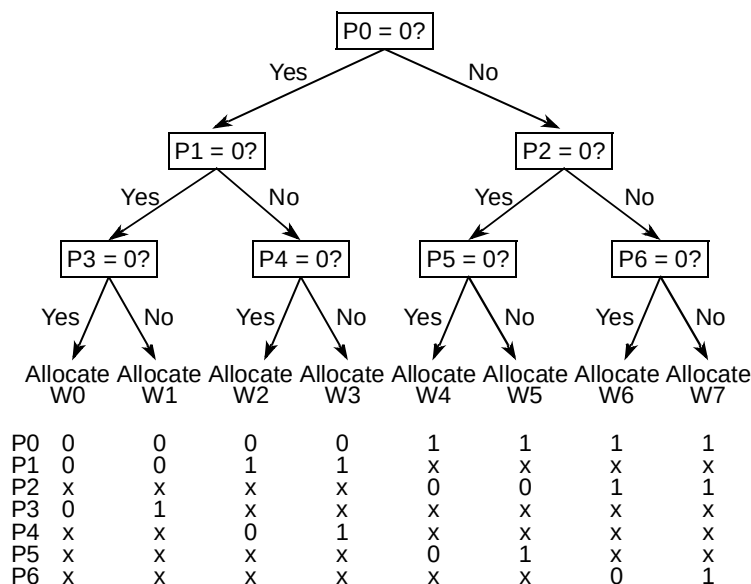
Figure 6-27. L2 Cache Line Replacement Algorithm
