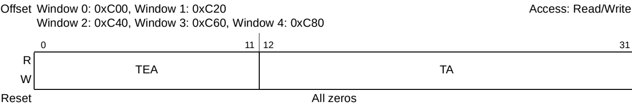
Figure 16-14. PCI Express Outbound Translation Address Registers (PEXOTAR n )
