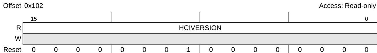
Figure 18-4. Host Controller Interface Version (HCVERSION)
