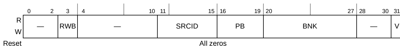
Figure 12-16. Transfer Error Attributes Register (LTEATR)
