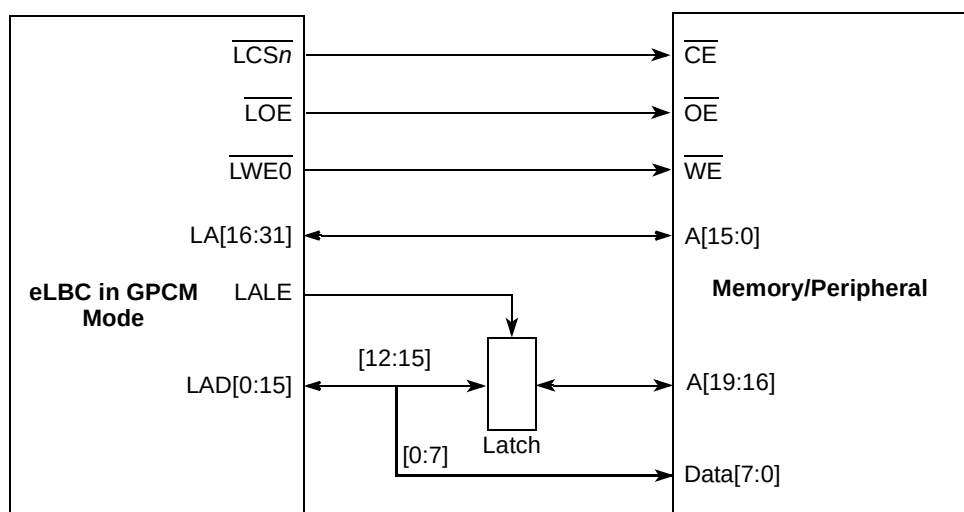
Figure 12-33. Enhanced Local Bus to GPCM Device Interface
