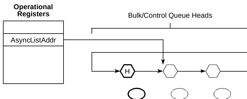
Figure 18-37. Asynchronous Schedule Organization
