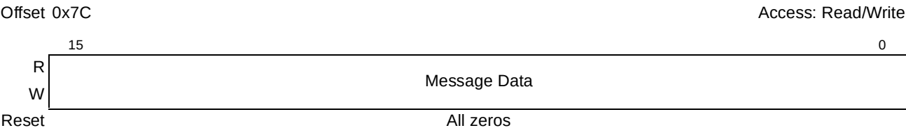
Figure 16-102. PCI Express MSI Message Data Register
