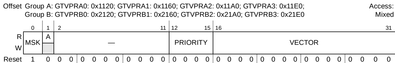
Figure 9-14. Global Timer Vector/Priority Register (GTVPR xn )
