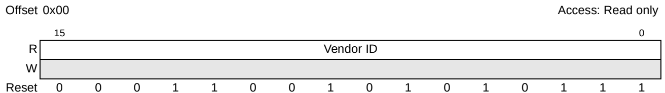
Figure 16-40. PCI Express Vendor ID Register
