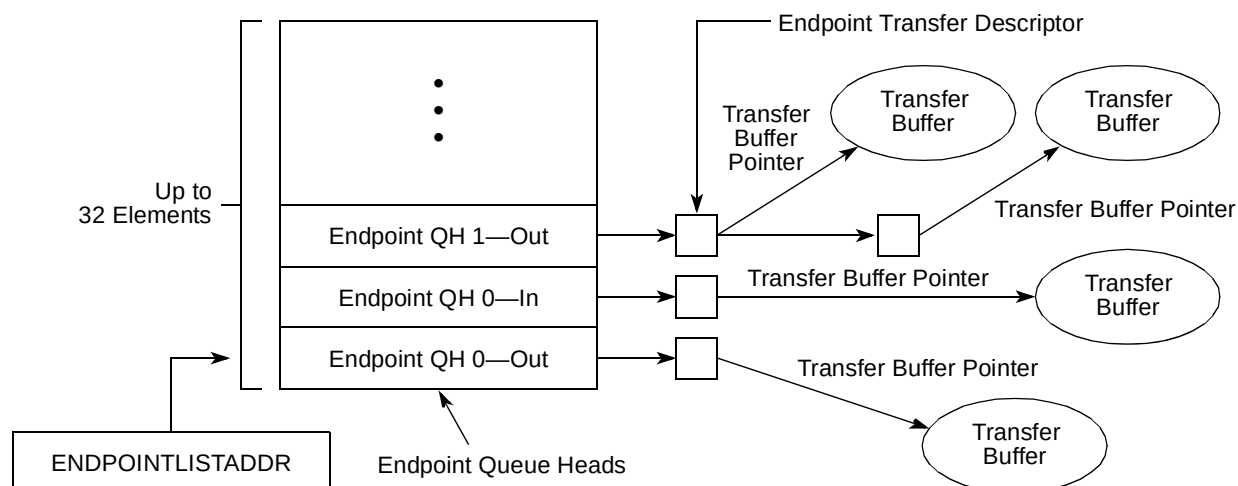
Figure 18-60. Endpoint Queue Head Organization
