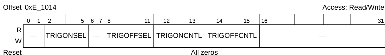
Figure 23-5. Performance Monitor Local Control Register B0 (PMLCB0)
