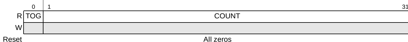
Figure 9-12. Global Timer Current Count Registers (GTCCR xn )
