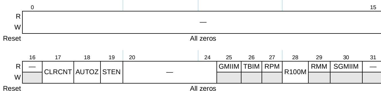
Figure 14-7. ECNTRL Register Definition
