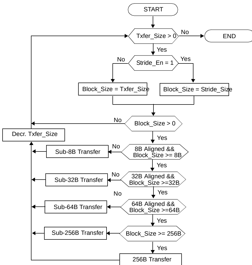
Figure 13-23. Source/Destination Engine Transaction Size Flow Chart
