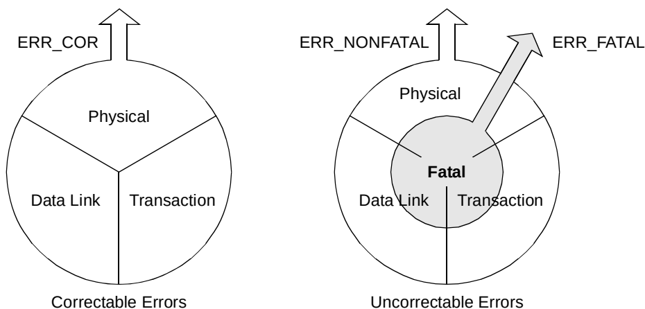
Figure 16-133. PCI Express Error Classification
