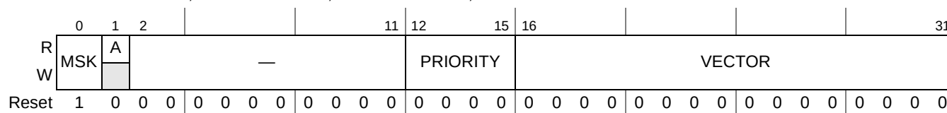
Figure 9-42. Messaging Interrupt Vector/Priority Registers (MIVPRn)
