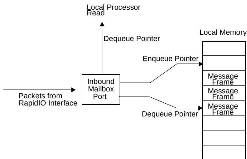
Figure 15-103. Inbound Message Structure
