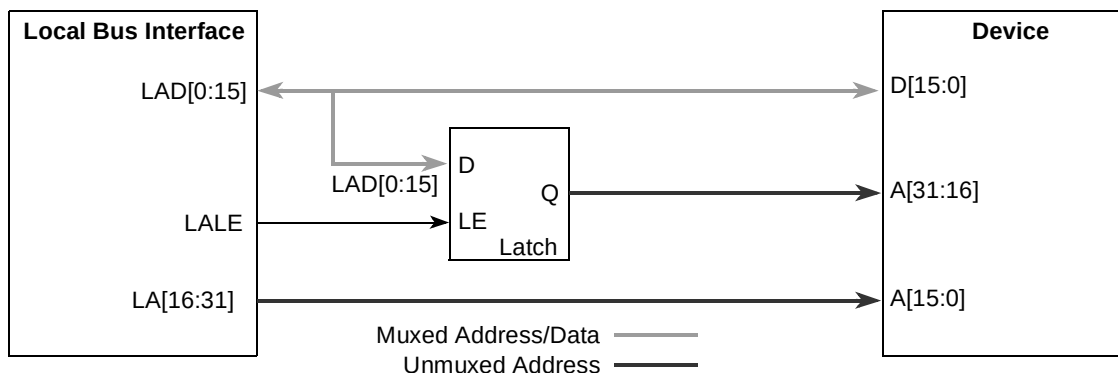
Figure 12-70. Multiplexed Address/Data Bus for 32-Bit Addressing
