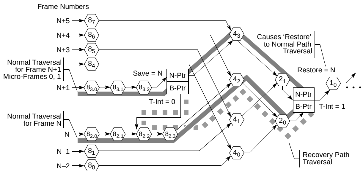
Figure 18-55. Example Host Controller Traversal of Recovery Path via FSTNs
