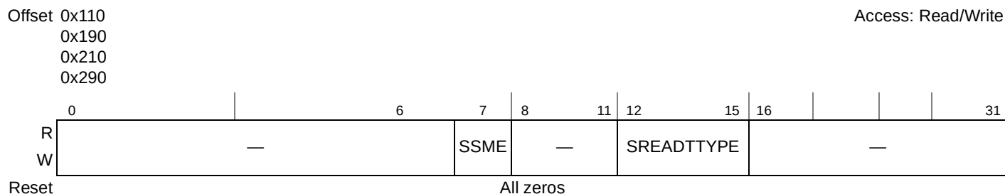
Figure 13-9. Source Attributes Registers (SATR n )
