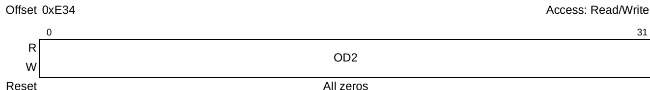
Figure 16-35. PCI Express Error Capture Register 3 (PEX_ERR_CAP_R3) Internal Source, Outbound Transaction
