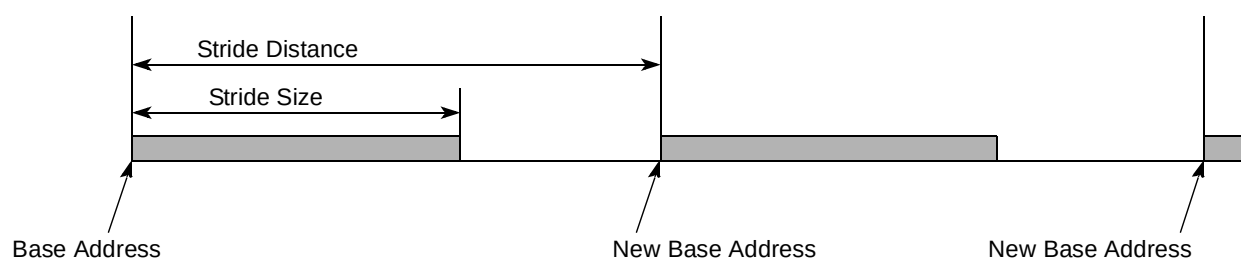
Figure 13-25. Stride Size and Stride Distance
