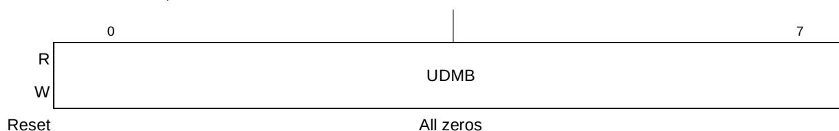
Figure 11-4. Divisor Most Significant Byte Registers (UDMB0, UDMB1)
