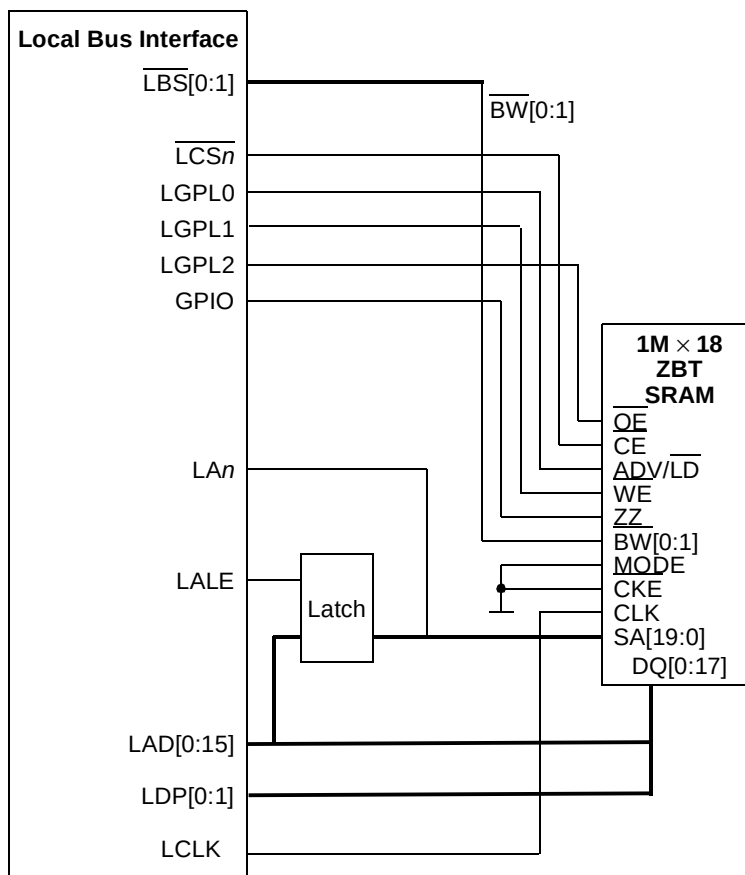
Figure 12-81. Interface to ZBT SRAM
