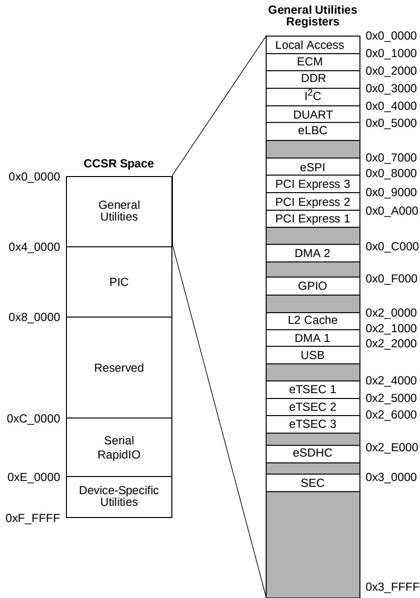
Figure 2-2. General Utilities Register Map within CCSR Space
