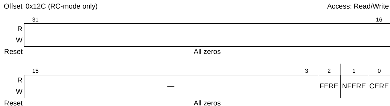
Figure 16-112. PCI Express Root Error Command Register
