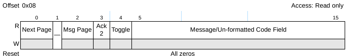
Figure 14-128. AN Link Partner Ability Next Page Register Definition
