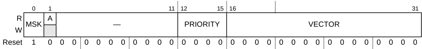
Figure 9-34. Shared Message Signaled Interrupt Vector/Priority Register (MSIVPRs)
