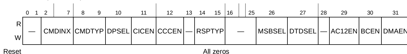
Figure 17-6. Transfer Type Register (XFERTYP)
