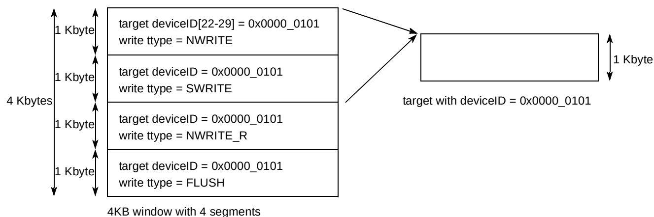
Figure 15-53. Example of Attribute Aliasing
