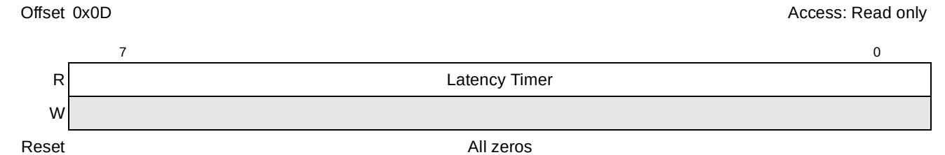
Figure 16-47. PCI Express Bus Latency Timer Register
