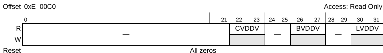
Figure 22-18. IO Voltage Select Status Register (IOVSELSR)
