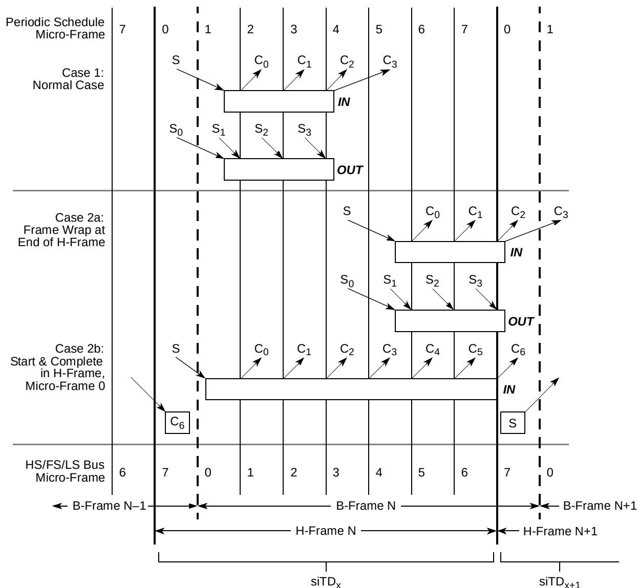
Figure 18-57. Split Transaction, Isochronous Scheduling Boundary Conditions
