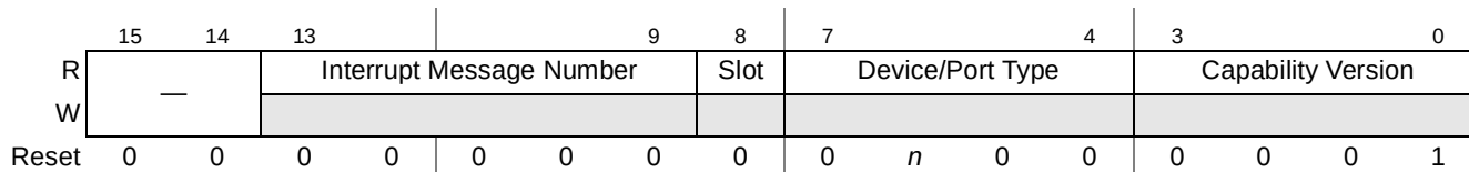
Figure 16-86. PCI Express Capabilities Register
