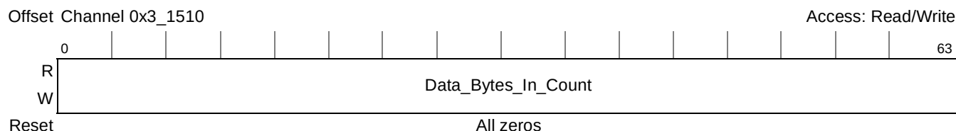
Figure 20-9. Data Bytes In Counter
