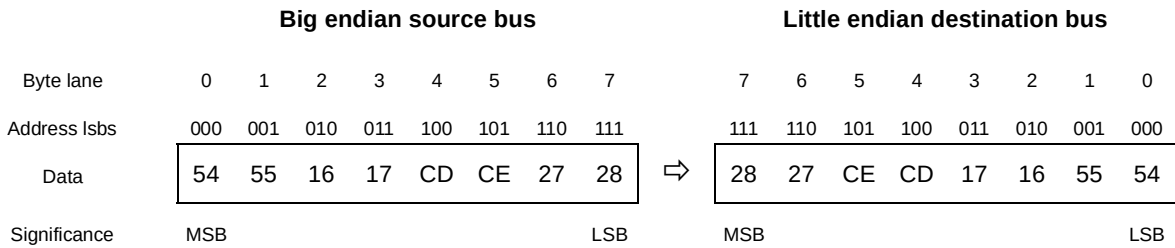
Figure 16-130. Address Invariant Byte Ordering—8 bytes Outbound
