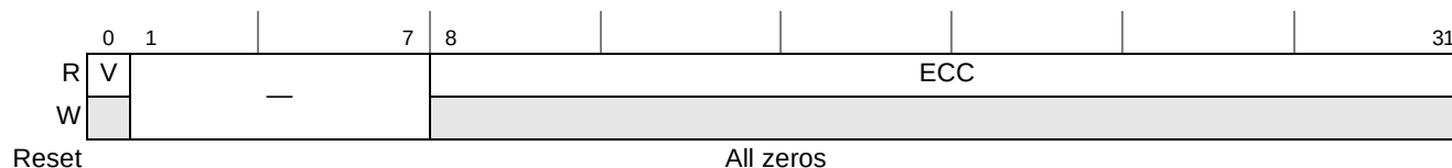
Figure 12-28. Flash ECC Block Register (FECC0-FECC3)
