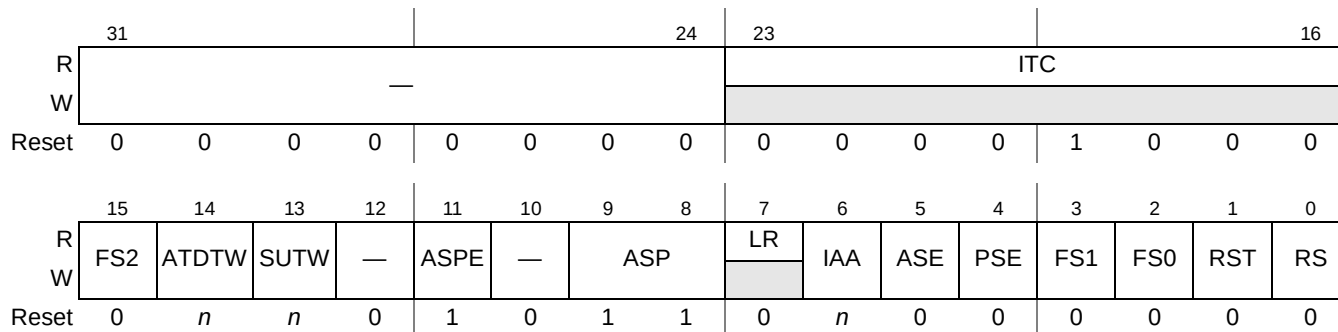
Figure 18-9. USB Command Register (USBCMD)
