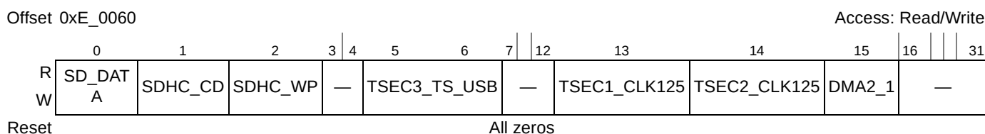
Figure 22-7. Alternate Function Pin Multiplex Control Register (PMUXCR)
