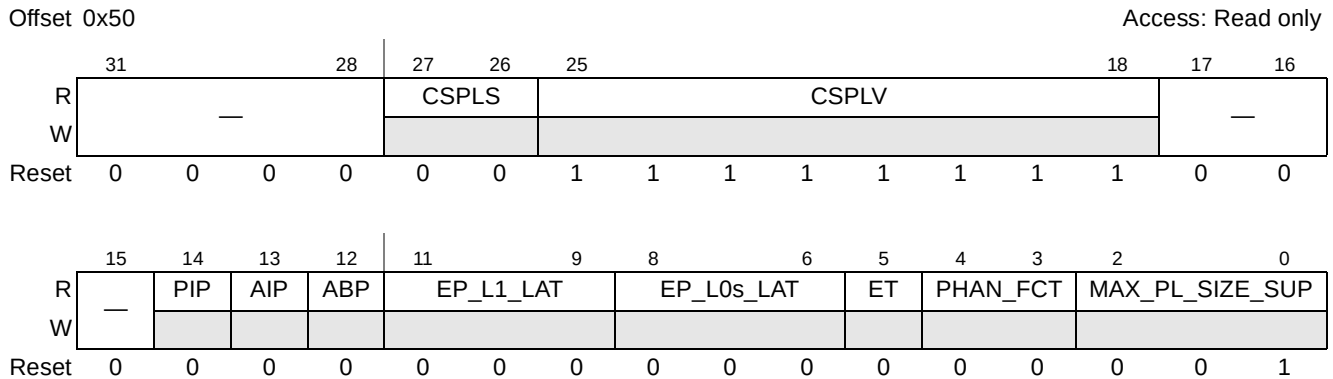
Figure 16-87. PCI Express Device Capabilities Register
