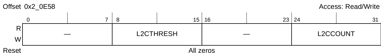
Figure 6-26. L2 Error Control Register (L2ERRCTL)
