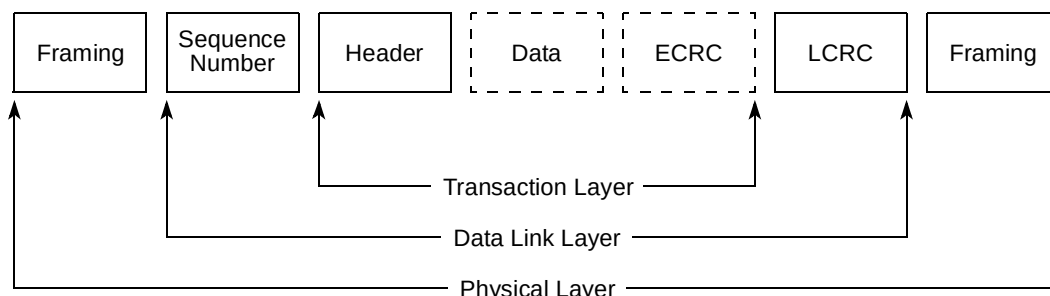
Figure 16-127. PCI Express Packet Flow
