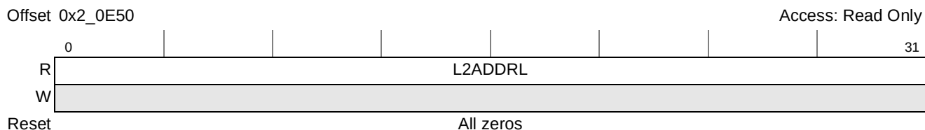
Figure 6-24. L2 Error Address Capture Register (L2ERRADDRL)
