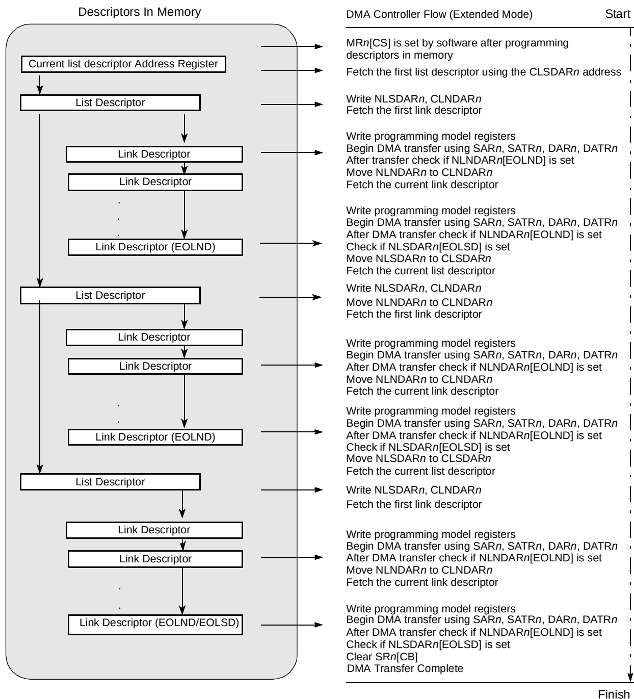
Figure 13-26. DMA Transaction Flow with DMA Descriptors
