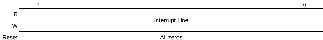
Figure 16-77. PCI Express Interrupt Line Register
