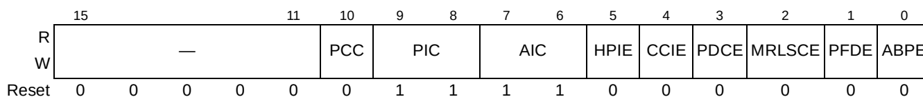
Figure 16-94. PCI Express Slot Control Register
