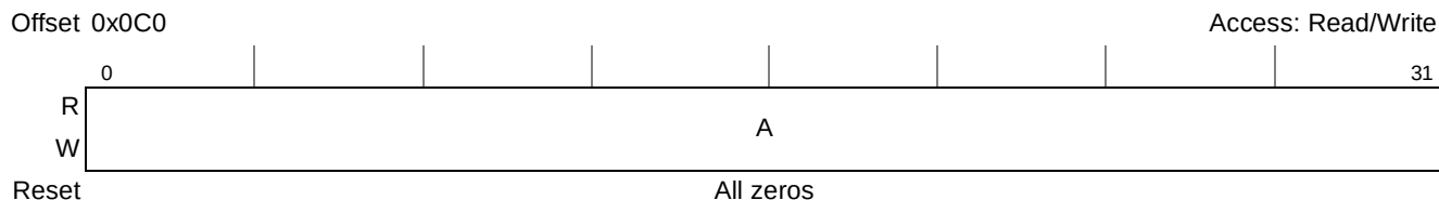
Figure 12-17. Transfer Error Address Register (LTEAR)
