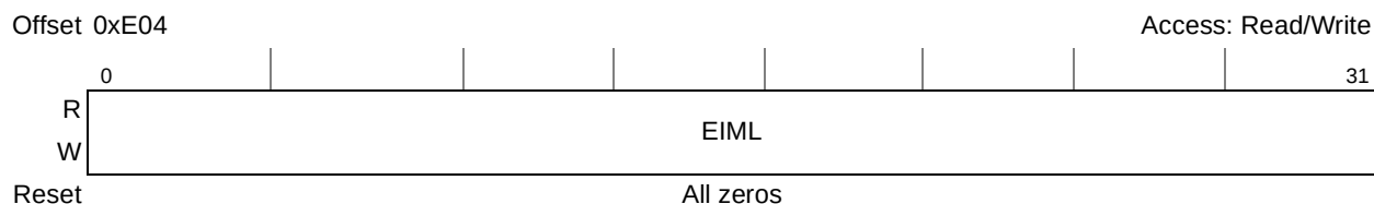
Figure 8-35. Memory Data Path Error Injection Mask Low Register (DATA_ERR_INJECT_LO)
