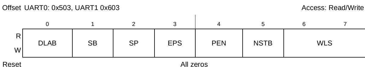
Figure 11-10. Line Control Register (ULCR)
