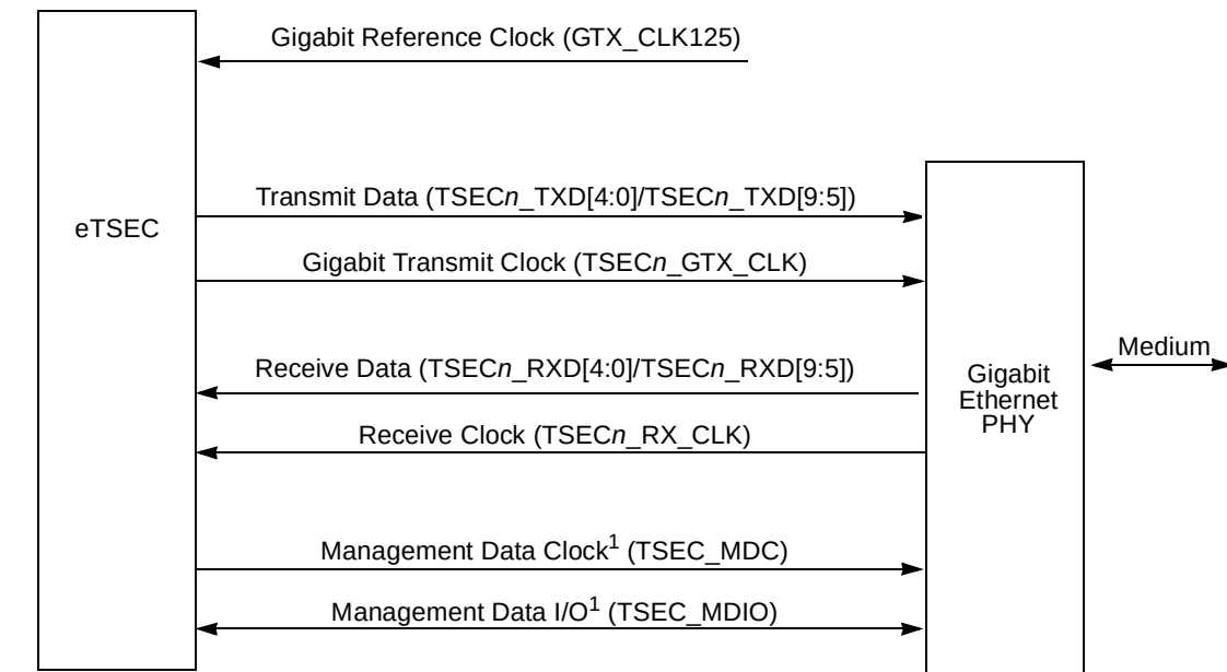
Figure 14-137. eTSEC-RTBI Connection
