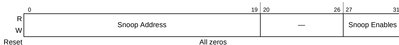
Figure 18-30. Snoop 1 and Snoop 2 (SNOOP n )
