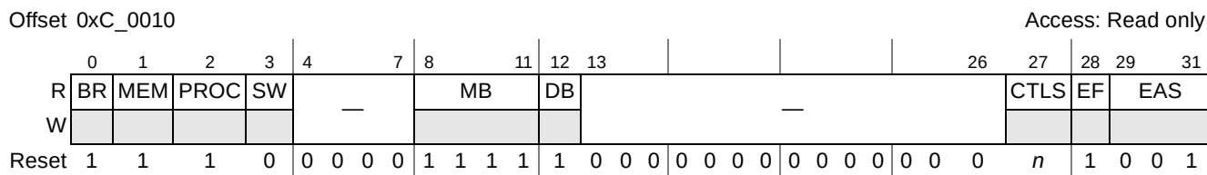
Figure 15-6. Processing Element Features Capability Register (PEFCAR)
