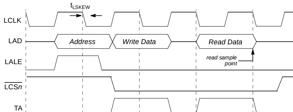
Figure 12-32. eLBC Bus Cycles in PLL-Bypassed Mode (GPCM and UPM only)
