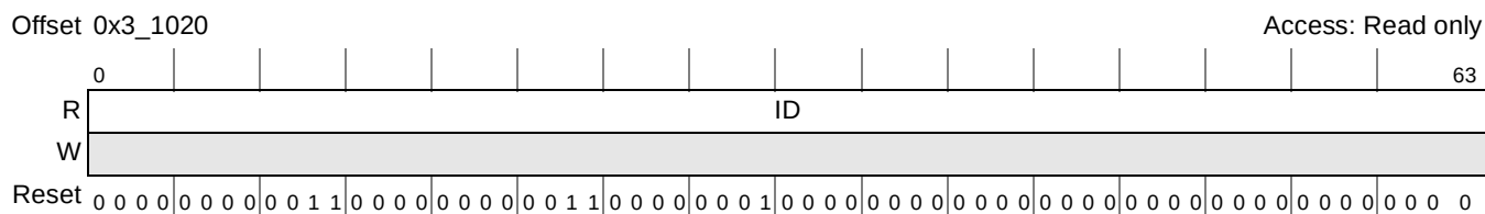
Figure 20-18. ID Register
