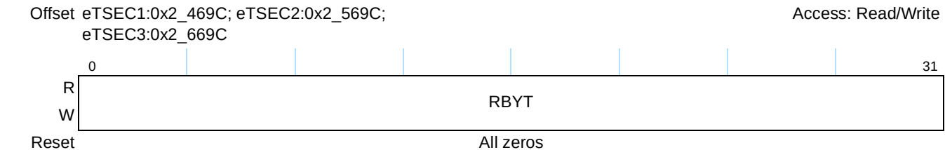
Figure 14-62. Receive Byte Counter Register Definition
