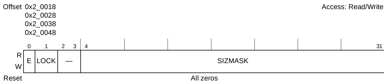
Figure 6-11. Cache External Write Control Registers (L2CEWCR0–L2CEWCR3)
