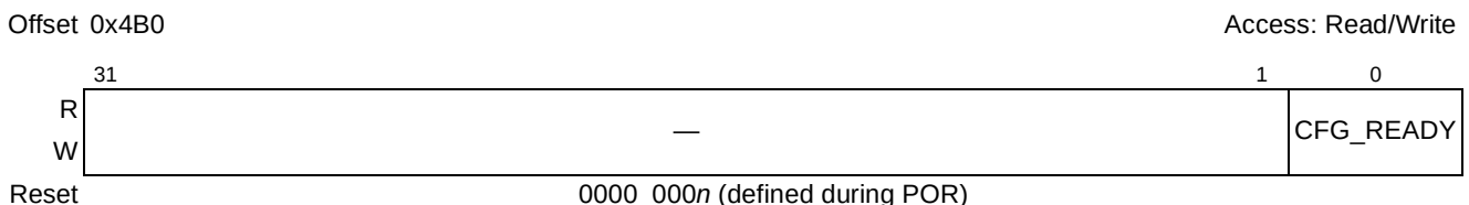
Figure 16-122. PCI Express Configuration Ready Register (PEX_CFG_READY)
