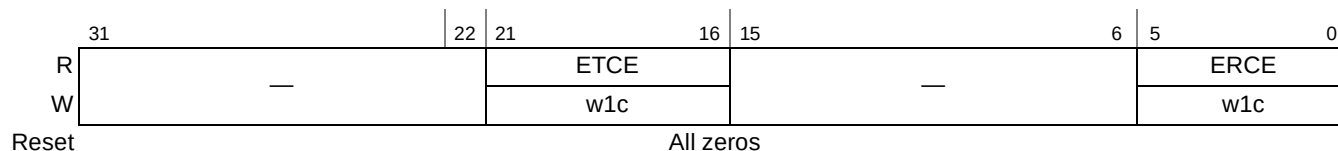
Figure 18-27. Endpoint Complete (ENDPTCOMPLETE)
