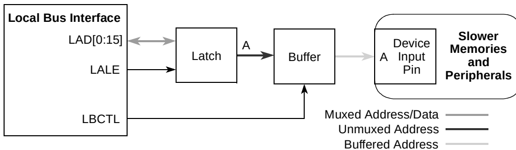
Figure 12-73. GPCM Address Timings
