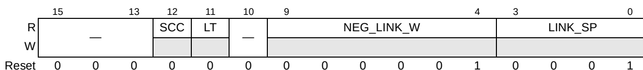
Figure 16-92. PCI Express Link Status Register
