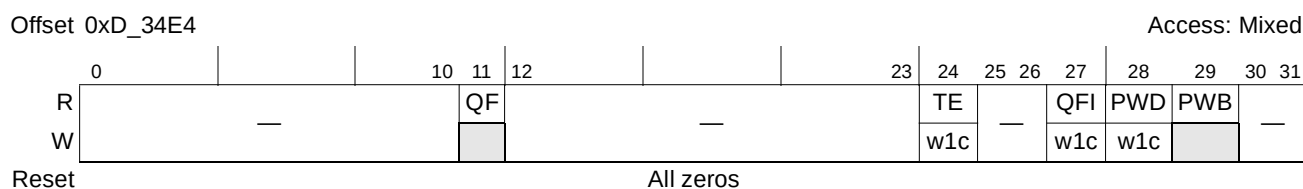
Figure 15-98. Inbound Port-Write Status Register (IPWSR)
