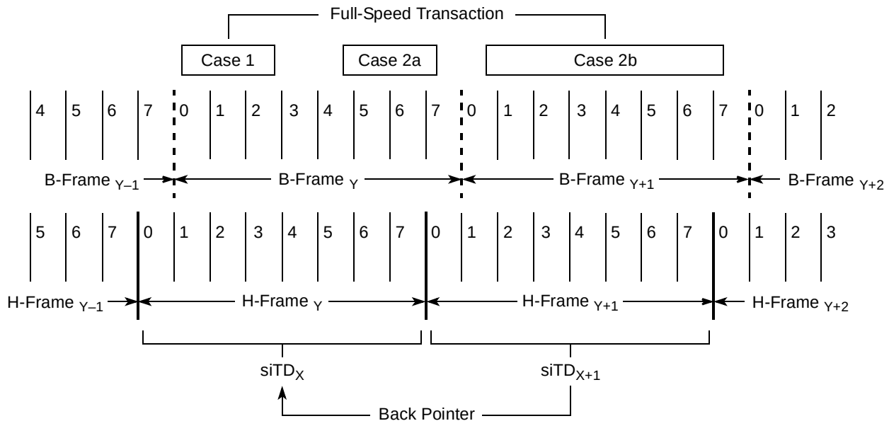
Figure 18-58. siTD Scheduling Boundary Examples
