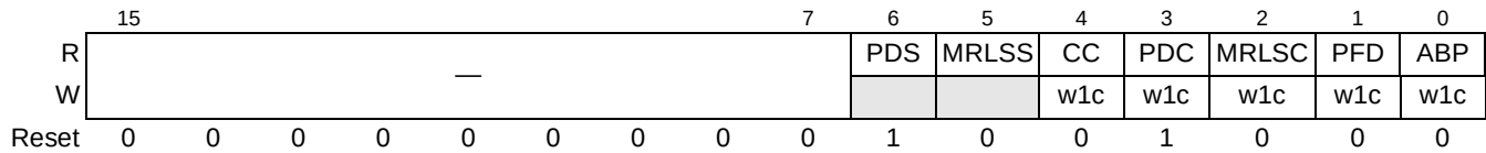
Figure 16-95. PCI Express Slot Status Register
