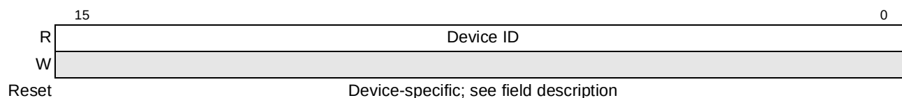
Figure 16-41. PCI Express Device ID Register
