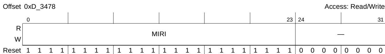
Figure 15-96. Inbound Doorbell Maximum Interrupt Report Interval Register (IDMIRIR)
