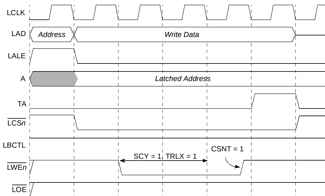
Figure 12-41. GPCM Relaxed Timing Write (XACS = 0, ACS = 00, SCY = 1, CSNT = 1, TRLX = 1)
