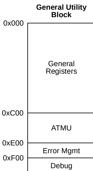
Figure 2-3. General Utility Register Block
