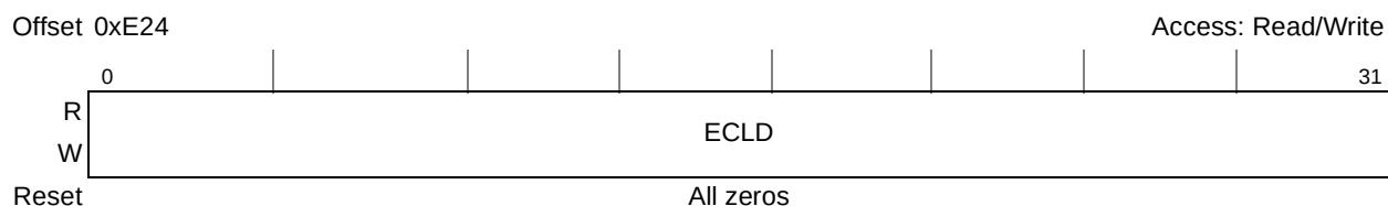
Figure 8-38. Memory Data Path Read Capture Low Register (CAPTURE_DATA_LO)
