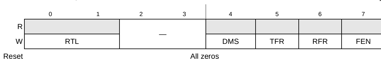
Figure 11-8. FIFO Control Registers (UFCR n )
