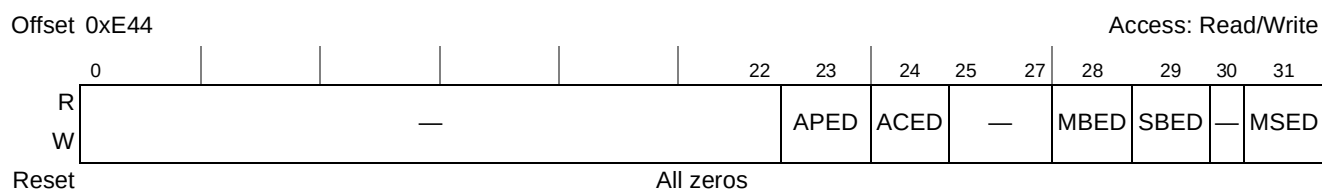
Figure 8-41. Memory Error Disable Register (ERR_DISABLE)
