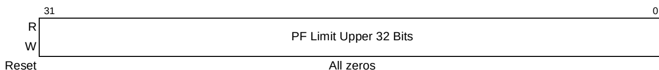
Figure 16-73. PCI Express Prefetchable Limit Upper 32 Bits Register
