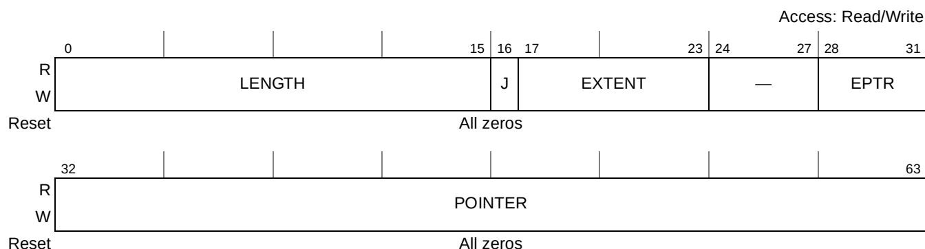
Figure 20-4. Pointer Dword
