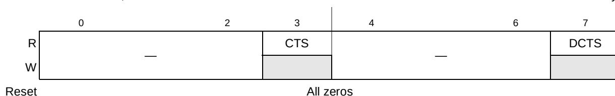
Figure 11-13. Modem Status Register (UMSR)
