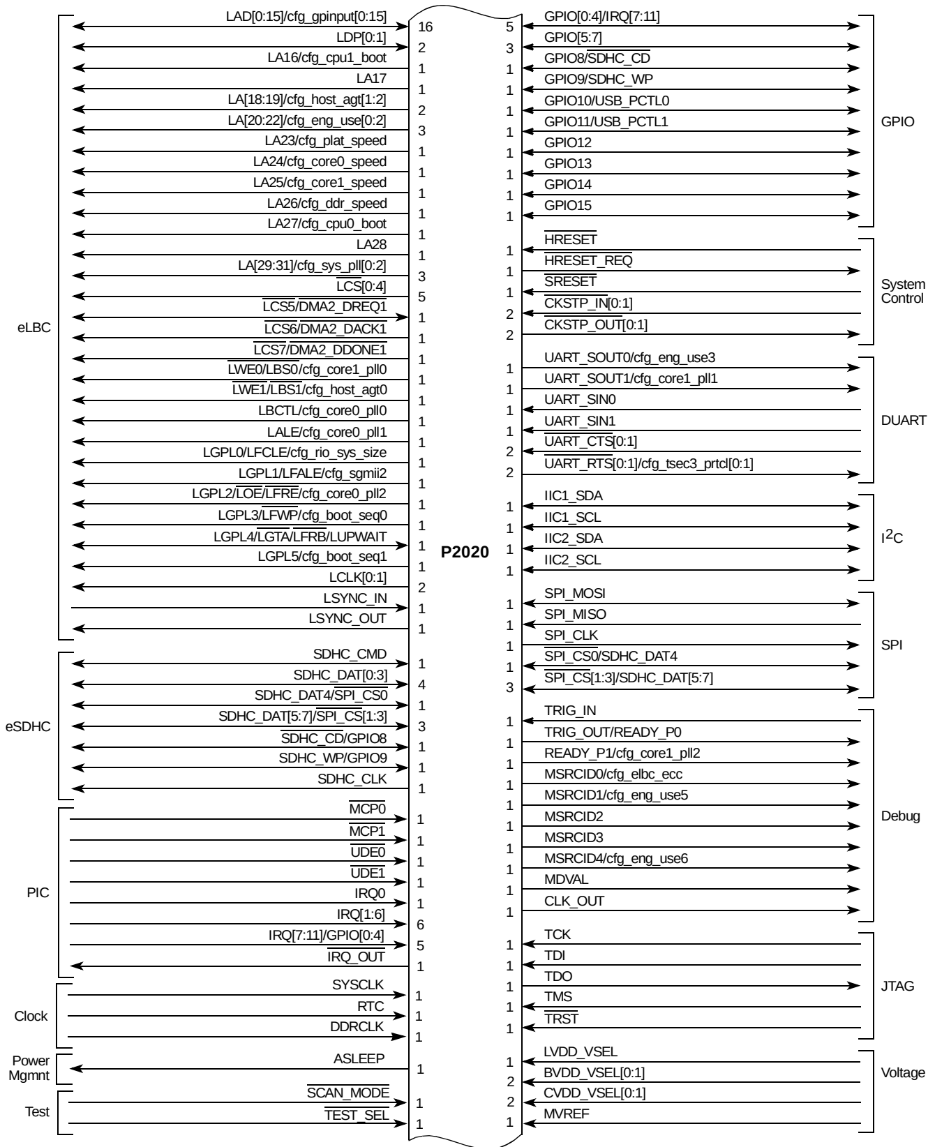
Figure 3-2. P2020 Signal Groupings (2/3) (Continued)
