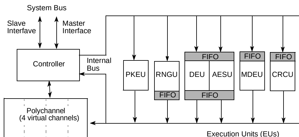
Figure 20-1. SEC Functional Modules
