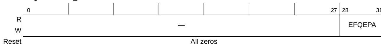
Figure 15-82. Extended Inbound Message n Frame Queue Enqueue Pointer Address Registers (EIM n FQEPAR)
