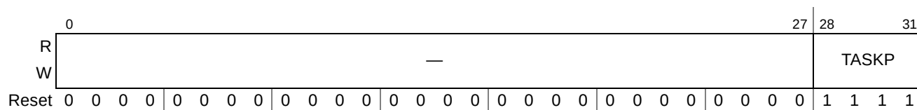
Figure 9-46. Processor Core Current Task Priority Registers (CTPR n )
