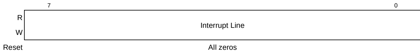
Figure 16-56. PCI Express Interrupt Line Register
