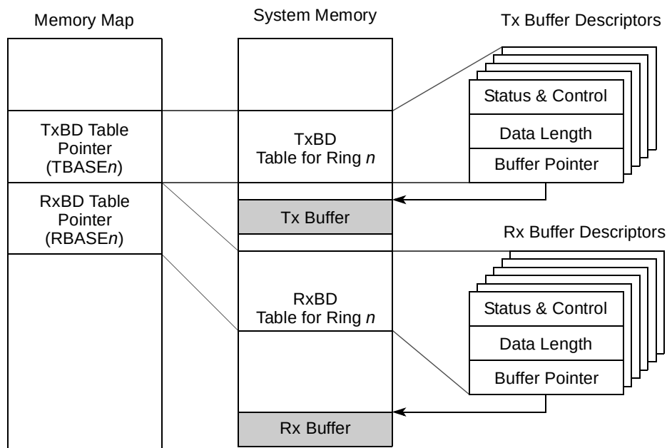
Figure 14-153. Example of eTSEC Memory Structure for BDs
