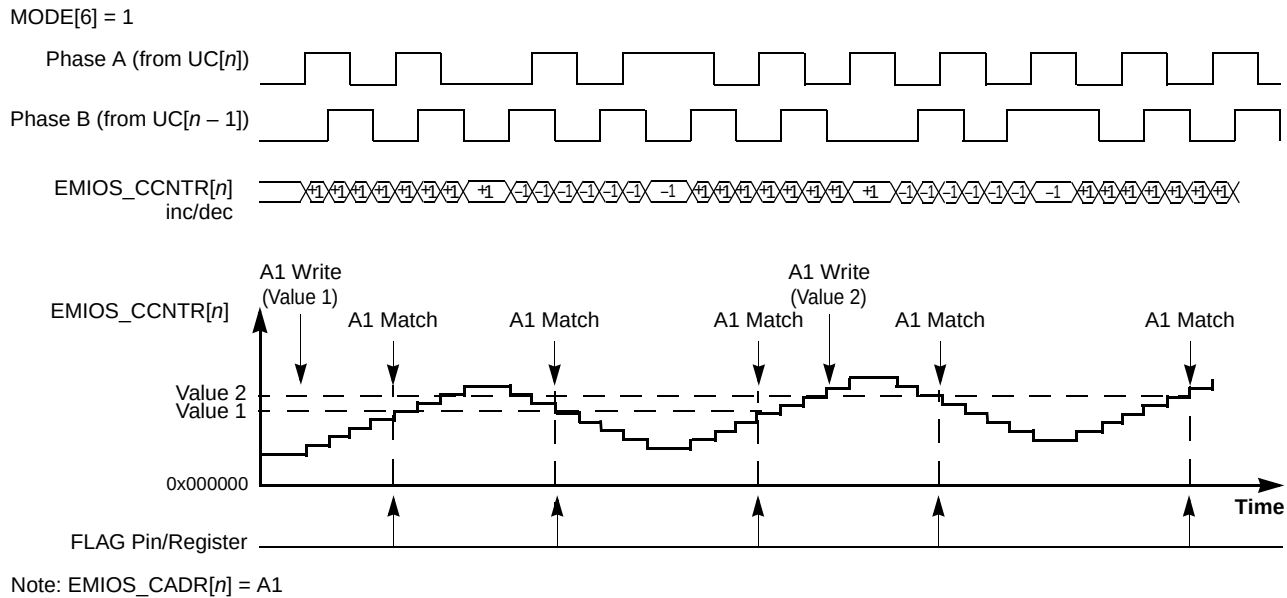
Figure 22-30. QDEC Example with Phase_A & Phase_B Encoder
