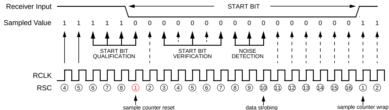
Figure 25-32. Start Bit Sampling and Strobing
