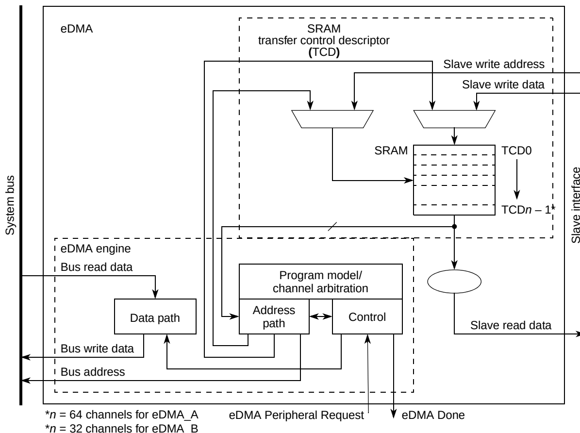
Figure 20-1. eDMA Block Diagram
