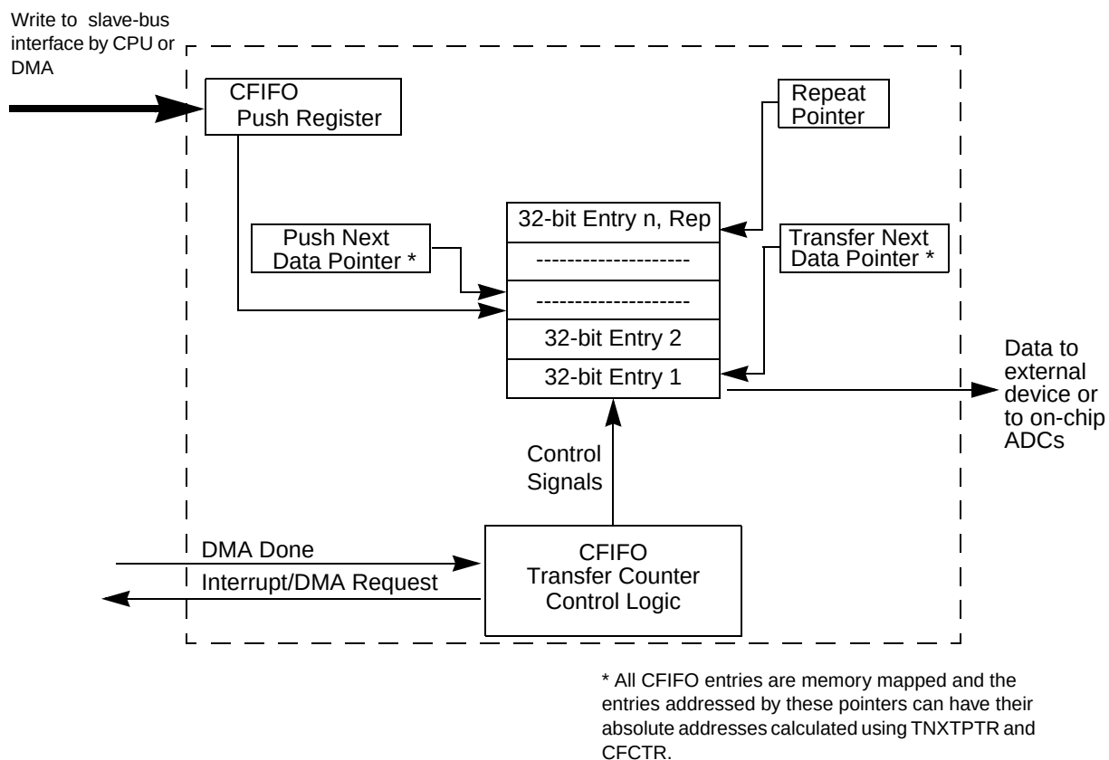
Figure 26-52. CFIFO0 in Streaming Mode Diagram
