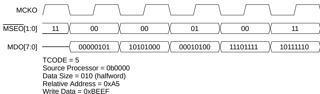
Figure 30-34. Data Trace—Data Write Message
