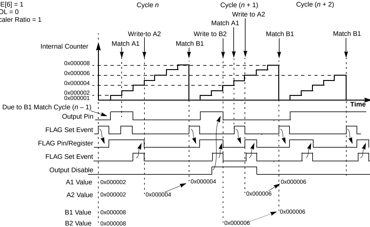
Figure 22-43. OPWFMB Mode with Active Output Disable
