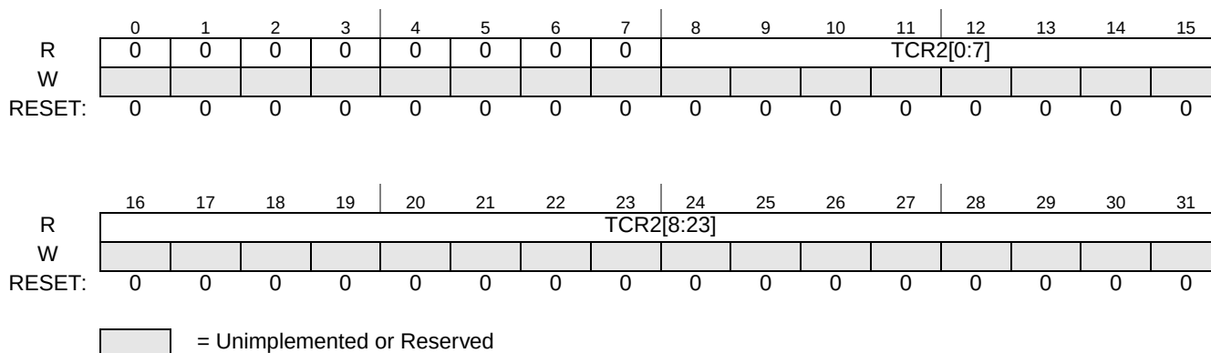
Figure 28-10. ETPUTB2R Register
