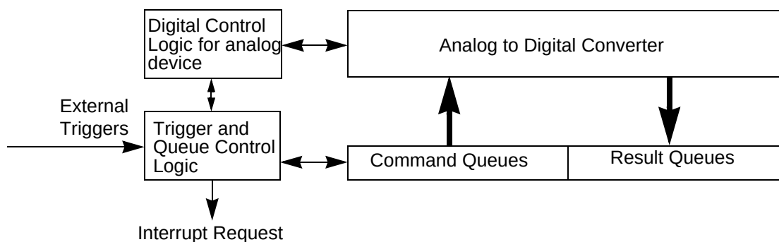
Figure 26-79. QADC Overview
