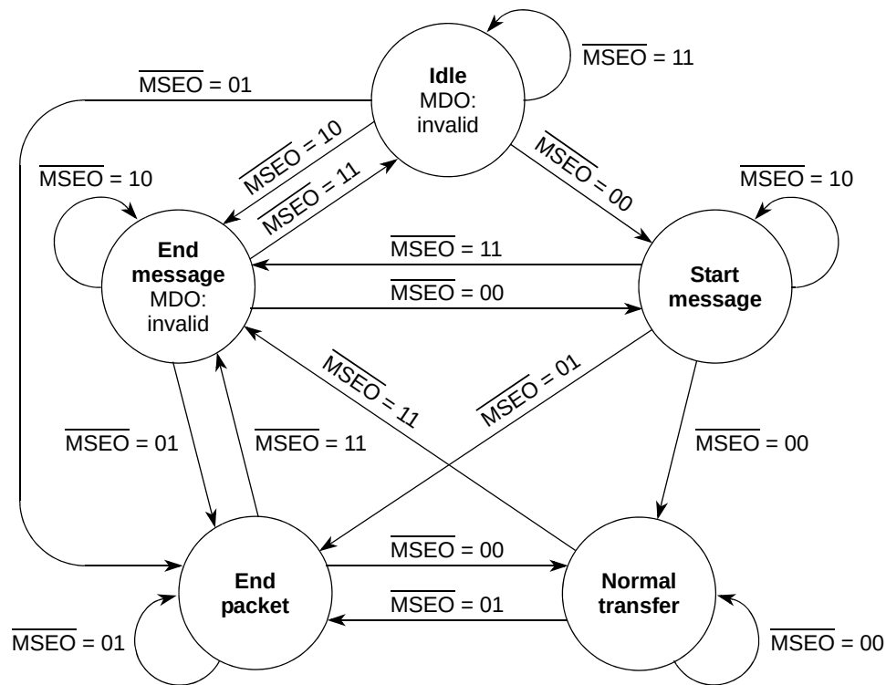
Figure 30-5. \overline{\text{MSEO}} Transfers
