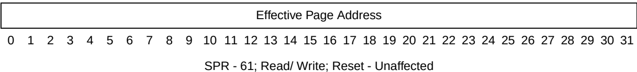
Figure 12-5. DEAR
