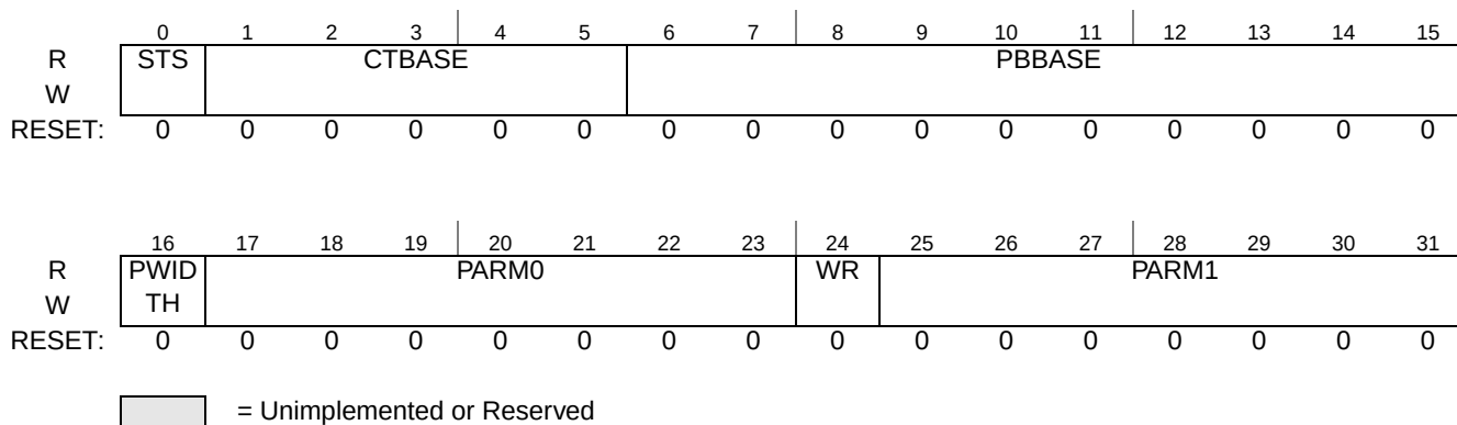
Figure 28-4. ETPUCDCR Register
