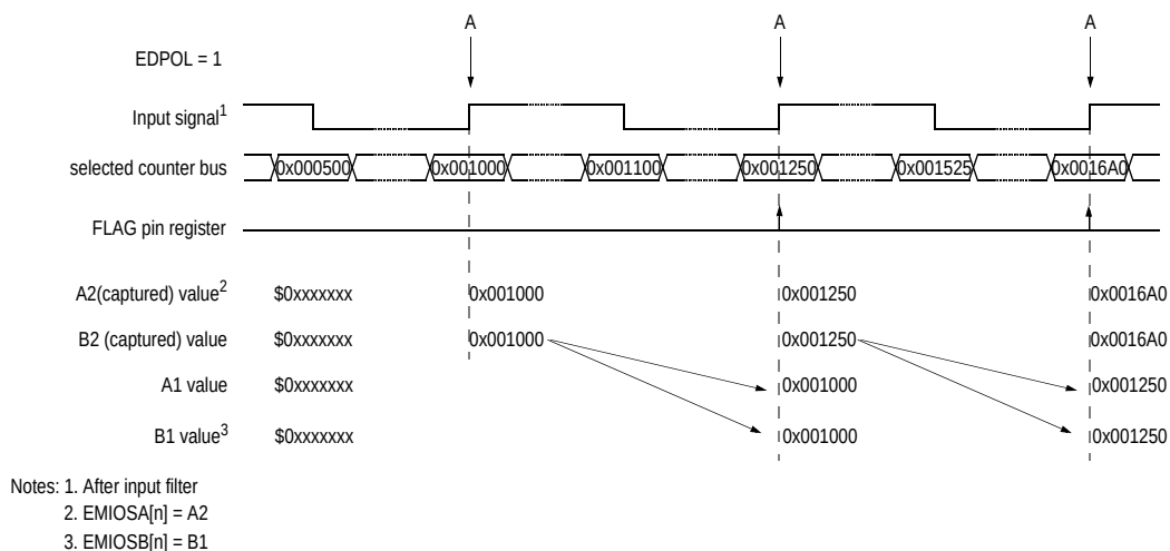
Figure 22-20. IPM Example
