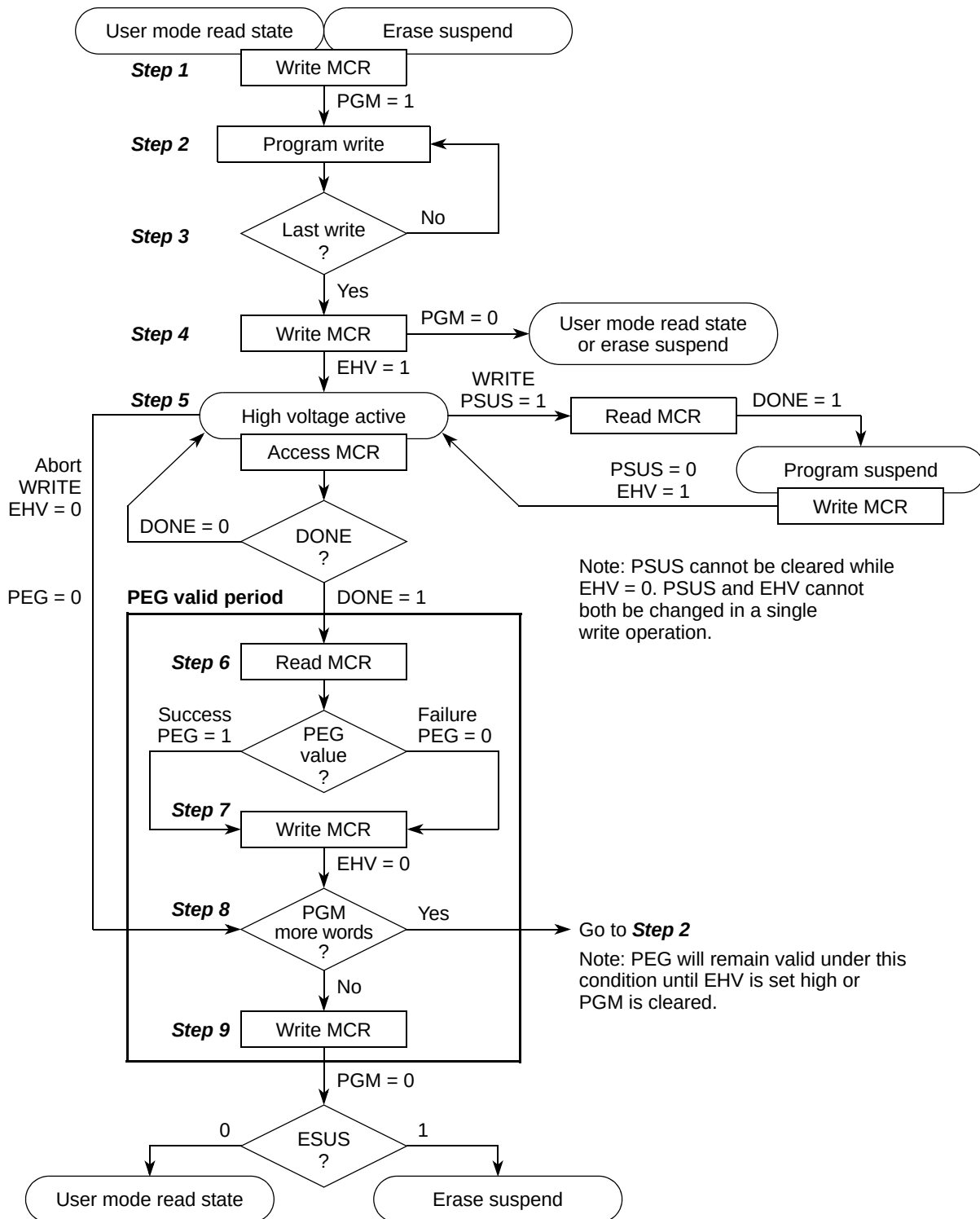
Figure 11-17. Program Sequence
