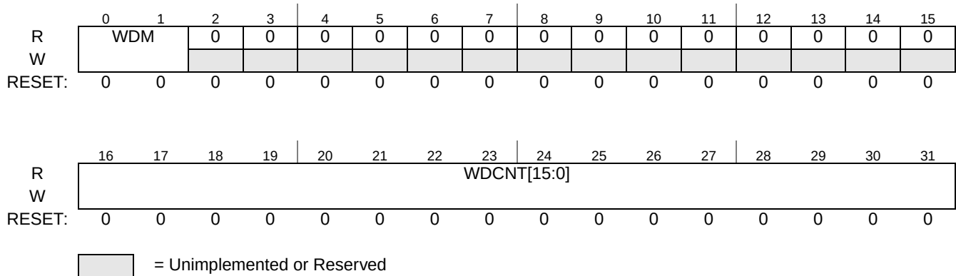
Figure 28-12. ETPUWDTR Register
