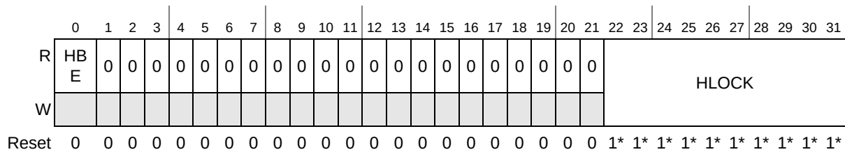
Figure 11-5. FLASH_x_HLR Register
