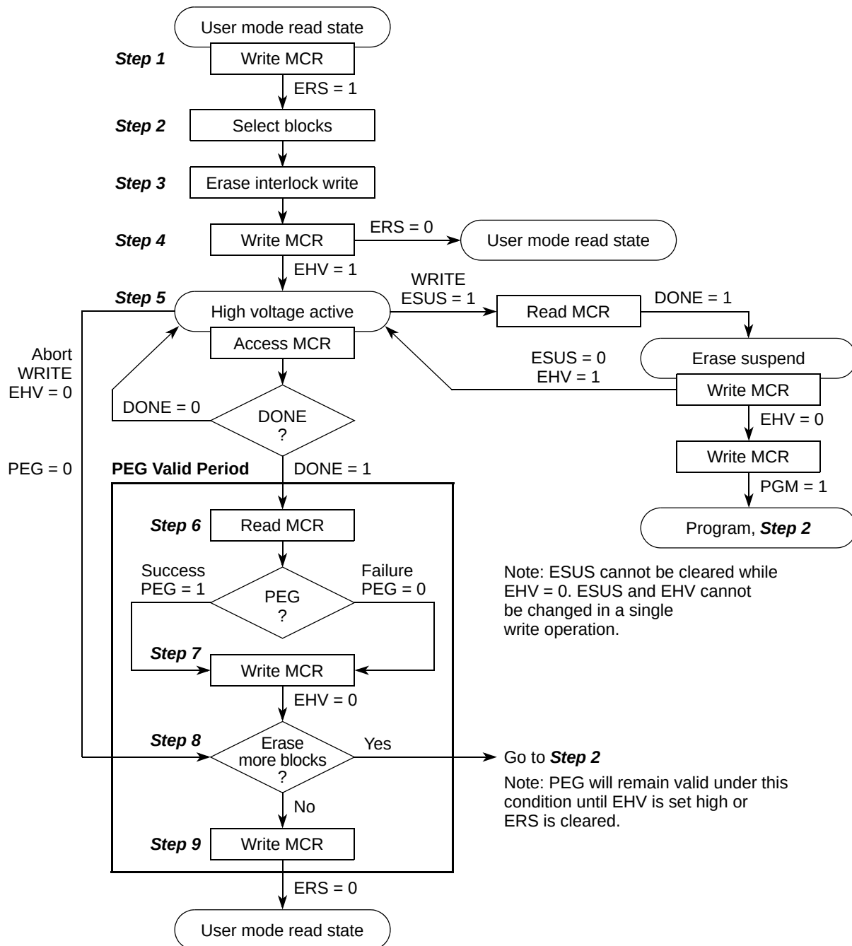
Figure 11-18. Erase Sequence
