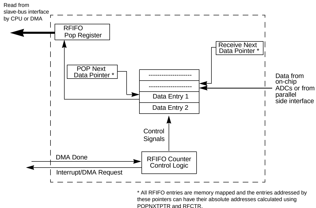
Figure 26-61. RFIFO Diagram
