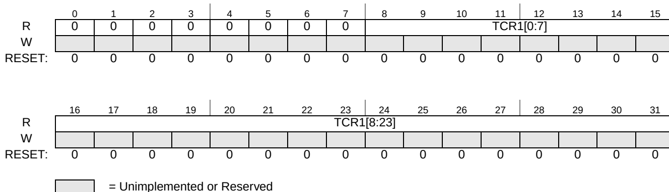
Figure 28-9. ETPUTB1R Register
