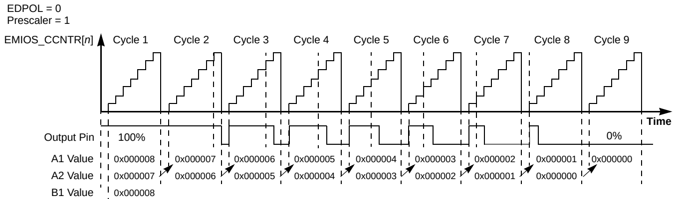
Figure 22-44. OPWFMB Mode from 100% to 0% Duty Cycle
