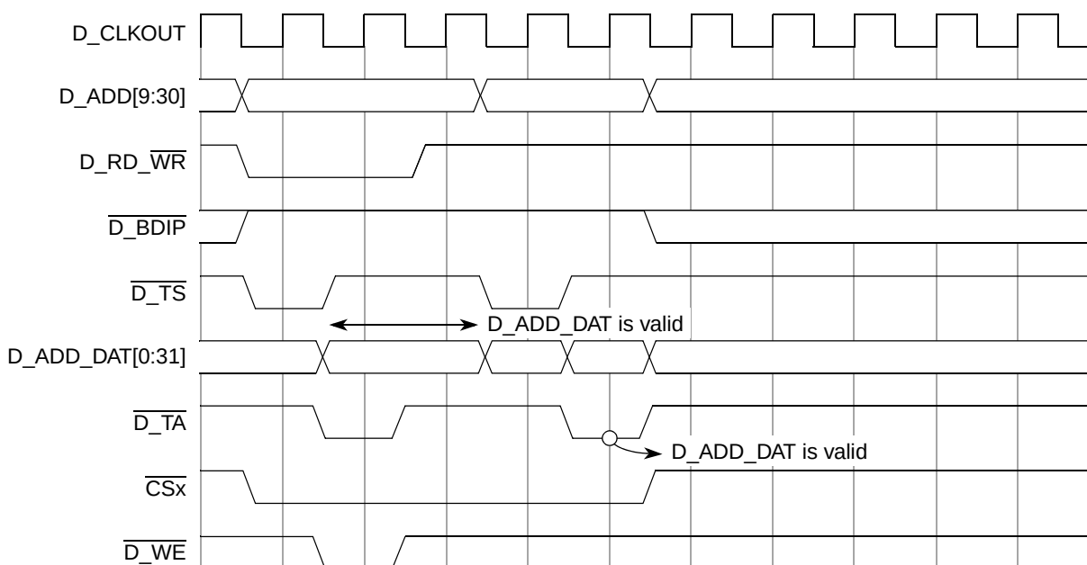
Figure 29-21. Read After Write to the Same \overline{CS} Bank
