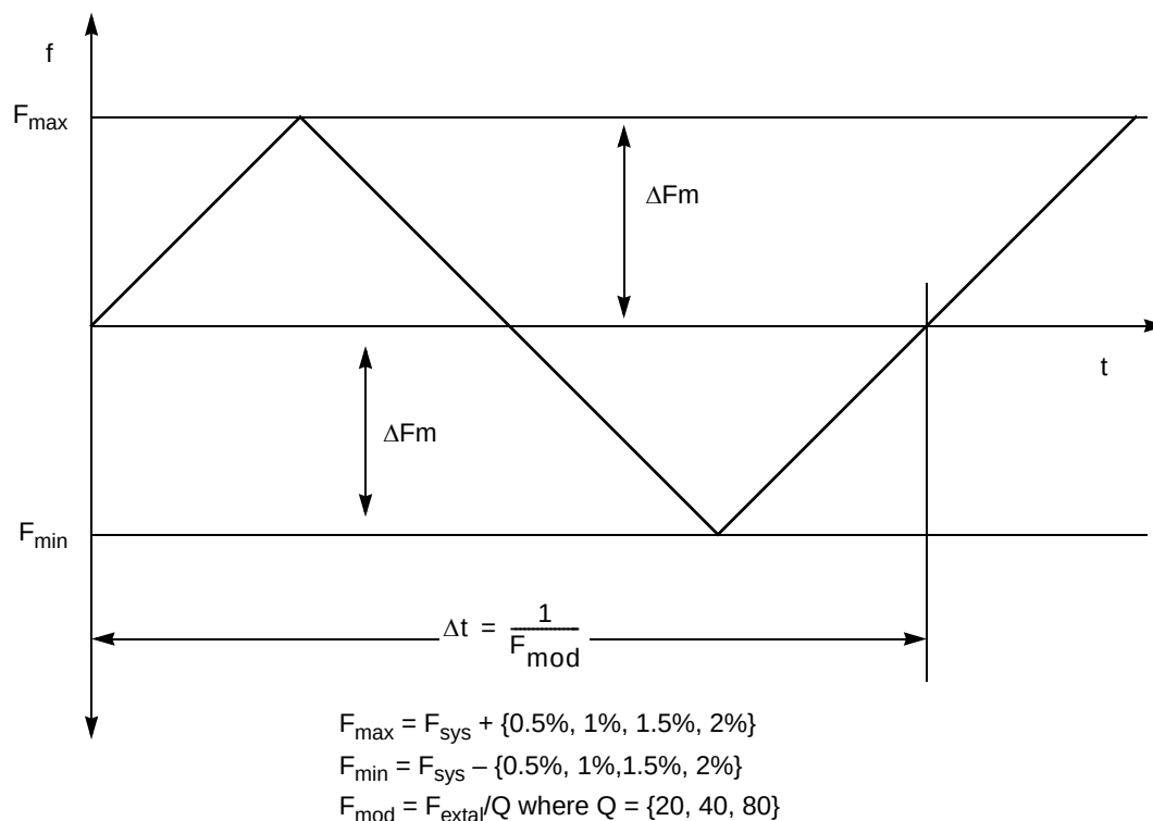
Figure 5-8. Frequency Modulation Waveform
