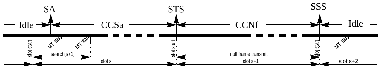
Figure 21-123. Null Frame Transmission from Idle state
