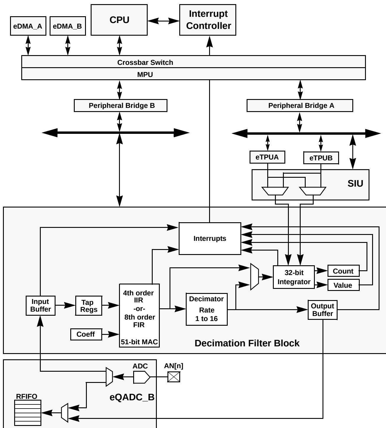
Figure 27-1. Decimation Filter Block Diagram
