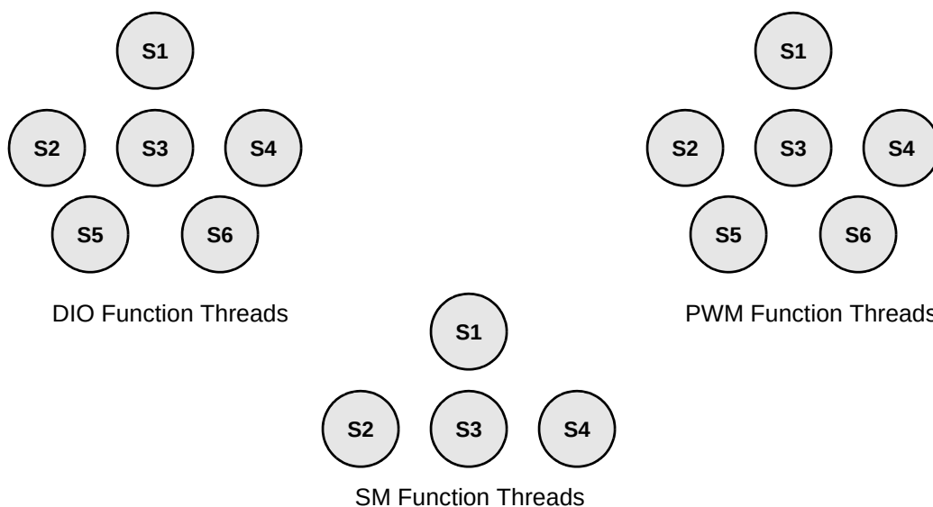
Figure 28-36. Function Threads
