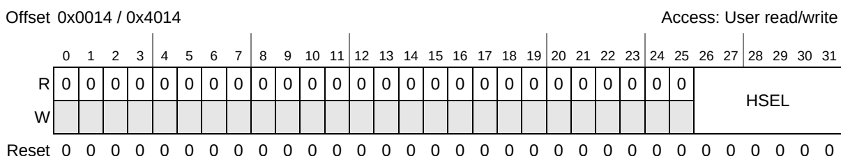
Figure 11-8. FLASH_x_HSR Register
