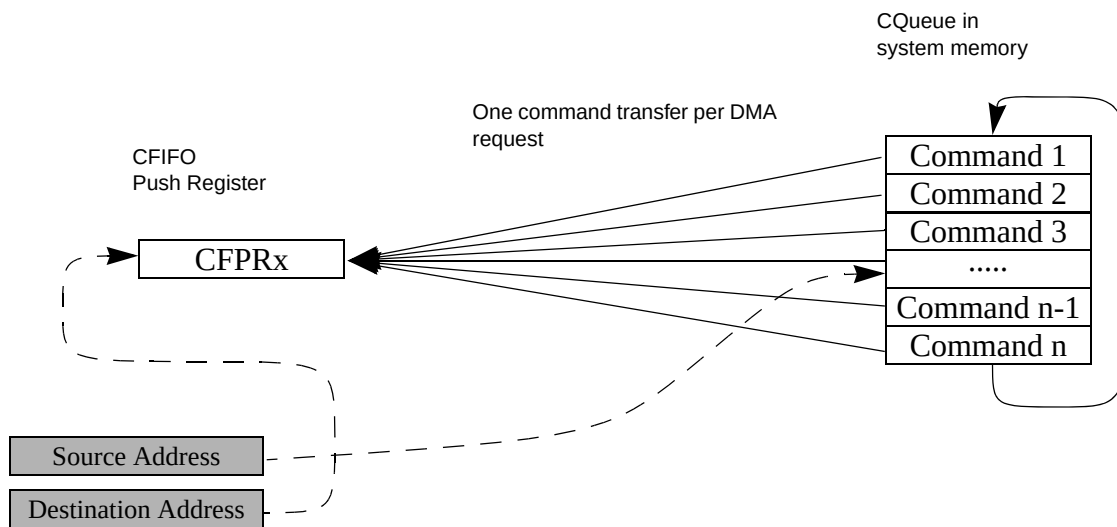
Figure 26-75. CQueue/CFIFO Interface
