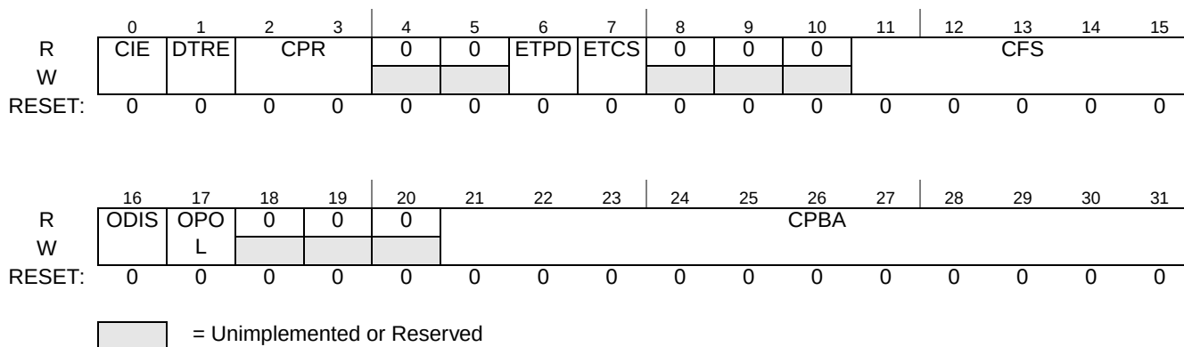
Figure 28-24. ETPUCxCR Register
