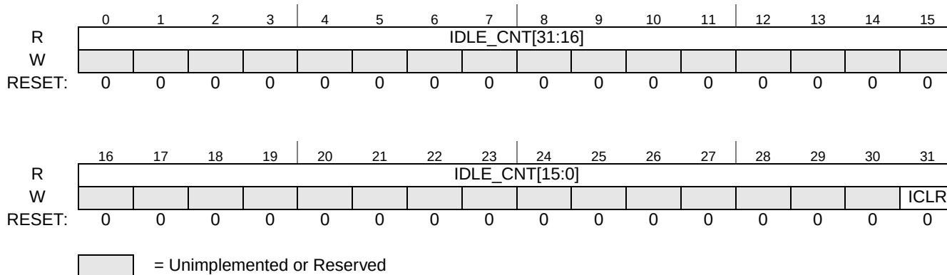
Figure 28-13. ETPUIDLER Register
