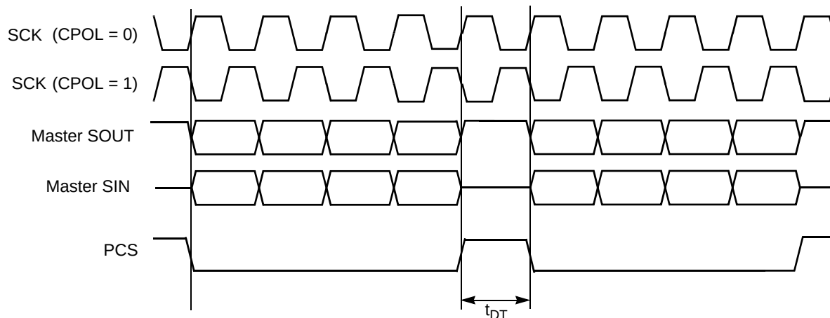
Figure 24-35. Continuous SCK Timing Diagram (CONT=0)
