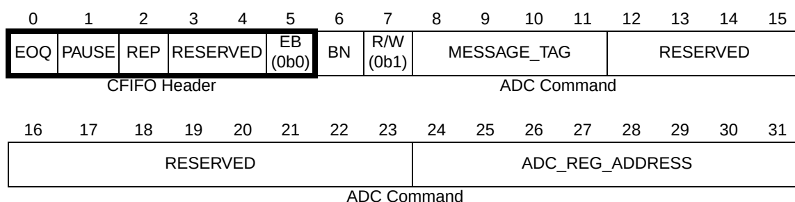
Figure 26-47. Read Configuration Command Format for On-Chip ADC Operation
