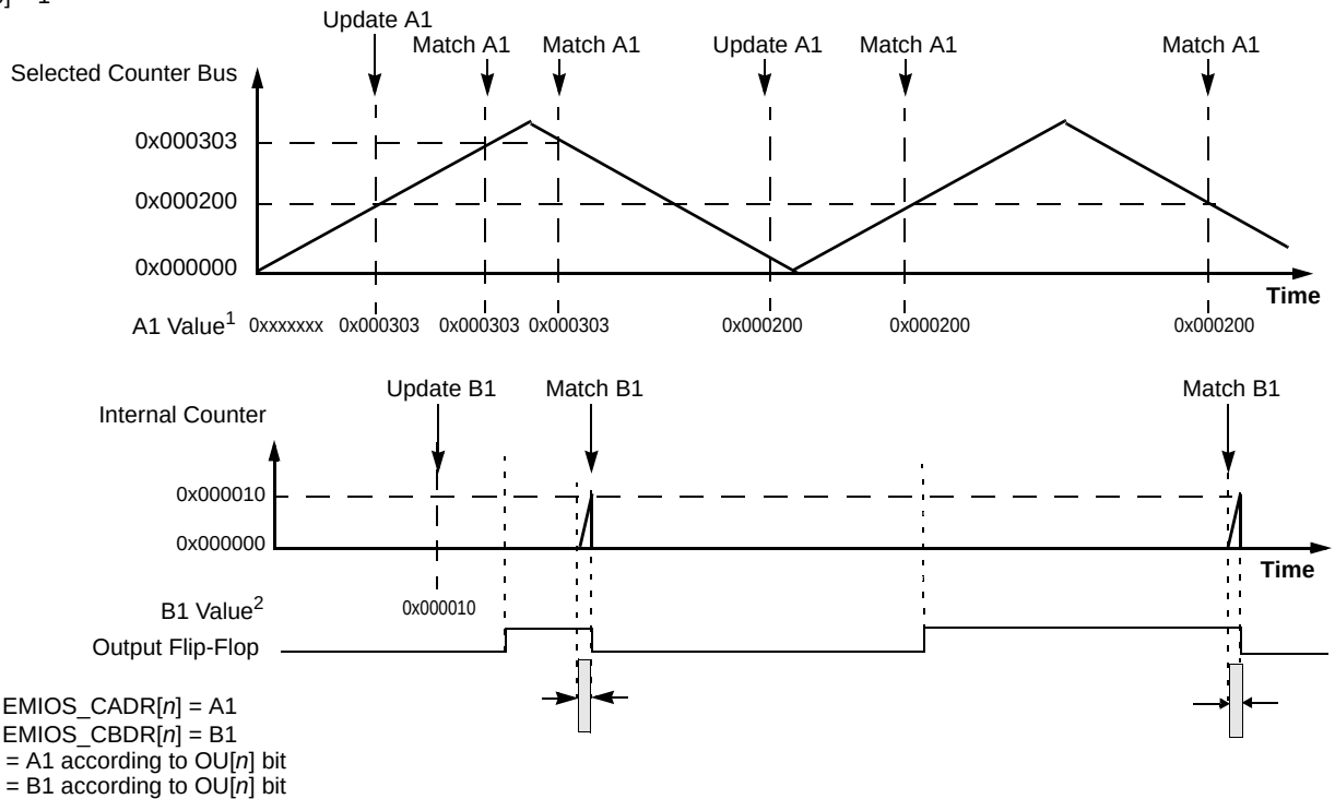
Figure 22-46. OPWMC with Trailing Dead Time Insertion
