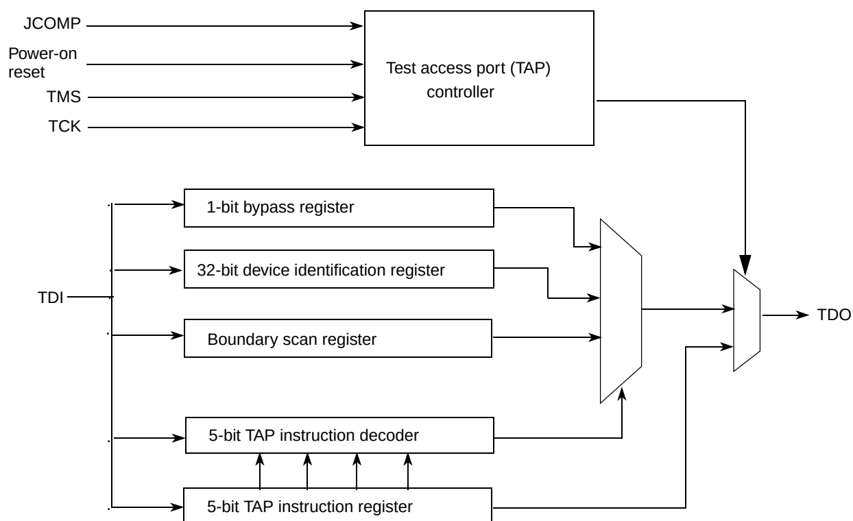
Figure 31-1. JTAG Controller Block Diagram
