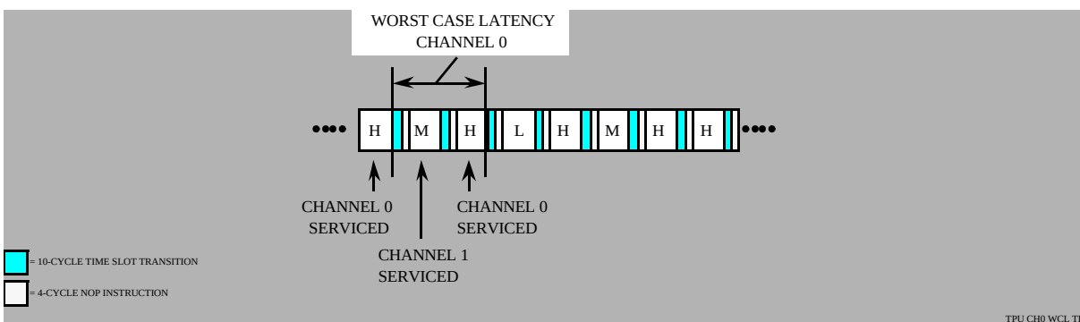
Figure 28-40. Next Servicing for Channel 0
