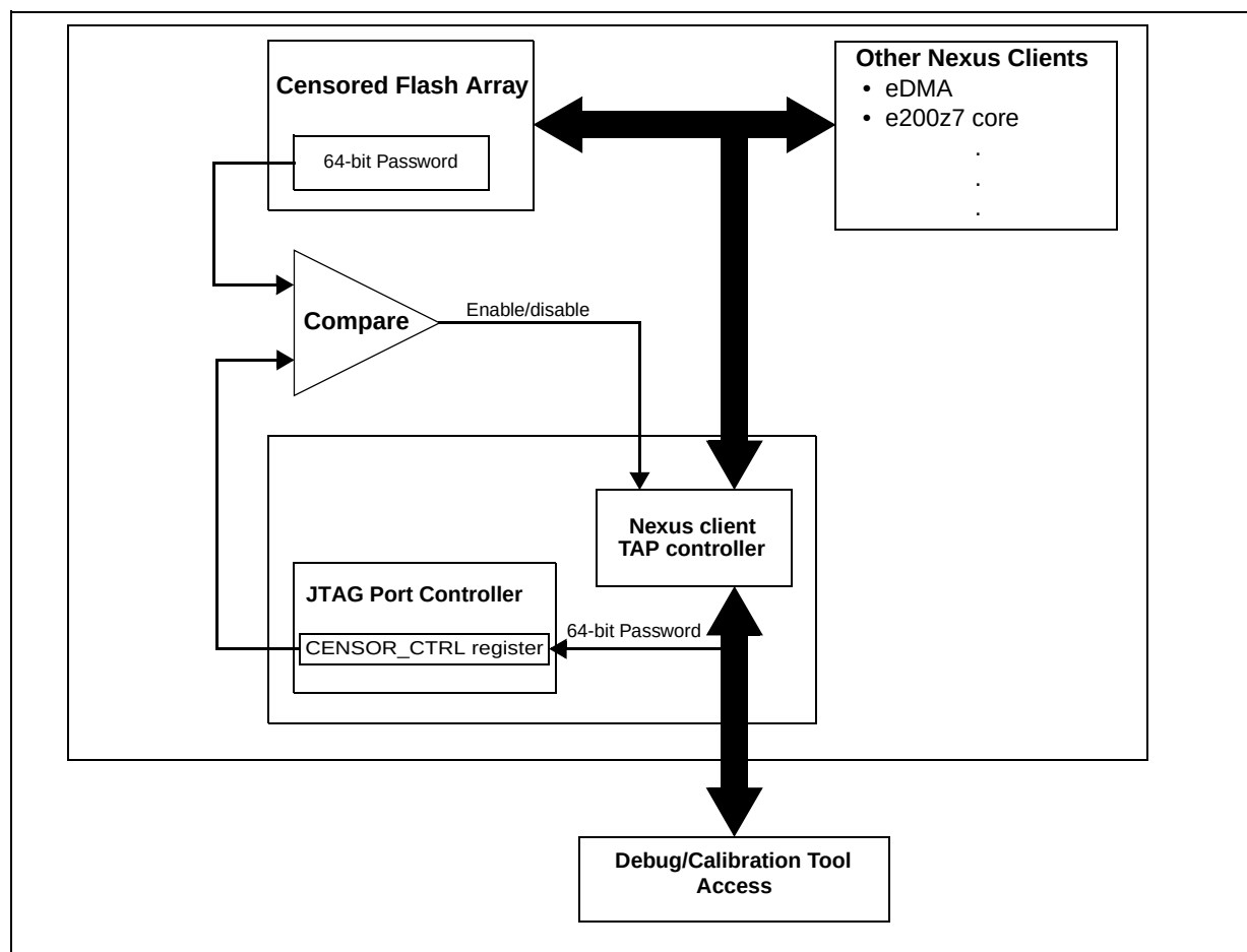
Figure 8-8. Enabling JTAG/Nexus port access on a censored device
