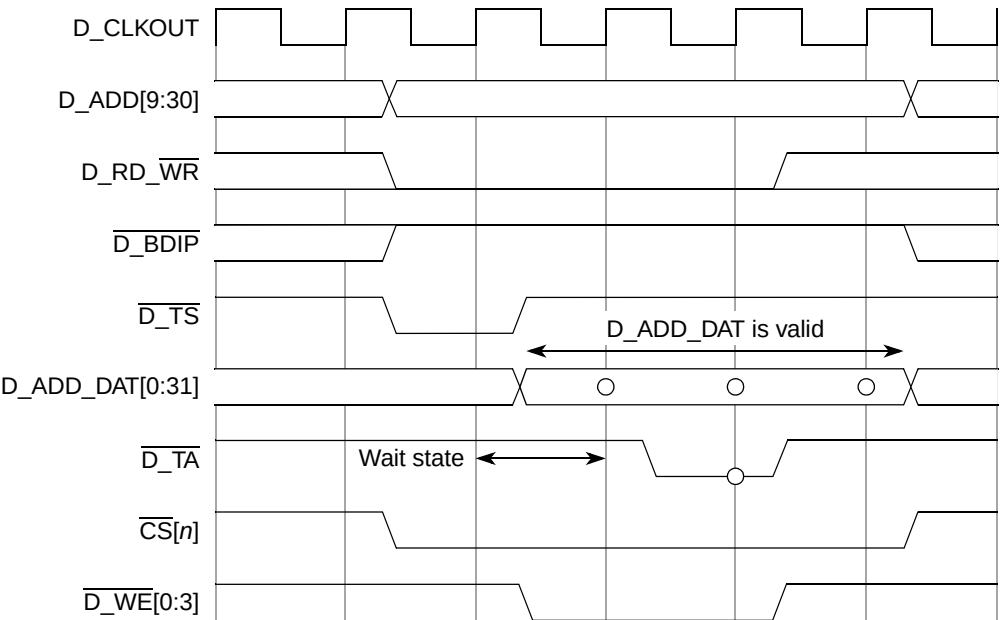
Figure 29-15. Single Beat 32-bit Write Cycle, \overline{CS} Access, One Wait State
