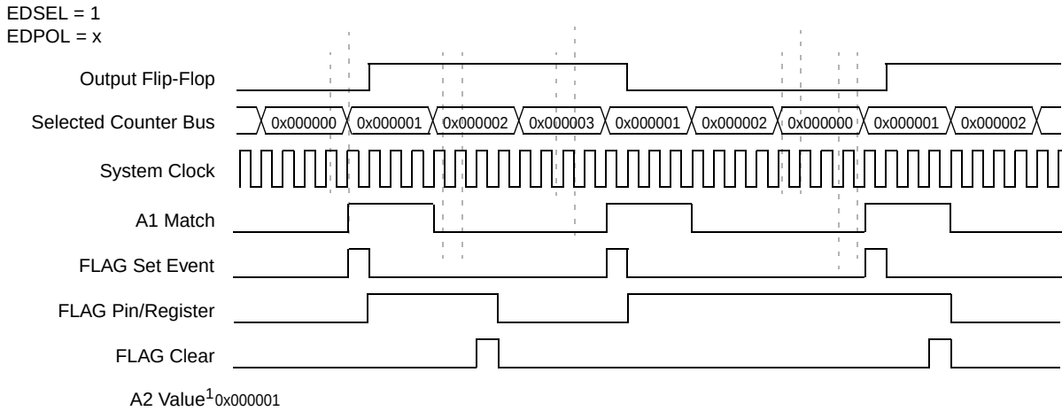
Figure 22-17. SAOC Example with Flag Behavior
