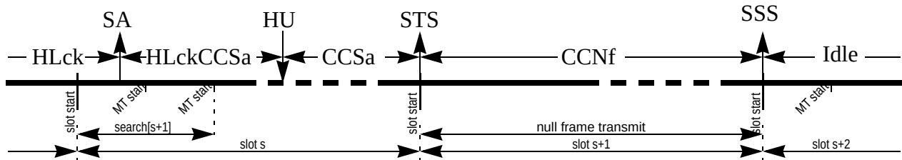
Figure 21-125. Null Frame Transmission from HLck state with unlock
