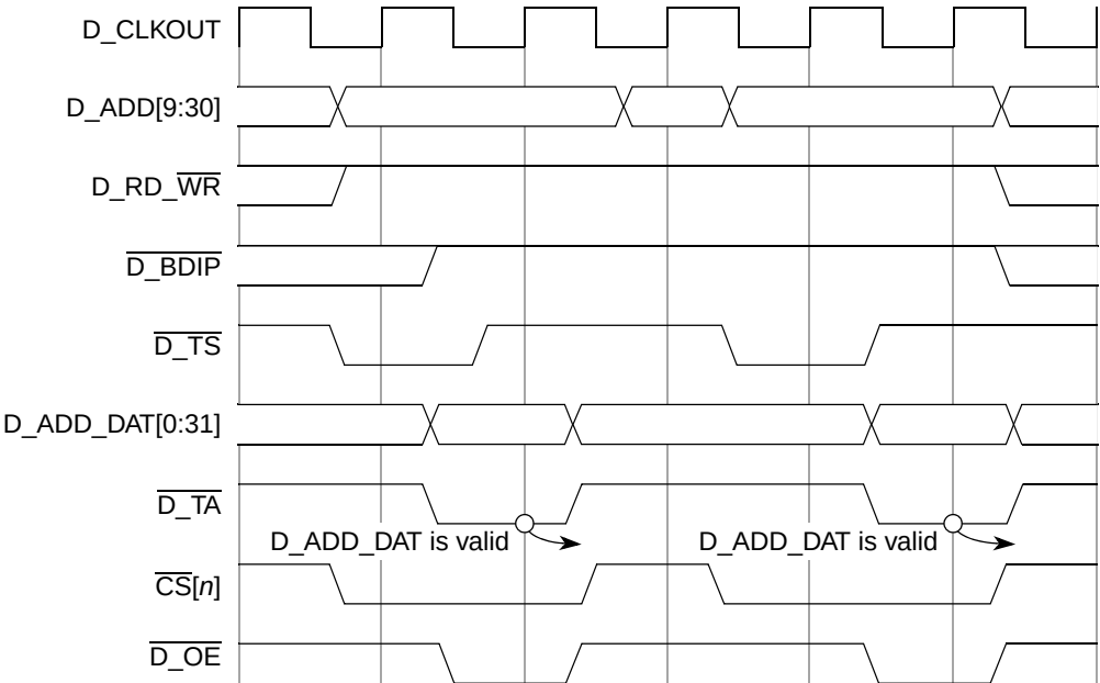
Figure 29-17. Back-to-Back 32-bit Reads to the Same \overline{CS} Bank
