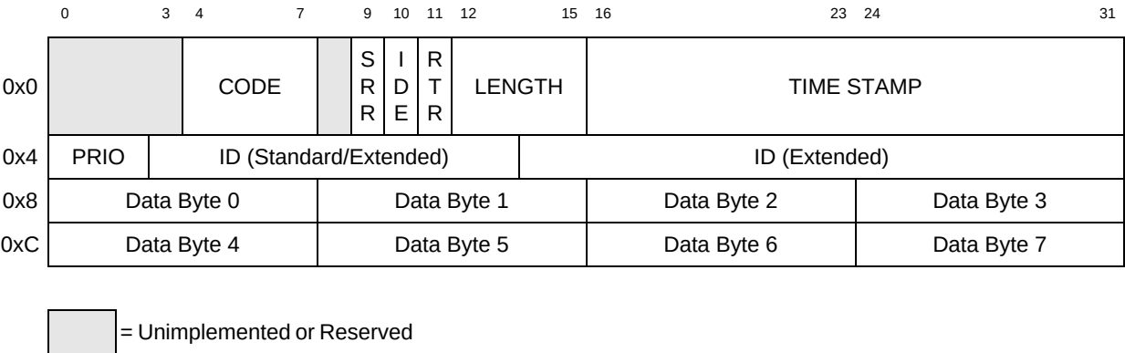
Figure 23-2. Message Buffer Structure
