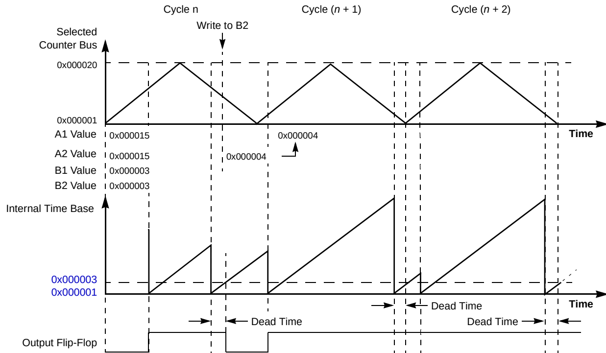
Figure 22-50. OPWMCB with 100% Duty Cycle (A1 = 4 and B1 = 3)
