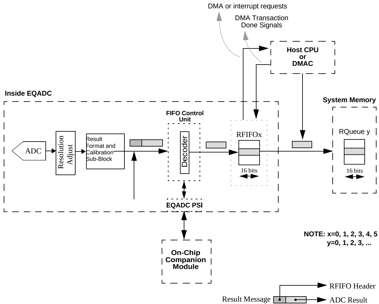
Figure 26-43. Result Flow during EQADC operation
