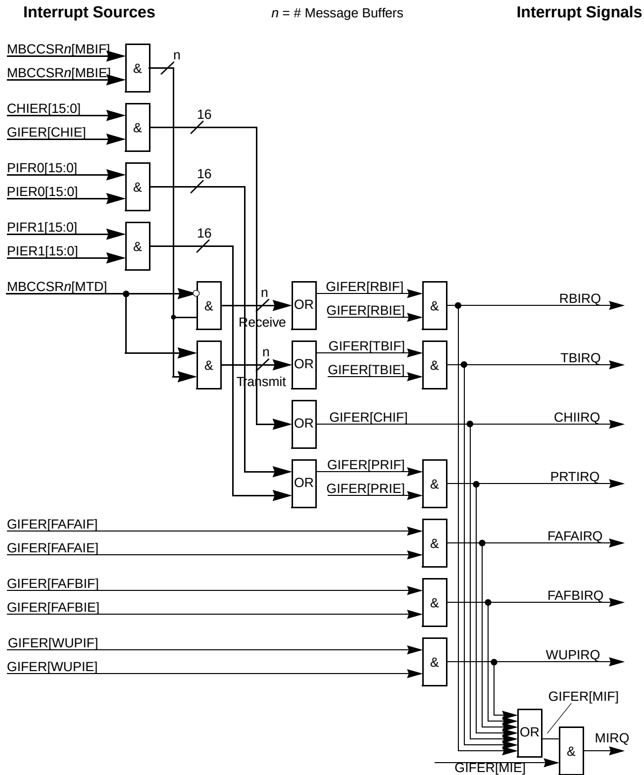
Figure 21-150. Scheme of cascaded interrupt request
