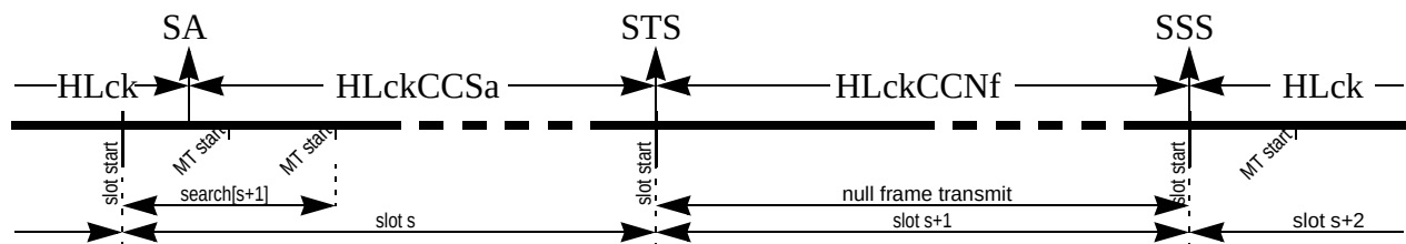
Figure 21-124. Null Frame Transmission from HLck state
