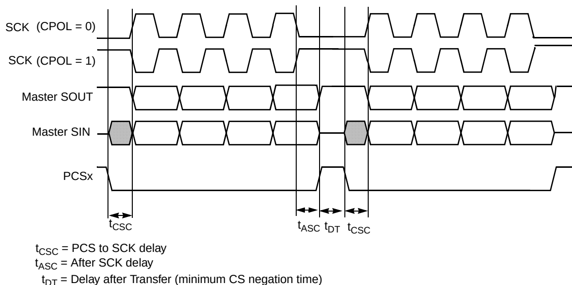
Figure 24-33. Example of Non-Continuous Format (CPHA=1, CONT=0)
