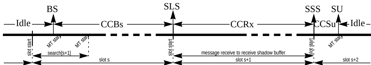
Figure 21-129. Message Reception Timing
