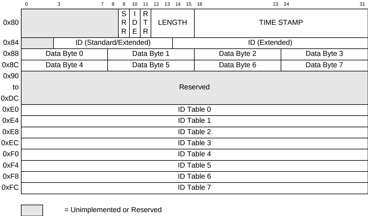
Figure 23-3. Rx FIFO Structure
