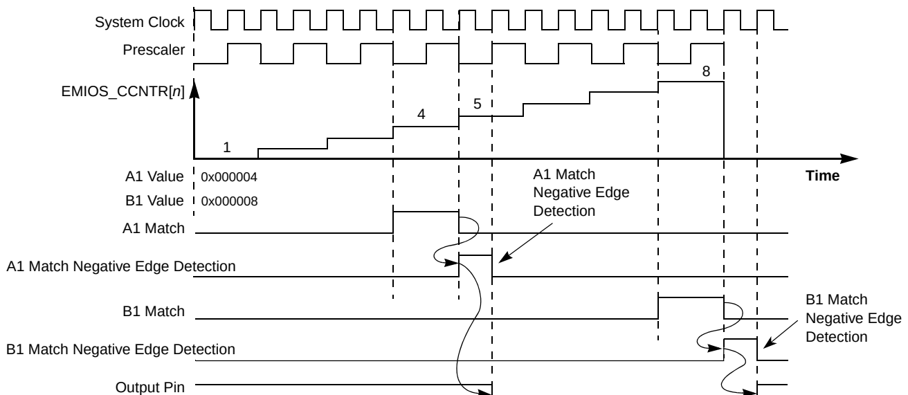
Figure 22-40. OPWFMB A1 and B1 Match to Output Register Delay
