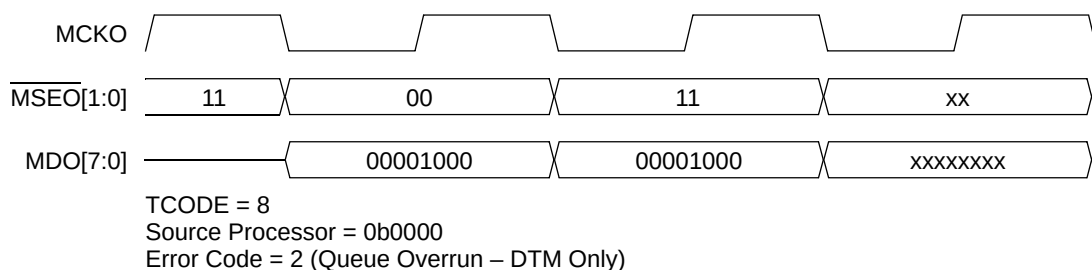
Figure 30-36. Error Message (Data Trace only encoded)
