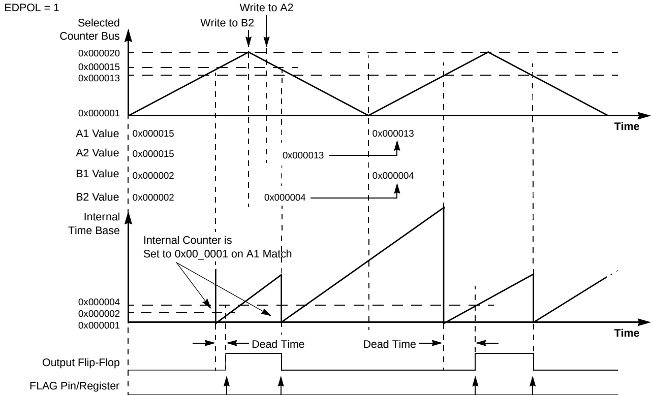
Figure 22-48. OPWMCB with Leading Dead Time Insertion
