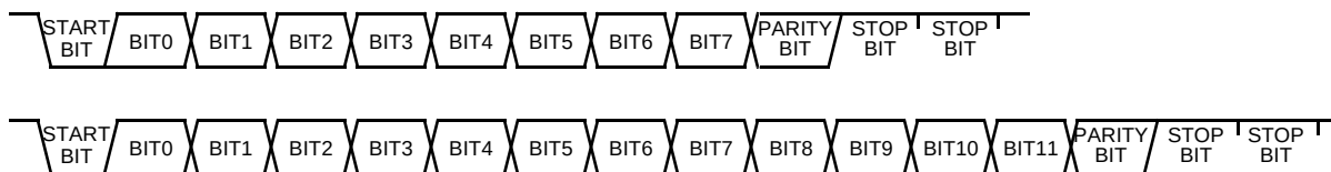
Figure 25-18. SCI Frame Formats (2 stop bits)
