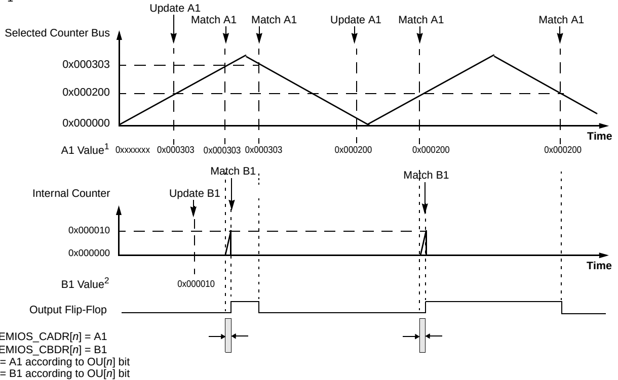
Figure 22-45. OPWMC with Leading Dead Time Insertion
