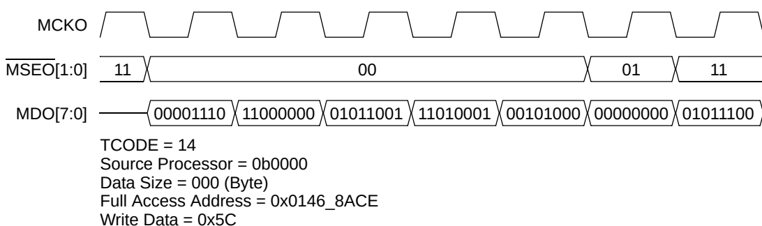
Figure 30-35. Data Trace—Data Read with Sync Message
