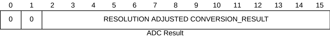
Figure 26-49. ADC Result Format when FMT=0 (Right Justified Unsigned)
