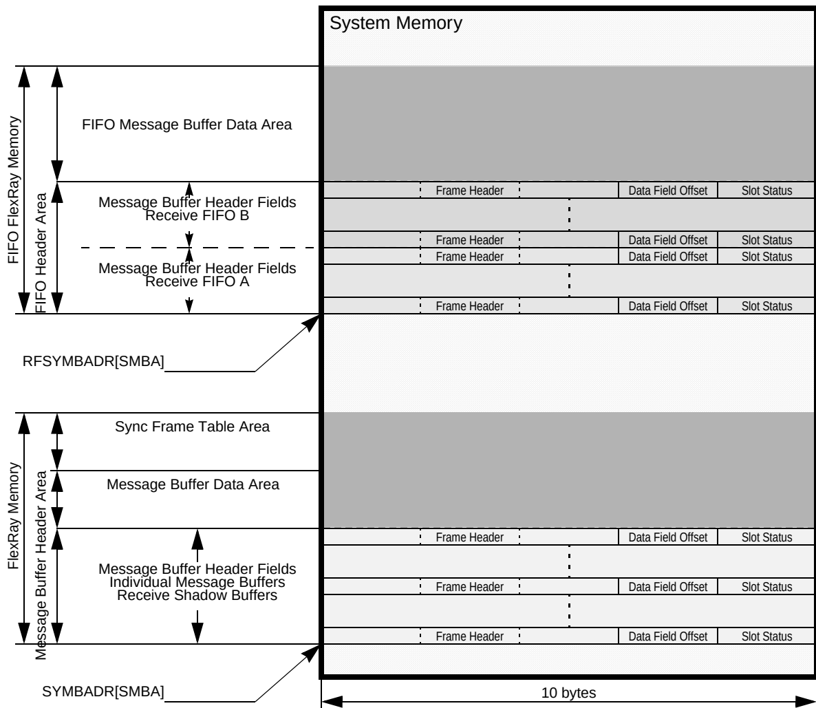
Figure 21-108. Example of FlexRay Memory Layout (MCR[FAM] = 1)
