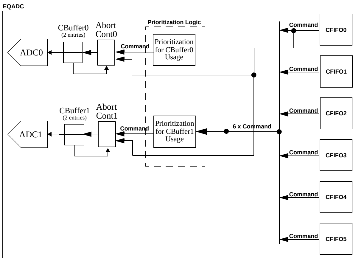
Figure 26-55. CFIFO Prioritization Logic
