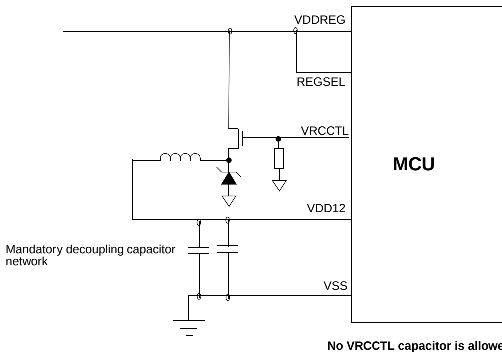
Figure 4-11. VRC 1.2V buck SMPS LDO configuration with external MOS - Schottky diode
