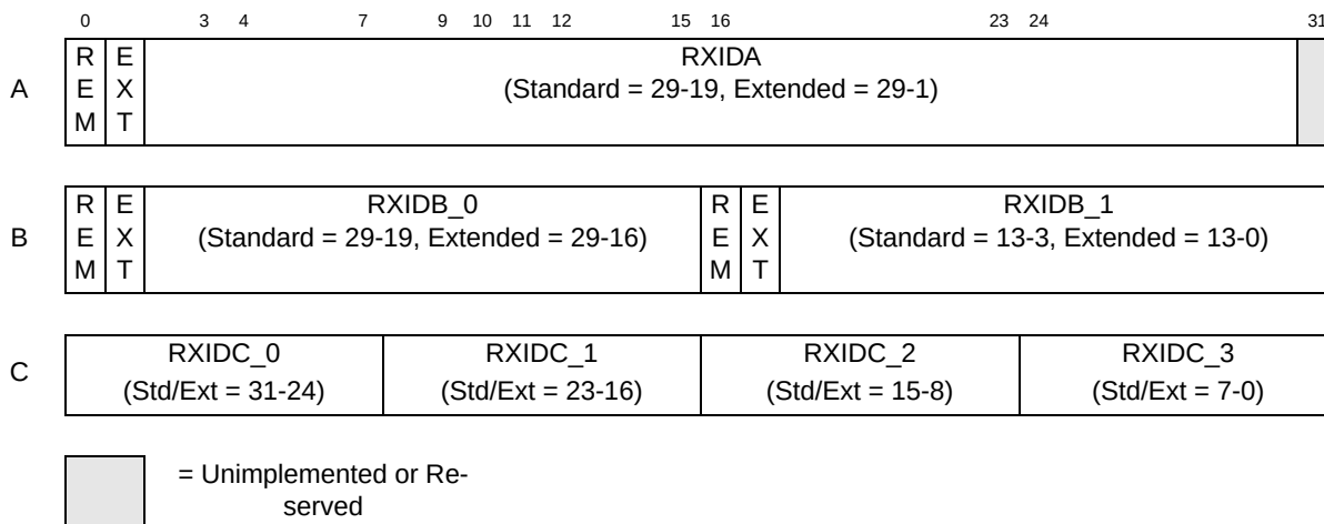
Figure 23-4. ID Table 0 - 7
