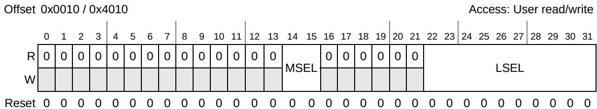
Figure 11-7. FLASH_x_LMSR Register
