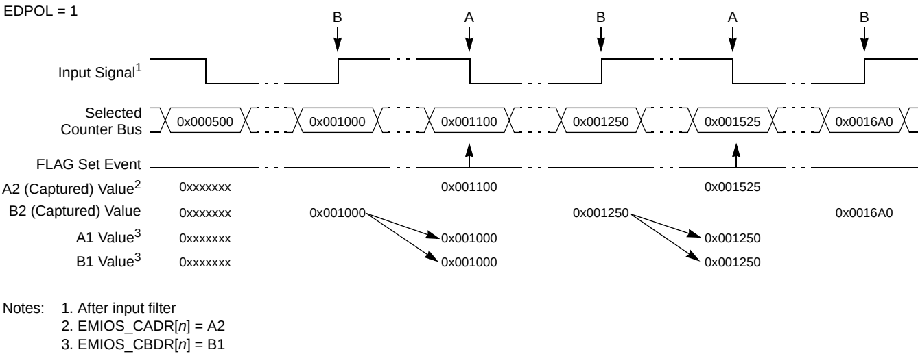
Figure 22-18. IPWM Example
