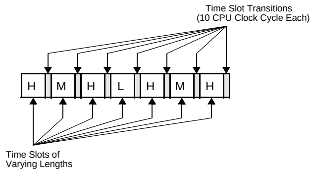
Figure 28-37. Time-Slot Sequence
