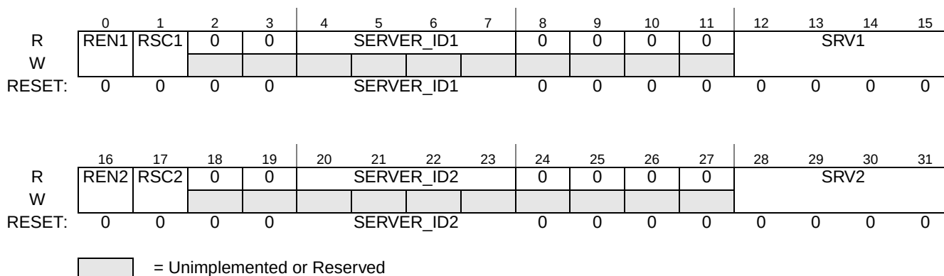
Figure 28-11. ETPUREDCCR Register
