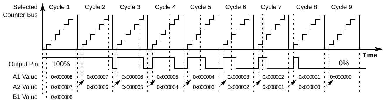
Figure 22-56. OPWMB Mode from 100% to 0% Duty Cycle
