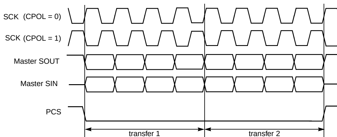
Figure 24-36. Continuous SCK Timing Diagram (CONT=1)
