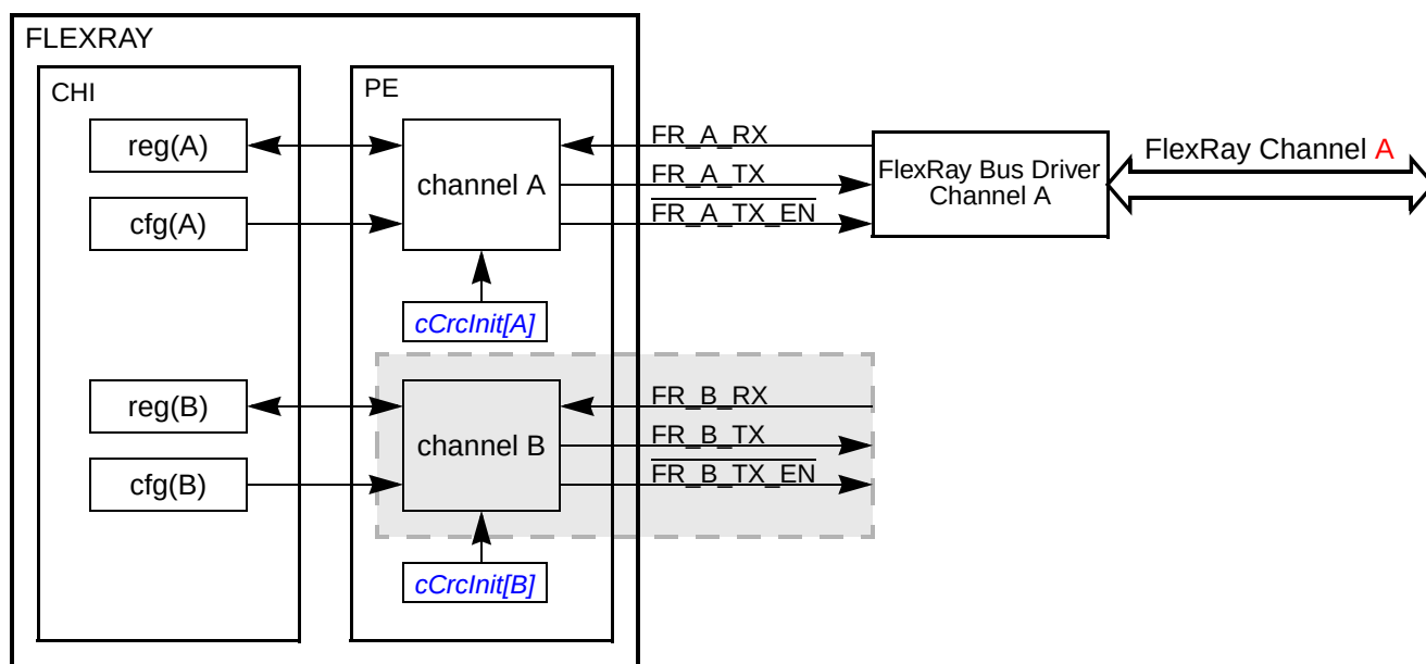
Figure 21-140. Single Channel Device Mode (Channel A)
