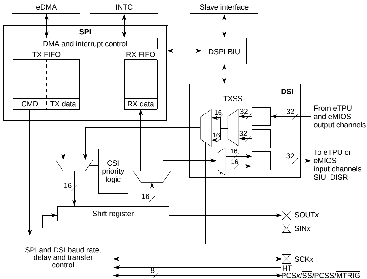
Figure 24-1. DSPI Block Diagram
