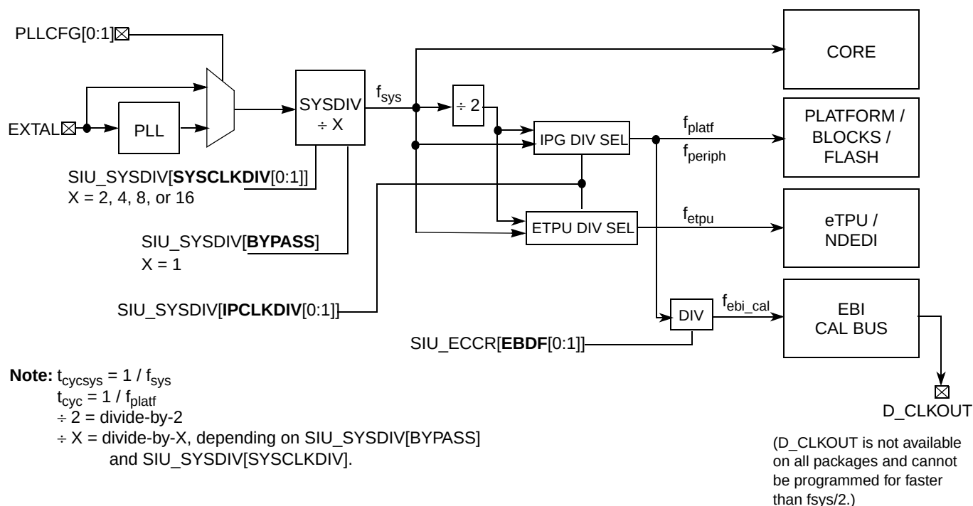
Figure 5-1. MPC5674F Block Operating Frequency Domain Diagram
