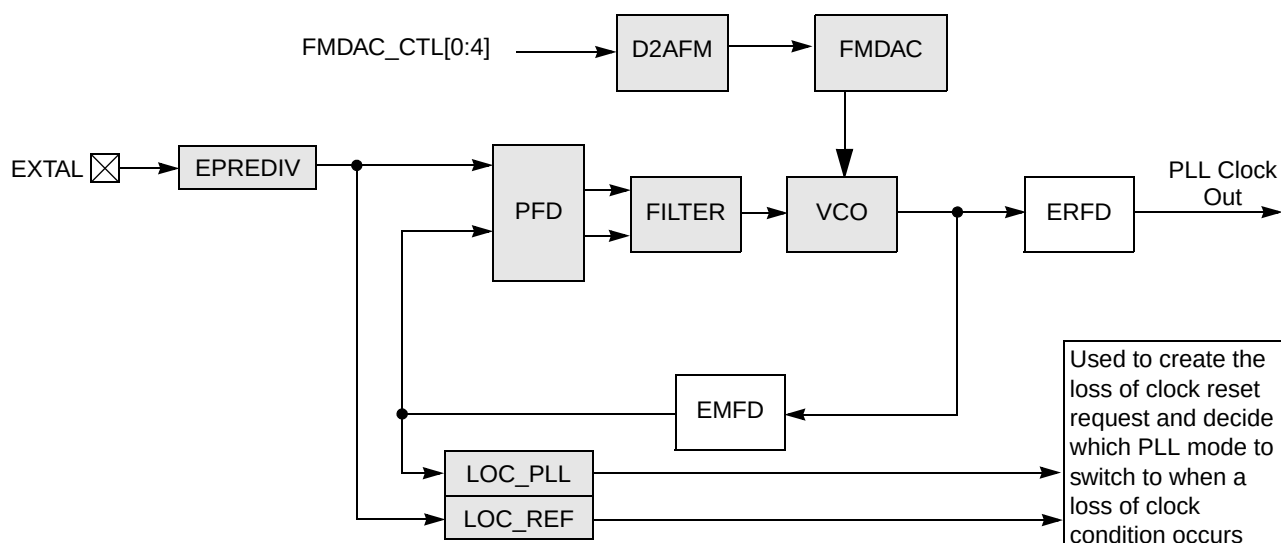
Figure 5-2. FMPLL Block Diagram
