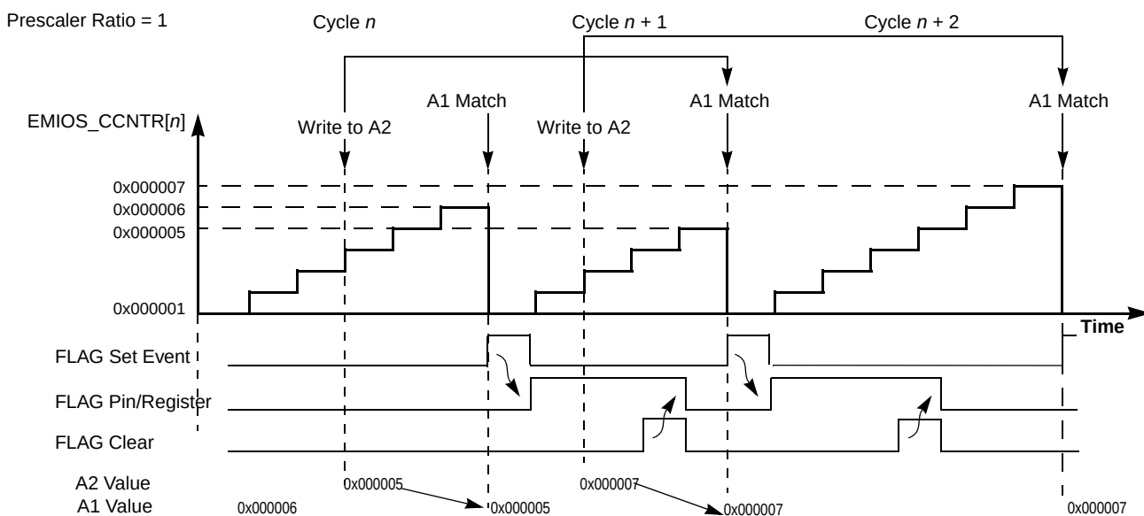
Figure 22-34. Modulus Counter Buffered (MCB) Up Count Mode
