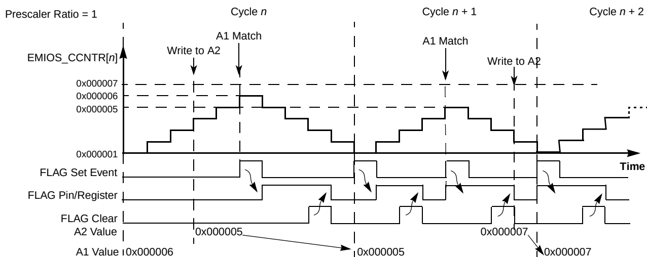
Figure 22-35. MCB Up/Down Mode
