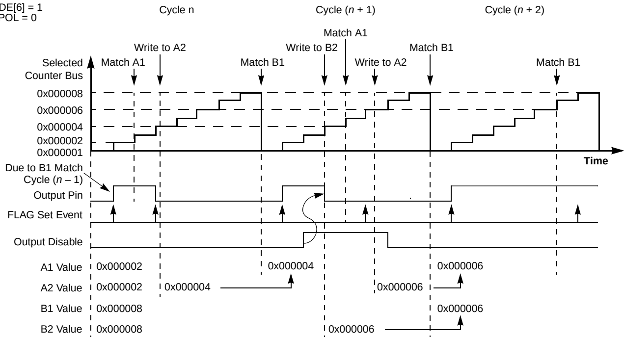
Figure 22-55. OPWMB Mode with Active Output Disable
