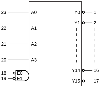
Fig 2. Logic symbol
