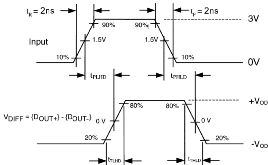
Figure 3. AC Waveforms
