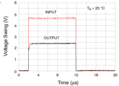
Figure 15. Pulse Response
