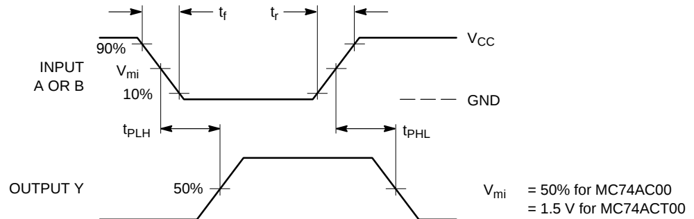
Figure 3. Switching Waveforms
