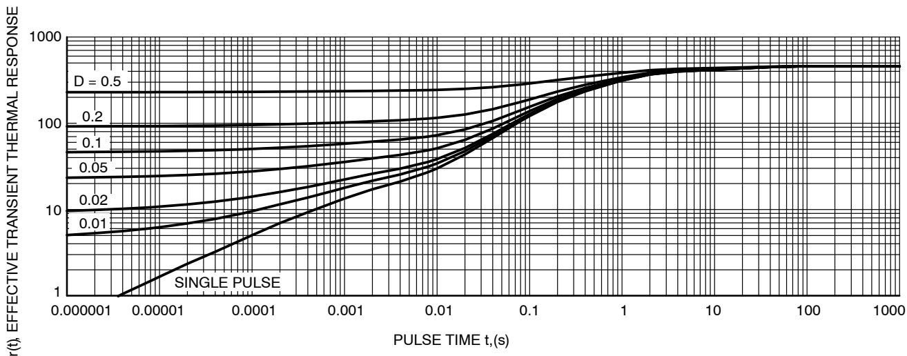
Figure 10. Thermal Response
