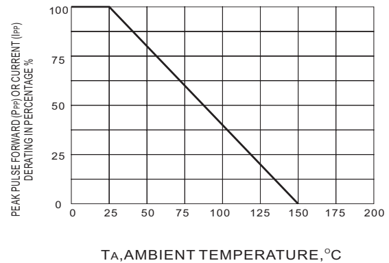
Fig.2 DERATING CURVE
