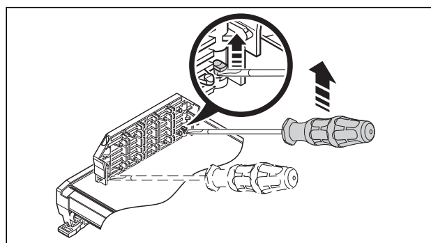
Figure 30 Removing the lateral elements
