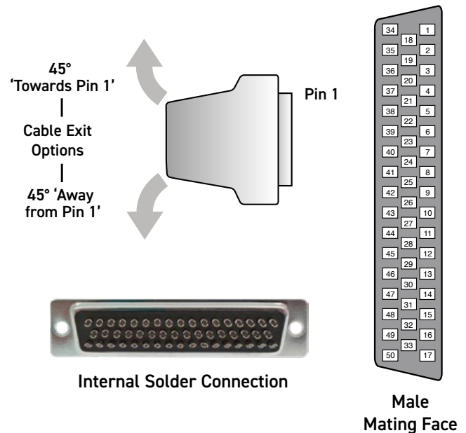
50-Pin D-Type Connector with Backshell
