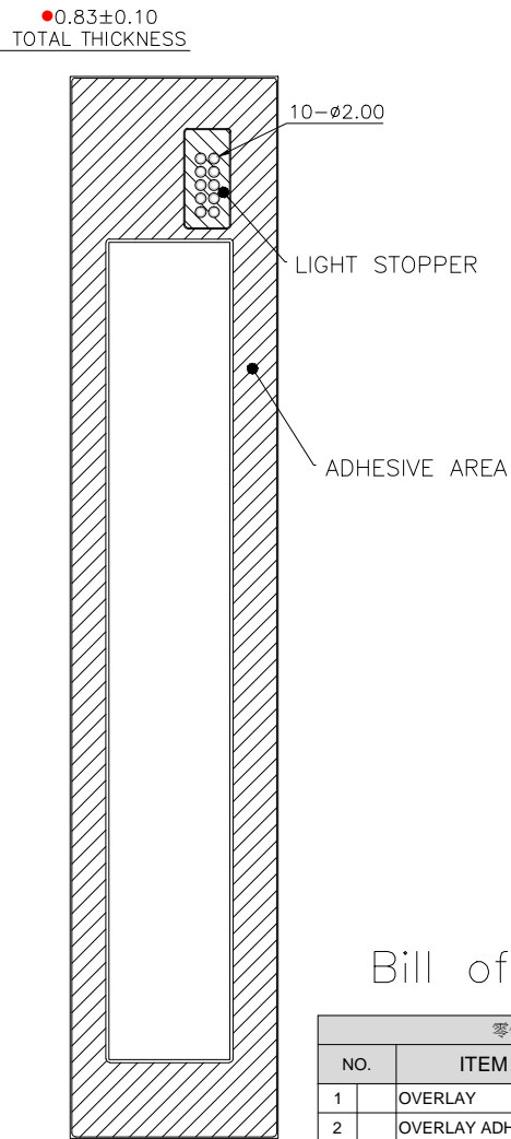
BACK VIEW
