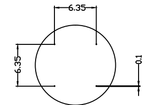
Detail C - DOT SPEC
